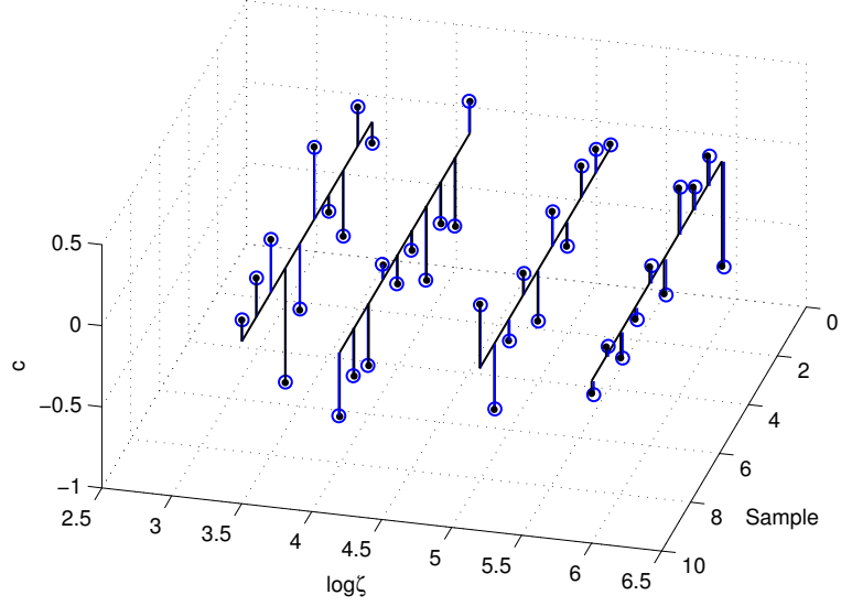
Figure 30: Theoretical and MMV-estimated DSRF of a four-relaxation target. The solid lines indicate the true relaxation frequencies. The stems with solid dots are the actual spectra; stems with hollow circle markers are the estimates.
