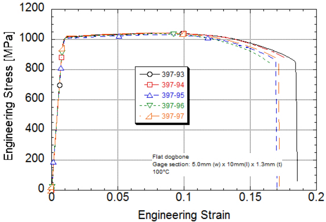
Ti 6-2-4-2S Engineering Stress-strain Post-yield strain rate of 11/s Machine rate of 125 mm/s DIC specimens 100°C
