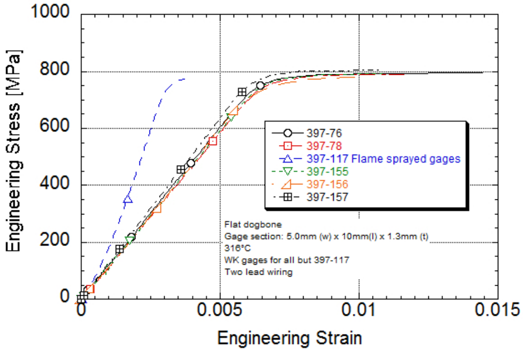
Ti 6-2-4-2S Engineering Stress-strain Post-yield strain rate of 10/s Machine rate of 120 mm/s Strain gaged specimens 316°C
