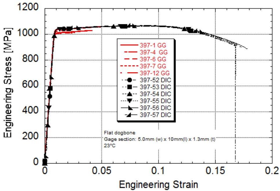
Ti 6-2-4-2S Engineering Stress-strain Post-yield strain rate of 0.1/s Machine rate of 1 mm/s Strain gaged and DIC specimens 23°C
