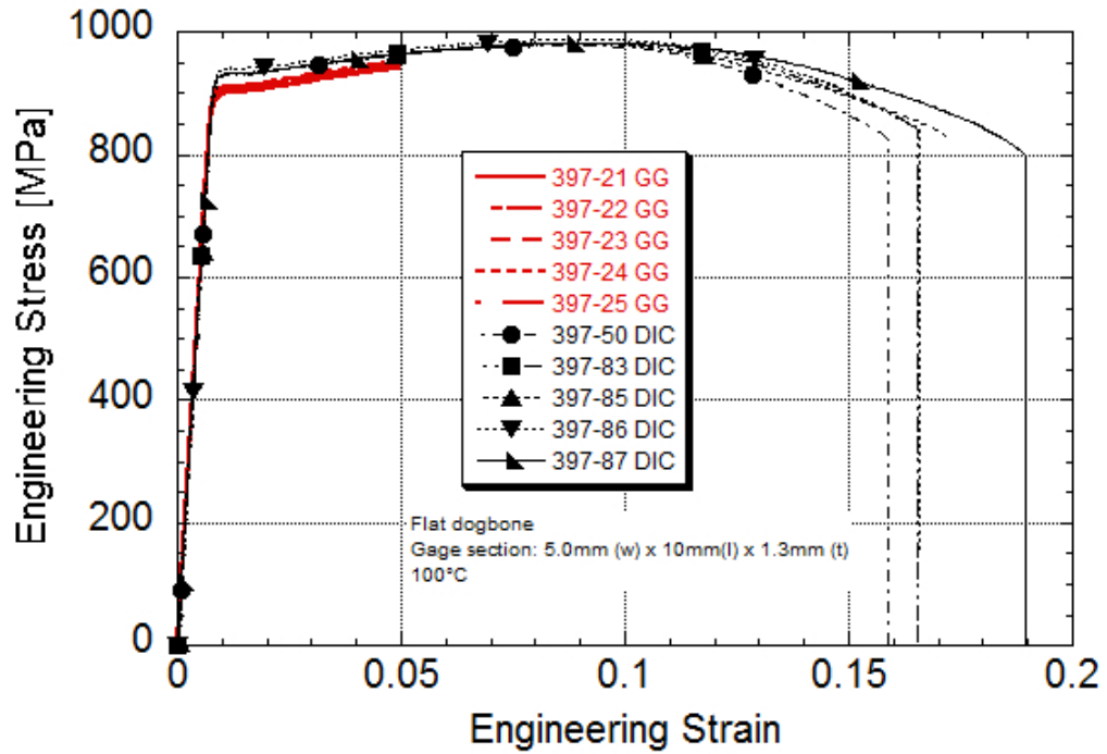
Ti 6-2-4-2S Engineering Stress-strain Post-yield strain rate of 0.1/s Machine rate of 1 mm/s Strain gaged and DIC specimens 100°C
