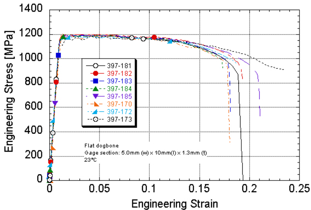
Ti 6-2-4-2S Engineering Stress-strain Post-yield strain rate of 100-150/s Machine rate of 1.8 m/s Digital image correlation specimens 23°C
