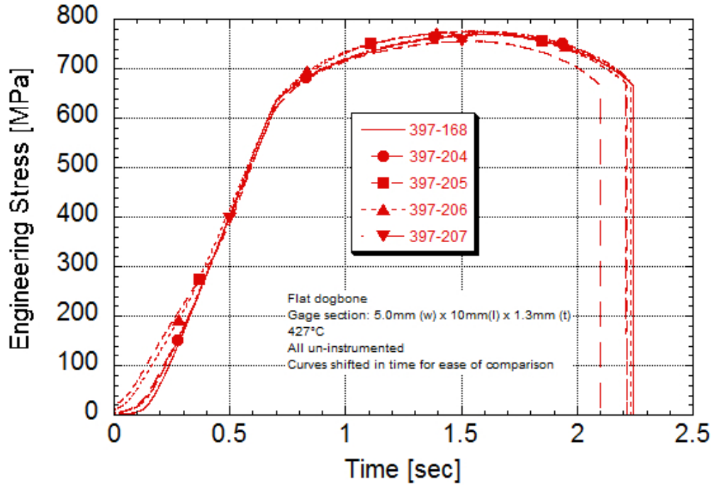
Ti 6-2-4-2S Engineering Stress versus Time Post-yield strain rate of 1.1/s Machine rate of 11 mm/s 427°C
