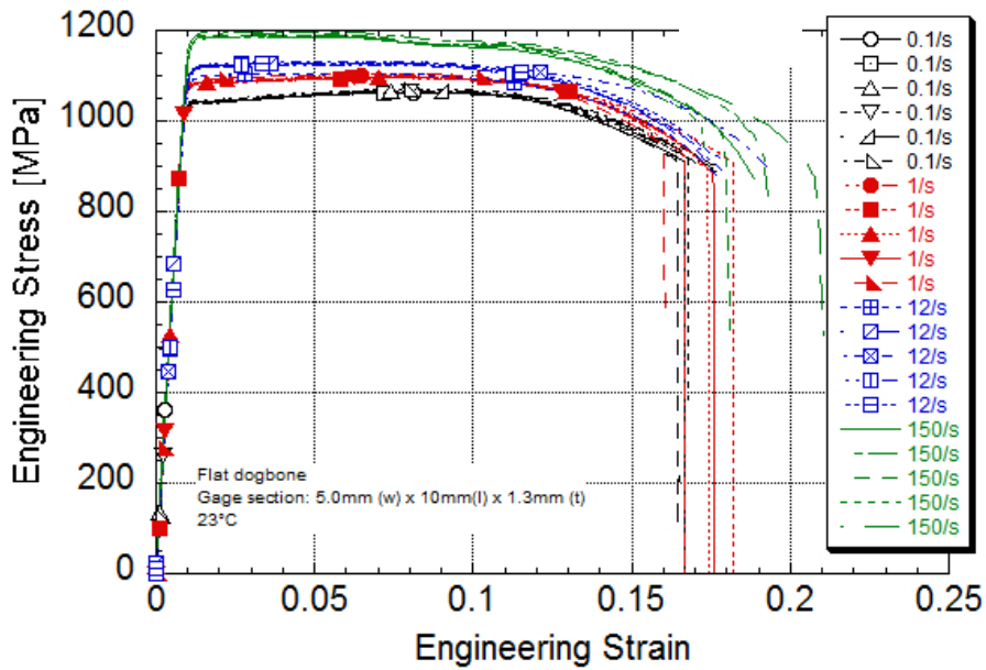
Ti 6-2-4-2S Engineering Stress-strain Digital image correlation specimens Post-yield engineering strain rates 23°C
