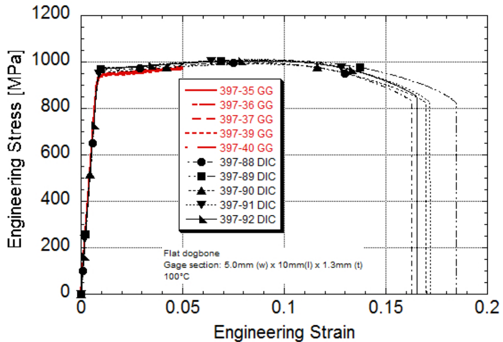
Ti 6-2-4-2S Engineering Stress-strain Post-yield strain rate of 1/s Machine rate of 11 mm/s Strain gaged and DIC specimens 100°C
