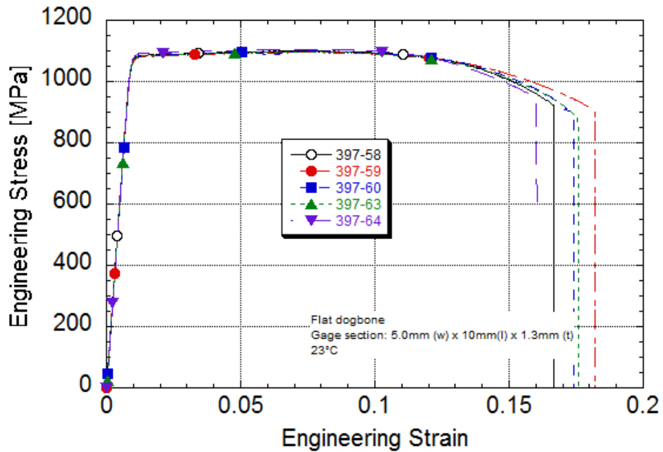
Ti 6-2-4-2S Engineering Stress-strain Post-yield strain rate of 1/s Machine rate of 11 mm/s Digital image correlation specimens 23°C
