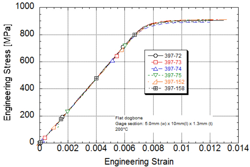
Ti 6-2-4-2S Engineering Stress-strain Post-yield strain rate of 10/s Machine rate of 120 mm/s Strain gaged specimens 200°C
