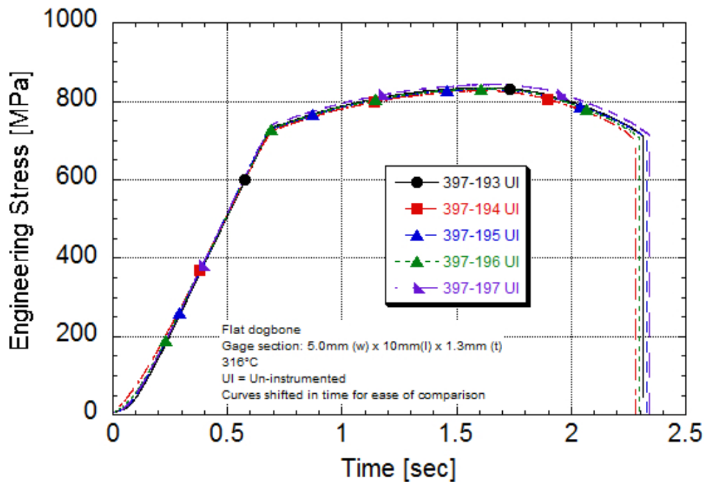
Ti 6-2-4-2S Engineering Stress versus Time Post-yield strain rate of 0.1/s Machine rate of 1.1 mm/s 316°C
