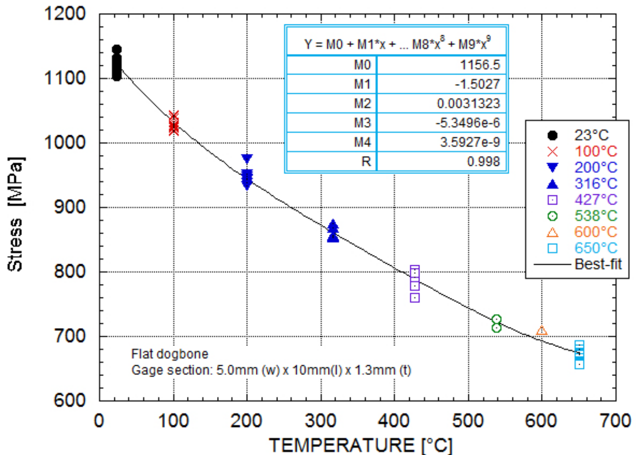
Figure 19. Effect of Increasing Temperature on the UTS of Ti 6-2-4-2S at 12/s
