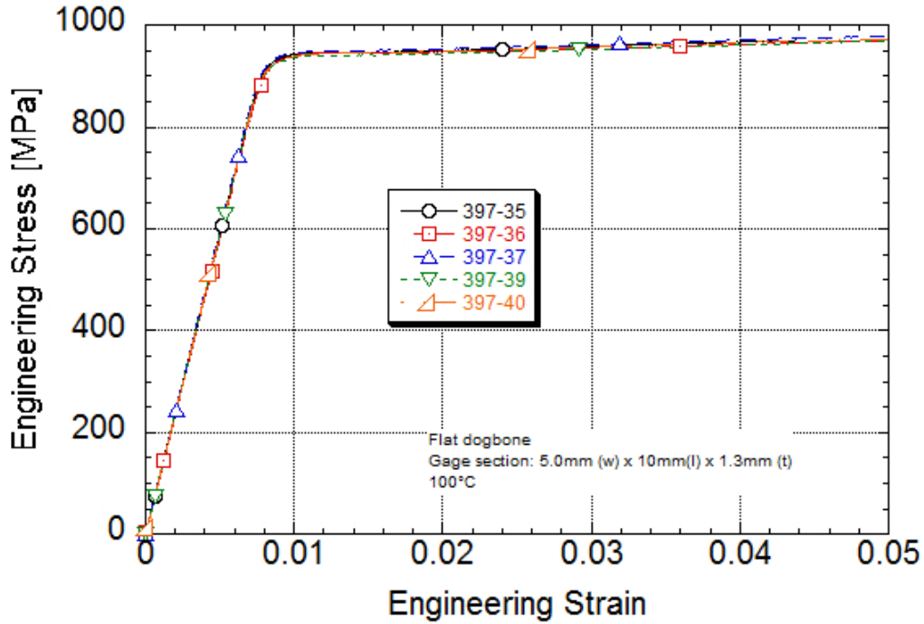
Ti 6-2-4-2S Engineering Stress-strain Post-yield strain rate of 1/s Machine rate of 12 mm/s Strain gaged specimens 100°C
