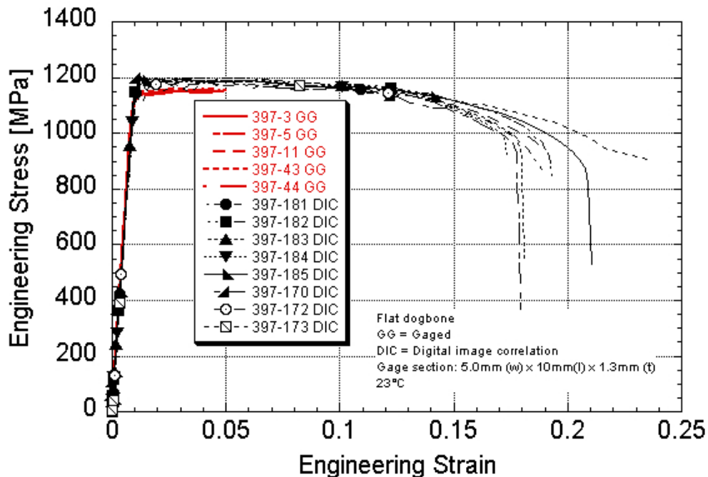
Ti 6-2-4-2S Engineering Stress-strain Post-yield strain rate of 150/s Machine rate of 1.8 m/s Strain gaged and DIC specimens 23°C
