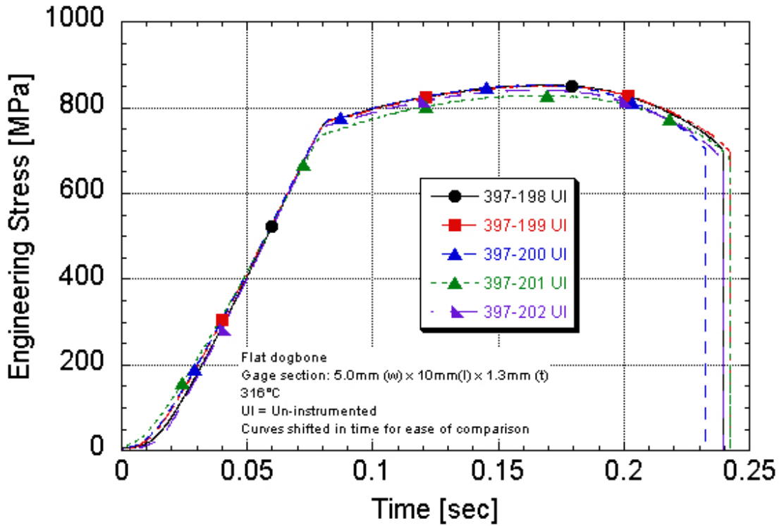
Ti 6-2-4-2S Engineering Stress versus Time Post-yield strain rate of 12/s Machine rate of 120 mm/s 316°C
