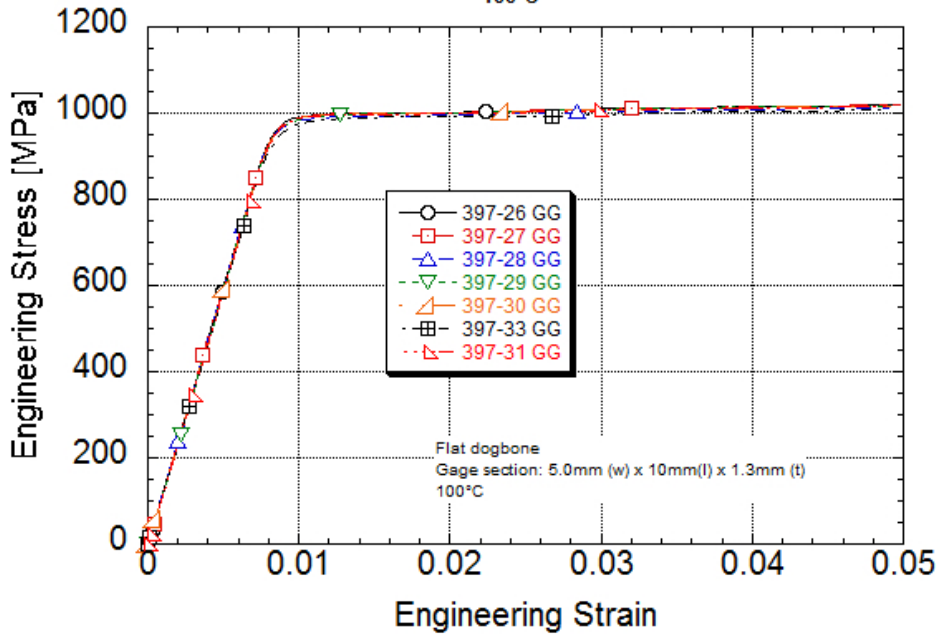
Ti 6-2-4-2S Engineering Stress-strain Post-yield strain rate of 10/s Machine rate of 120 mm/s Strain gaged specimens 100°C
