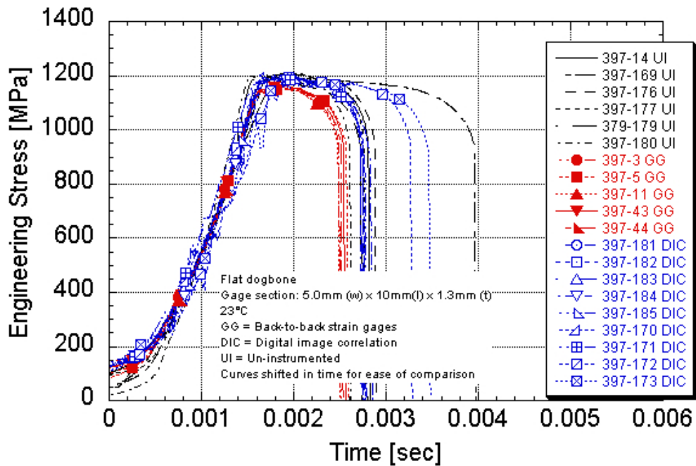
Ti 6-2-4-2S Engineering Stress versus Time Post-yield strain rate of 150/s Machine rate of 1.8 m/s 23°C
