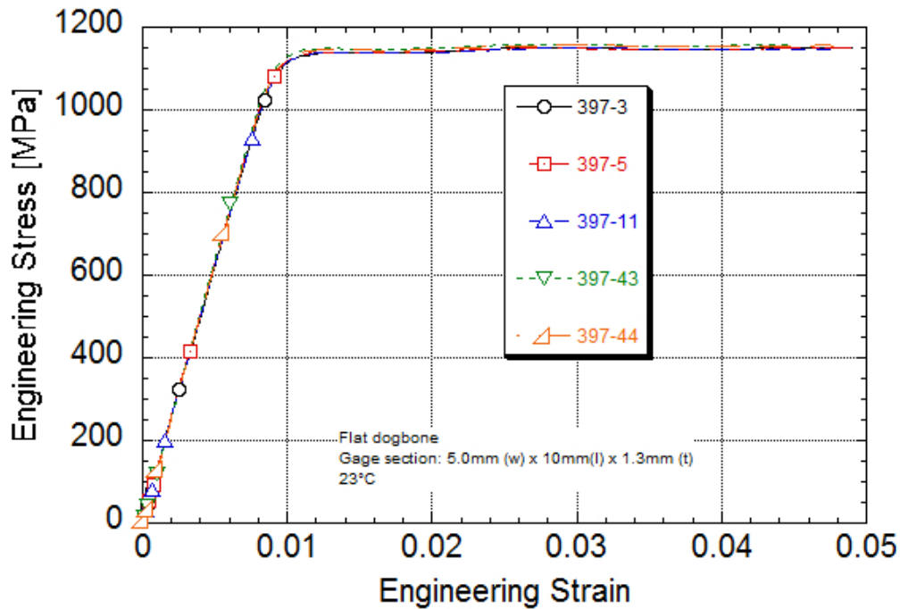
Ti 6-2-4-2S Engineering Stress-strain Post-yield strain rate of 100/s Machine rate of 1.8 m/s Strain gaged specimens 23°C
