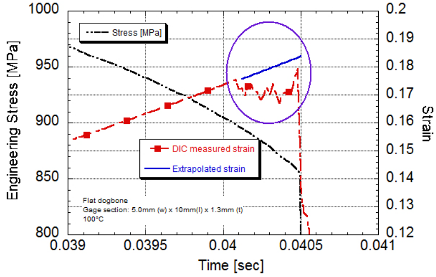
Figure 10. As-Measured and Extrapolated DIC Strain Before Fracture
