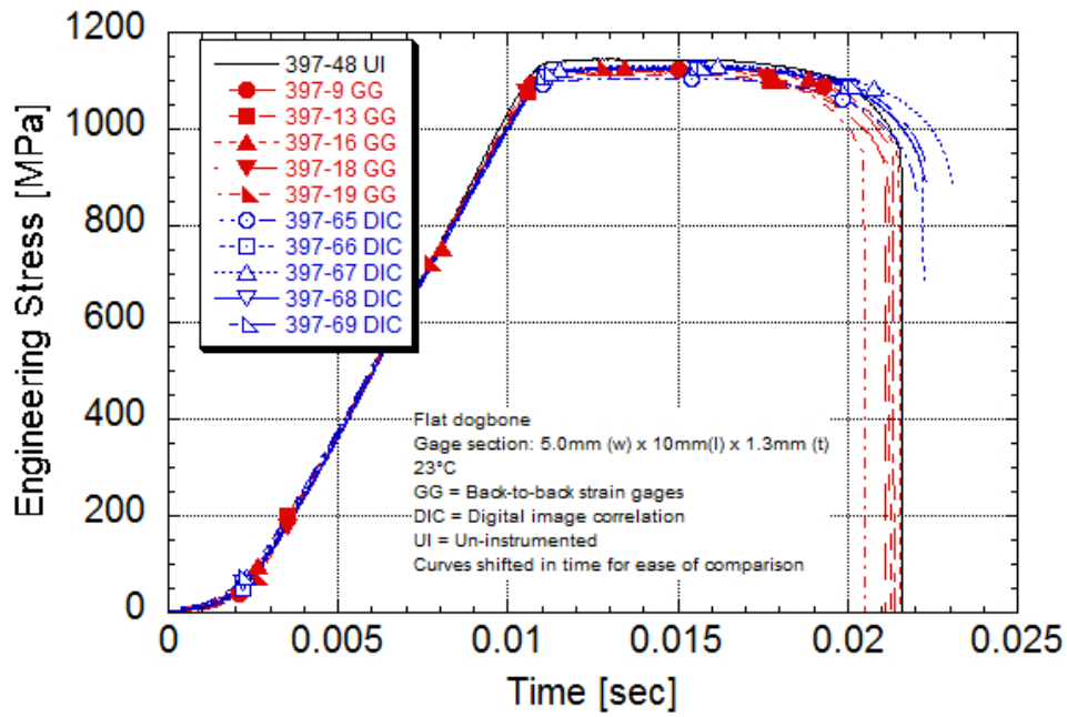
Ti 6-2-4-2S Engineering Stress versus Time Post-yield strain rate of 12/s Machine rate of 120 mm/s 23°C
