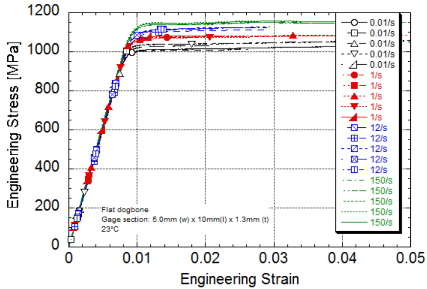
Ti 6-2-4-2S Engineering Stress-strain Strain gaged specimens Post-yield engineering strain rates 23°C
