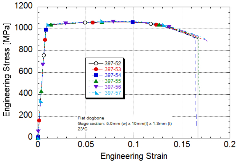
Ti 6-2-4-2S Engineering Stress-strain Post-yield strain rate of 0.1/s Machine rate of 1 mm/s Digital image correlation runs
