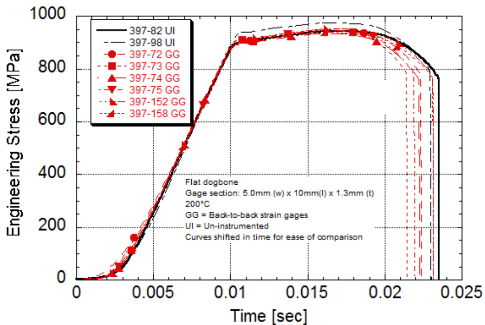
Ti 6-2-4-2S Engineering Stress versus Time Post-yield strain rate of 11/s Machine rate of 120 mm/s 200°C
