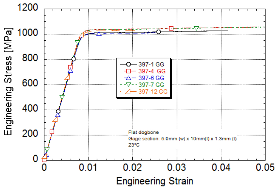
Ti 6-2-4-2S Engineering Stress-strain Post-yield strain rate of 0.1/s Machine rate of 1 mm/s Strain gaged specimens
