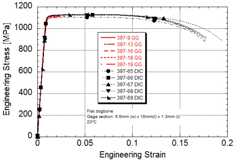
Ti 6-2-4-2S Engineering Stress-strain Post-yield strain rate of 11/s Machine rate of 120 mm/s Strain gaged and DIC specimens 23°C
