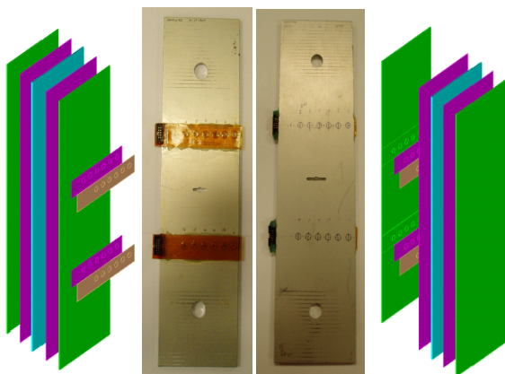
Hybrid material with internal (Right) and externally (left) affixed PZT SMART layer networks.
