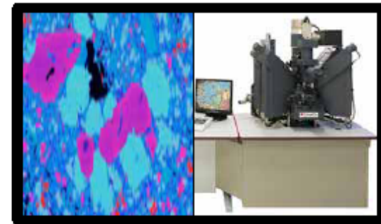
Electron Microprobe Analyzer and Wave Dispersive Spectroscopy (WDS) to study compositional variations across interfaces
