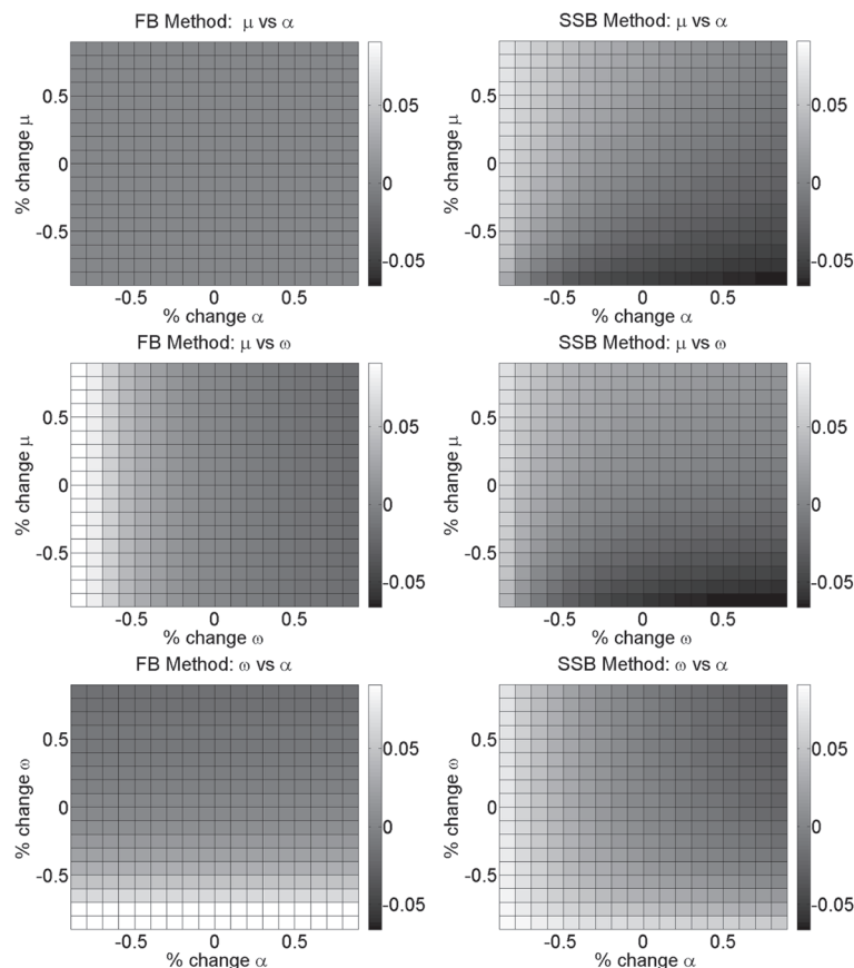
Figure 7 Error propagation. The average difference of the Forward Backward and Stomakhin-Short-Bertozzi score functions with the parameters varied by \pm 90\% of the target values, \mu_k = 0.01 , \omega_k = 0.1 , and \alpha_k = 0.5 .
