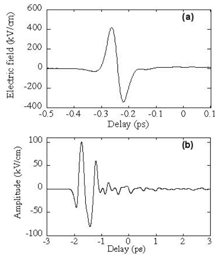
Fig. 3: Time domain traces of (a) a 2-colour excited air plasma and (b) a 450 \mu\text{m} thick OH-1 crystal excited at 9 \text{mJ}/\text{cm}^2 . (a) was obtained by air biased coherent detection and (b) by electro-optic sampling in a 40 \mu\text{m} thick ZnTe crystal. Fundamental excitation wavelength is 1300 nm in both cases. Detection wavelength is 800 nm.
