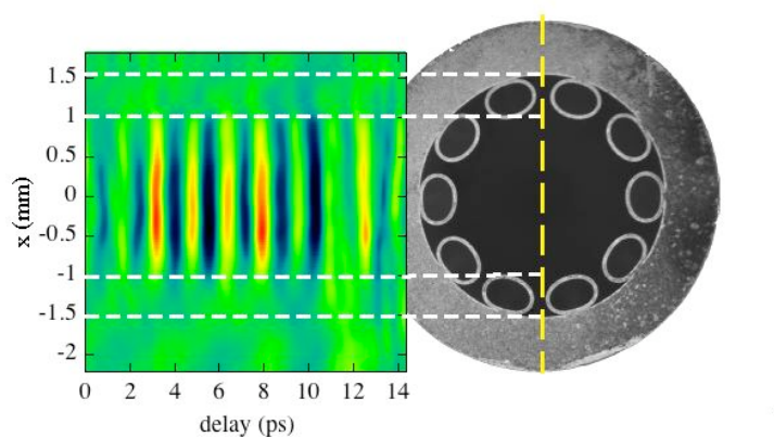
Fig. 1: Space time THz waveguide image of pulse propagation in the MOF with optical micrograph cross section shown. It is clear that radiation is largely confined to the region inside the ring of thin wall silica tubes.
