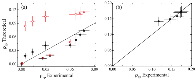
FIG. 2 (color online). Panel (a): experimentally determined excitation fraction in Ba^+ versus theoretical predictions of the quantum Liouville (●) and rate equation (○) treatment. Panel (b): experimentally determined excitation fraction in Ca versus predictions of a 4-level rate equation model. In both panels the solid line has a unit slope, representing ideal agreement.
