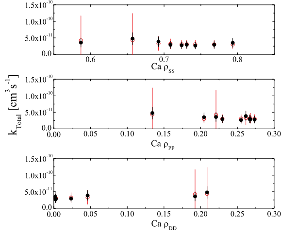
FIG. 4 (color online). Measured rate constant as a function of Ca population fractions. Experimental result in black. Best fit (\{k_{ps}, k_{sd}, k_{pd}, k_{dd}\} = \{4.2 \pm 1.9, \leq 3, \leq 20, \leq 7\} \times 10^{-10} \text{ cm}^3 \text{ s}^{-1}) to the four entrance channel model shown as open red circles (○). For these measurements, the \text{Ba}^+ population fractions were fixed at \rho_{ss}^{\text{Ba}} \sim 0.4 , \rho_{pp}^{\text{Ba}} \sim 0.1 , \rho_{dd}^{\text{Ba}} \sim 0.5 .
