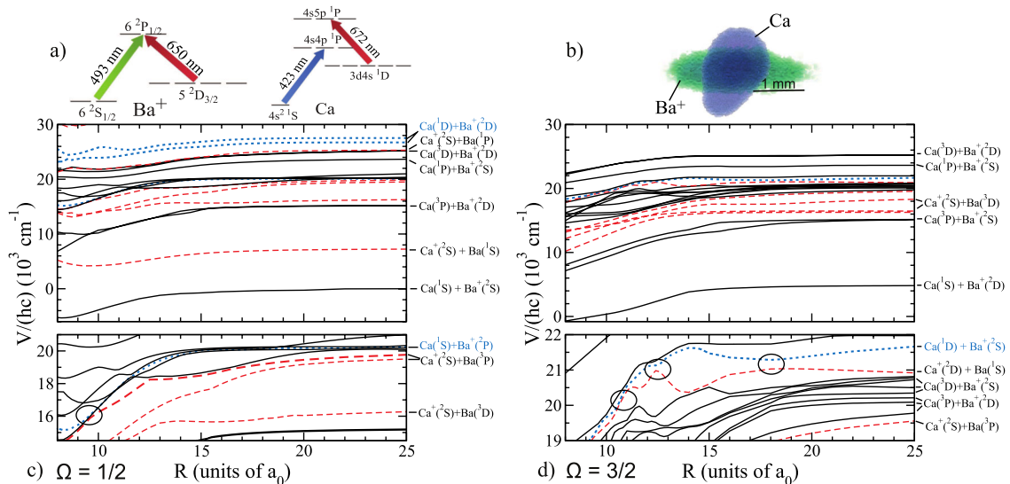
FIG. 1 (color online). (a) \text{Ba}^+ and Ca relevant energies levels and laser cooling schemes. (b) Fluorescence images of Ca MOT and \text{Ba}^+ ion cloud. (c) and (d) Molecular potentials of the \Omega = \frac{1}{2}, \frac{3}{2} excited states of the \text{CaBa}^+ molecule, respectively, as a function of interatomic separation R . The bottom panels show higher detail for potentials near 20 \times 10^3 \text{ cm}^{-1} above the \text{Ca}^+(^2S) + \text{Ba}(^1D) dissociation limit. Entrance and exit channels, as defined in the text, dissociate to blue (dotted) and red (dashed) potentials, respectively.
