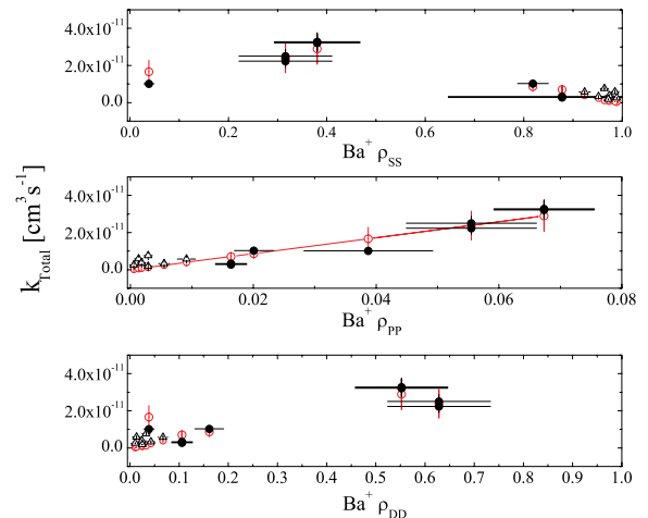
FIG. 3 (color online). Measured rate constant as a function of Ba^+ population fractions. Experimental result in black. Best fit ( \{k_{ps}, k_{sd}, k_{pd}, k_{dd}\} = \{4.2 \pm 1.9, \leq 3, \leq 20, \leq 7\} \times 10^{-10} \text{ cm}^3 \text{ s}^{-1} ) to the four entrance channel model shown as open red circles (○). For these measurements, Ca population fractions were fixed at \rho_{ss}^{Ca} \sim 0.75 , \rho_{pp}^{Ca} \sim 0.20 , \rho_{dd}^{Ca} \sim 0.05 .
