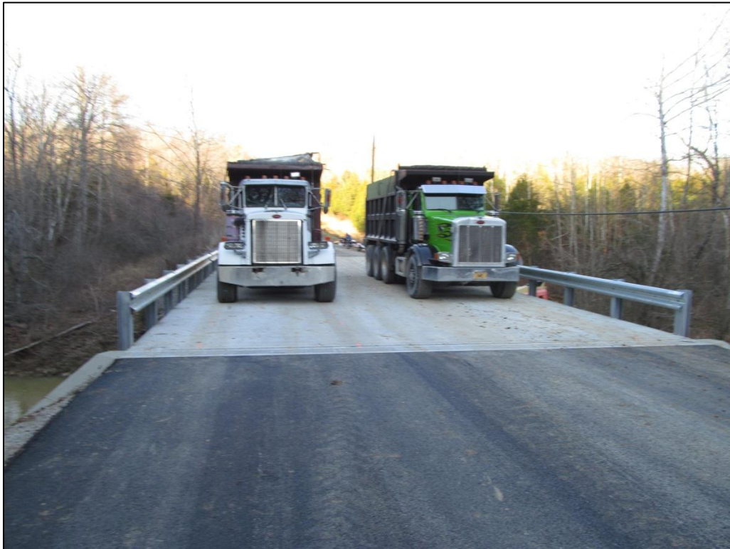
Figure 1.7 – Round 1 Tests - Two lane truck test: Truck 1 @ Y3 & Truck 2 @ Y1.
