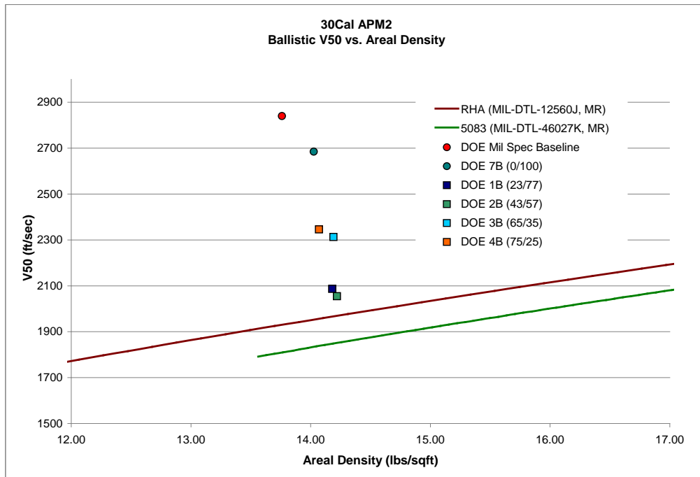
Fig. 60 Ballistic results
