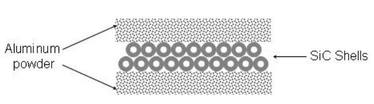
Fig. 16 Schematic detailing the starting arrangement for the powder-based approach to producing a syntactic foam
