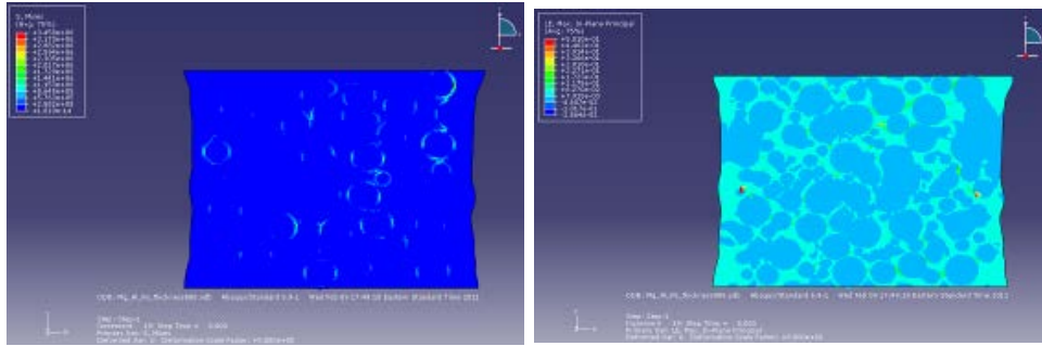
(a) von Mises stress pattern (wall thickness 0.18 mm) (b) logarithmic strain distribution
