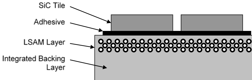
Fig. 58 LSAM test panel construction
