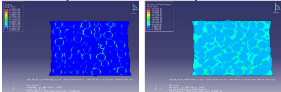
(c) von Mises stress pattern (wall thickness 0.24 mm) (d) logarithmic strain distribution
