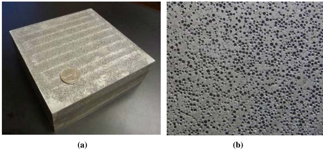
Fig. 27 a) Al/SiC hollow sphere syntactic block of size 6 × 6 × 2 inches, and b) close-up of syntactic surface
