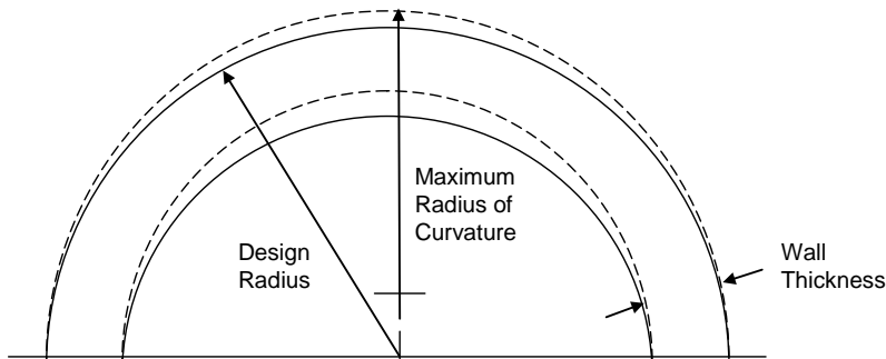
Fig. 6 Representation of hollow sphere parameters
