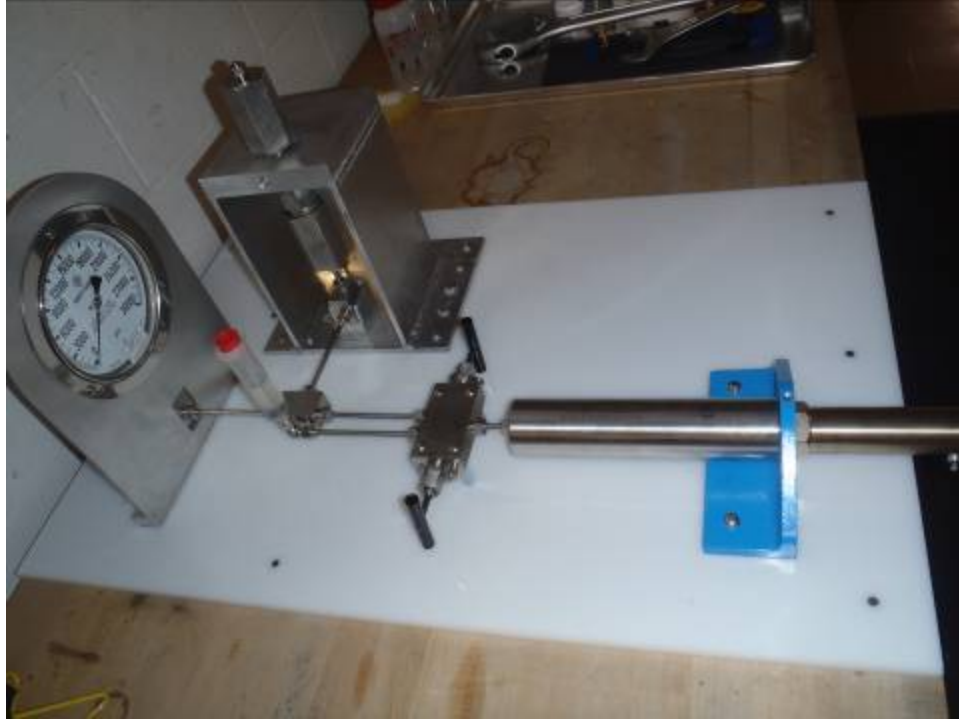
Fig. 13 Hydrostatic compression tester
