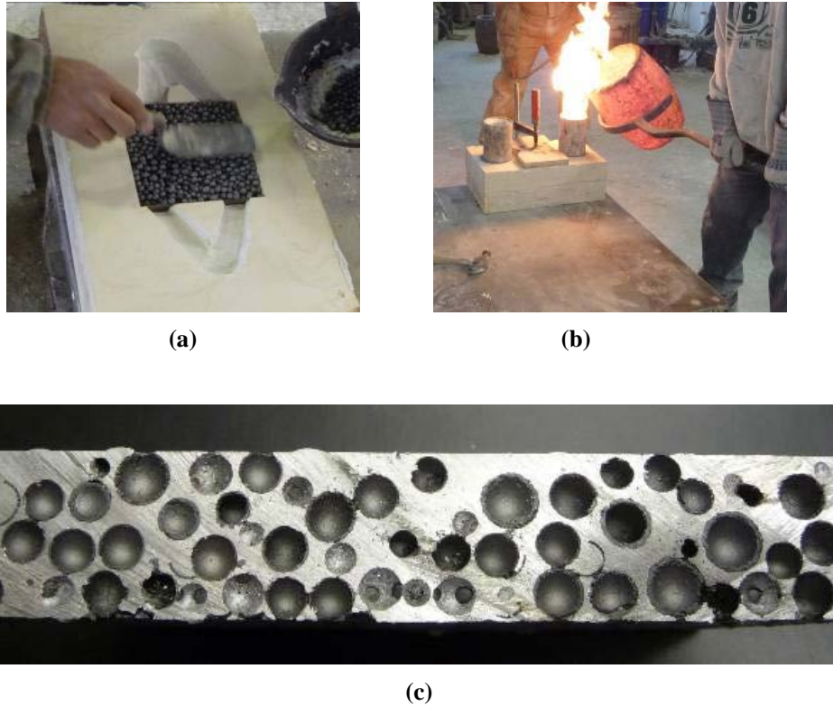
Fig. 25 Early casting of M350 hollow spheres in an aluminum alloy 319: a) 19-mm cavity fill, b) casting pour, and c) cross section of 10-mm SiC syntactic foam
