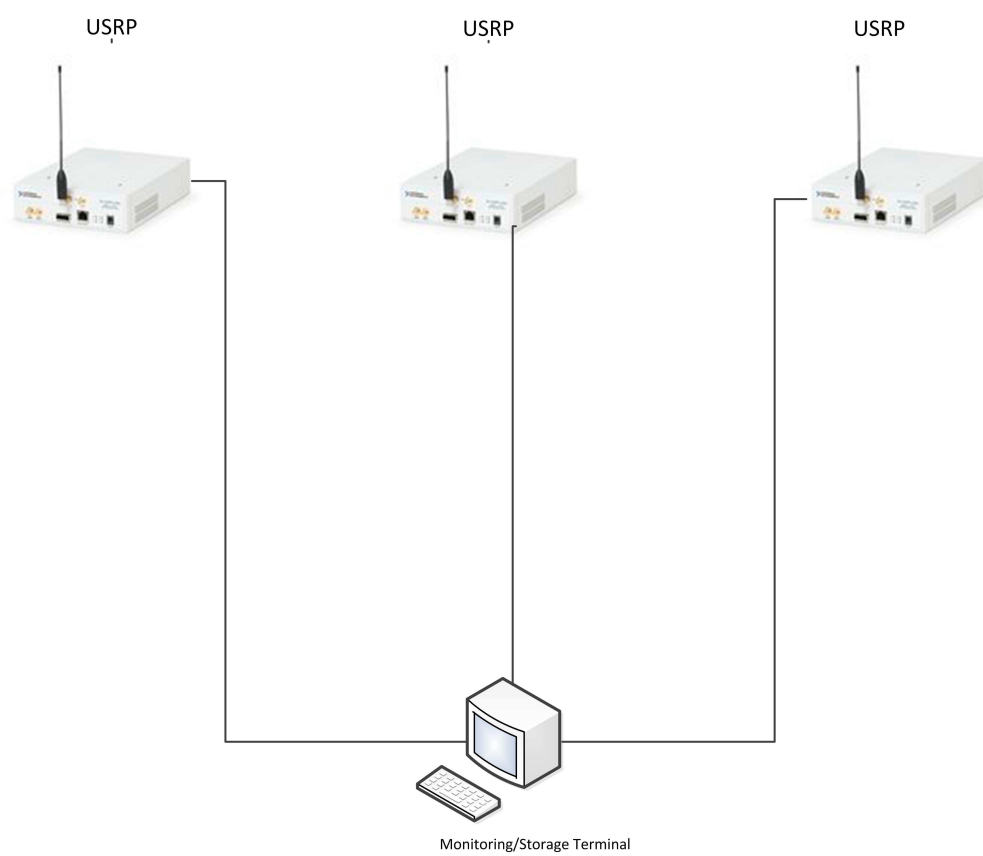
Figure 6.1 Distributed RF trace collection testbed.
