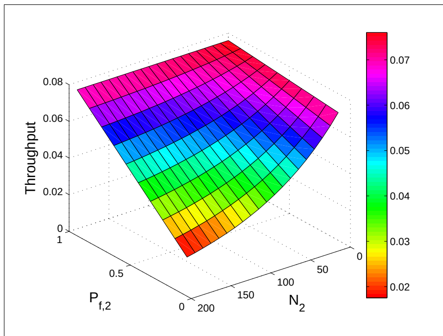
Figure 5.7 Effects of the network density and probability of false alarm of CRN_2 on the performance of CRN_1 .
