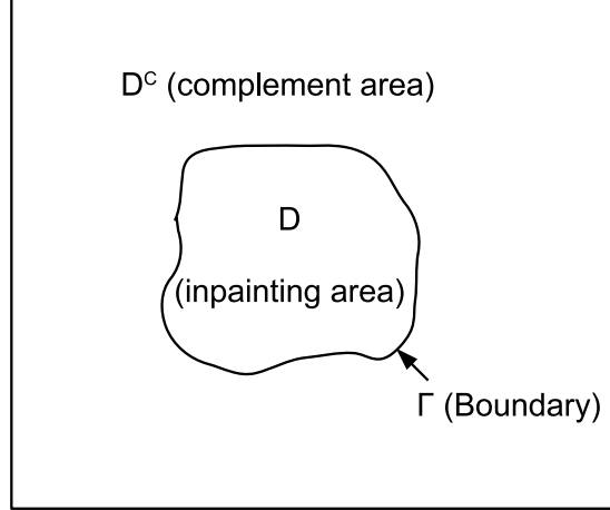
Figure 1.5 The TV inpainting model finds the best guess for u|_D based on the TV norm on the extended area D^C \cup D and the noise constraint on D^C .
