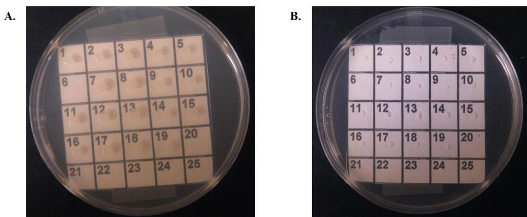
Figure 19. Spot plating white pigmented colonies on both LB medium and selective medium to confirm absence of the selection marker. A. LB agar medium. B. LB agar supplemented with 50 \mu\text{g/ml} apramycin. White pigmented colonies from the replicated plates were spotted onto both plates depicted above. Absence of growth on the corresponding apramycin plate indicated absence of the resistant selection marker.
