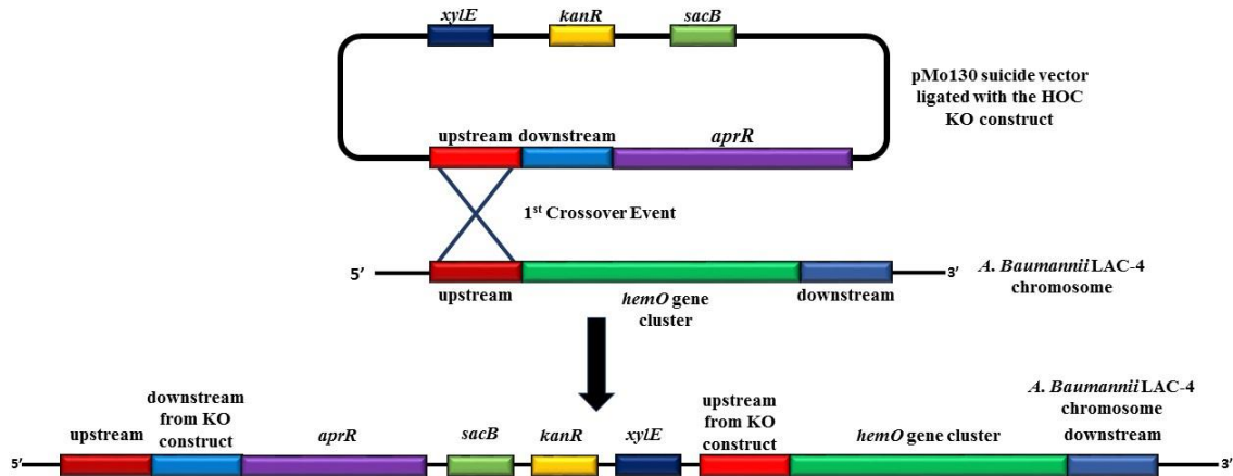
Figure 5. Co-integration of the plasmid via a Single-Crossover Event. A single-crossover event occurs between the homologous recombination of either the upstream flanking regions or the downstream flanking regions. Upstream recombination is shown above illustrating how the plasmid inserts itself behind the chromosomal upstream flanking region, linking the constructs upstream flanking region to the hemO gene cluster in its place.
