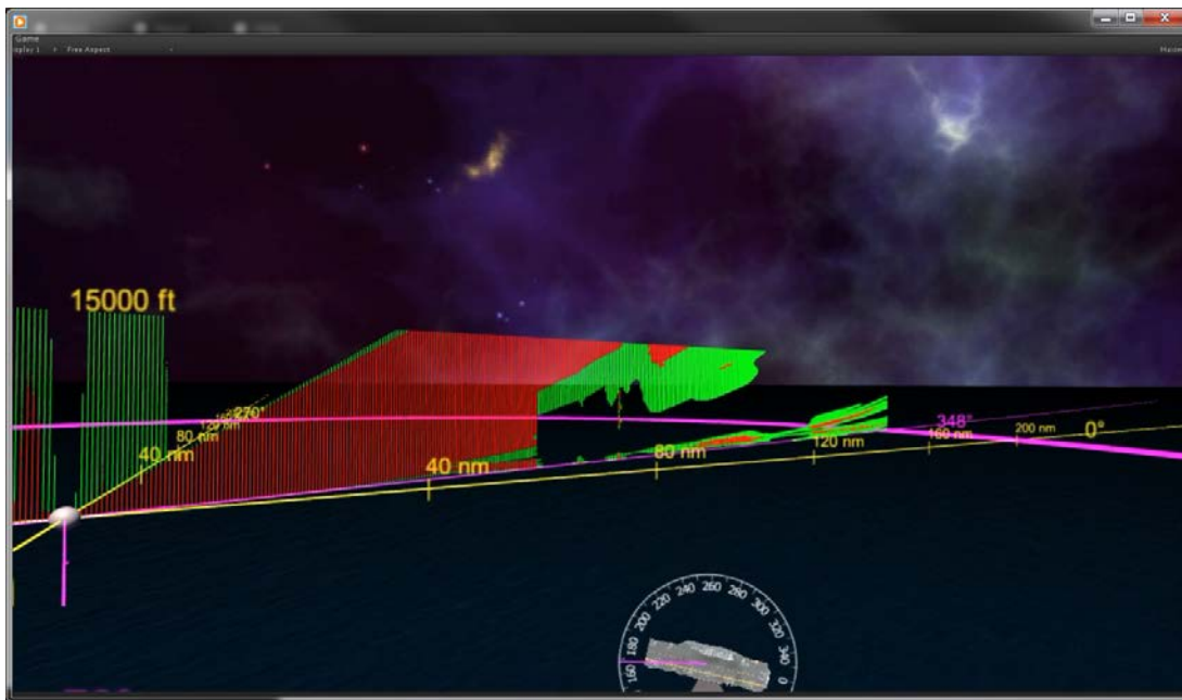
Figure 19. From the same dataset as in Figure 18, but at bearing 348°, a large radar coverage gap is apparent, potentially representing an increased vulnerability to the ship.
