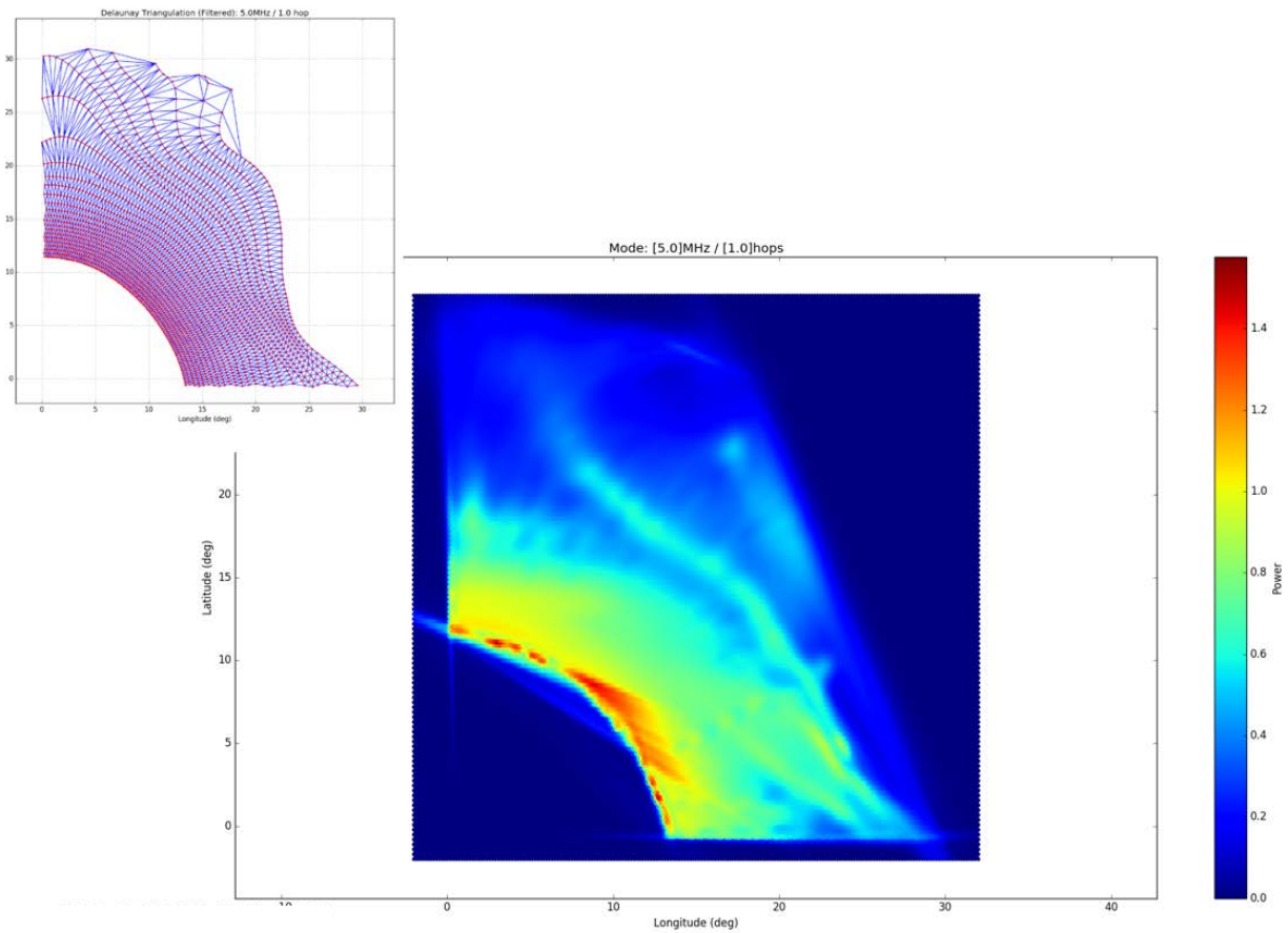
Figure 6. An example of IonRayTrace's results for an illumination application. Delaunay triangulation (inset) used for sorting ray points by mode type and phase path difference, for use in computing covariance eigenvectors for Gaussian ray bundle-based estimation of incident intensity.
