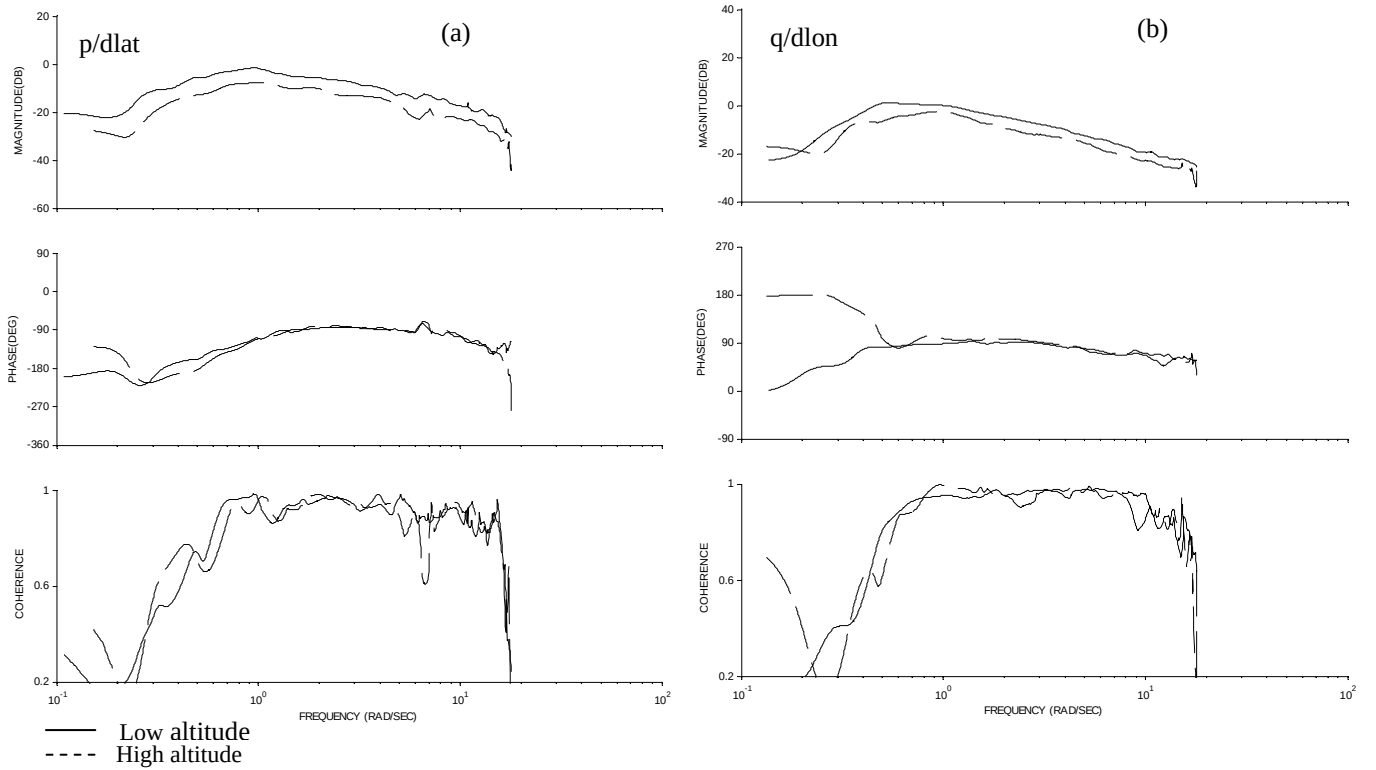
Figure 6 – Effect of altitude at hover, (a) roll rate response to lateral cyclic, (b) pitch rate response to longitudinal cyclic
