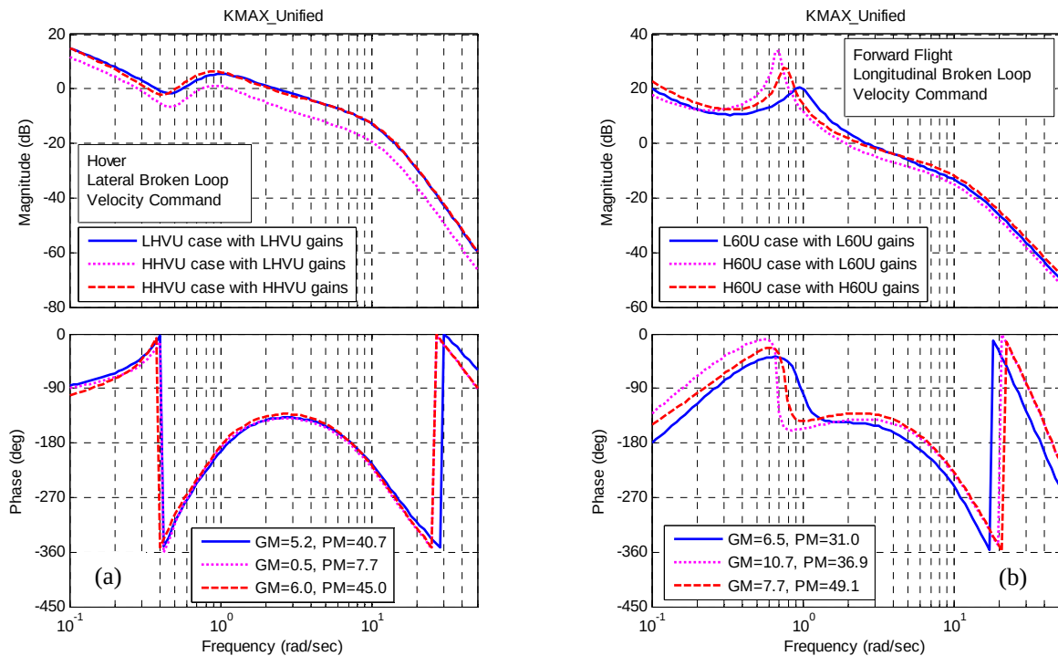
Figure 11 – Broken-loop frequency responses highlighting effect of altitude and need for gain scheduling: a) lateral hover, b) longitudinal forward flight
