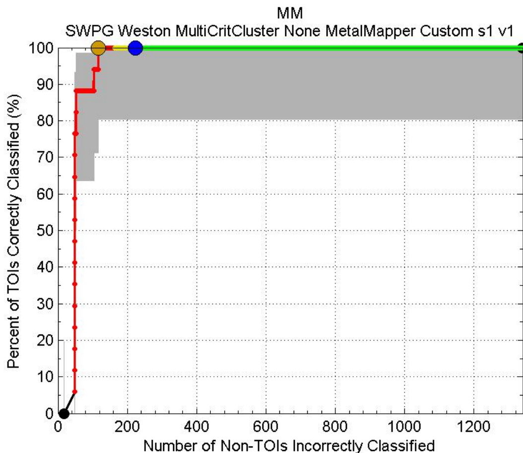
Figure 7-1. SWPG Final ROC Curve
