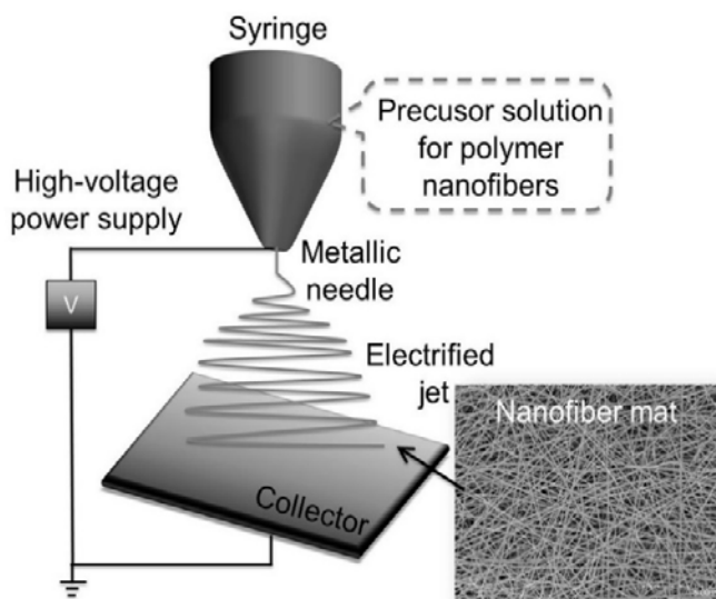
Figure 1. Schematic of an electrospinning apparatus, including high-voltage power supply, spinneret (metallic needle), collector (aluminum foil or metallic drum) and syringe pump.
