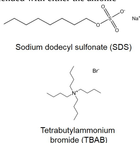
Figure 5. Chemical structure of SDS and TBAB surfactants.
