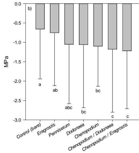
Figure 58. Soil water potential in A) open versus shade treatments and B) species treatments.
