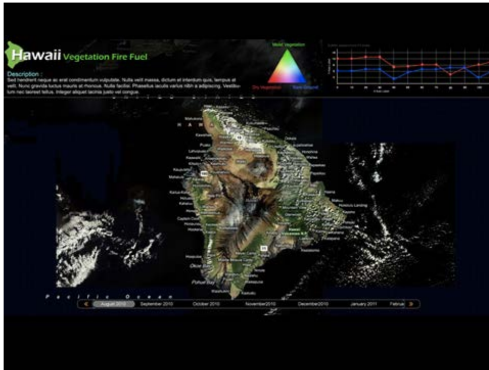
Figure 64. Each figure pane represents the Island of Hawaii across inter- and intra-annual timescales. Note the variation in PV and NPV.
