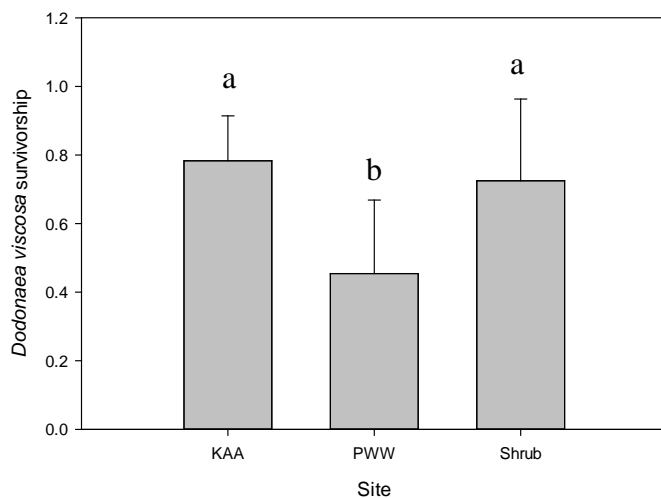
Figure 32. Survivorship of Dodonaea viscosa outplants (second outplanting) across sites. Error bars show 1SD. Letters indicate statistically different means, P < 0.05
