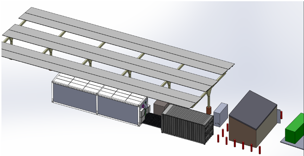
Figure 5-12: 3D CAD image of the ESS location.
