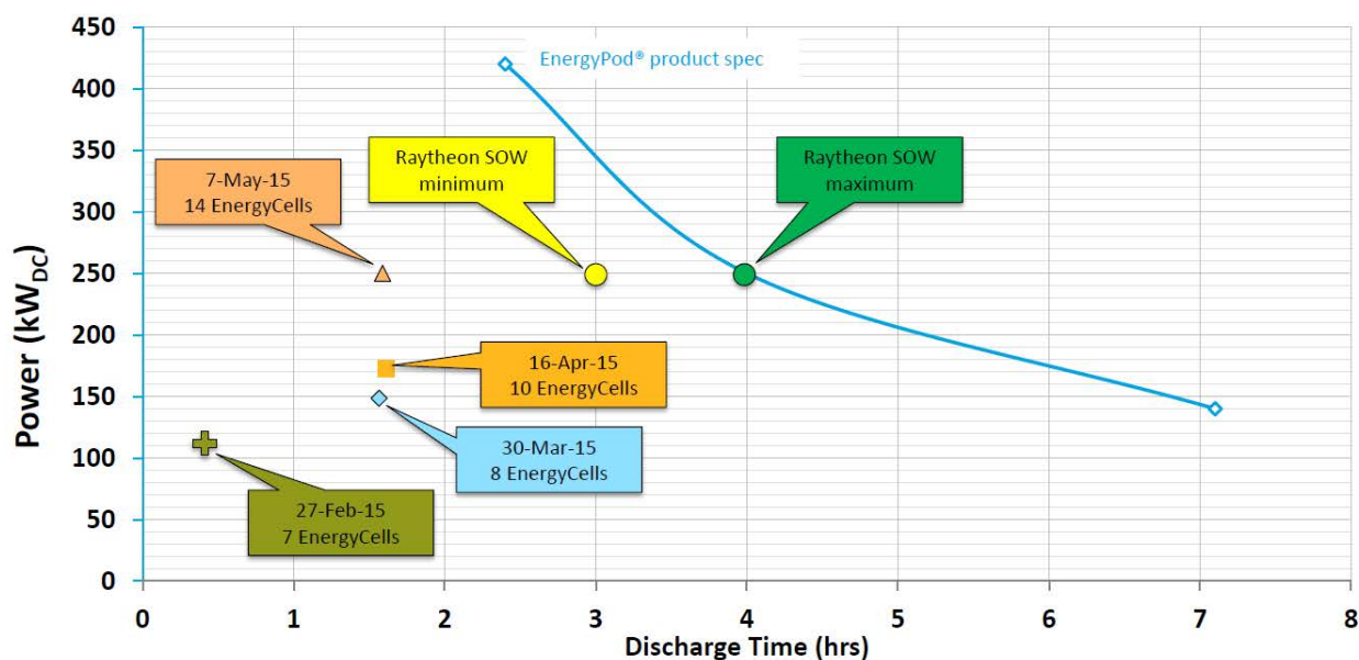
Figure 2-16: Energy capacity timeline and scale up from Primus Power since the November 2013 briefing.
