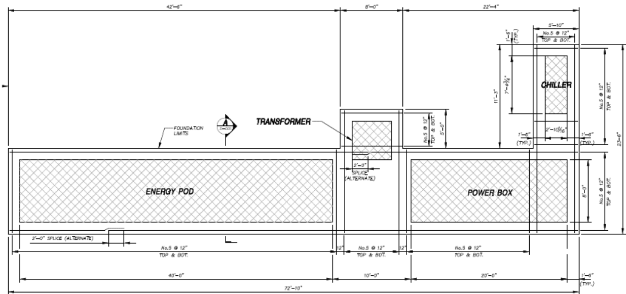
Figure 5-11: Construction drawing schematic of ESS location.
