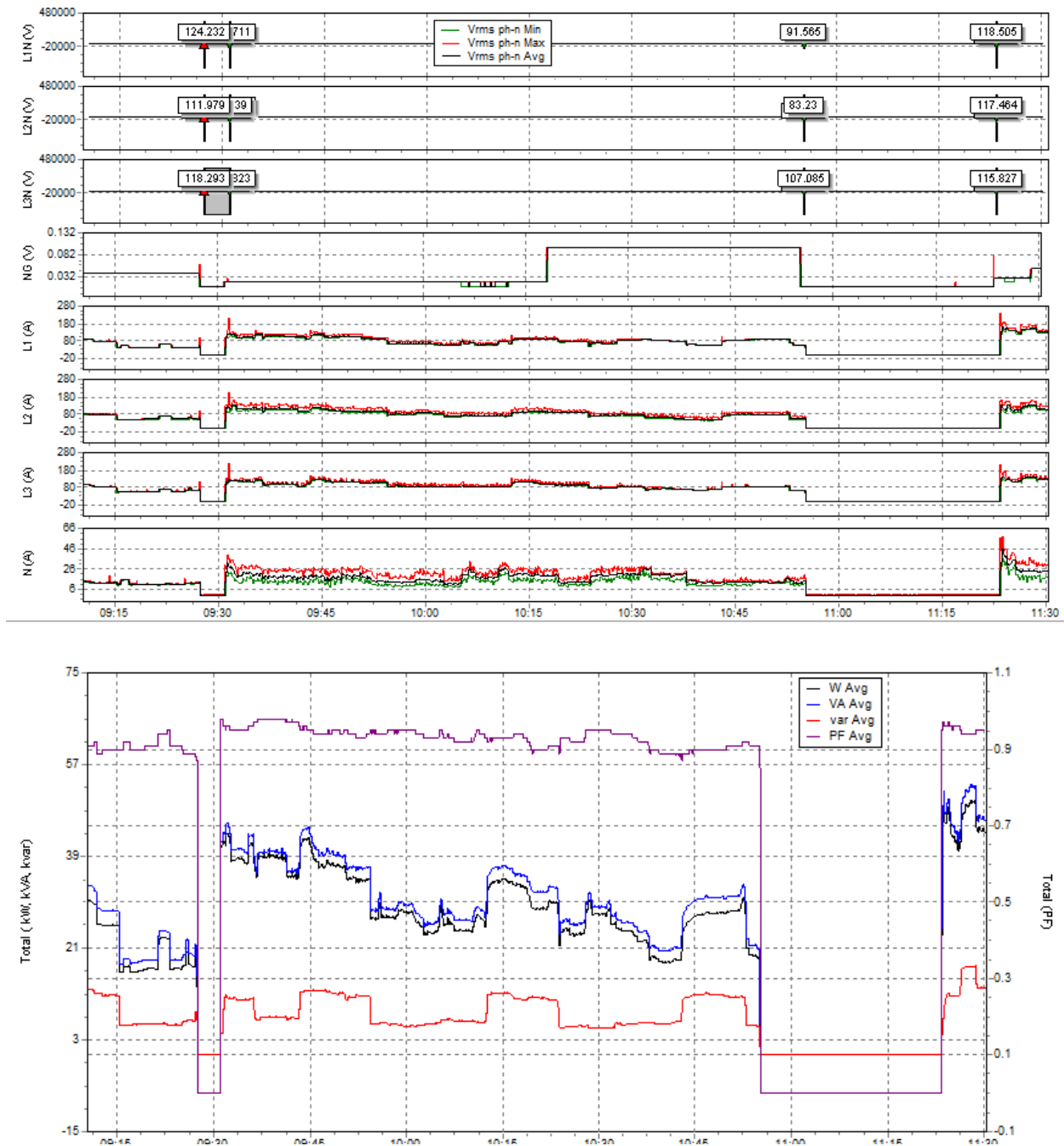
Figure 5-29: Detailed load data taken from Fluke 437II that was attached to Building 6311 circuit during 12/12/15 morning islanding test.
