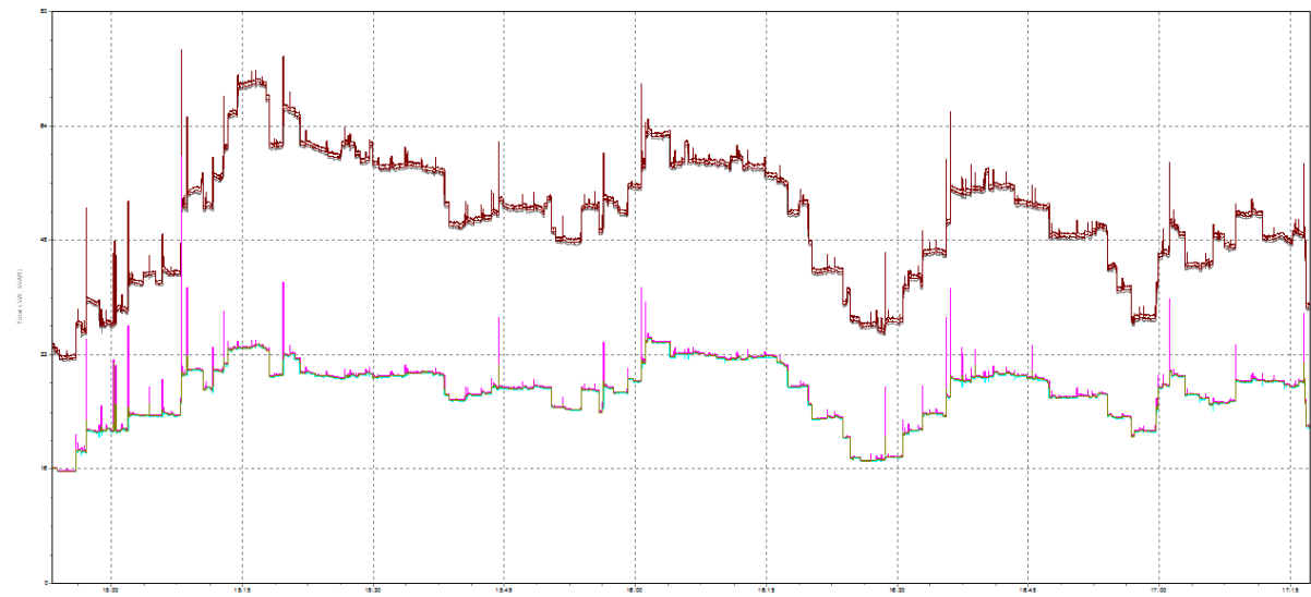
Figure 5-23: Plot of total real power (kW) and reactive power (kVAR) over time. Power factor ranged from about 0.86 to 0.89. Peak 6311 load on Sunday was about 70 kW at 1515.
