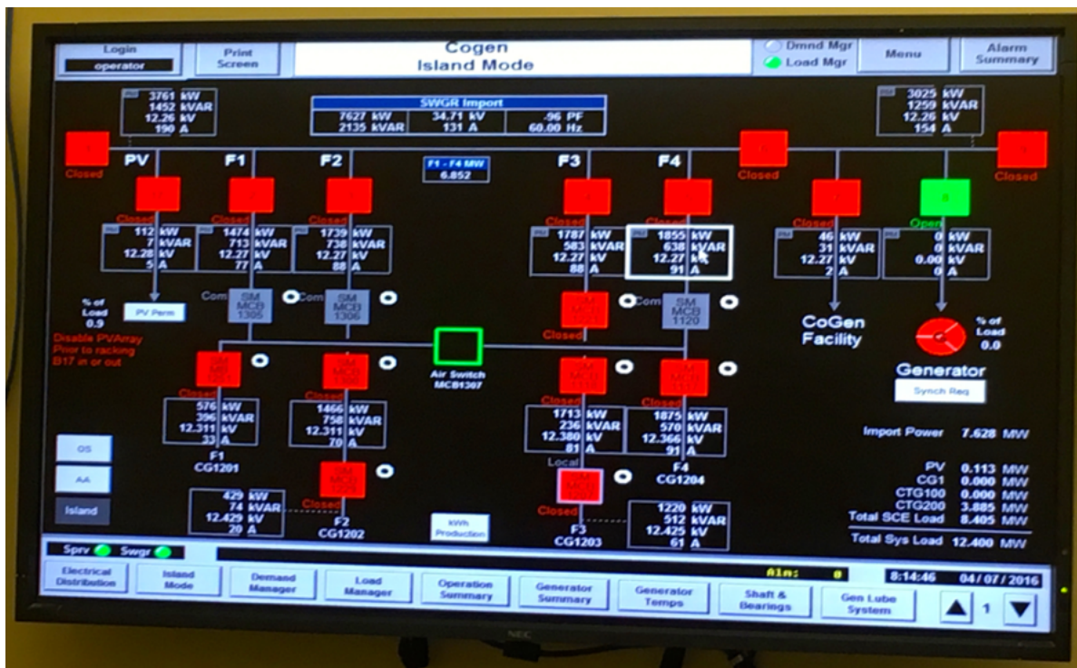
CoGen Plant #2 HMI
