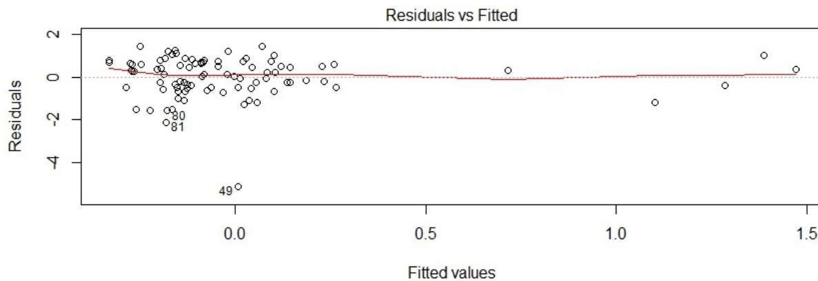
Figure 36 Fitted Values vs. 208V Model Residuals
