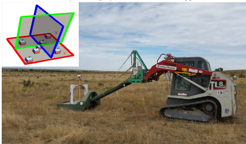
Figure 2.2 Antenna Array and Deployment of the MetalMapper at PCD
