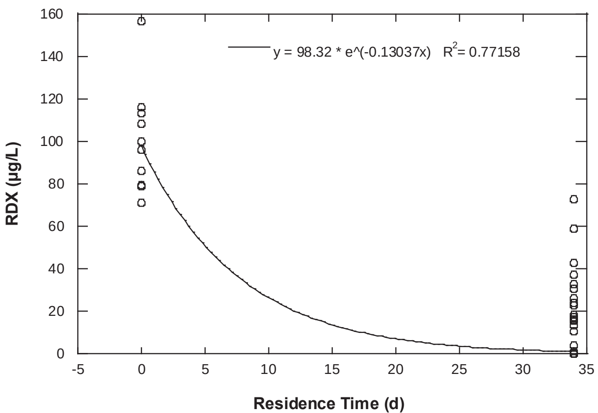
Figure 6.22. RDX degradation rate using data from upgradient well MW-10 versus all three in-barrier monitoring wells.
