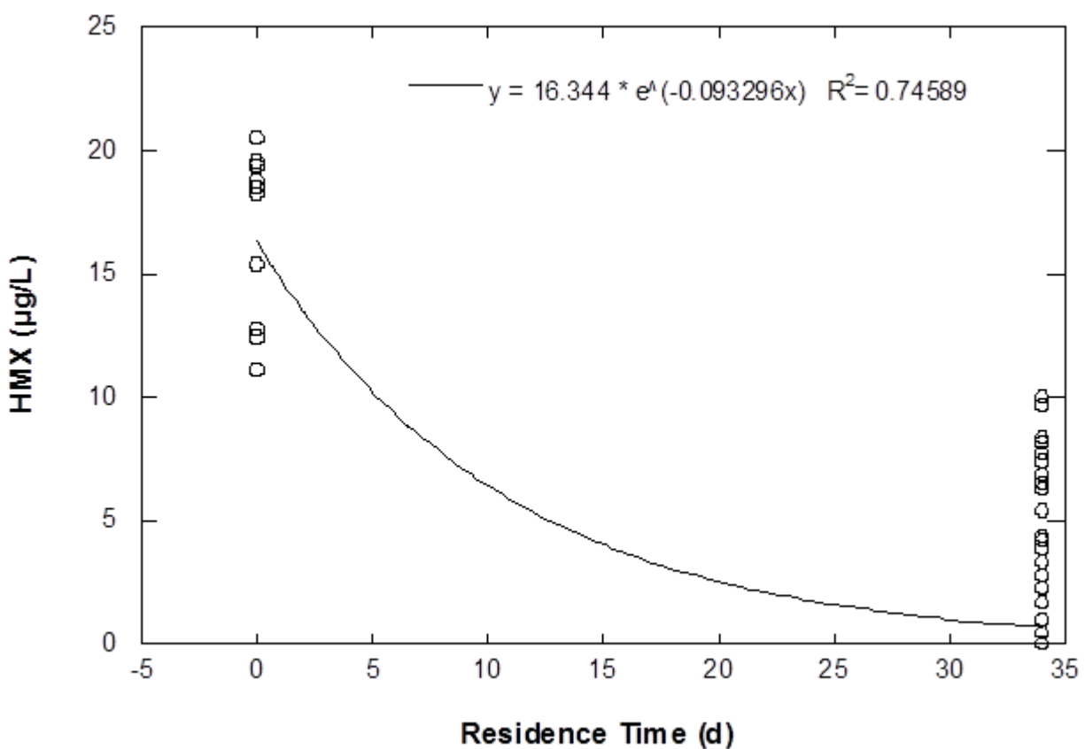
Figure 6.27. HMX degradation rate using data from upgradient well MW-10 versus all three in-barrier monitoring wells.
