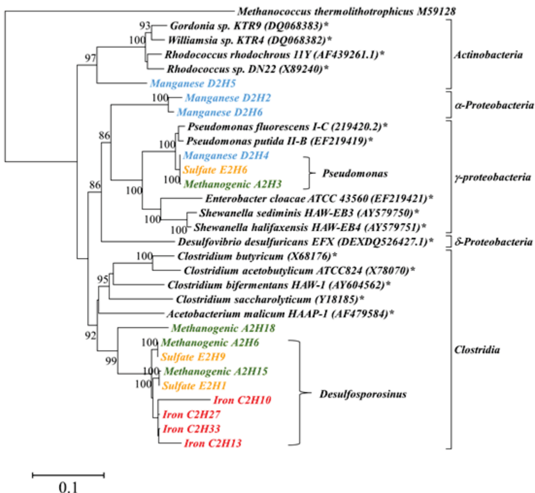
Figure 6.37. Phylogenetic tree representing 16S rRNA gene sequences derived from ^{13}\text{C} -DNA fractions of microcosms receiving ^{13}\text{C} -labeled RDX under different electron acceptor conditions.
