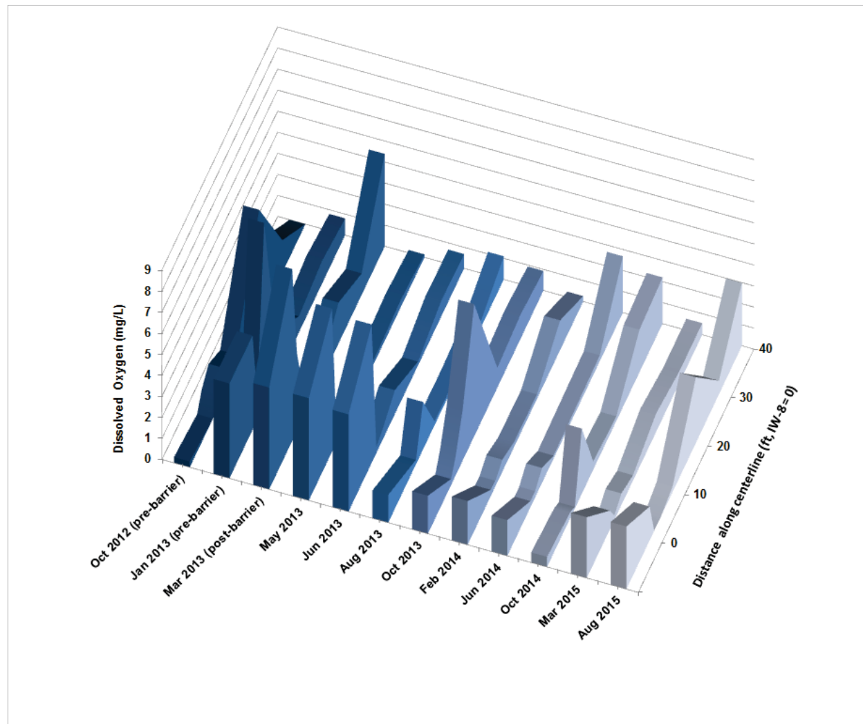
Figure 6.4. Dissolved oxygen concentrations along the demonstration plot centerline. Emulsified oil was re-injected after the October 2015 sampling event.
