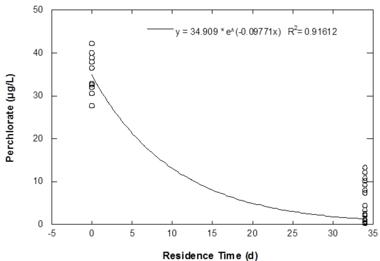
Figure 6.32. Perchlorate degradation rate using data from upgradient well MW-10 versus all three in-barrier monitoring wells.
