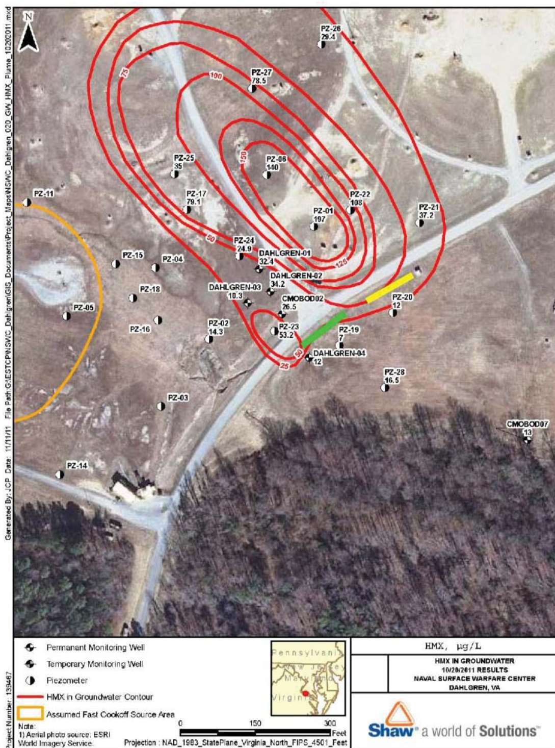
Figure 5.29. Plume map for HMX in the southeast area of the Churchill Range.
