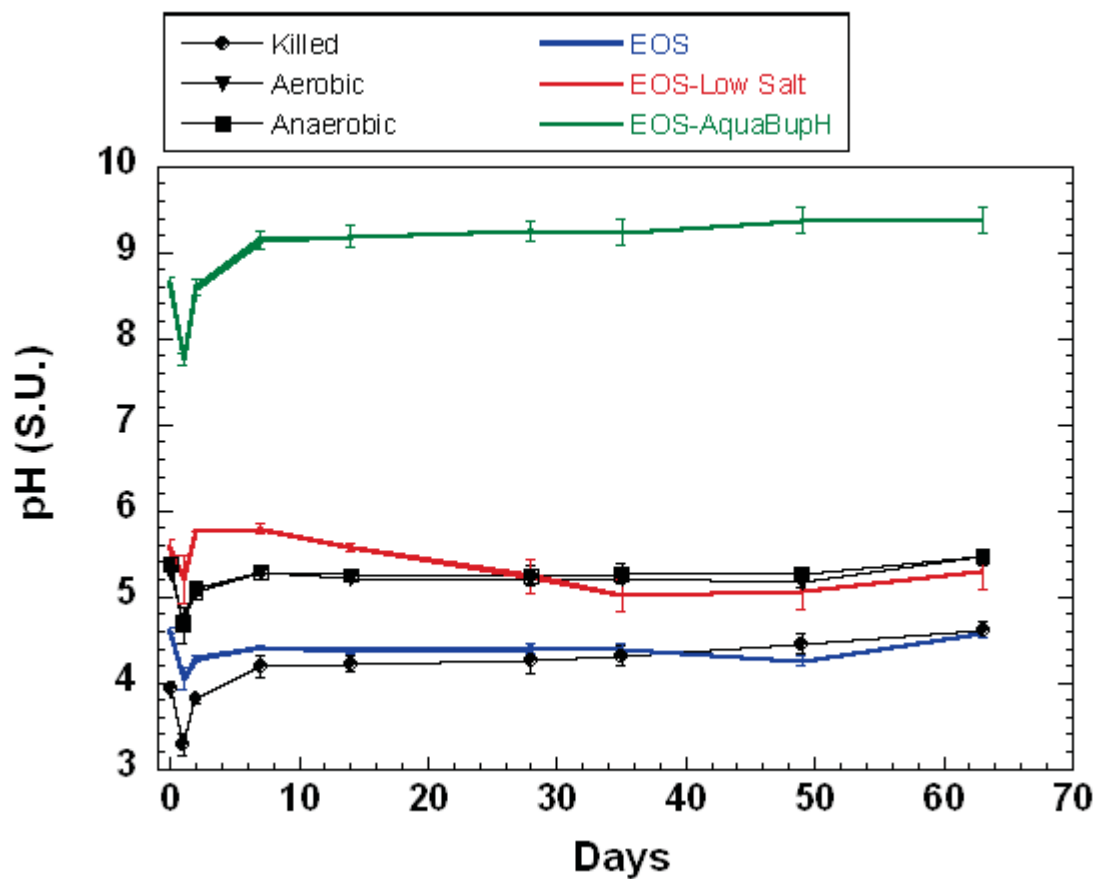
Figure 5.4. Measured pH in the site-derived microcosms over time. (Average and standard deviation of triplicate microcosms of each treatment).
