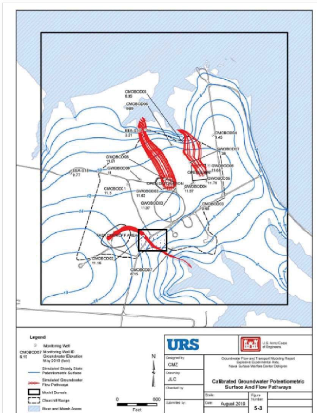
Figure 4.8. Potentiometric surfaces and modeled groundwater flow pathways from the Open Burn, Open Detonation, and Fast Cookoff areas on the Churchill Range Figure from URS, 2010. The primary demonstration site is indicated by a bold black square.
