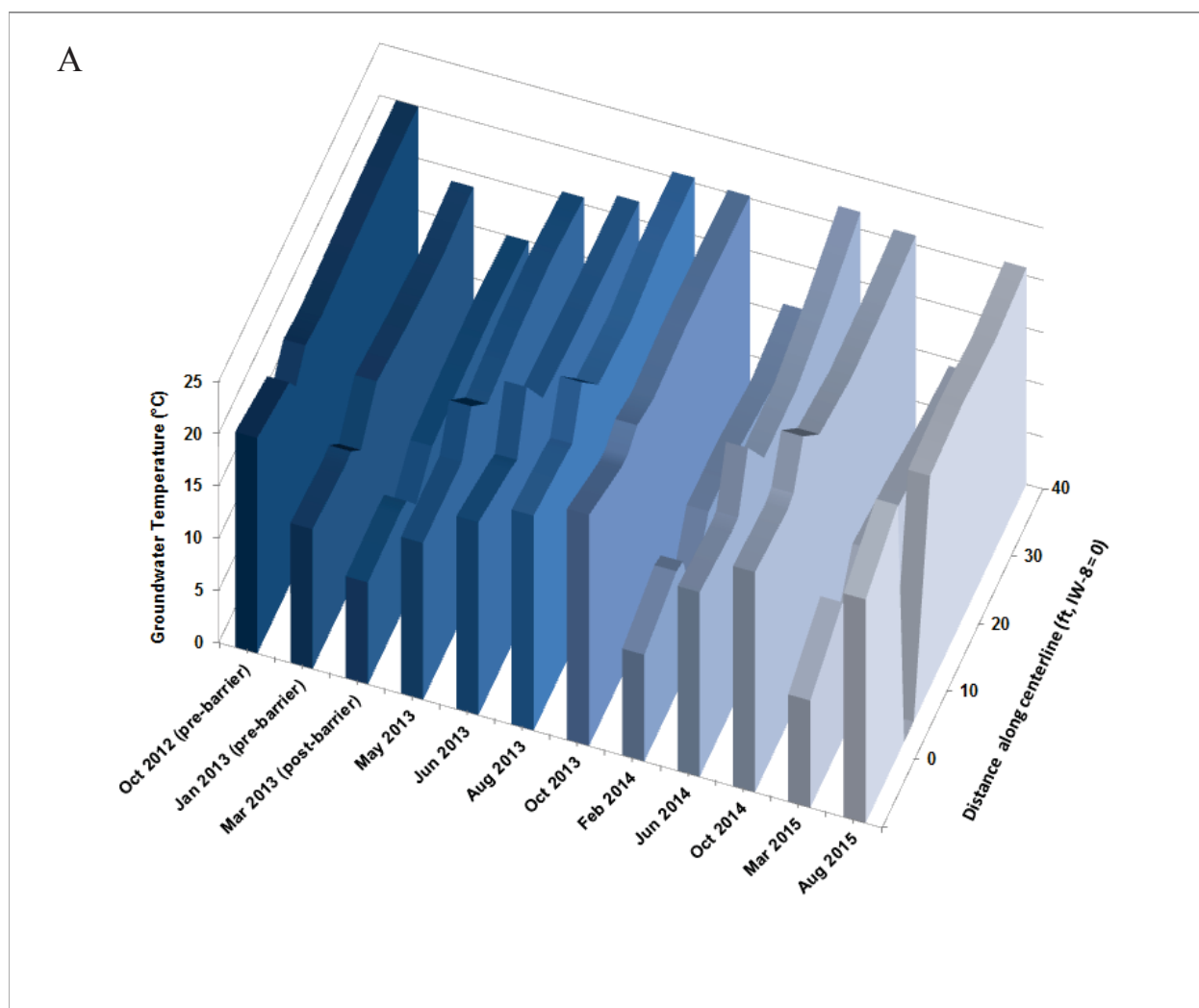
Figure 6.3. Groundwater temperatures during the demonstration period.
