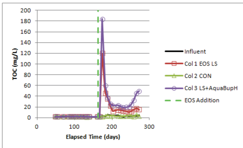
Figure 5.11. TOC in the influent groundwater and the effluent of the three flow-through columns.
