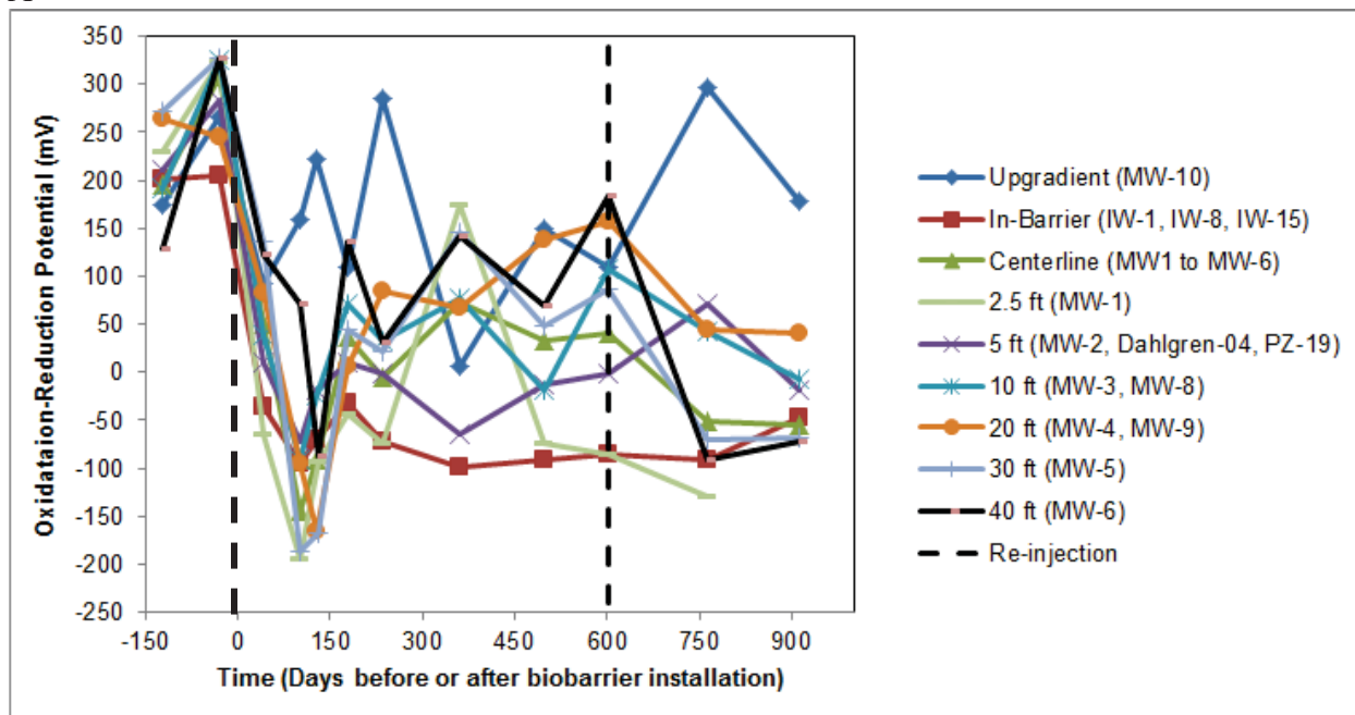
Figure 6.7. Oxidation-reduction potential over time in the demonstration plot. All wells are represented as a function of distance from the biobarrier in panel A and the upgradient, in-barrier, and centerline downgradient wells are represented in panel B.
