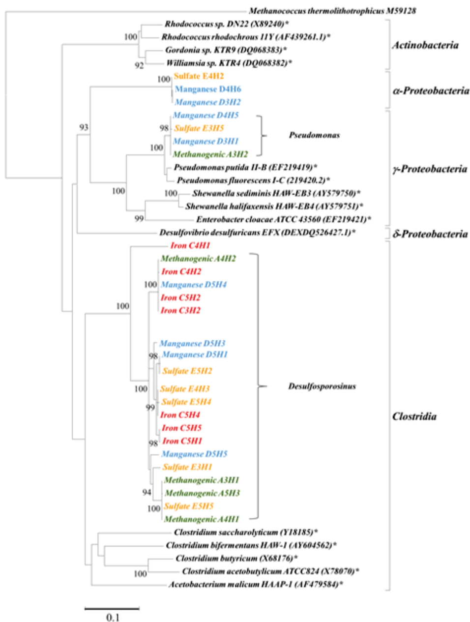
Figure 6.38. Phylogenetic tree representing 16S rRNA gene sequences derived from ^{15}\text{N} -DNA fractions of microcosms receiving ^{15}\text{N} -labeled RDX (ring- or nitro- ^{15}\text{N}_3 -RDX, and fully-labeled ^{15}\text{N}_6 -RDX) under different electron acceptor conditions.
