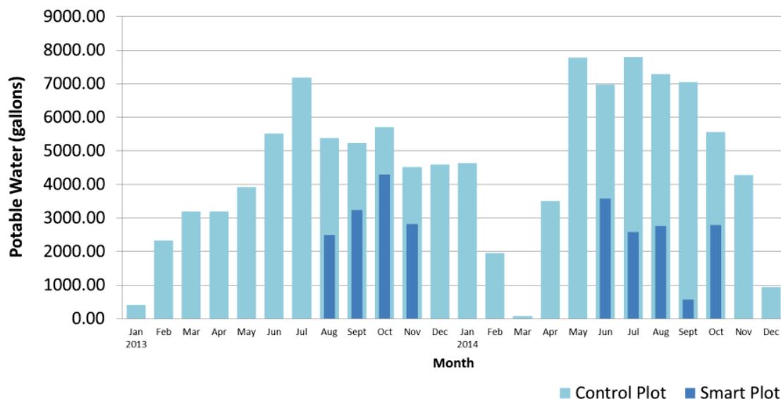
Figure 14. Potable Water Savings by ET and Moisture Sensor
