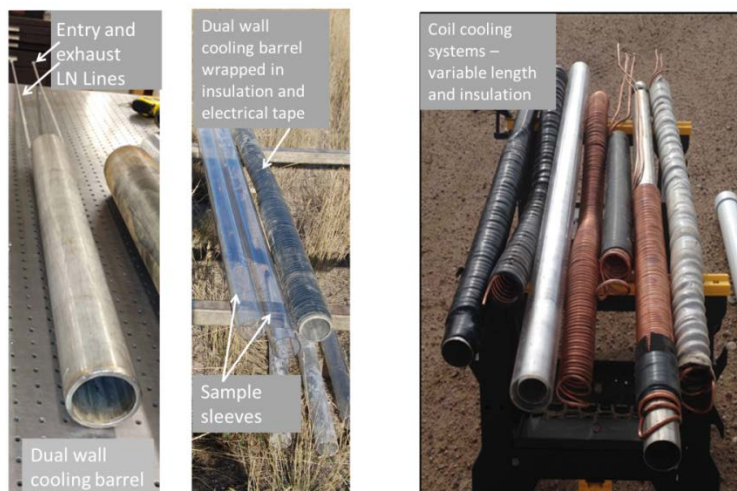
Figure 3-9. Dual-wall cooling cylinder, insulated cooling cylinder, and coil cooling system
