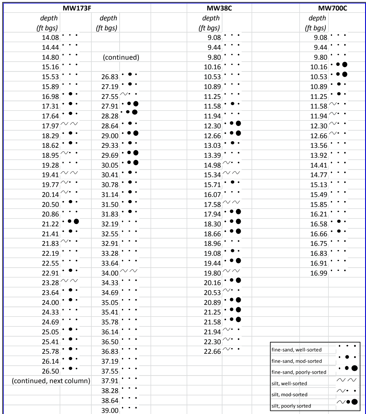
Figure 4-19. Geologic log summary
