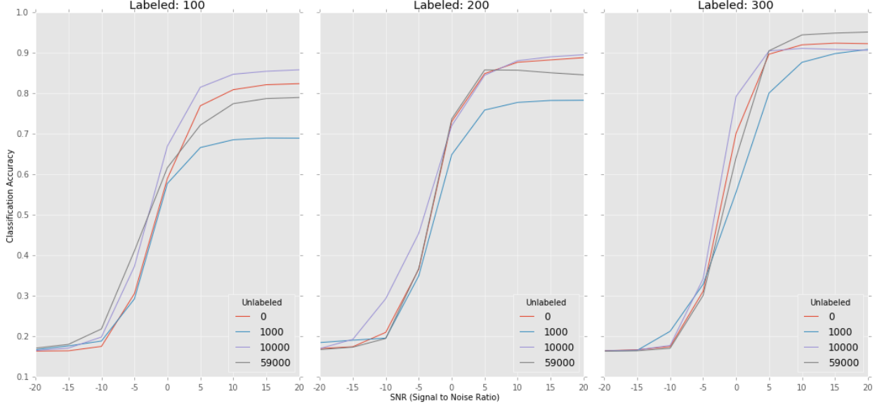
Figure 3. Example results of incorporating variable ratios of labeled and unlabeled examples into the semi-supervised training of a CAE
