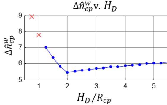
Figure 16: \Delta\hat{n}_{cp}^w v. H_D . \Delta\hat{n}_{cp}^w decreases with H_D for H_D < 2R_{cp} and increases with H_D for H_D > 2R_{cp} . (The points with the red x's represent cases in which Q_{cp} does not encompass the area needed for all the rays paths originating within 60^\circ of the axis of symmetry.)
