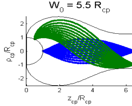
Figure 6b: Ray Bundles through Reimager with W_0 = 5.5R_{cp}
