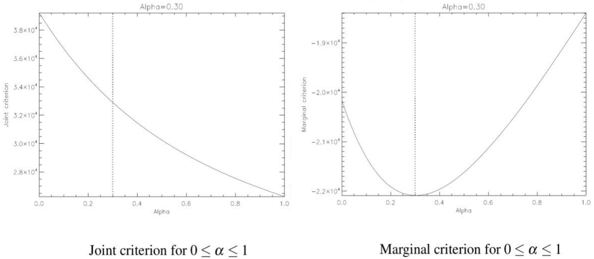
Fig. 3. Plot for the joint (left) and the marginal (right) estimator when the PSF is a linear combination of two modes related with one single coefficient of value \alpha=0.3 , i.e., \mathbf{h} = \alpha \cdot \mathbf{h}_{foc} + (1 - \alpha) \cdot \mathbf{h}_{defoc} . The reader can notice that the marginal criterion has its minimum at the correct value of \alpha , whereas the joint criterion has its minimum for that \alpha that pushes the PSF to be the focused one, i.e., the sharpest one.
