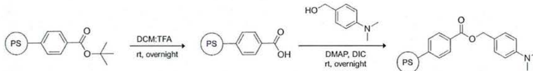
Scheme 5. Synthetic approach to DMA-functionalized particles.
