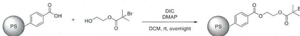
Scheme 6. Synthetic approach to initiator-functionalized particles.
