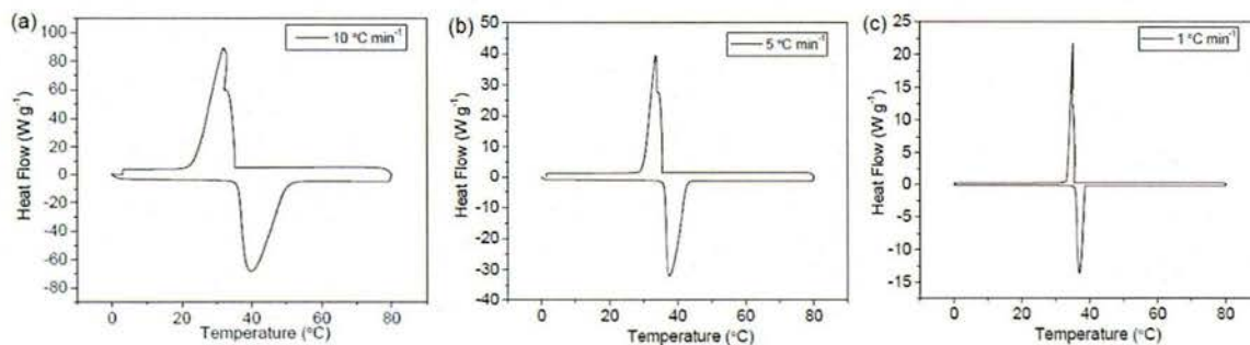
Figure 9. DSC curves of C_{20}H_{42} capsules of about 200 \mu\text{m} in different heating-cooling rates: (a) 10\text{ }^{\circ}\text{C min}^{-1} ; (b) 5\text{ }^{\circ}\text{C min}^{-1} ; (c) 1\text{ }^{\circ}\text{C min}^{-1} .
