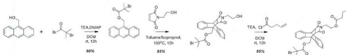
Scheme 8. Synthesis of double-bond functionalized anthracene-maleimide based mechanophore initiator.
