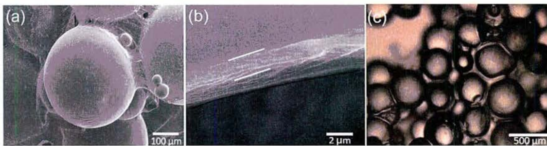
Figure 23. (a), (b) SEM images and (c) optical image of the sodium acetate solution-infilled microcapsules.
