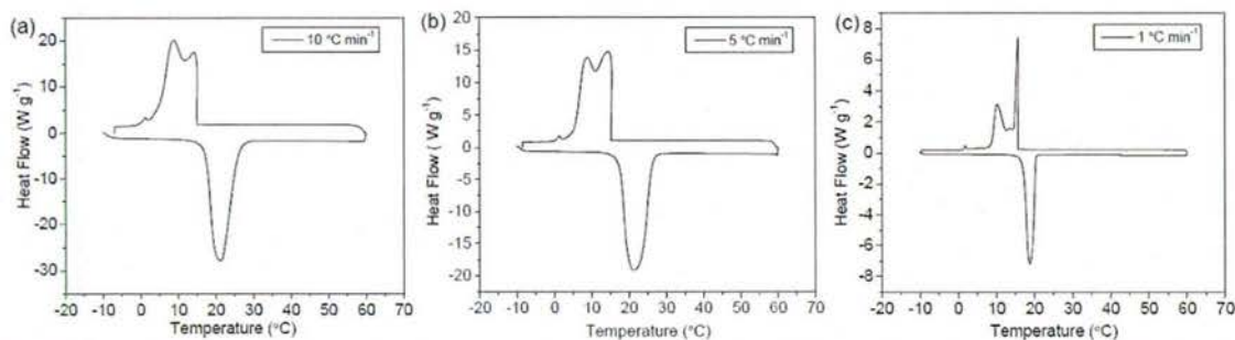
Figure 4. DSC curves of C_{16}H_{34} capsules ( \sim 20 \mu m ) in different heating-cooling rates: (a) 10 \text{ }^\circ\text{C min}^{-1} ; (b) 5 \text{ }^\circ\text{C min}^{-1} ; (c) 1 \text{ }^\circ\text{C min}^{-1} .
