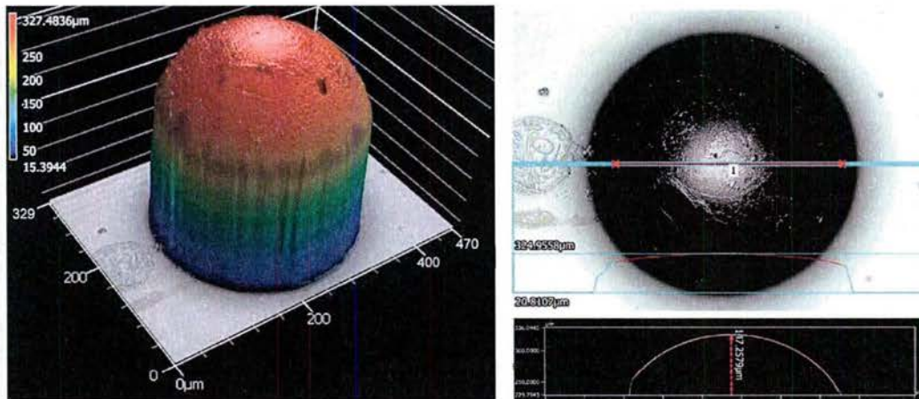
Figure 22. Three-dimensional microscopy image of the sodium acetate solution-infilled microcapsule.
