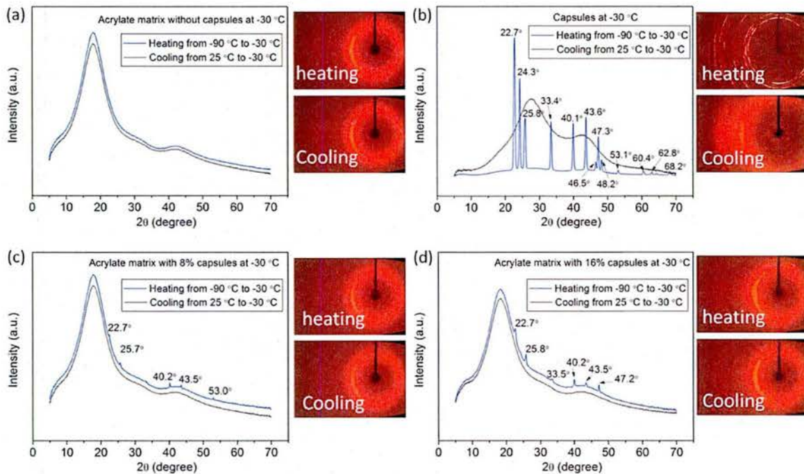
Figure 31. Cold stage XRD patterns obtained at -30\text{ }^{\circ}\text{C} on different samples: (a) acrylate matrix without sodium acetate solution-infilled capsules, (b) sodium acetate solution-infilled acrylate capsules, (c) acrylate matrix embedded with 8% sodium acetate solution-infilled capsules, and (d) acrylate matrix with 16% sodium acetate solution-infilled capsules. The insets are the actual diffraction images for each sample.
