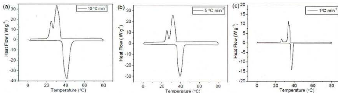
Figure 10. DSC curves of C_{20}H_{42} capsules of about 50 \mu\text{m} in different heating-cooling rates: (a) 10\text{ }^{\circ}\text{C min}^{-1} ; (b) 5\text{ }^{\circ}\text{C min}^{-1} ; (c) 1\text{ }^{\circ}\text{C min}^{-1} .
