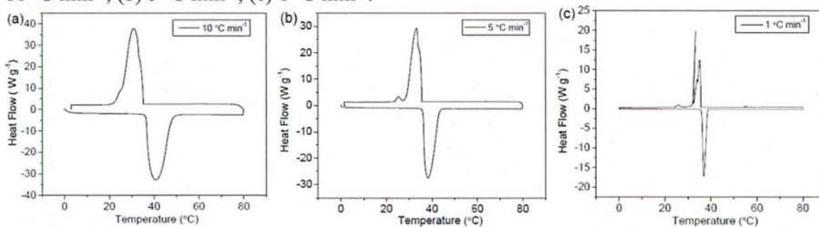
Figure 11. DSC curves of C_{20}H_{42} capsules of about 20 \mu\text{m} in different heating-cooling rates: (a) 10\text{ }^{\circ}\text{C min}^{-1} ; (b) 5\text{ }^{\circ}\text{C min}^{-1} ; (c) 1\text{ }^{\circ}\text{C min}^{-1} .
