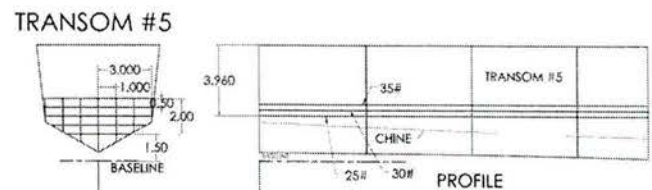
Fig. 4 Transom #5 stripping and dimensions with grid used to measure wave elevations (dimensions shown in inches, displacement in lbf)
