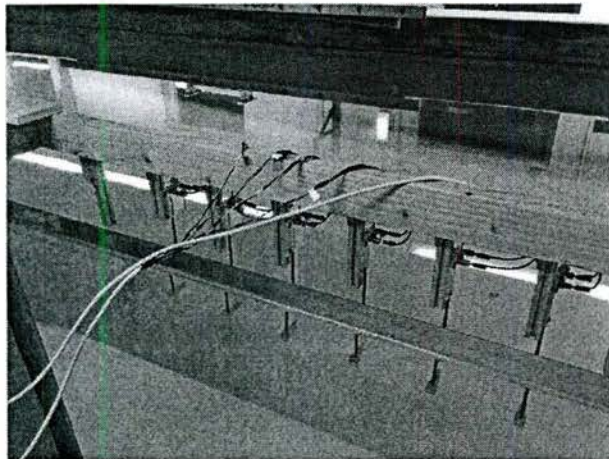
Fig. 7 Photo of wave probe array fixed in the tank side
