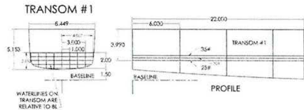
Fig. 1 Transom #1 stripping and dimensions with grid used to Measure wave elevations (dimensions shown in inches, displacement in lbf)
