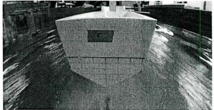
Fig. 3 Transom #5 during unsteady experiment
