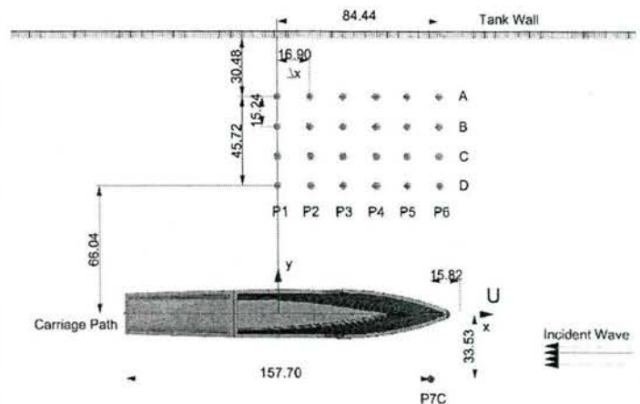
Fig. 8 Wave probe arrangement (dimensions in cm)
