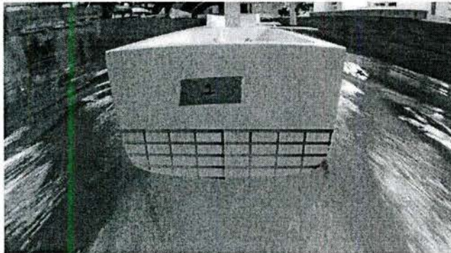
Fig. 2 Transom #1 during unsteady experiment
