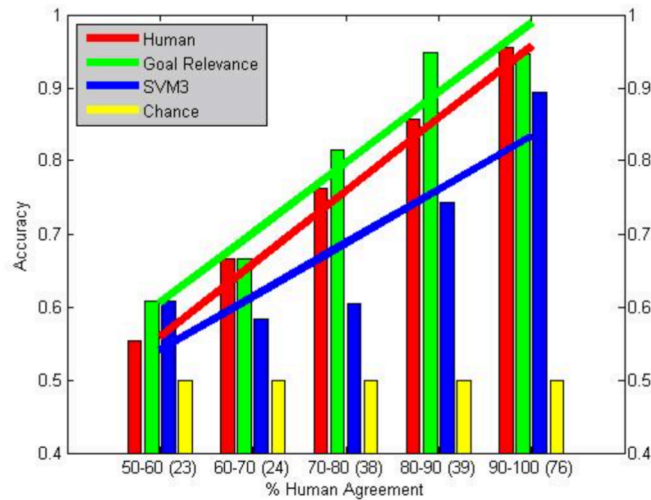
Figure 18: Model accuracies for image pairs with different levels of human agreement, and corresponding regression lines. The number of image pairs in each category is shown on the X axis with the agreement values.
