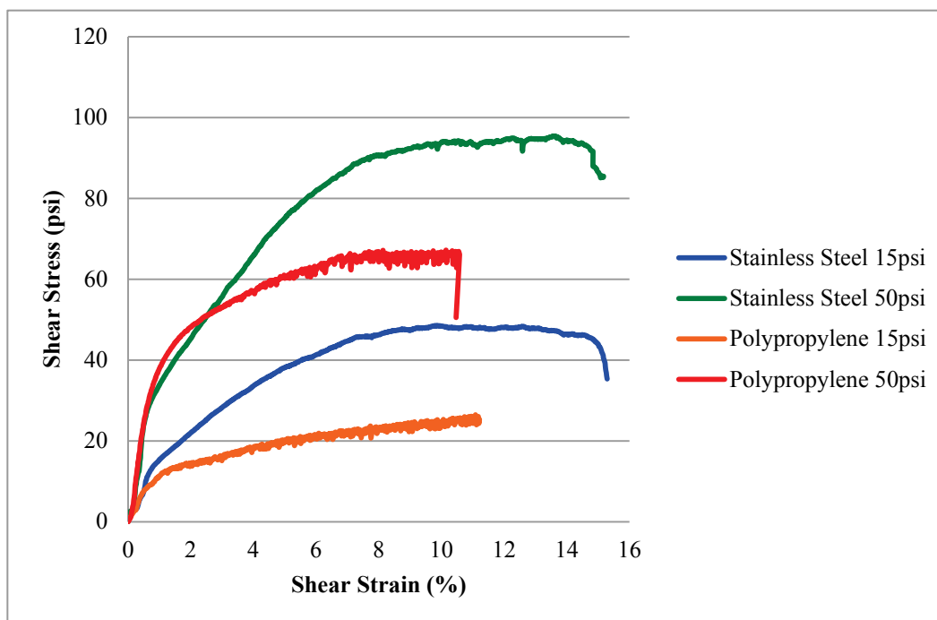
Figure 13. Stress-strain behavior of uniform 0.1875-in. spheres.
