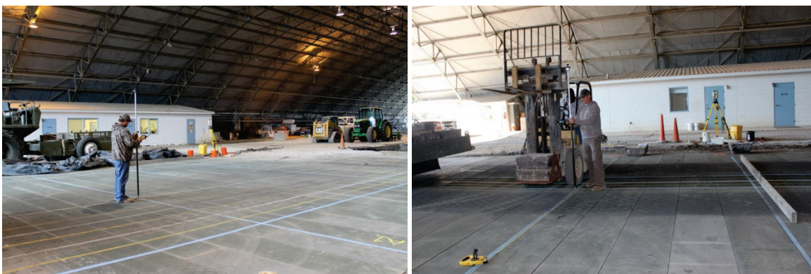
Figure 3.24. Surveying unloaded (left) and loaded (right) cross section.
