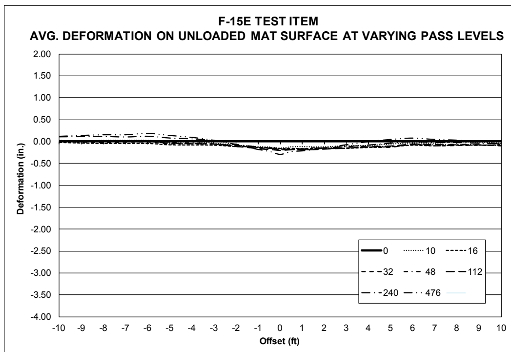
Figure 5.10. Average deformation on the unloaded mat surface of the F-15E item.
