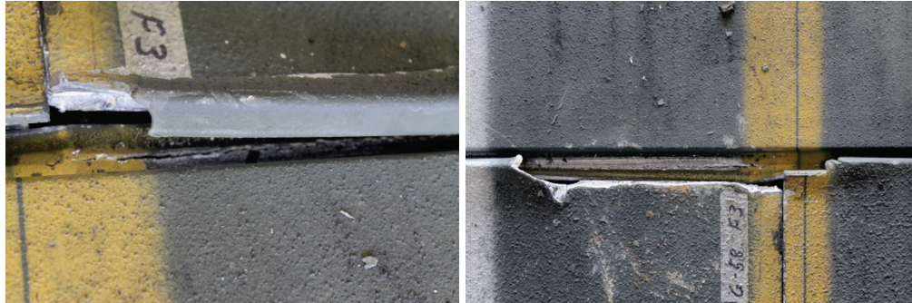
Figure 7.20. Joint of Panels G58 and G53.
