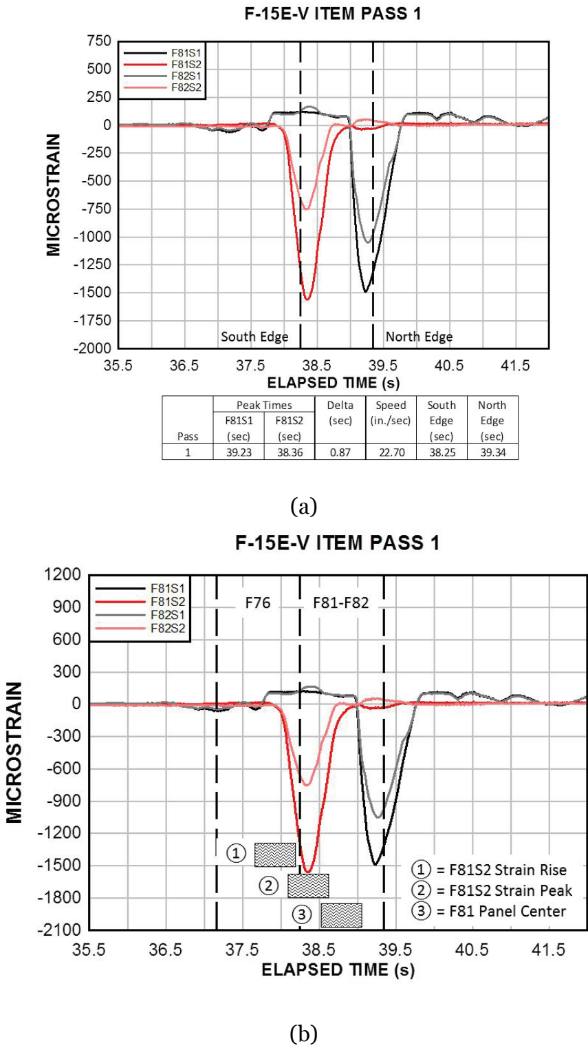
Figure 7.18. (a) F81-F82 joint strain data during pass 1 and (b) tire load footprint locations.
