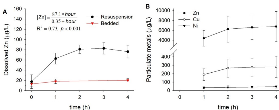
Figure 5-11. Mean ( \pm 1 SD, n = 4 to 8) dissolved Zn (A) and particulate Zn, Cu and Ni (B) during 4-h resuspension and bedded experiments with Lake DePue sediment. Equation in panel A represents nonlinear least squares regression fit model for dissolved metal release during sediment resuspension. Dissolved Cu, Ni, Cr, and Pb were not detected for the duration of experiments.
