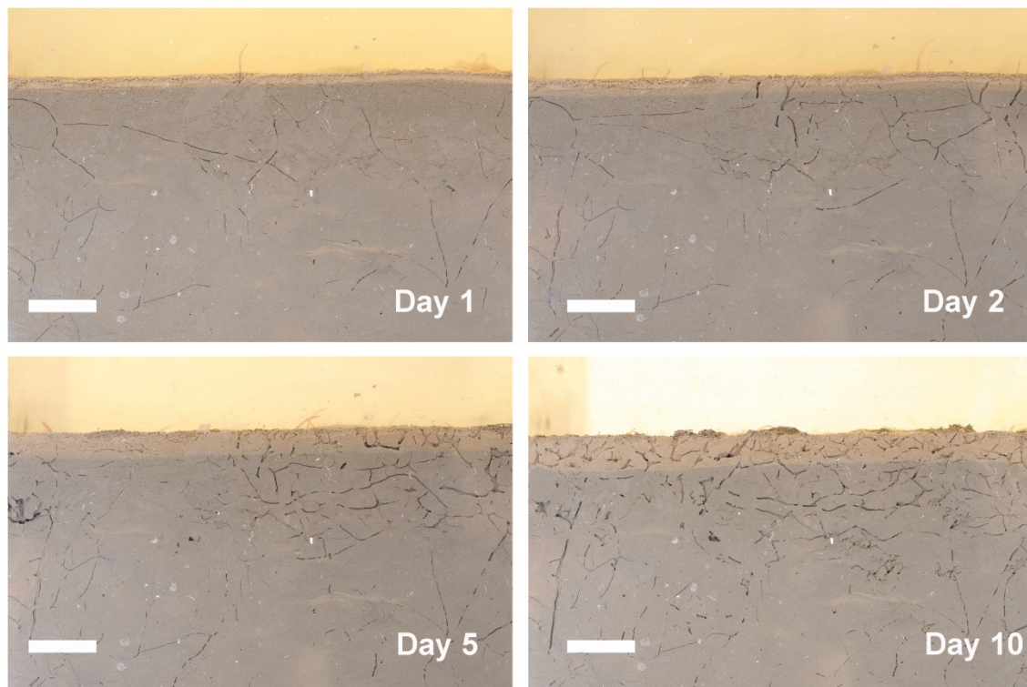
Figure 5-19. Evolution of sediment structures in experiment with reference sediment (B1). Scale bars = 1 cm.
