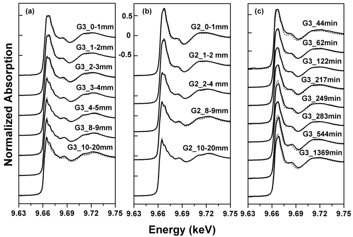
Figure 5-7. XANES spectra (full lines) and reconstructed curves (dotted lines) of sediment samples.
