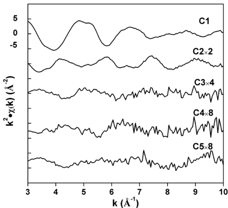
Figure 5-5. The first five components identified by PCA analysis. Amplitudes of C2, C3, C4 and C5 were multiplied by 2, 4, 8, and 8 respectively for clarity.
