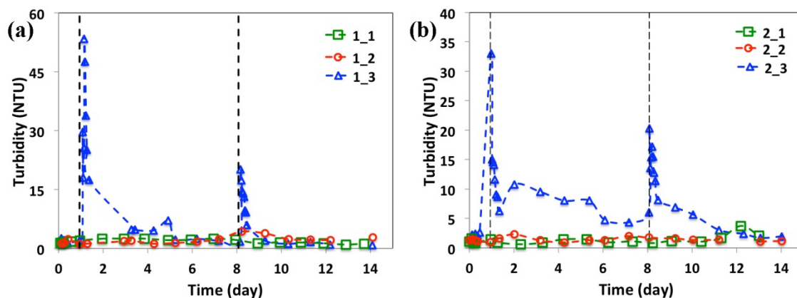
Figure 5-33. Overlying water turbidity. (a) Experiments with fine grained sediments; (b) Experiments with coarser-grained sediments.
