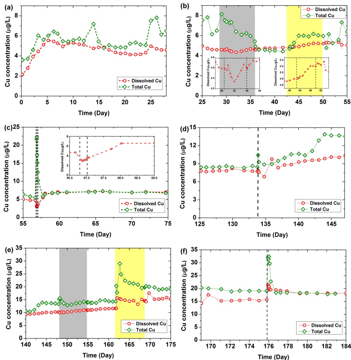
Figure 5-41. Dissolved and total Cu concentrations in the overlying water under varied conditions. (a) Stabilization period with baseline shear stress. (b) Increased hydrodynamic forcing. (c) Sediment resuspension. (d) Bioturbation with baseline shear. (e) Bioturbation with increased hydrodynamic shear. (f) Bioturbation with resuspension. Light gray area and light yellow area indicate 0.22 Pa shear stress and 0.47 Pa shear stress, respectively. Dashed lines in (c) and (f) indicate sediment resuspension. Dashed line in (d) indicates 40 Nereis virens introductions. Error bars represent one standard deviation from Cu analysis.
