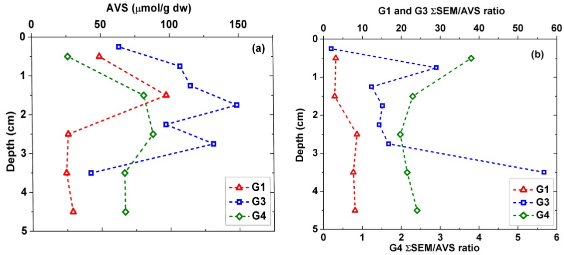
Figure 5-3. Profiles of AVS and SEM:AVS ratio in homogeneous sediments (G4) and intact sediment cores (G1 and G3).
