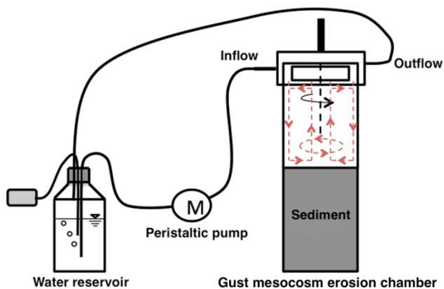
Figure 4-2. Gust chamber setup. Dashed lines inside the chamber indicate the flow pattern within the chamber.
