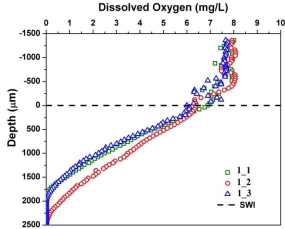
Figure 5-37. Dissolved oxygen concentration profiles in experiments with finer-grained sediments did not vary substantially with overlying flow conditions.
