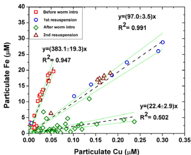
Figure 5-45. Correlation between Fe and Cu concentrations in suspended sediments (particulate fraction of overlying water samples). Red squares represent samples obtained before resuspension and worm introduction (days 10-50). Blue circles represent samples obtained during the first sediment resuspension (day 57). Green diamonds represent samples obtained after the introduction of N. virens but before the second sediment resuspension (days 136-173). Brown triangles represent samples obtained during the second resuspension event (day 176).
