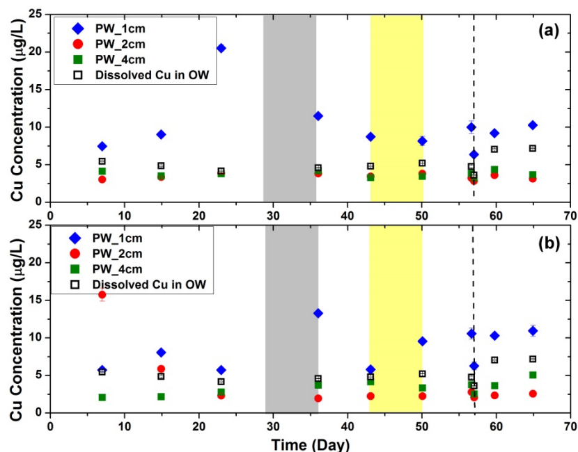
Figure 5-42. Cu concentrations in pore water and overlying water before introduction of Nereis virens at two sampling locations (a,b). Black dashed lines represent sediment resuspension events that lasts for four hours. Error bars represent one standard deviation of replicate measurements.
