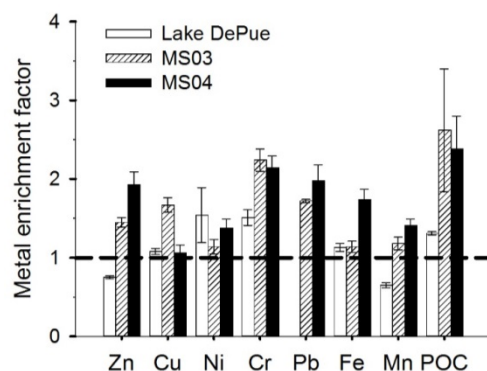
Figure 5-12. Mean ( \pm 1 SD, n = 4-8 ) calculated enrichment factors (e.g., Zn_{SPM}/Zn_{BEDDED} ) after 4-h resuspension experiments of Lake DePue and Portsmouth Naval Shipyard (MS03 and MS04) sediments (POC = particulate organic carbon).
