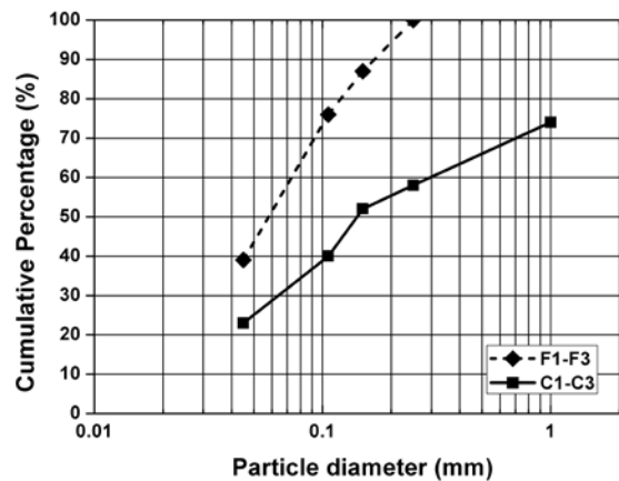
Figure 5-29. Sediment particle size distributions.
