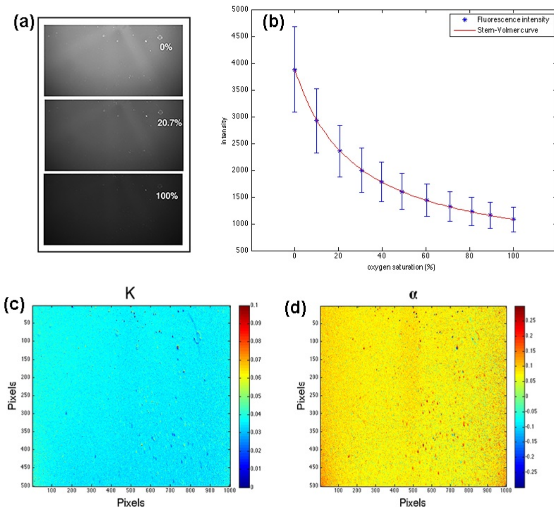
Figure 5-25. (a) Optode images under different O 2 concentrations, reported as percentage of oxygen saturation. (b) The Stern-Volmer equation showed good performance for calibration of optode data under different oxygen concentrations. (c) (d) Distributions of Stern-Volmer equation constants in each pixel across the field of view.
