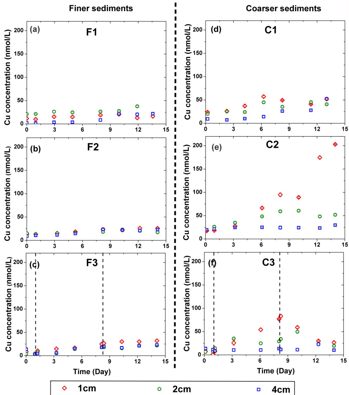
Figure 5-34. Temporal variations in pore water Cu concentrations in experiments with finer-grained sediments (a, b, c) and coarser-grained sediments (d, e, f). Episodic sediment resuspension events in experiments F3 (c) and C3 (f) are indicated by vertical dashed lines. Each sediment resuspension lasted 4 hours (0.17 day).
