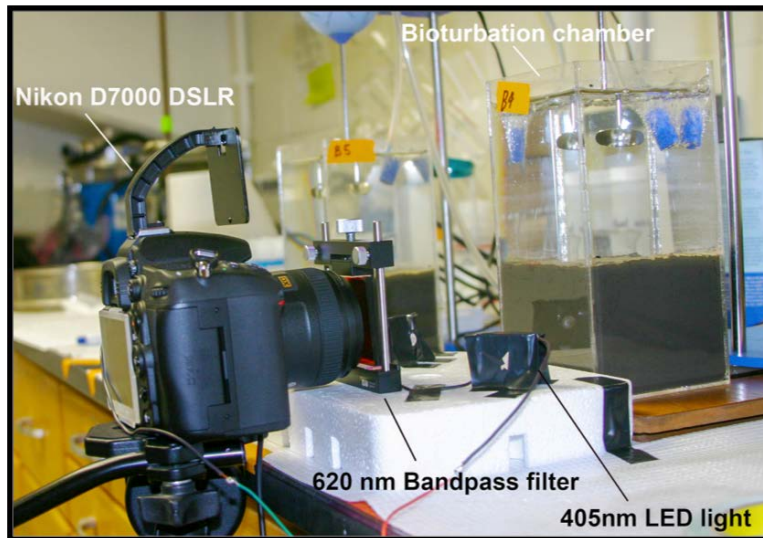
Figure 4-7. LIF-bioturbation experimental setup.
