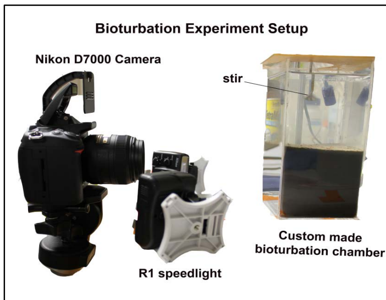
Figure 4-6. Bioturbation experimental setup.
