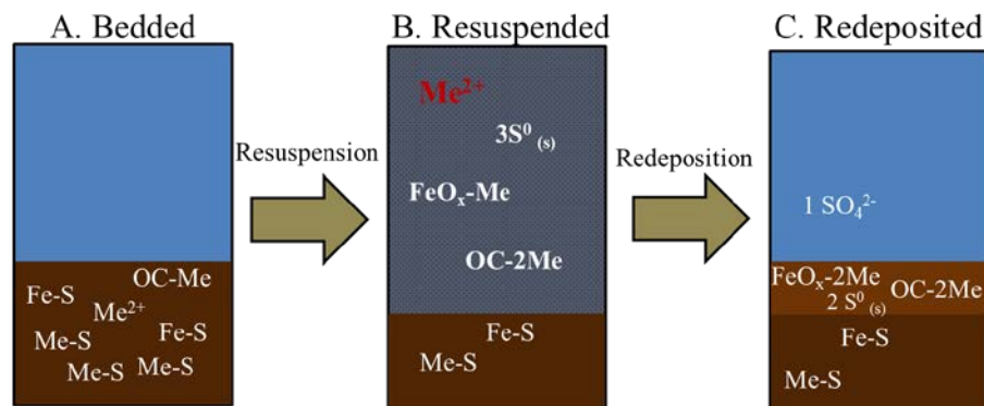
Figure 4-4. Conceptual model of important metal (Me) speciation in various sediment redox states. In bedded sediment (A) the majority of metal is bound as insoluble sulfides or associated with organic carbon (OC). When resuspended, (B) sulfide species are oxidized, mobilizing metals into the overlying water. However, the mobilized metal is scavenged by OC and freshly-precipitated Fe x O x . As particles redeposit, and are returned to the benthic environment (C), further oxidation of sulfur to sulfate can occur in the water column or in the aerobic sediment layer over longer durations (10 – 30h). Note that not all potential chemical reactions and species are represented in this schematic, and sulfur stoichiometry is balanced for clarity but speciation may differ depending on environmental conditions.
