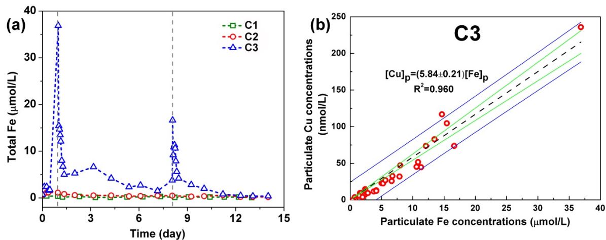
Figure 5-32. (a) Total Fe concentrations in experiments with coarser grained sediments. (b) Particulate Cu and particulate Fe in overlying water samples showed strong correlations. The black dashed line, green curves, and blue curves represent the best linear fit, the 95% confidence interval, and the 95% prediction interval of the fit, respectively.
