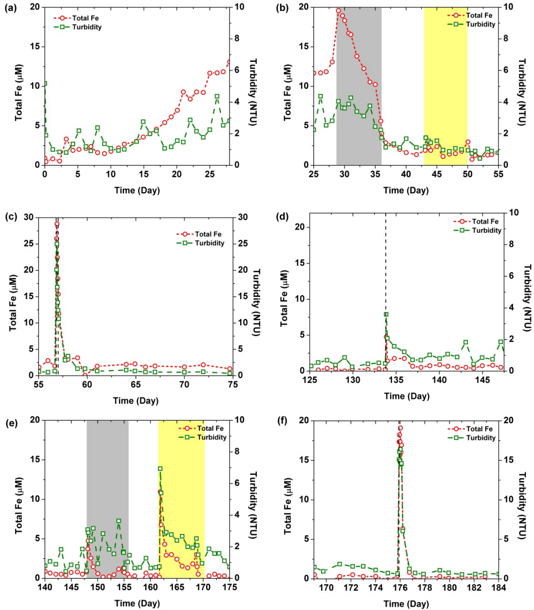
Figure 5-39. Fe concentration and turbidity in the water column in long-term flume experiment. (a) Stabilization period under baseline shear stress. (b) Increased hydrodynamic forcing. (c) Sediment resuspension. (d) Bioturbation with baseline shear. (e) Bioturbation with increased hydrodynamic shear. (f) Bioturbation with resuspension. Light gray area and light yellow area indicate imposed shear stress of 0.22 and 0.47 Pa, respectively. Dashed lines in (c) and (f) indicate sediment resuspension. Dashed line in (d) indicates introduction of 40 Nereis virens .
