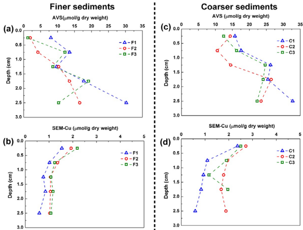
Figure 5-38. AVS and SEM-Cu profiles in experiments with finer and coarser sediments.
