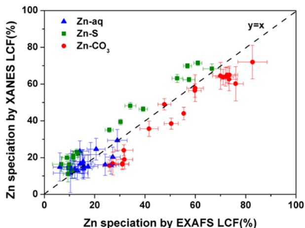
Figure 5-8. Correlation between percentages of Zn species determined by LCF from EXAFS and XANES spectra.
