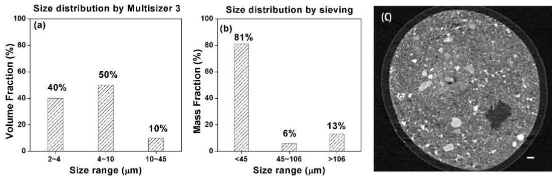
Figure 5-1. (a)(b) Particle size distribution of lake DePue sediments and (c) Microstructure of sediments obtained by XMT imaging. Sample shown has an O.D of 1.9 mm, and was obtained by sub-coring an intact sediment core. The white scale bar represents 100 \mu\text{m} .
