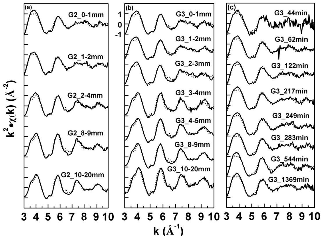
Figure 5-4. EXAFS spectra (full lines) and LCF reconstructed curves (dotted lines) for sediment samples in experiment G2 and G3. (a) Sediment core from experiment G2; (b) Sediment core obtained from experiment G3; (c) Resuspended sediments from experiment G3.
