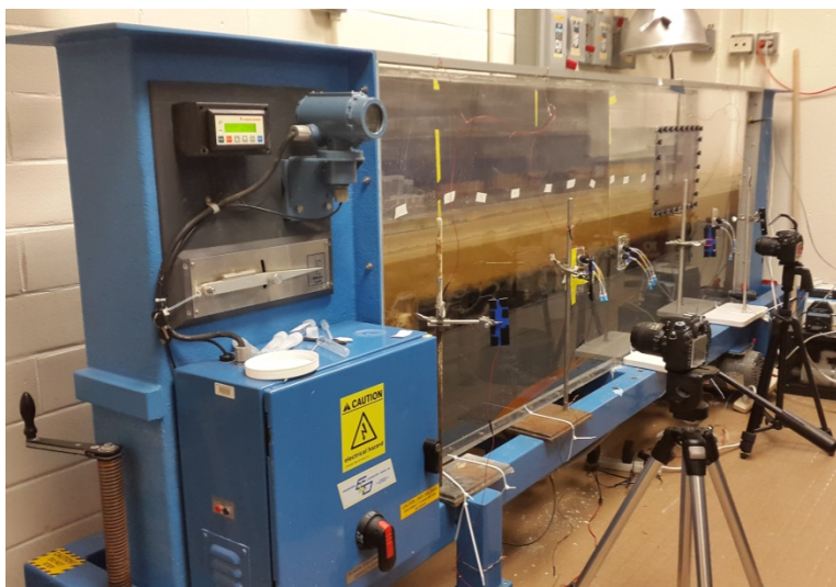
Figure 4-11. Flume experimental setup.
