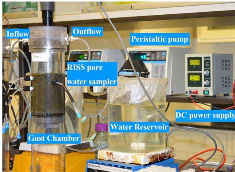
Figure 4-10. Gust chamber system with contaminated sediments.
