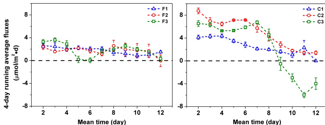
Figure 5-31. 4-day running average fluxes of dissolved Cu in experiments with (a) finer-grained sediments and (b) coarser-grained sediments.
