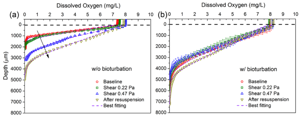
Figure 5-44. Figure 6. Dissolved oxygen profiles under varied hydrodynamic conditions without and with bioturbation. (a) Hydrodynamic forcing enhanced the delivery of oxygen into sediments. (b) Bioturbation also enhanced the transport of oxygen into sediment. Oxygen profiles on each hydrodynamic condition represent average of two individual replicate measurements, and error bars represent the standard deviation. Only one replicate profile was measured for “after resuspension” condition (Dark yellow triangles). Black horizontal dashed curves represent sediment water interface. Purple dashed lines represent the best fitting profiles calculated using the numerical interpretation method by Berg et al. 149
