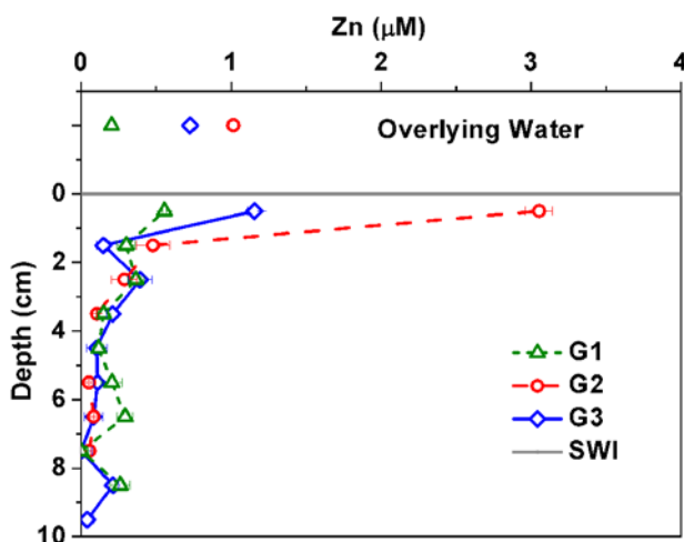
Figure 5-2. Zn concentrations in pore water. G3 was sampled two days after resuspension, G2 was sampled immediately after resuspension, and there was no resuspension in G1. Error bars represent \pm 1 standard deviation.
