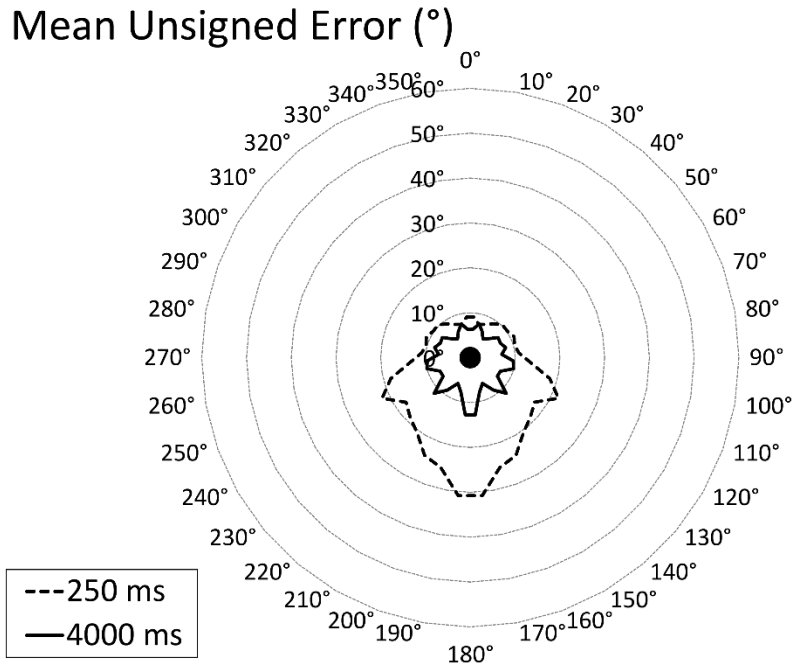
Fig. 12 Mean unsigned error shown as a function of stimulus duration and sound source azimuth
