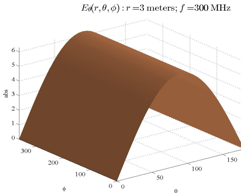
Figure 14: Synthesis of E_\theta(a, \theta, \phi) with m \leq n \leq 3 .
