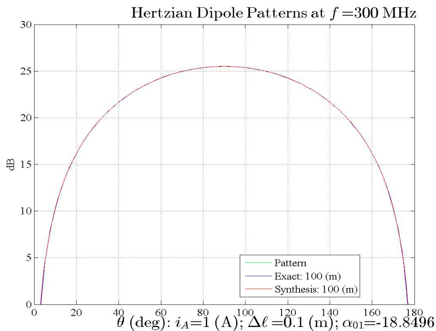
Figure 18: Far-field pattern comparison: i_A = 1 A(A), \lambda = 1 (m), \Delta \ell = \lambda/10 (m).
