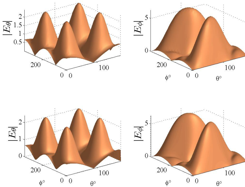
Figure 28: Horizontal dipole at 300 MHz in 3-D; i_A = 1 amp, \ell = \lambda/10 ; upper panels are the simulated fields, lower panels are the synthesized fields.
