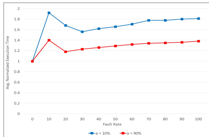
Figure 5: Performance overhead of fault aware thread assignment for modeling accuracy rates of 10 and 90%. Note that this quickly plateaus once the faulty cores have been isolated.
