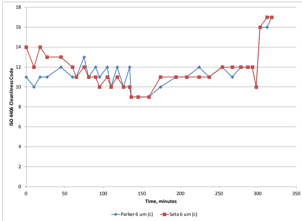
Figure 10. JP-8+100 Test Fuel (20:1 dilution) – Comparison of Particle Counters at 6 µm (c)
