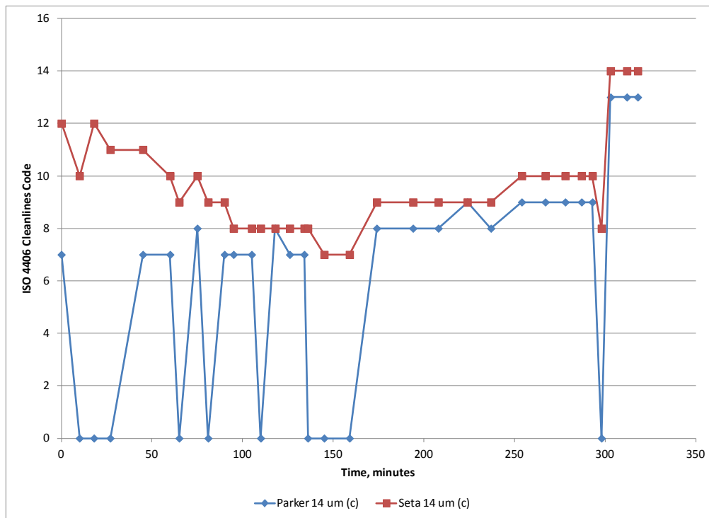
Figure 11. JP-8+100 Test Fuel (20:1 dilution) – Comparison of Particle Counters at 14 µm (c)
