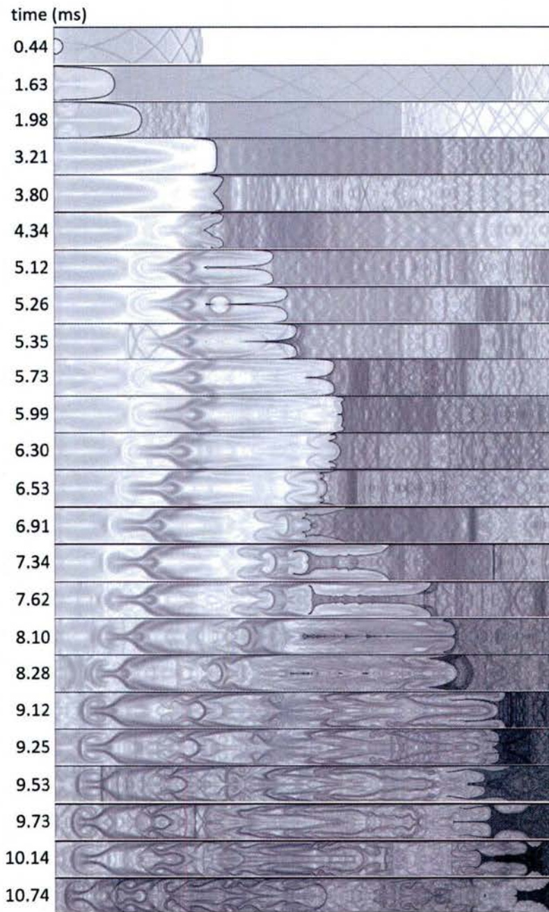
Figure 10. Sequence of numerical schlieren images showing the evolution of premixed stoichiometric hydrogen-air flame and strong pressure waves interacting with the flames in a 4\text{ cm} \times 56\text{ cm} closed channel. Time (ms) is given on the left side of each frame. Only half of the channel was simulated and each time instance is mirrored about the symmetry line (centerline).
