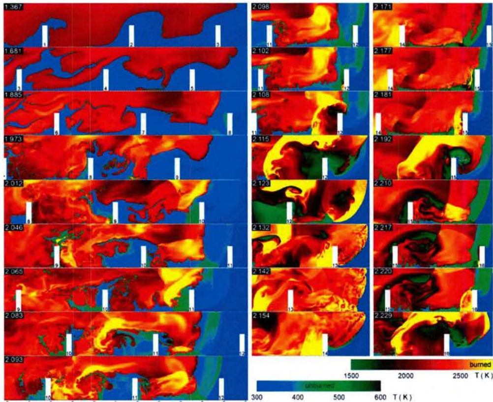
Figure 2. Accelerating flame (left column), DDT, and quasi-detonation (2 right columns) in a half-channel with obstacles computed for the conditions shown by the schematic on top [8]. d/2 = 2 cm, the total channel length L = 64 cm, and dx_{min} = 1/512 cm. Times in milliseconds are shown in frame corners. The channel is filled with a stoichiometric hydrogen-air mixture at P_0 = 1 atm.
