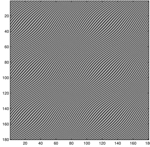
Figure 11: Wideband sinusoidal FM image with IF components outside the range of ESA constraint
