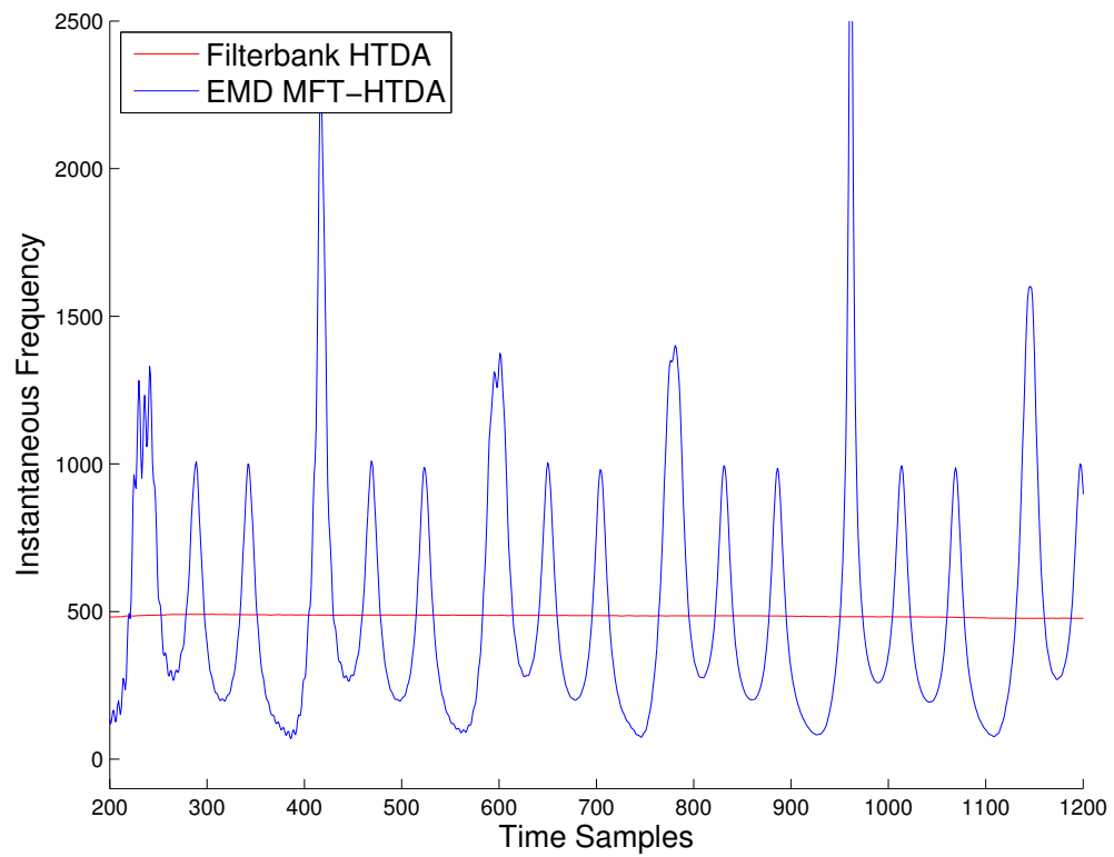
Figure 15: IF demodulation of the first formant
