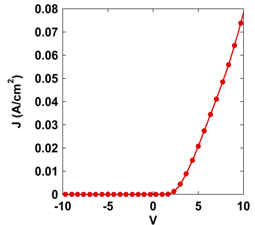
Figure 4. I-V curve of the vertical Mg-implanted GaN pin. The turn on voltage is around 3 V with an on/off ratio of over 10^6 .
