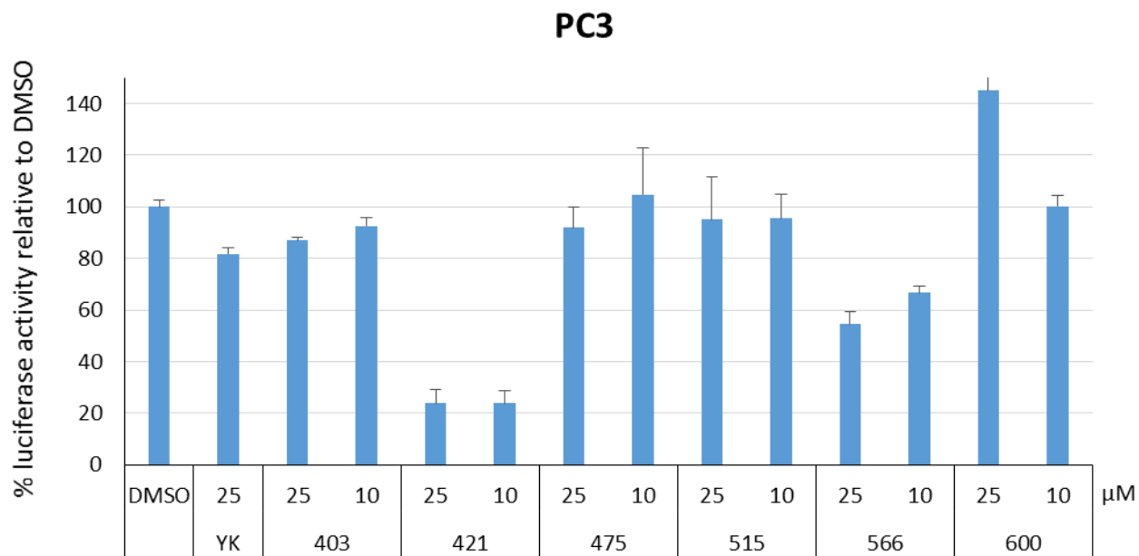
Figure 13. Representative compounds from the luciferase screening assay in PC3 cells. The assay has identified a list of preliminary hit compounds that inhibited the luciferase activity at 10 or 25 μM in PC3 cells that overexpressed ETV4.
