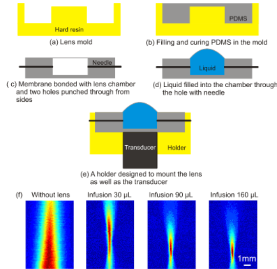
Figure 1. Fabrication of the liquid acoustic lens (a)-(e), measurement of the tunable focal length (f)
