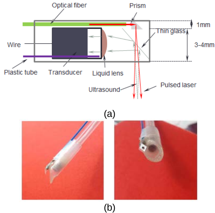
Figure 7. (a) Structure of the endoscopic PAT probe, (b) Fabricated endoscopic PAT probe
