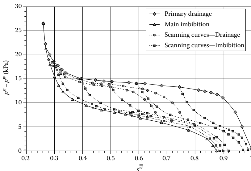
FIGURE 1.3 Pressure-saturation quasi-equilibrium states computed using the LBM.
