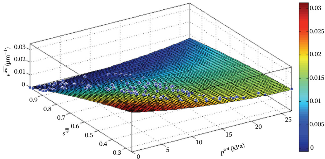
FIGURE 1.6 \bar{\epsilon}^{wn} as a function of p^{wn} and \bar{s}^w for the case in which DNP is excluded.
