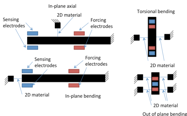
Figure 5. Proposed approach to combine single crystal silicon MEMS (Sandia) fab capabilities and form supporting structure for 2D materials (VU).
