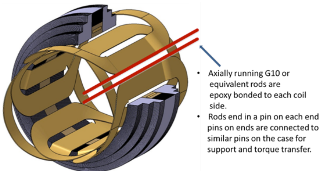
Fig. 2.33: Individual armature coil supported by axially running G10 (or equivalent) support rod
