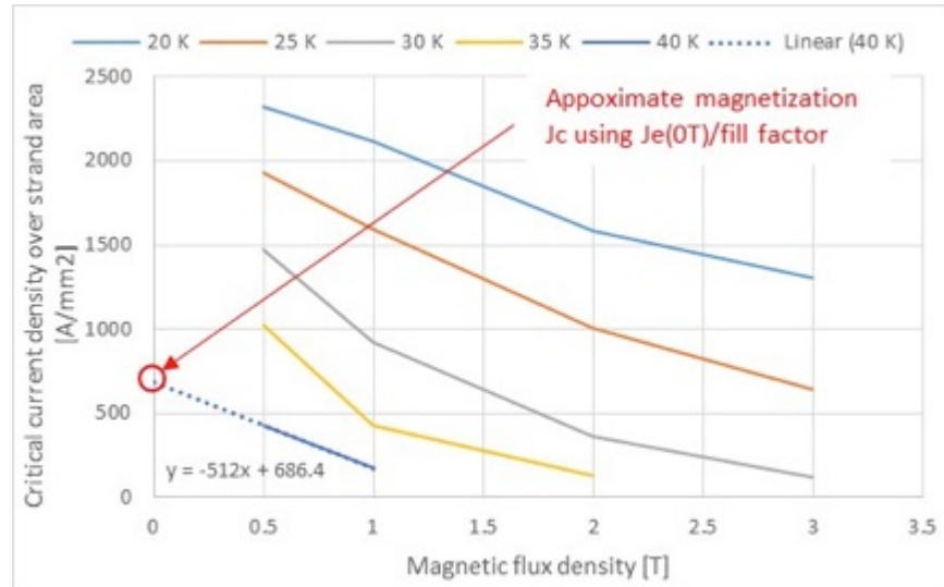
Figure 6.2 Projected performance data for Bi-2212 strands with improved filament density.
