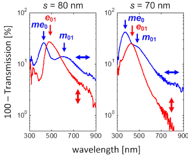
Figure 7. Preferential excitation of magnetic-electric mode in the ultraviolet spectrum. The magnetic, electric, and magnetic-electric modes of v-SRR ( \theta = 30^\circ with 14 nm lateral offset between the arms) for s = 80 nm and s = 70 nm. The insets show the fabricated v-SRR, where the scale bars correspond to 100 nm. The gap separation and feature width are 28 nm and 21 nm, respectively.
