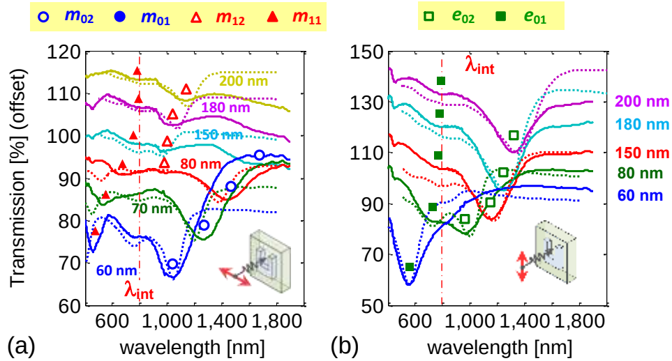
Figure 5. The resonance modes of aluminum u - SRR and their interactions with aluminum interband transition at \lambda_{\text{int}} = 800 nm. Near the interband transition, the fundamental magnetic mode ( m_0 ) splits into m_{01} and m_{02} while the electric mode ( e_0 ) splits into e_{01} and e_{02} . The experimental (solid) and calculated (dashed) transmission spectra of u -SRRs on ITO glass for (a) x-polarization, s = 60 - 100 nm, w = 25 nm, and (b) y-polarization, s = 120 - 200 nm, w = 40 nm. The fundamental magnetic modes are indicated by filled ( m_{01} ) and hollow ( m_{02} ) circles, while the higher order magnetic modes are indicated by filled ( m_{11} ) and hollow ( m_{12} ) triangles. The electric modes are indicated by filled ( e_{01} ) and hollow ( e_{02} ) squares.
