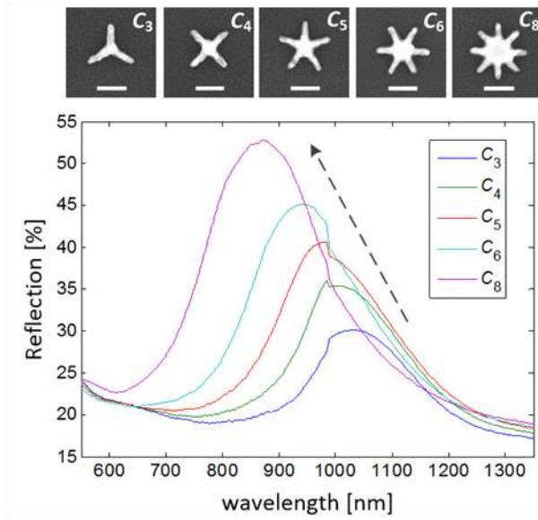
Figure 8. The role of rotational symmetry in the resonance strength. The optical response increase progressively as the internal rotational symmetry changes from three-fold ( n = 3 ) to n = 8 eight-fold ( n = 8 ). The arm length ( s ) and periodicity ( p ) are s = 100 nm and p = 300 nm, respectively. The scale bars in all the insets represent 100 nm.
