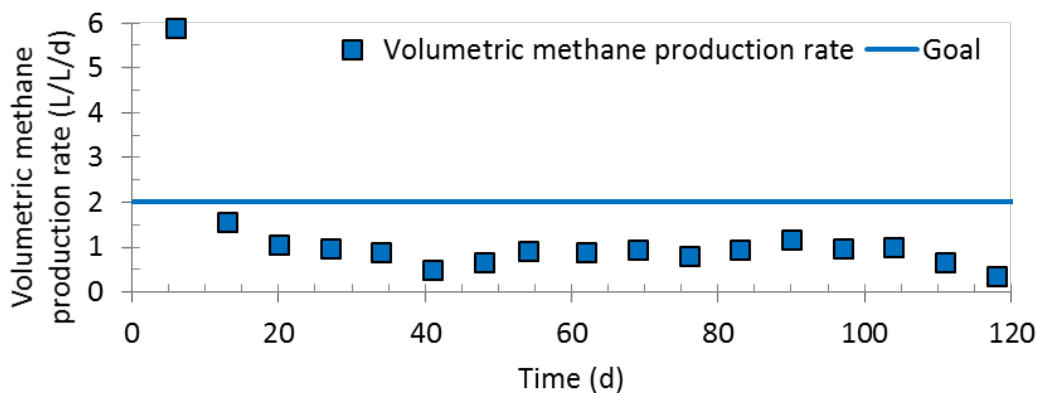
Figure 15. Volumetric Methane Production Rate during Phases II and III Compared to Goal.
