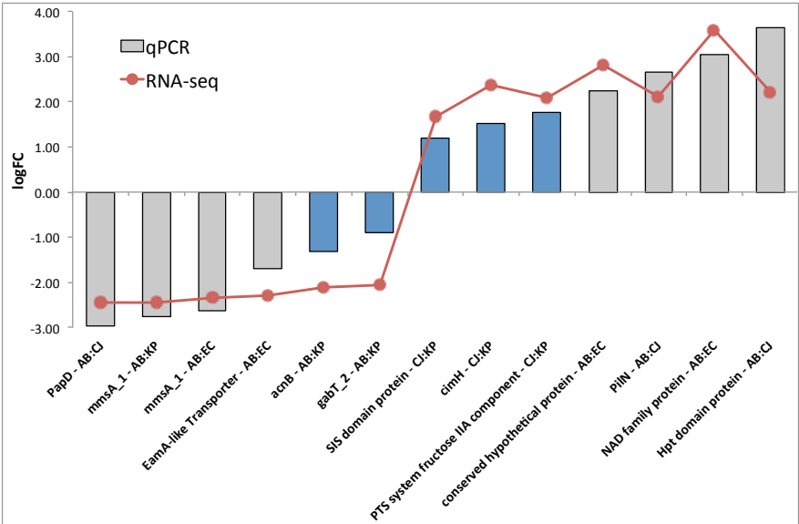
Figure 7. Validation of DE genes. Lines indicated logFC expression from EdgeR analysis of RNA-Seq data and bars indicate logFC expression as measured by qPCR where blue bars are K. pneumoniae genes and gray bars are A. baumannii genes.
