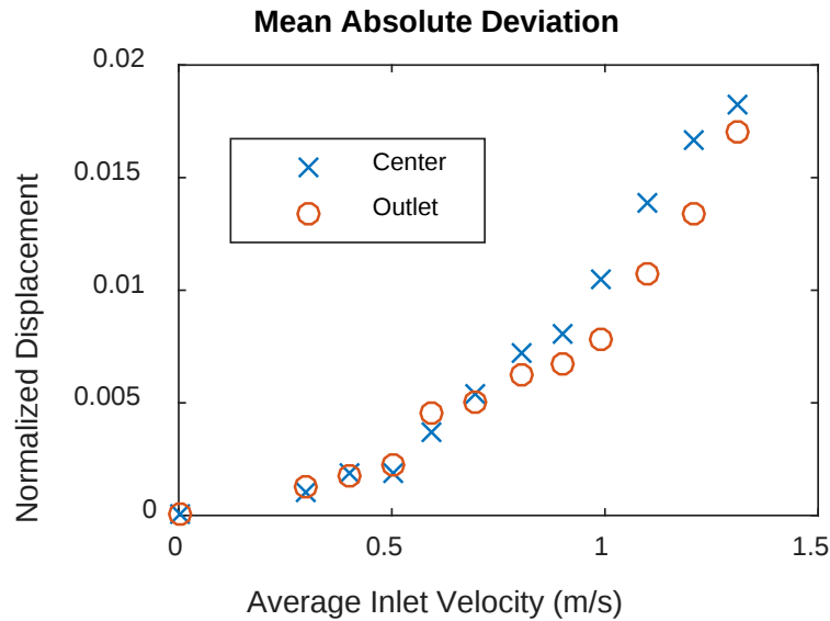
Figure 25. Mean Absolute Deviation from Mean Displacement of the 1.0 mm (0.04”) Thick Plate.
