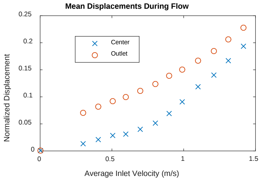
Figure 24. Mean Normalized Displacements of the 1.0 mm (0.04") Thick Plate.
