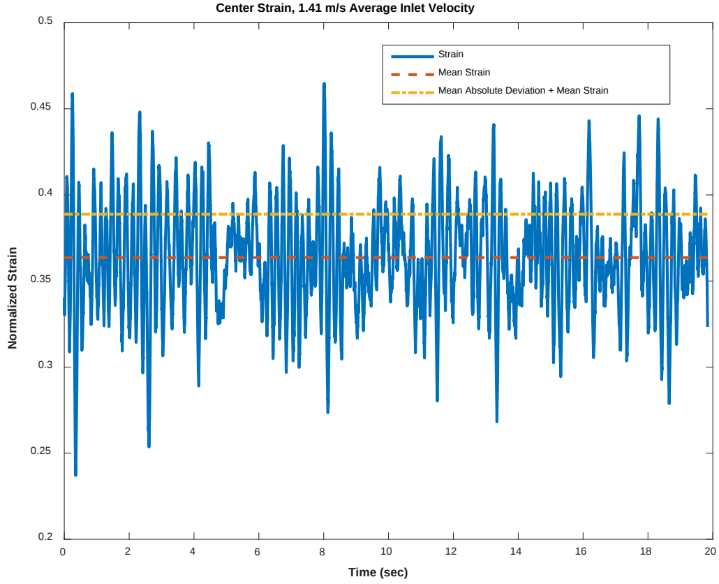
Figure 23. Strain Time History.
