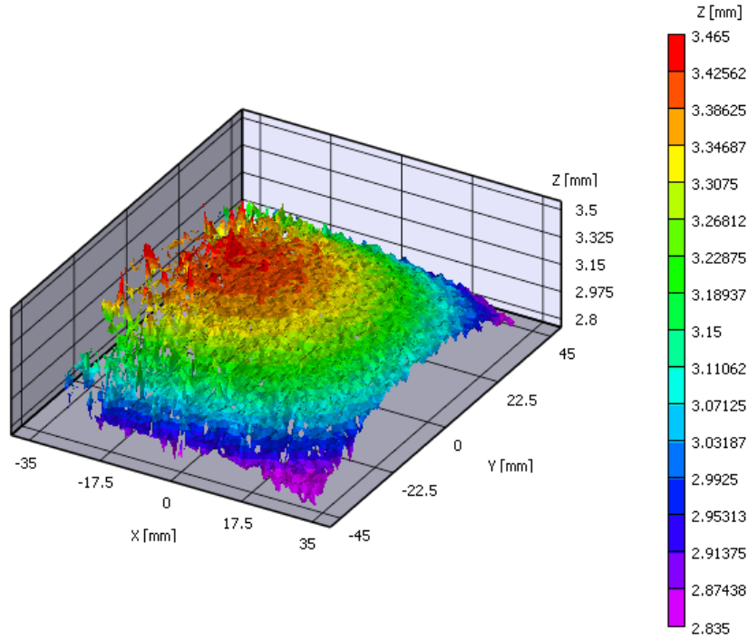
Figure 10. Incomplete Deformation Plot.
