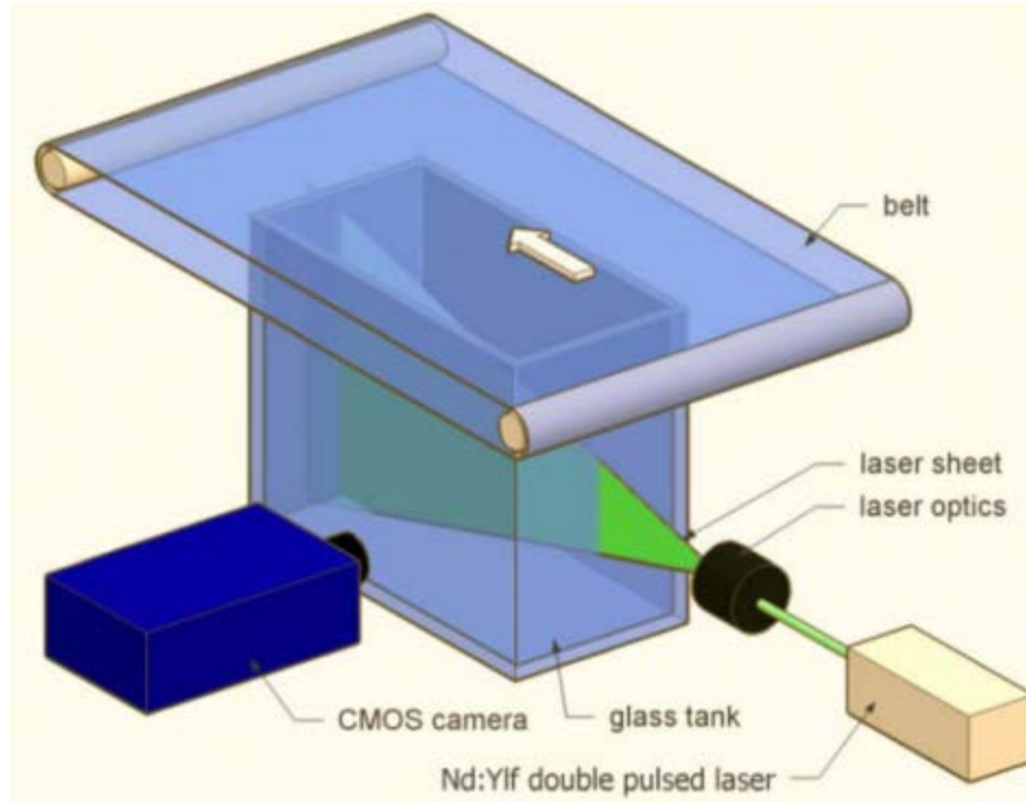
Figure 2. Lid-driven Cavity Flow Belt Drive. Source: [2].
