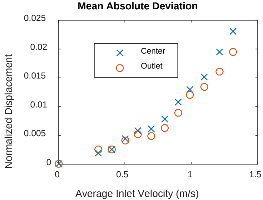
Figure 27. Mean Absolute Deviation from Mean Displacement of the 0.5 mm (0.02") Thick Plate.
