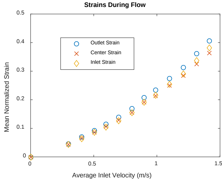
Figure 21. Mean Normalized Strains.
