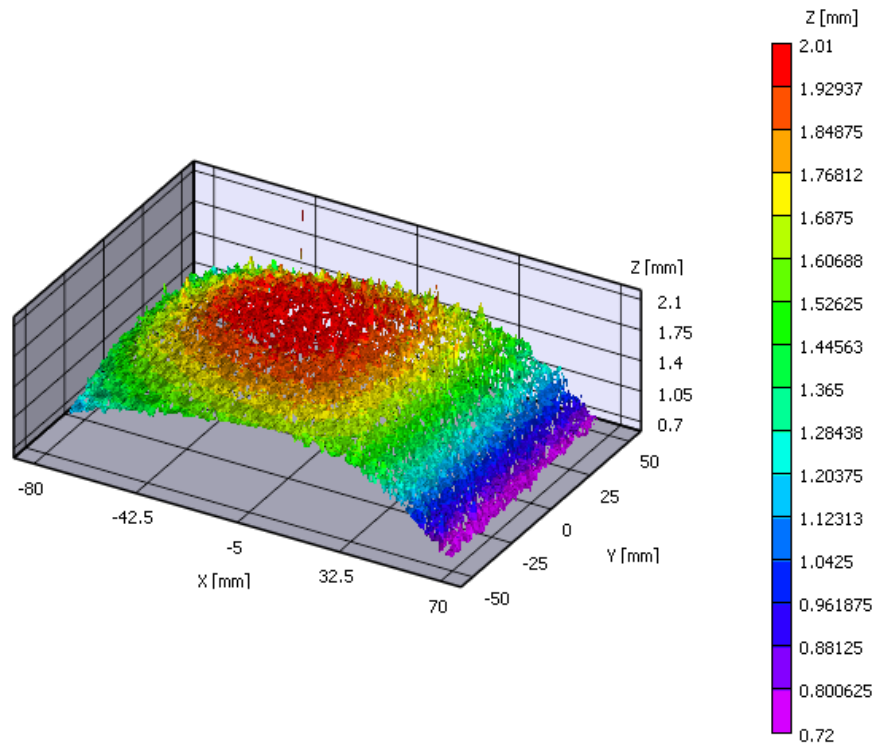
Figure 19. Aluminum Displacement.
