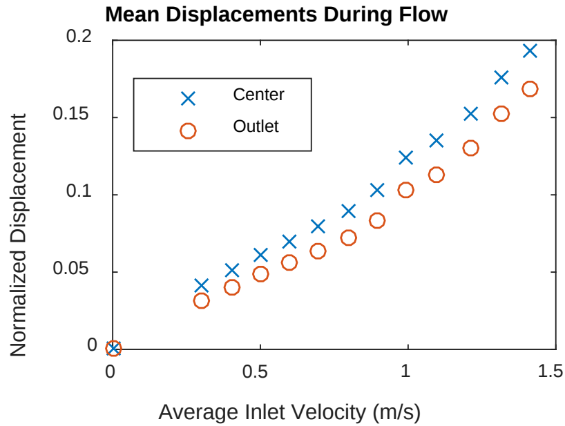
Figure 26. Mean Normalized Displacements of the 0.5 mm (0.02”) Thick Plate.
