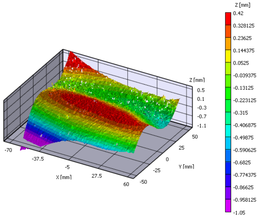
Figure 14. Warping Deformation of Stainless Steel.
