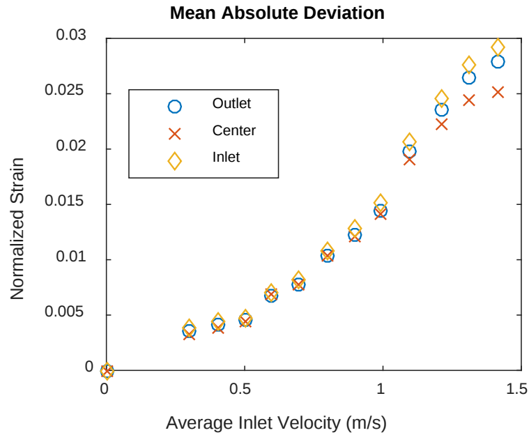
Figure 22. Mean Absolute Deviation of Strains.
