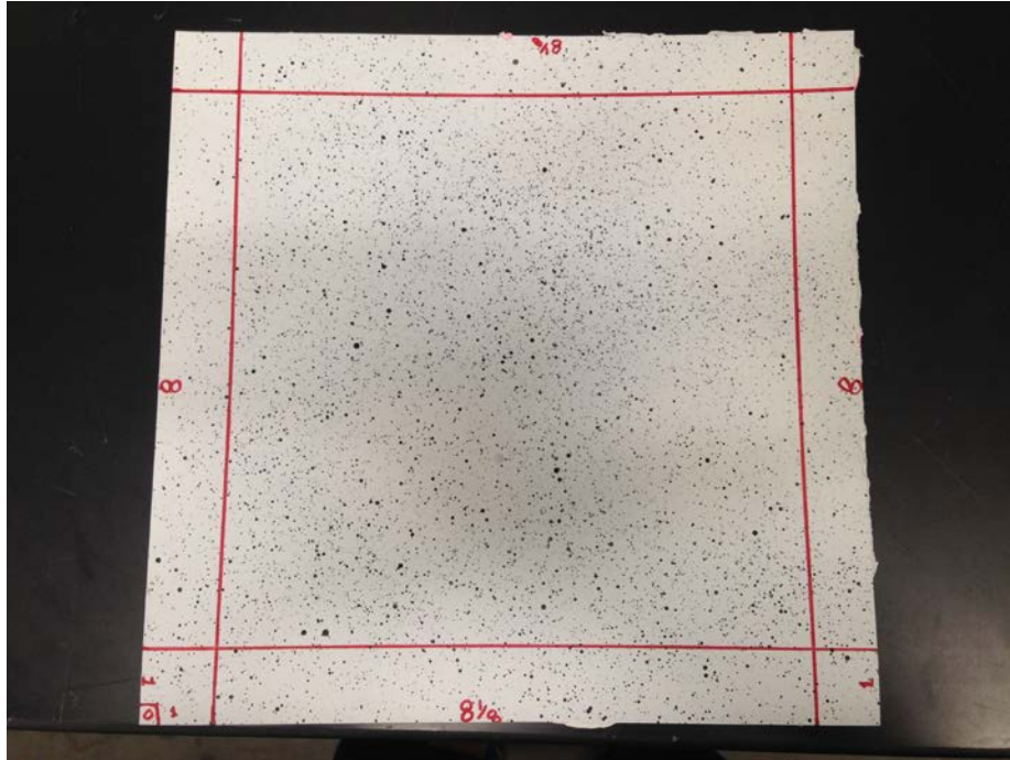
Figure 9. Speckle Pattern on the Deformable Plate.
