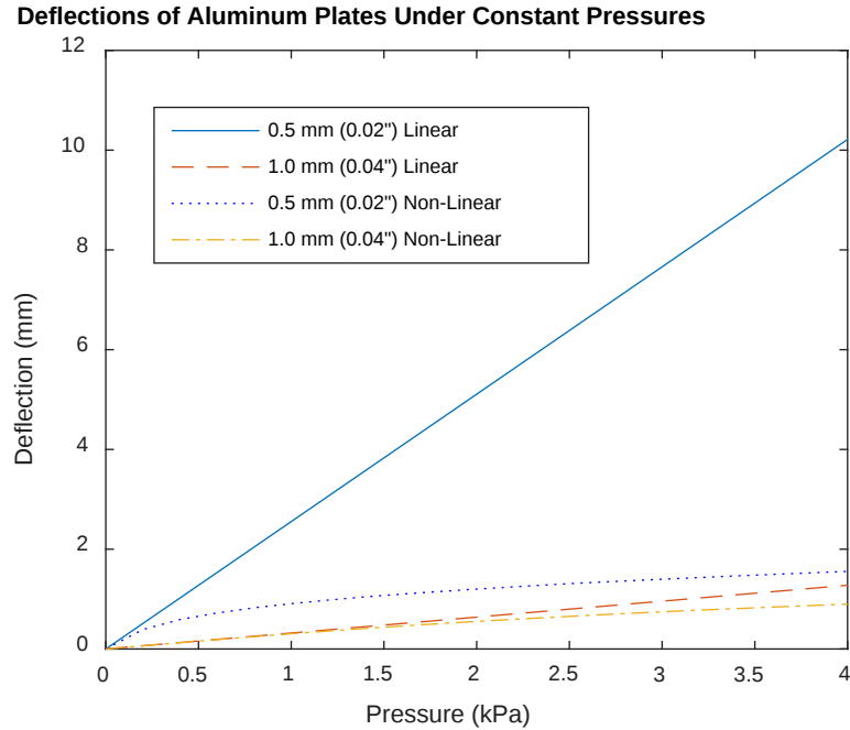
Figure 15. Deflection of Aluminum Plates.
