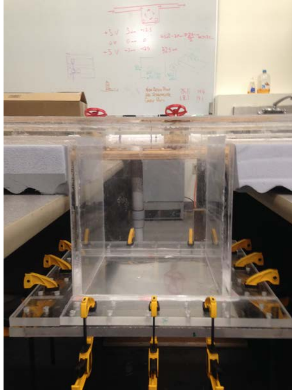
Figure 13. Cavity with Clamped Boundary Conditions of Plate.
