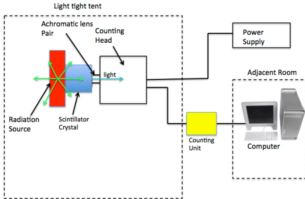
Figure 22. Gamma radiation Hamamatsu 7421-40 counting head and dark room setup.
