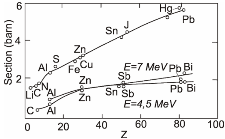
Figure 5. Inelastic scattering cross section (lower curves) of target nuclei with atomic number (Z) for the neutron energies 4.5 MeV and 7 MeV. Source: [3].
