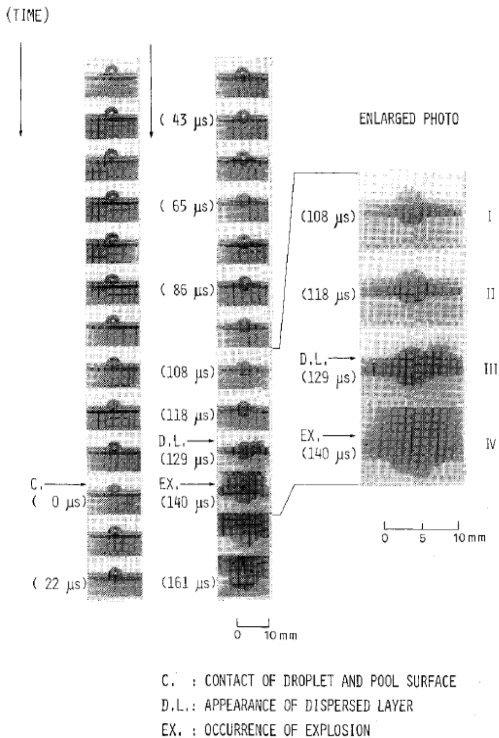
Figure 2. High speed motion pictures (92900 frames per second) of the contact of a \text{N}_2\text{H}_4 droplet falling into a NTO pool.
