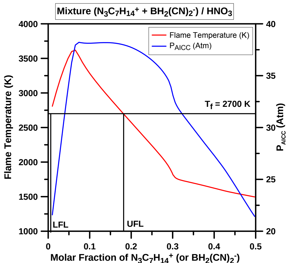
Figure 21: Flame temperature and P_{\text{AICC}} for different \text{N}_3\text{C}_7\text{H}_{14}^+ + \text{BH}_2(\text{CN})_2^- / \text{HNO}_3 mixtures at 298.15 K and 1 Atm.
