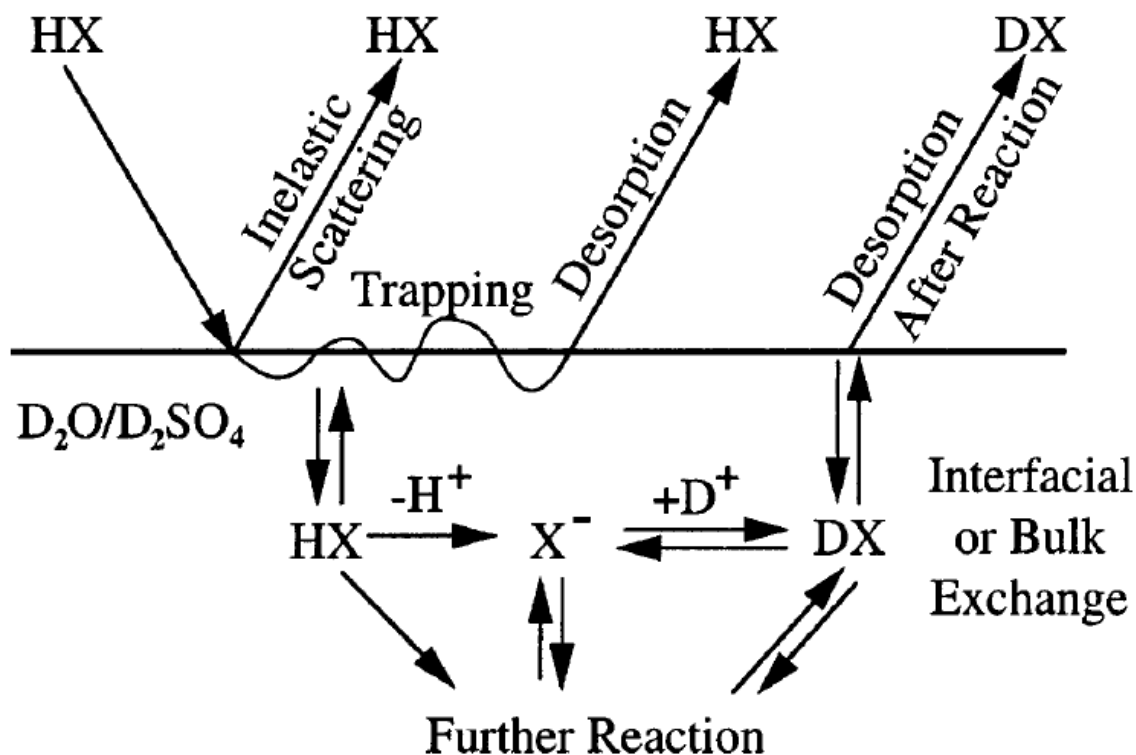
Figure 5. Observed pathways for an acidic molecule \text{HX} colliding into \text{D}_2\text{O}/\text{D}_2\text{SO}_4 [Nathanson, 2004].
