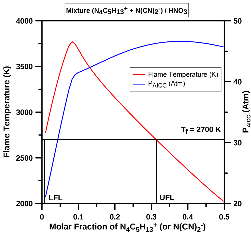
Figure 17: Flame temperature and P_{AICC} for different N 4 C 5 H 13 + + N(CN) 2 - / HNO 3 mixtures at 298.15 K and 1 Atm.
