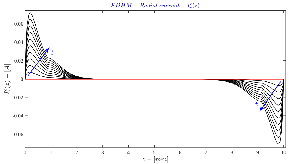
Figure 4.11: FDHM - Total radial electric current
