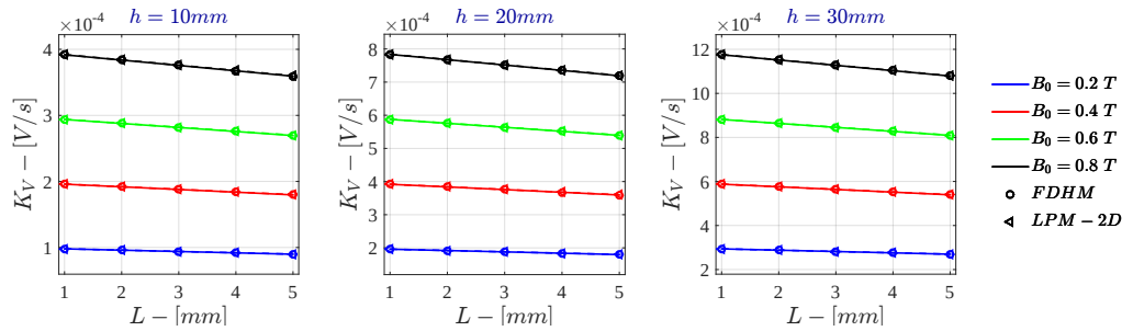
Figure G.28: Bidimensional LPM K_V for \sigma = 10^3 \text{ S/m} - r_{out} = 50\text{mm}
