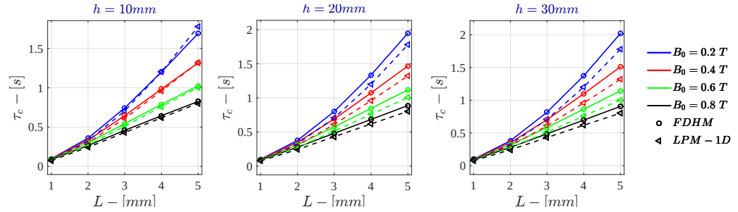
Figure H.10: Monodimensional LPM - Current Drive \tau_c for \sigma = 10^4 \text{ S/m} - r_{out} = 50 \text{ mm}
