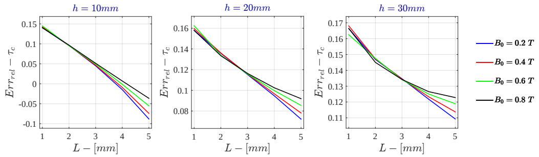
Figure G.14: Monodimensional LPM - Current Drive Relative Error - \tau_c for \sigma = 10^3 \text{ S/m} - r_{out} = 50\text{mm}
