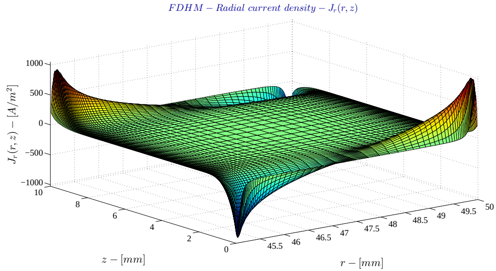
Figure 5.2: FDHM - Radial electric current density
