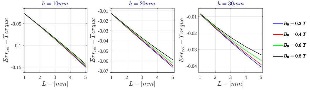
Figure 7.37: Bidimensional LPM - Current Drive Relative Error - \dot{\Gamma} for \sigma = 10 \text{ S/m} - r_{out} = 50\text{mm}
