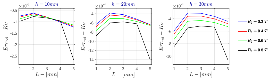
Figure H.8: Monodimensional LPM Relative Error - K_V for \sigma = 10^4 \text{ S/m} - r_{out} = 50\text{mm}
