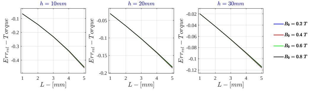
Figure 7.21: Monodimensional LPM - Voltage Drive Relative Error - \dot{\Gamma} for \sigma = 10 \text{ S/m} - r_{out} = 50\text{mm}
