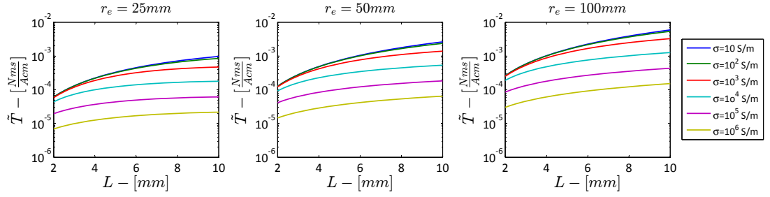
Figure 8.7: Torque function of L for \sigma = 10 \div 10^6 S/m and 3 different outer radii r_e = 25, 50, 100mm . B_0 = 1.0 T . \rho = 1000 Kg/m^3 .
