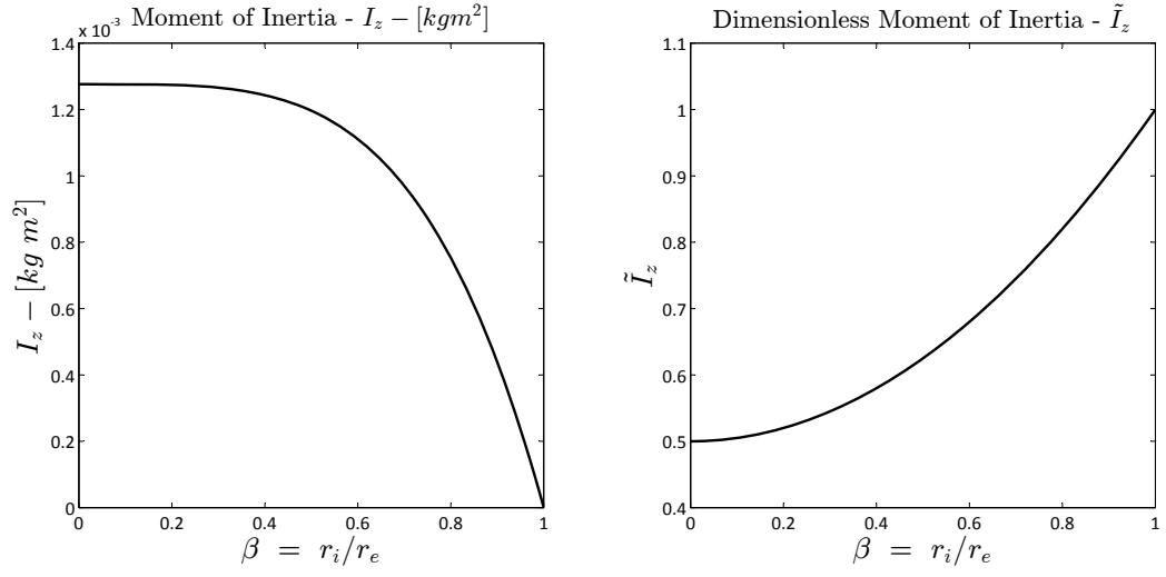
Figure 2.5: Dimensional and Dimensionless Moment of Inertia - 1 st Configuration
