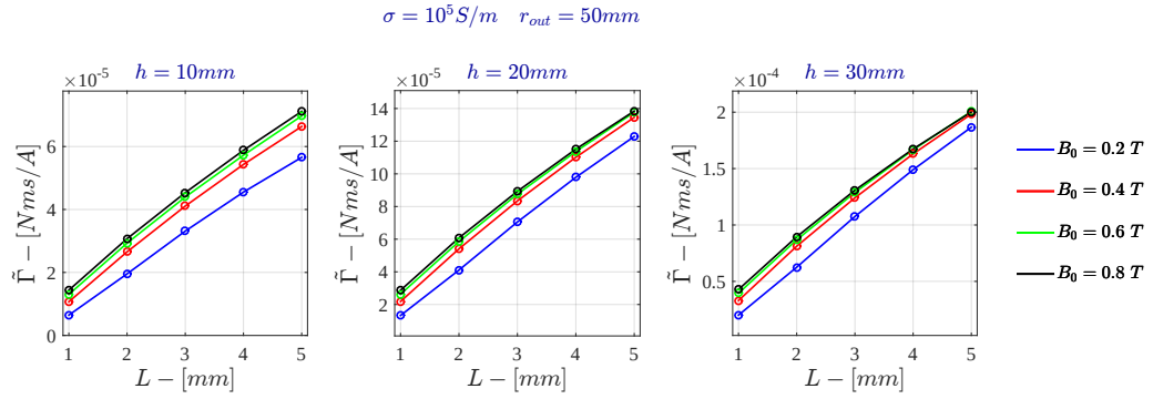
Figure E.10: Voltage Drive - Specific Angular Momentum for \sigma = 10^5 \text{ S/m} - FDHM
