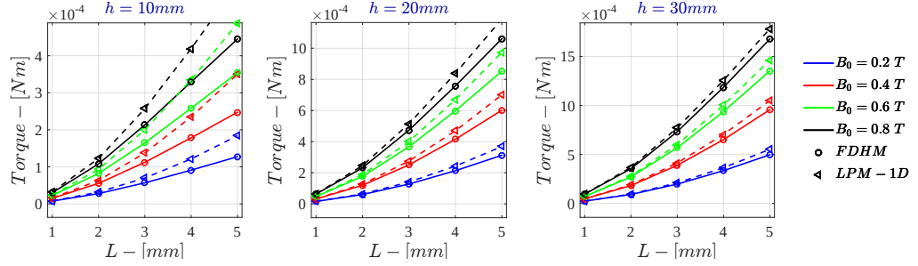
Figure G.9: Monodimensional LPM - Current Drive \dot{\Gamma} for \sigma = 10^3 \text{ S/m} - r_{out} = 50\text{mm}
