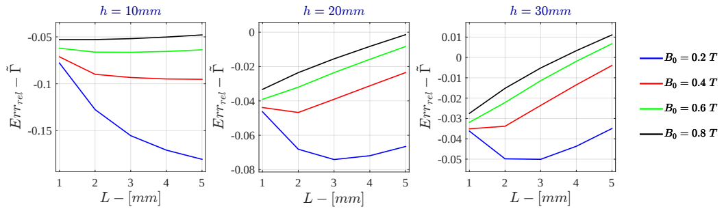
Figure I.24: Monodimensional LPM - Voltage Drive Relative Error - \tilde{I} for \sigma = 10^5 \text{ S/m} - r_{out} = 50\text{mm}
