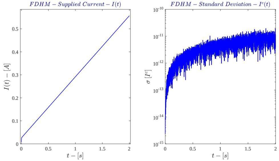
Figure 4.12: FDHM - Error of the electric side of the MHD problem
