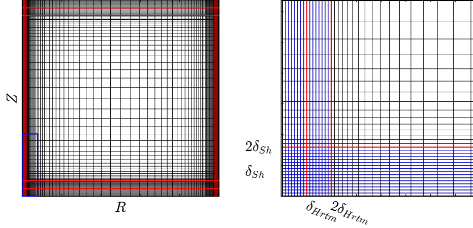
Figure 4.3: Grid for \delta_{Sh} \leq h/6 and \delta_{Hrtm} \leq (r_e - r_i)/6 .
