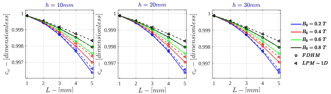
Figure H.3: Monodimensional LPM c_\omega for \sigma = 10^4 \text{ S/m} - r_{out} = 50 \text{ mm}
