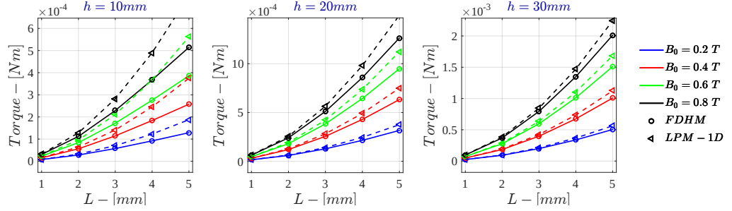
Figure 7.9: Monodimensional LPM - Current Drive \dot{\Gamma} for \sigma = 10 \text{ S/m} - r_{out} = 50 \text{ mm}
