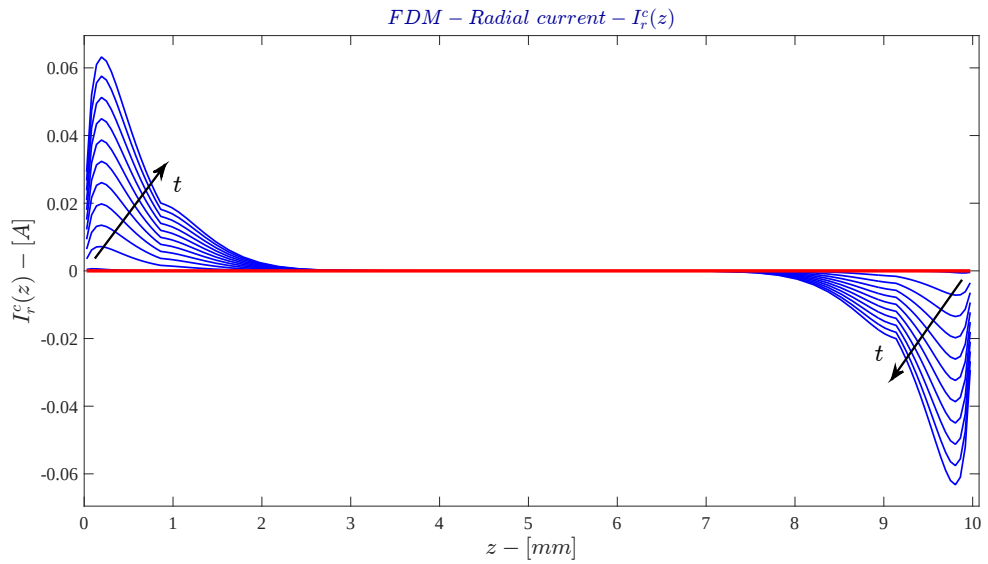
Figure 4.7: FDM - Total radial electric current
