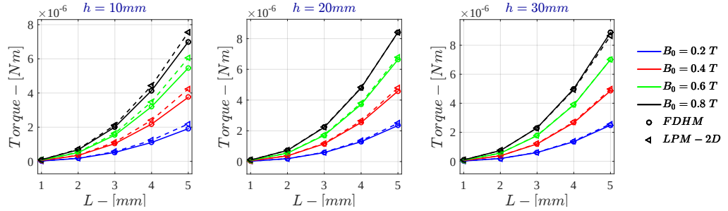
Figure F.41: Bidimensional LPM - Voltage Drive \dot{\Gamma} for \sigma = 10^2 \text{ S/m} - r_{out} = 50\text{mm}
