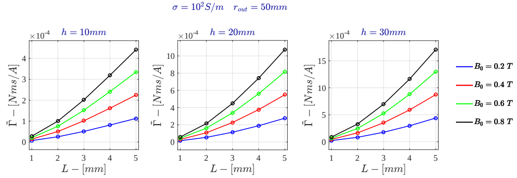
Figure B.10: Voltage Drive - Specific Angular Momentum for \sigma = 10^2 \text{ S/m} - FDHM
