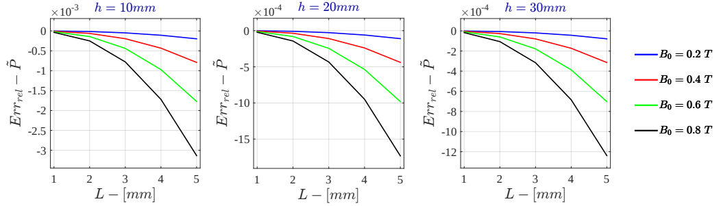
Figure 7.23: Monodimensional LPM - Voltage Drive Relative Error - \tilde{P} for \sigma = 10 \text{ S/m} - r_{out} = 50\text{mm}
