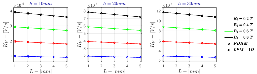
Figure I.4: Monodimensional LPM K_V for \sigma = 10^5 \text{ S/m} - r_{out} = 50 \text{ mm}
