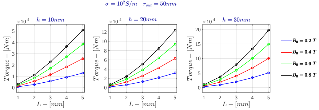
Figure B.1: Current Drive - Torque for \sigma = 10^2 \text{ S/m} - FDHM
