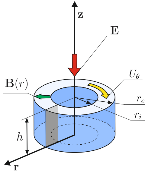
Figure 2.1: Section of an annulus with applied electric field \mathbf{E} and radial magnetic field \mathbf{B}(r) .
