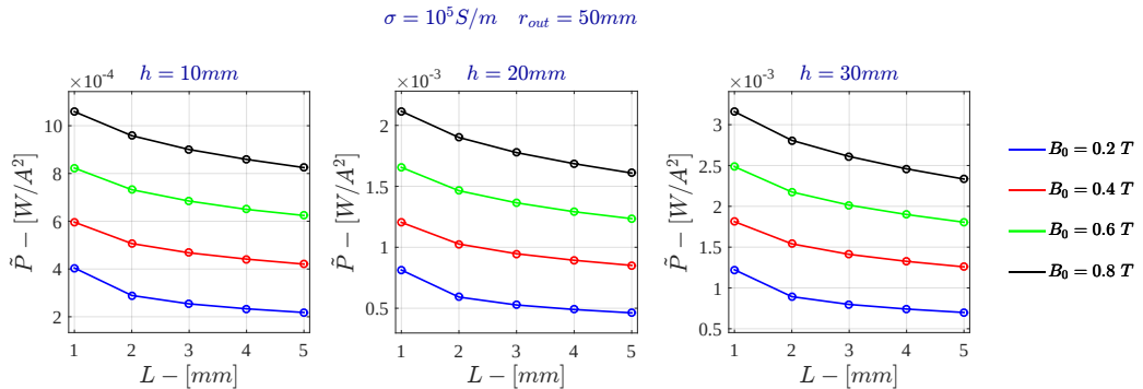
Figure E.9: Voltage Drive - Specific Power for \sigma = 10^5 \text{ S/m} - FDHM
