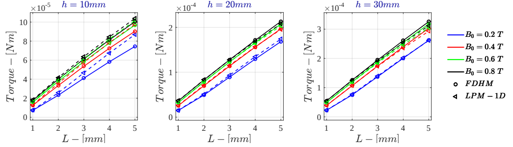
Figure I.9: Monodimensional LPM - Current Drive \dot{\Gamma} for \sigma = 10^5 \text{ S/m} - r_{out} = 50\text{mm}
