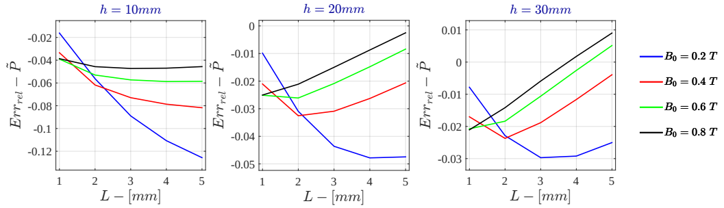
Figure I.23: Monodimensional LPM - Voltage Drive Relative Error - \tilde{P} for \sigma = 10^5 \text{ S/m} - r_{out} = 50\text{mm}
