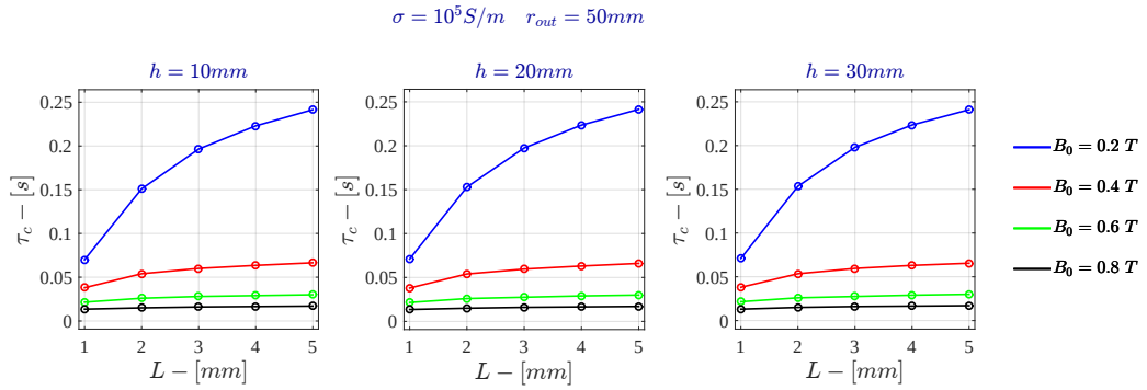
Figure E.8: Voltage Drive - Characteristic time for \sigma = 10^5 \text{ S/m} - FDHM
