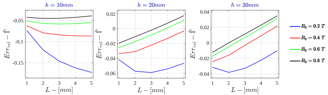
Figure I.16: Monodimensional LPM - Current Drive Relative Error - \tilde{\Gamma} for \sigma = 10^5 \text{ S/m} - r_{out} = 50\text{mm}
