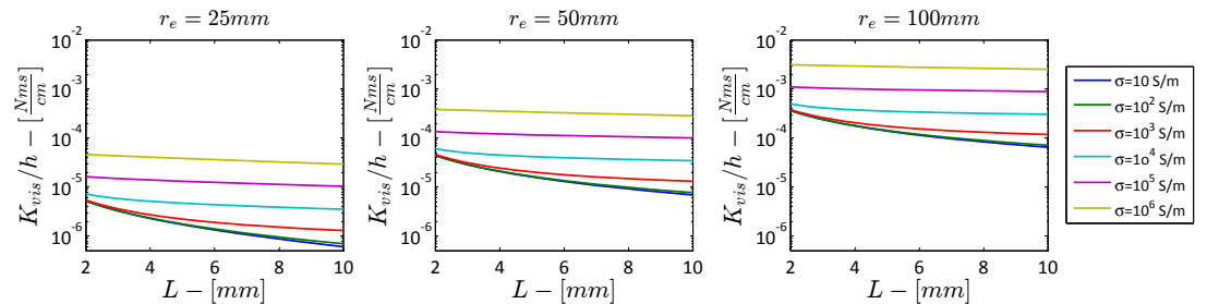
Figure 8.6: K_{vis} function of L for \sigma = 10 \div 10^6 \text{ S/m} and 3 different outer radii r_e = 25, 50, 100 \text{ mm} . B_0 = 1.0 \text{ T} . \rho = 1000 \text{ Kg/m}^3 .
