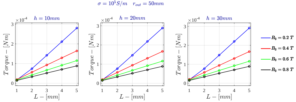
Figure E.7: Voltage Drive - Torque for \sigma = 10^5 \text{ S/m} - FDHM
