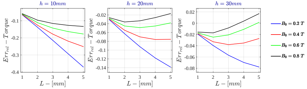
Figure H.13: Monodimensional LPM - Current Drive Relative Error - \dot{\Gamma} for \sigma = 10^4 \text{ S/m} - r_{out} = 50\text{mm}
