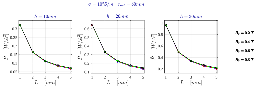
Figure B.3: Current Drive - Specific Power for \sigma = 10^2 \text{ S/m} - FDHM
