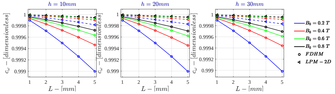
Figure 7.75: Bidimensional LPM c_w for \sigma = 10^6 S/m - r_{out} = 50\text{mm}
