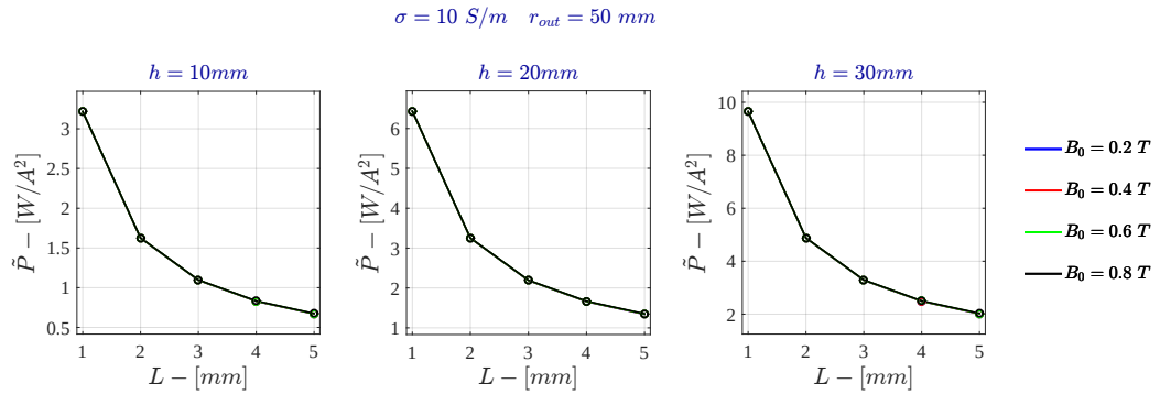
Figure 5.18: Voltage Drive - Specific Power for \sigma = 10 \text{ S/m} - FDHM
