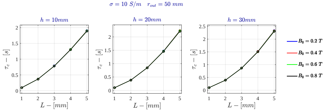
Figure 5.17: Voltage Drive - Characteristic time for \sigma = 10 \text{ S/m} - FDHM
