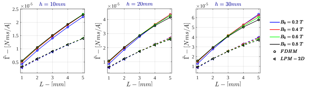
Figure 7.92: Bidimensional LPM - Voltage Drive \tilde{\Gamma} for \sigma = 10^6 S/m - r_{out} = 50 mm
