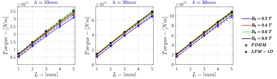
Figure 7.81: Bidimensional LPM - Current Drive \dot{\Gamma} for \sigma = 10^6 S/m - r_{out} = 50 mm
