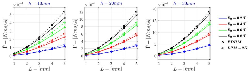
Figure 7.36: Bidimensional LPM - Current Drive \tilde{\Gamma} for \sigma = 10 \text{ S/m} - r_{out} = 50\text{mm}
