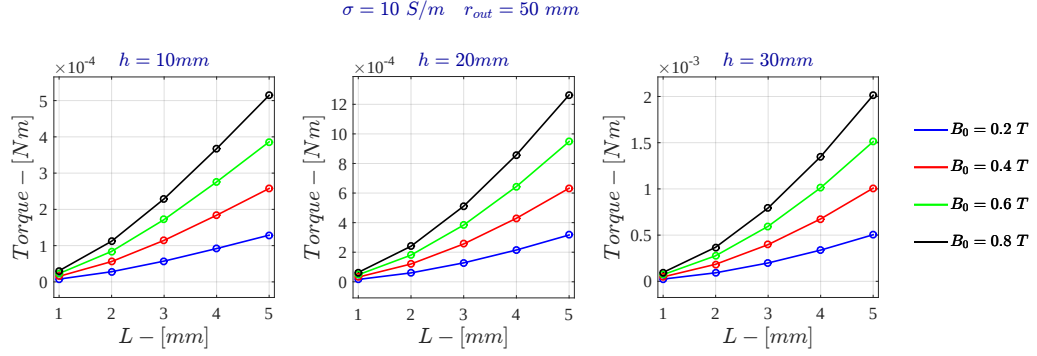
Figure 5.10: Current Drive - Torque for \sigma = 10 \text{ S/m} - FDHM
