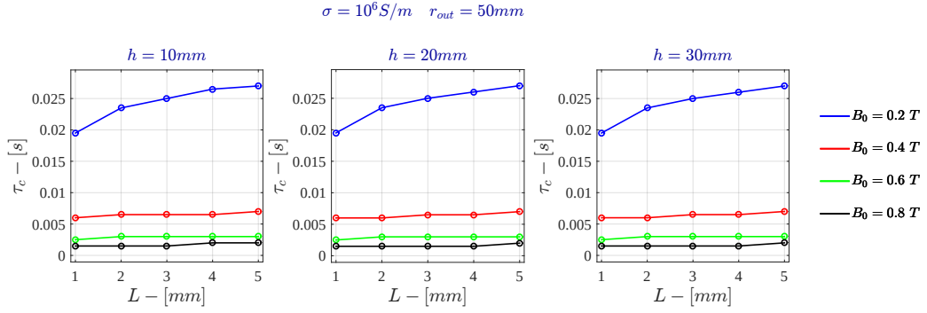
Figure 5.29: Voltage Drive - Characteristic time for \sigma = 10^6 \text{ S/m} - FDHM
