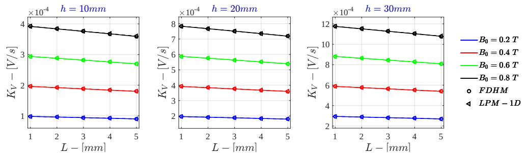
Figure H.4: Monodimensional LPM K_V for \sigma = 10^4 \text{ S/m} - r_{out} = 50 \text{ mm}
