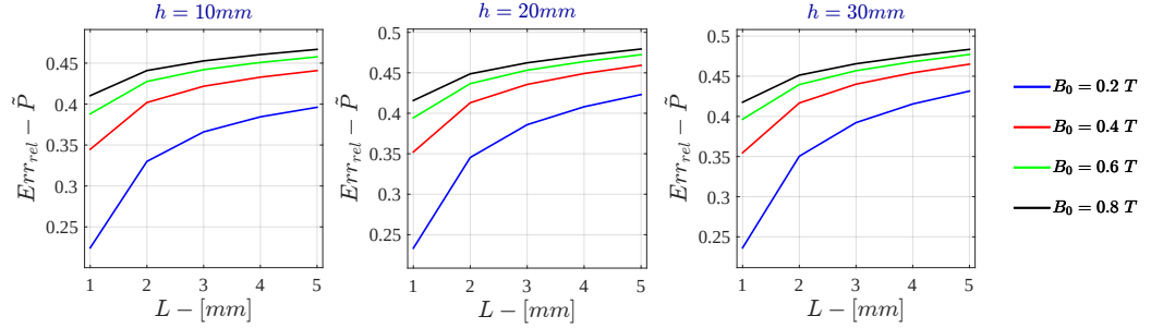
Figure 7.87: Bidimensional LPM - Current Drive Relative Error - \tilde{P} for \sigma = 10^6 S/m - r_{out} = 50 mm
