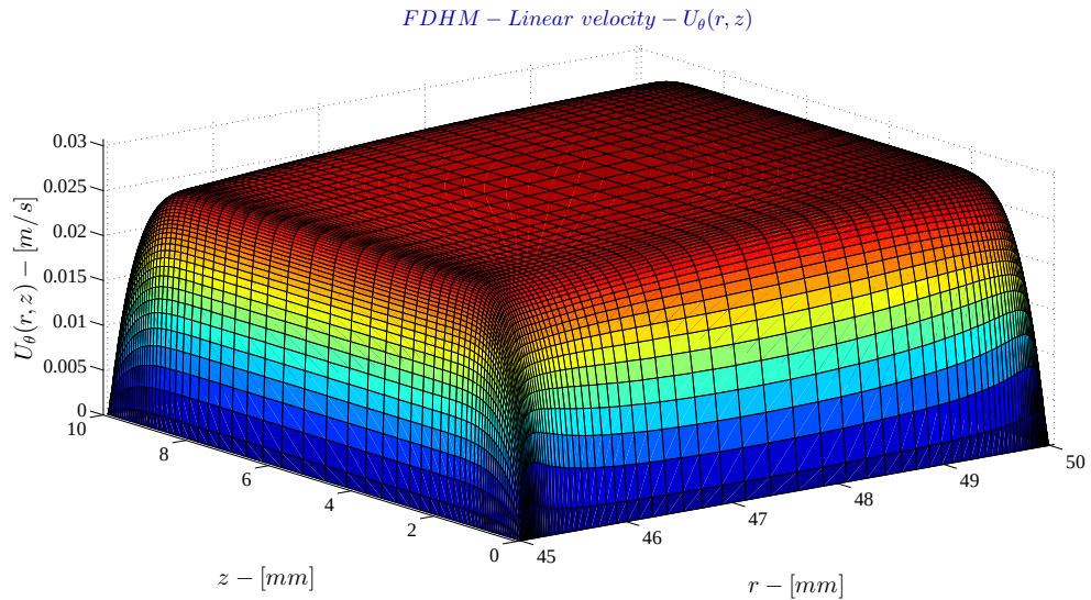
Figure 5.3: FDHM - Linear velocity
