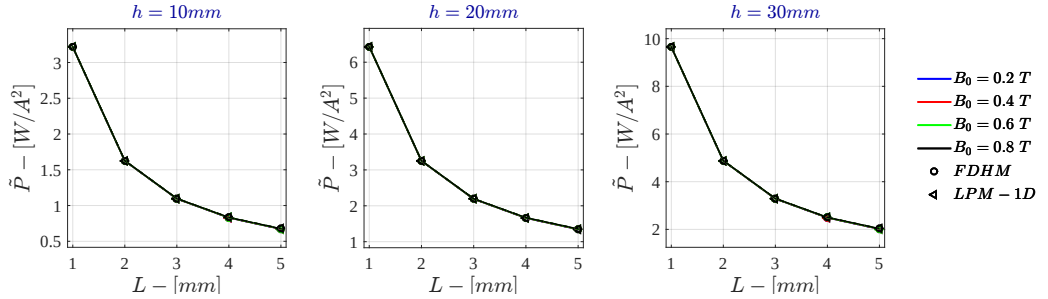
Figure 7.19: Monodimensional LPM - Voltage Drive \dot{P} for \sigma = 10 \text{ S/m} - r_{out} = 50 \text{ mm}
