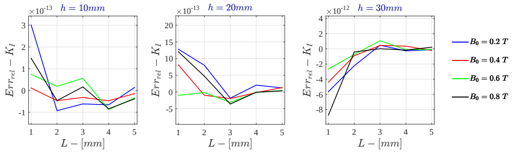
Figure F.6: Monodimensional LPM Relative Error - K_I for \sigma = 10^2 \text{ S/m} - r_{out} = 50\text{mm}
