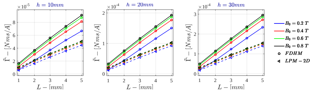
Figure I.36: Bidimensional LPM - Current Drive \tilde{\Gamma} for \sigma = 10^5 \text{ S/m} - r_{out} = 50 \text{ mm}
