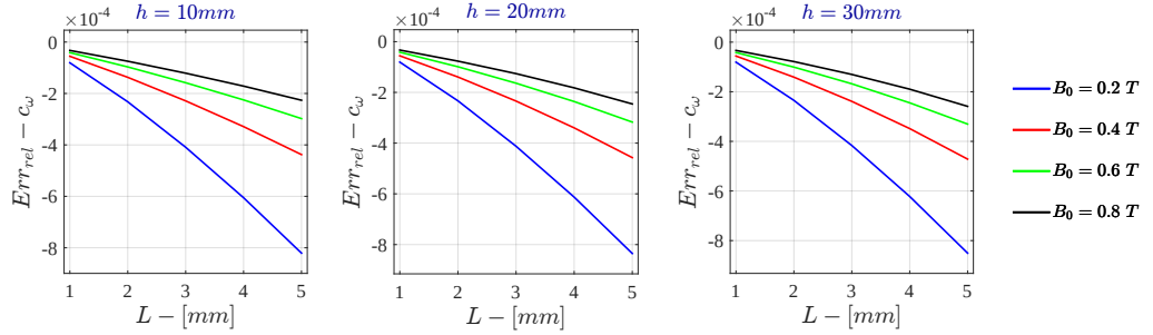
Figure 7.79: Bidimensional LPM Relative Error - c_\omega for \sigma = 10^6 S/m - r_{out} = 50 mm
