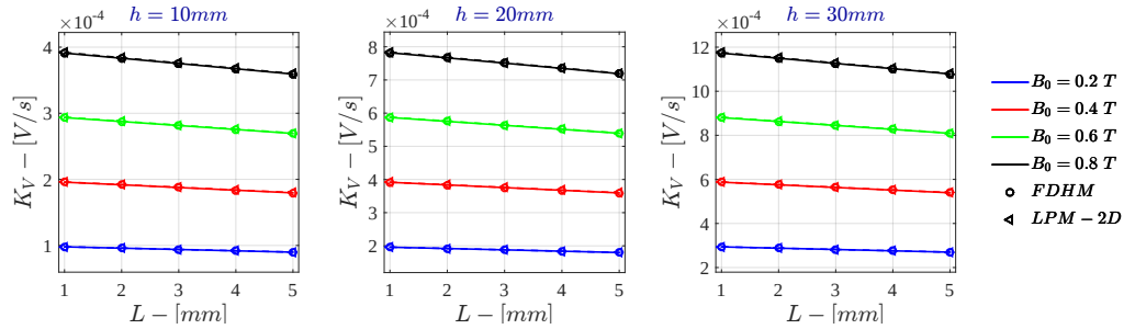
Figure I.28: Bidimensional LPM K_V for \sigma = 10^5 \text{ S/m} - r_{out} = 50\text{mm}
