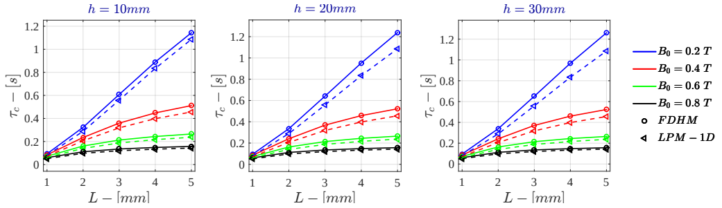
Figure H.18: Monodimensional LPM - Voltage Drive \tau_c for \sigma = 10^4 \text{ S/m} - r_{\text{out}} = 50\text{mm}
