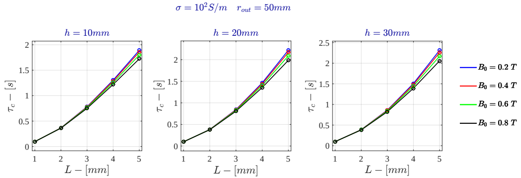
Figure B.8: Voltage Drive - Characteristic time for \sigma = 10^2 \text{ S/m} - FDHM
