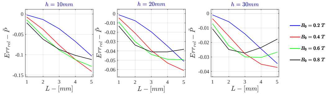
Figure H.23: Monodimensional LPM - Voltage Drive Relative Error - \tilde{P} for \sigma = 10^4 \text{ S/m} - r_{out} = 50\text{mm}
