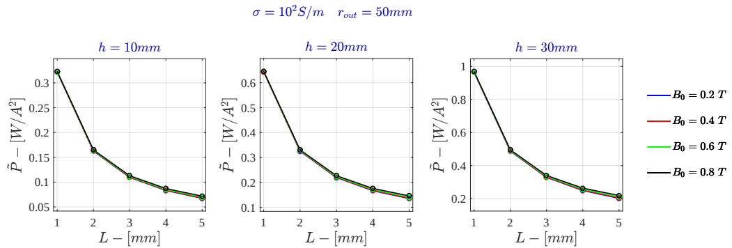
Figure B.9: Voltage Drive - Specific Power for \sigma = 10^2 \text{ S/m} - FDHM
