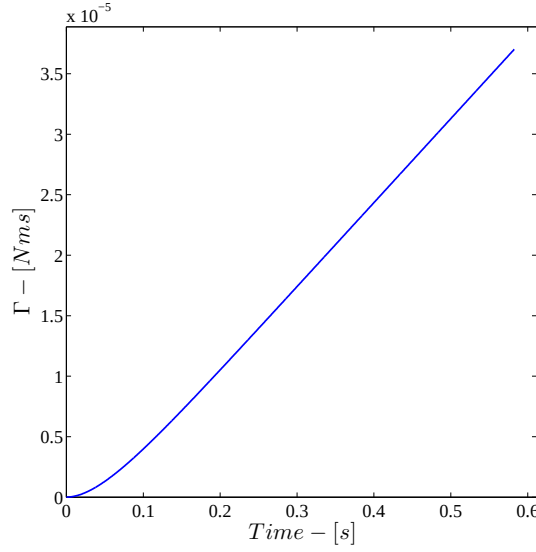
Figure 5.9: FDHM - Angular Momentum \Gamma
