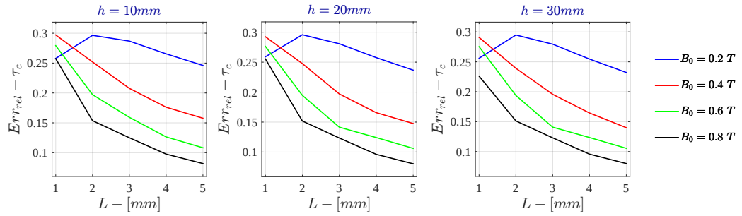
Figure I.46: Bidimensional LPM - Voltage Drive Relative Error - \tau_c for \sigma = 10^5 \text{ S/m} - r_{out} = 50\text{mm}
