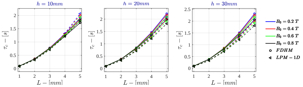
Figure F.18: Monodimensional LPM - Voltage Drive \tau_c for \sigma = 10^2 \text{ S/m} - r_{out} = 50\text{mm}
