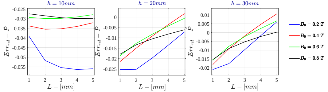
Figure 7.71: Monodimensional LPM - Voltage Drive Relative Error - \tilde{P} for \sigma = 10^6 S/m - r_{out} = 50 mm
