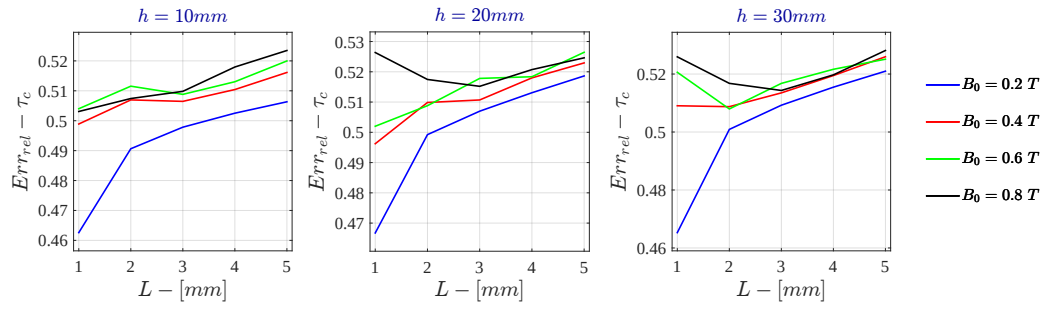
Figure 7.86: Bidimensional LPM - Current Drive Relative Error - \tau_c for \sigma = 10^6 S/m - r_{out} = 50 mm
