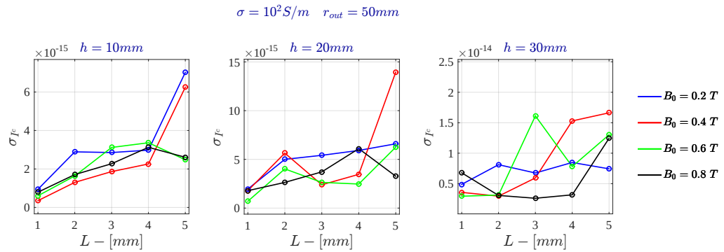
Figure B.12: Voltage Drive - Standard deviation of the electric current for \sigma = 10^2 \text{ S/m} - FDHM
