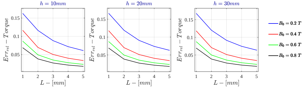
Figure 7.93: Bidimensional LPM - Voltage Drive Relative Error - \dot{\Gamma} for \sigma = 10^6 S/m - r_{out} = 50 mm
