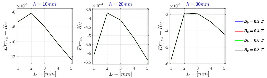
Figure 7.8: Monodimensional LPM Relative Error - K_V for \sigma = 10 S/m - r_{out} = 50 mm
