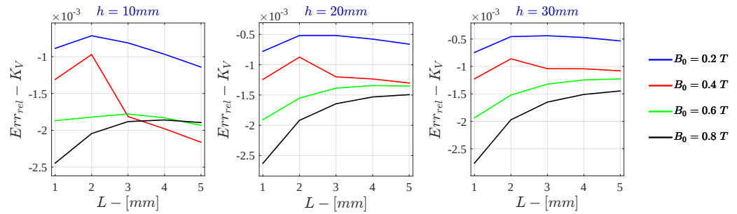
Figure I.8: Monodimensional LPM Relative Error - K_V for \sigma = 10^5 \text{ S/m} - r_{out} = 50 \text{ mm}
