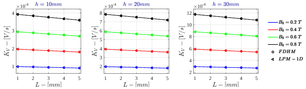
Figure G.4: Monodimensional LPM K_V for \sigma = 10^3 \text{ S/m} - r_{out} = 50\text{mm}
