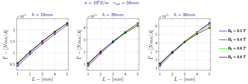
Figure 5.31: Voltage Drive - Specific Angular Momentum for \sigma = 10^6 \text{ S/m} - FDHM
