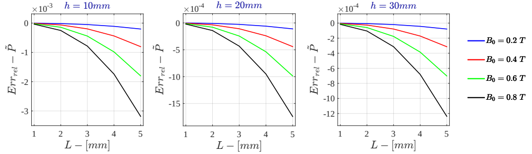
Figure 7.15: Monodimensional LPM - Current Drive Relative Error - \tilde{P} for \sigma = 10 \text{ S/m} - r_{out} = 50\text{mm}
