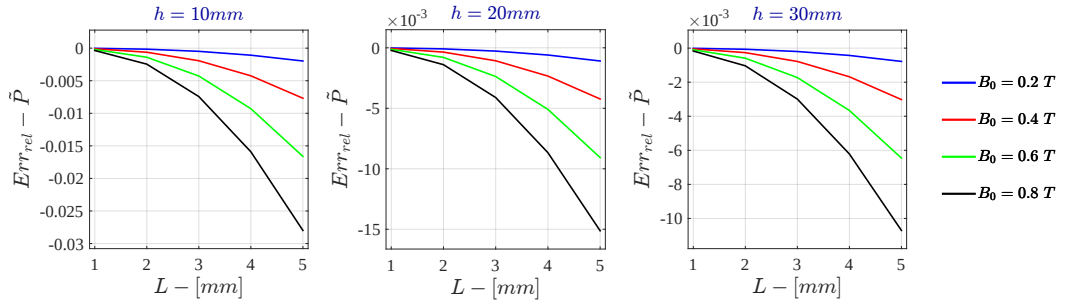
Figure F.23: Monodimensional LPM - Voltage Drive Relative Error - \tilde{P} for \sigma = 10^2 \text{ S/m} - r_{out} = 50\text{mm}
