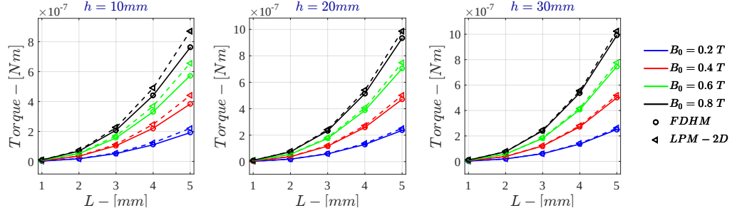
Figure 7.41: Bidimensional LPM - Voltage Drive \dot{\Gamma} for \sigma = 10 S/m - r_{out} = 50 mm
