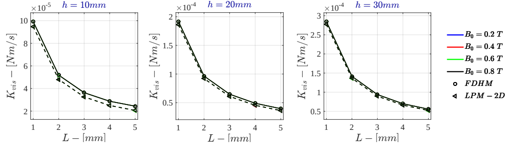
Figure 7.25: Bidimensional LPM K_{vis} for \sigma = 10 S/m - r_{out} = 50mm
