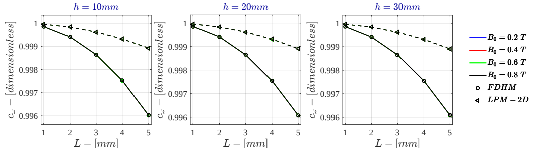
Figure 7.27: Bidimensional LPM c_\omega for \sigma = 10 S/m - r_{out} = 50mm
