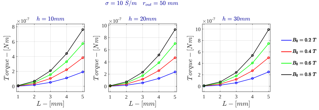
Figure 5.16: Voltage Drive - Torque for \sigma = 10 \text{ S/m} - FDHM
