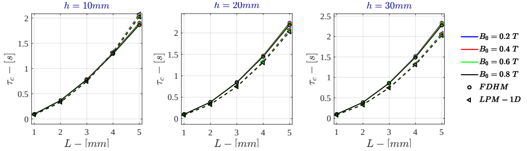
Figure F.10: Monodimensional LPM - Current Drive \tau_c for \sigma = 10^2 \text{ S/m} - r_{out} = 50\text{mm}
