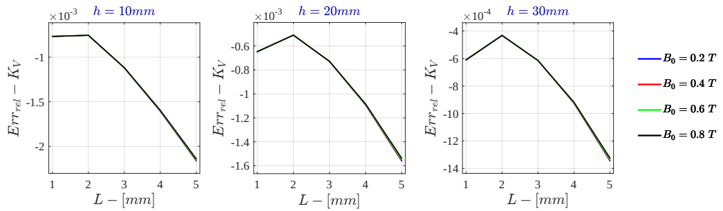
Figure G.32: Bidimensional LPM Relative Error - K_V for \sigma = 10^3 \text{ S/m} - r_{out} = 50\text{mm}
