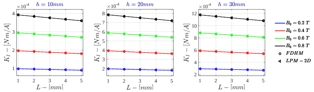
Figure H.26: Bidimensional LPM K_I for \sigma = 10^4 \text{ S/m} - r_{out} = 50\text{mm}
