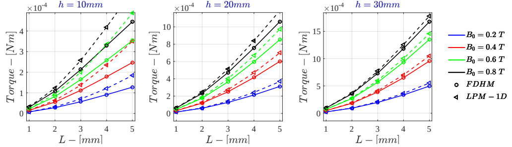
Figure G.33: Bidimensional LPM - Current Drive \dot{\Gamma} for \sigma = 10^3 \text{ S/m} - r_{out} = 50\text{mm}
