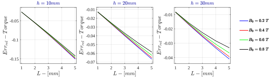
Figure 7.45: Bidimensional LPM - Voltage Drive Relative Error - \dot{\Gamma} for \sigma = 10 \text{ S/m} - r_{out} = 50\text{mm}
