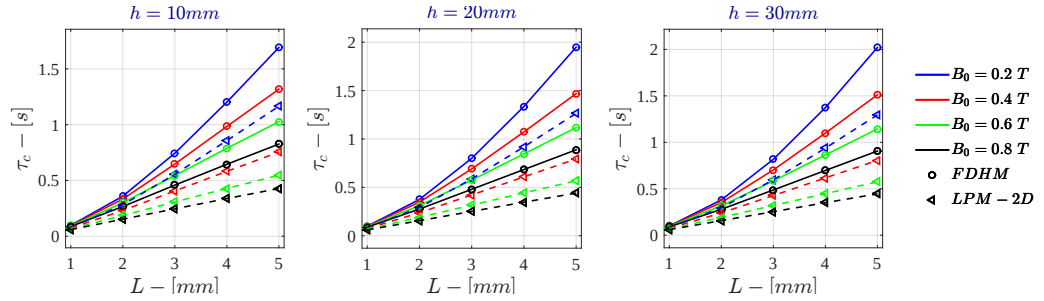
Figure H.34: Bidimensional LPM - Current Drive \tau_c for \sigma = 10^4 \text{ S/m} - r_{out} = 50\text{mm}
