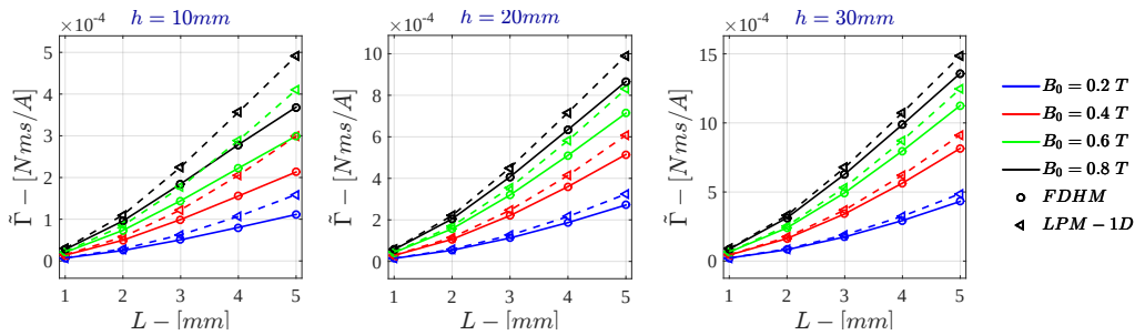
Figure G.20: Monodimensional LPM - Voltage Drive \tilde{\Gamma} for \sigma = 10^3 \text{ S/m} - r_{out} = 50 \text{ mm}
