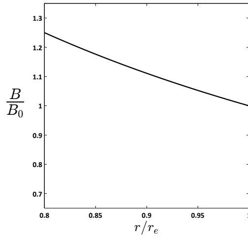
Figure 6.3: Magnetic Field Density \mathbf{B} normalized with respect of the Magnetic Field Density B_0 at the outer radius.
