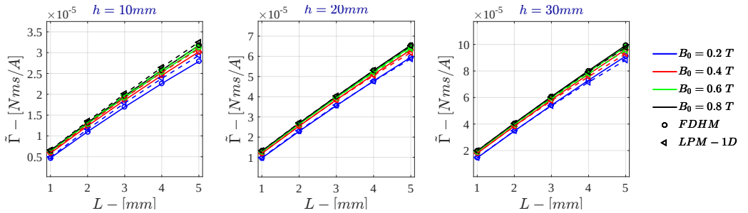
Figure 7.60: Monodimensional LPM - Current Drive \tilde{\Gamma} for \sigma = 10^6 \text{ S/m} - r_{out} = 50\text{mm}
