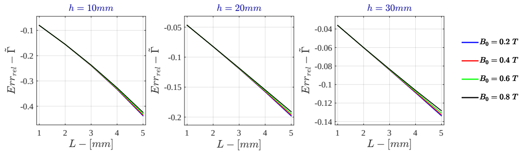
Figure F.24: Monodimensional LPM - Voltage Drive Relative Error - \tilde{I} for \sigma = 10^2 \text{ S/m} - r_{out} = 50\text{mm}
