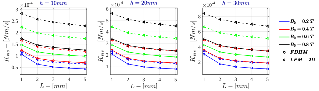
Figure I.25: Bidimensional LPM K_{vis} for \sigma = 10^5 \text{ S/m} - r_{out} = 50\text{mm}
