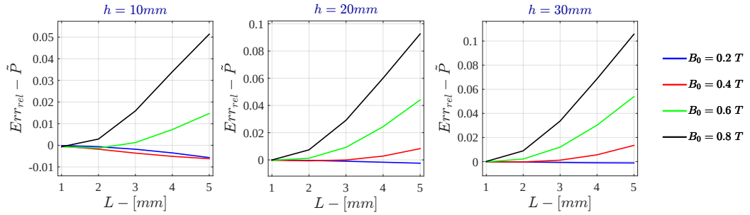
Figure G.39: Bidimensional LPM - Current Drive Relative Error - \tilde{P} for \sigma = 10^3 \text{ S/m} - r_{out} = 50\text{mm}
