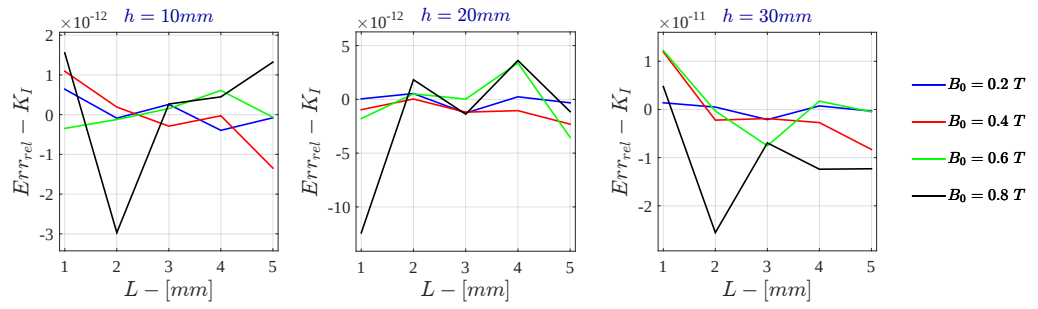
Figure I.6: Monodimensional LPM Relative Error - K_I for \sigma = 10^5 \text{ S/m} - r_{out} = 50 \text{ mm}
