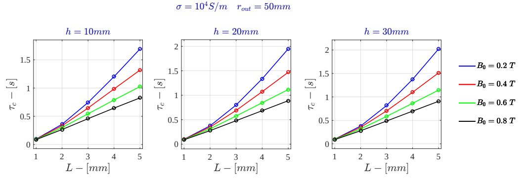
Figure D.2: Current Drive - Characteristic time for \sigma = 10^4 \text{ S/m} - FDHM
