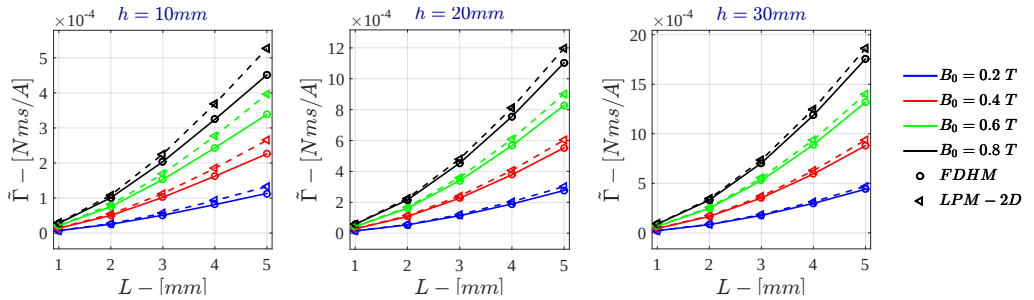
Figure 7.44: Bidimensional LPM - Voltage Drive \tilde{\Gamma} for \sigma = 10 S/m - r_{out} = 50 mm
