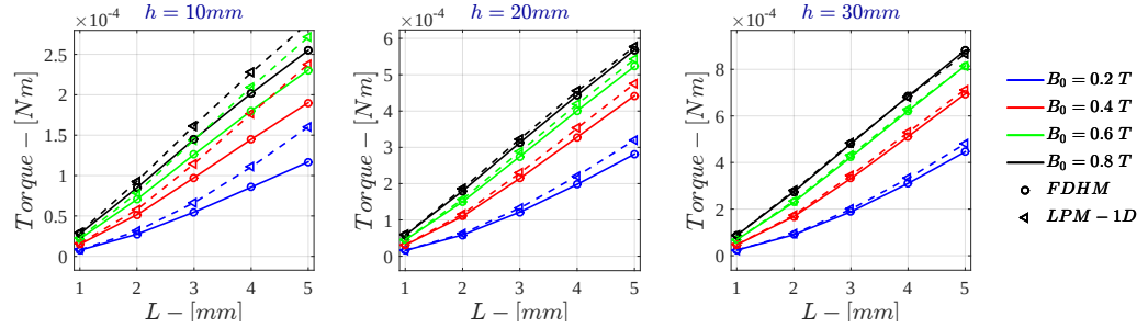
Figure H.9: Monodimensional LPM - Current Drive \dot{\Gamma} for \sigma = 10^4 \text{ S/m} - r_{out} = 50 \text{ mm}
