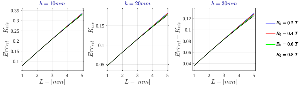
Figure F.5: Monodimensional LPM Relative Error - K_{vis} for \sigma = 10^2 \text{ S/m} - r_{out} = 50\text{mm}
