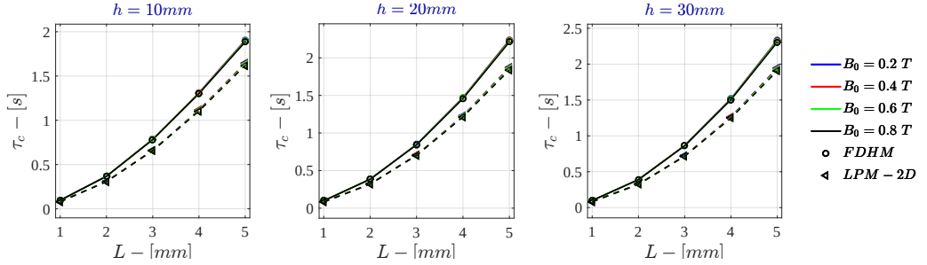
Figure 7.42: Bidimensional LPM - Voltage Drive \tau_c for \sigma = 10 S/m - r_{out} = 50 mm
