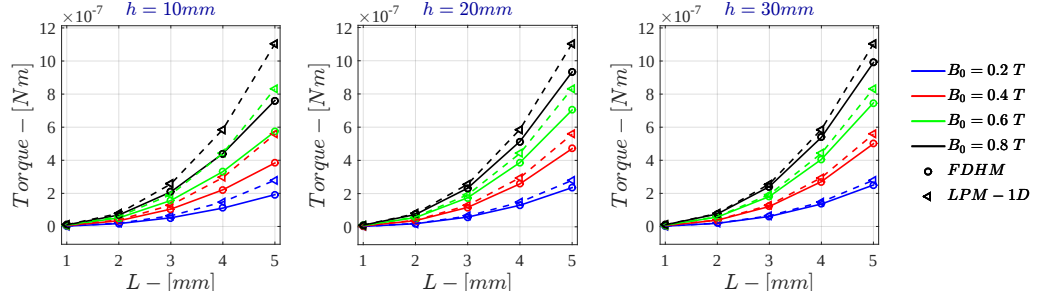
Figure 7.17: Monodimensional LPM - Voltage Drive \dot{\Gamma} for \sigma = 10 \text{ S/m} - r_{out} = 50 \text{ mm}
