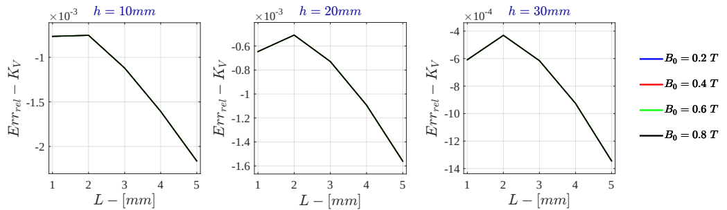
Figure 7.32: Bidimensional LPM Relative Error - K_V for \sigma = 10 S/m - r_{out} = 50 mm
