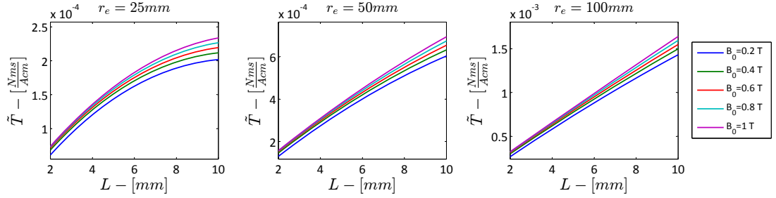
Figure 8.3: Torque function of L for B_0 = 0.2 \div 1.0 and 3 different outer radii r_e = 25, 50, 100\text{mm} . Liquid: Mercury (Hg).
