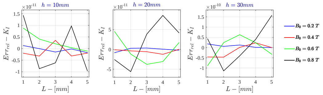
Figure 7.78: Bidimensional LPM Relative Error - K_I for \sigma = 10^6 S/m - r_{out} = 50 mm
