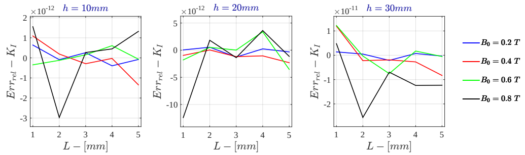
Figure I.30: Bidimensional LPM Relative Error - K_I for \sigma = 10^5 \text{ S/m} - r_{out} = 50\text{mm}
