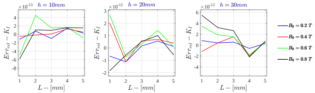
Figure H.30: Bidimensional LPM Relative Error - K_I for \sigma = 10^4 \text{ S/m} - r_{out} = 50\text{mm}
