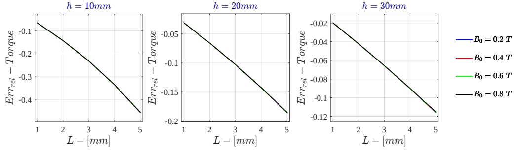
Figure 7.13: Monodimensional LPM - Current Drive Relative Error - \dot{\Gamma} for \sigma = 10 \text{ S/m} - r_{out} = 50\text{mm}
