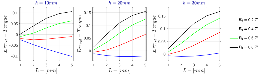
Figure G.45: Bidimensional LPM - Voltage Drive Relative Error - \dot{\Gamma} for \sigma = 10^3 \text{ S/m} - r_{out} = 50\text{mm}
