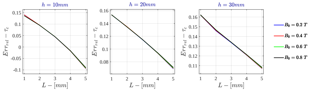
Figure 7.22: Monodimensional LPM - Voltage Drive Relative Error - \tau_c for \sigma = 10 \text{ S/m} - r_{out} = 50\text{mm}
