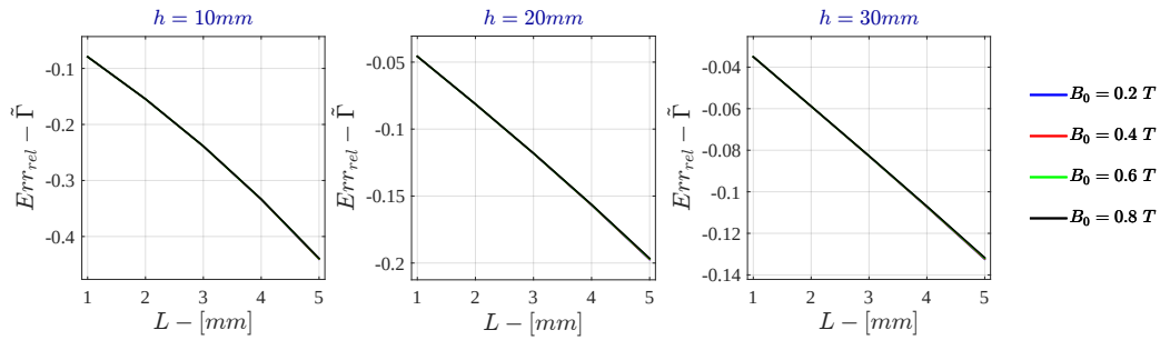
Figure 7.16: Monodimensional LPM - Current Drive Relative Error - \tilde{I} for \sigma = 10 \text{ S/m} - r_{out} = 50\text{mm}
