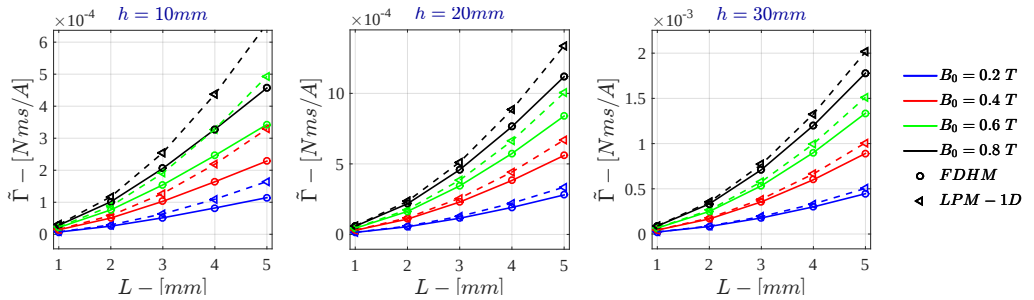
Figure 7.12: Monodimensional LPM - Current Drive \tilde{\Gamma} for \sigma = 10 \text{ S/m} - r_{out} = 50 \text{ mm}
