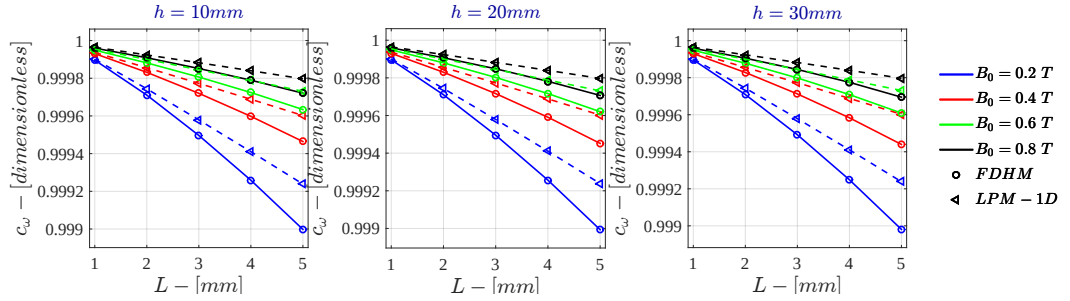
Figure 7.51: Monodimensional LPM c_\omega for \sigma = 10^6 S/m - r_{out} = 50mm
