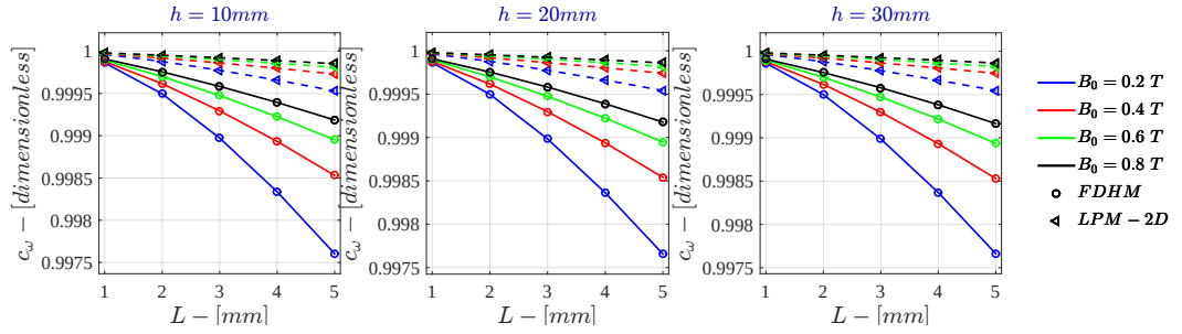
Figure I.27: Bidimensional LPM c_\omega for \sigma = 10^5 \text{ S/m} - r_{out} = 50\text{mm}
