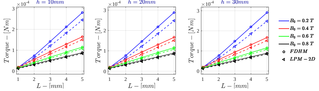
Figure I.41: Bidimensional LPM - Voltage Drive \dot{\Gamma} for \sigma = 10^5 \text{ S/m} - r_{out} = 50 \text{ mm}
