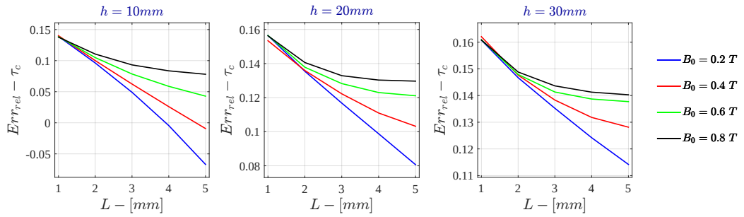
Figure G.22: Monodimensional LPM - Voltage Drive Relative Error - \tau_c for \sigma = 10^3 \text{ S/m} - r_{out} = 50\text{mm}
