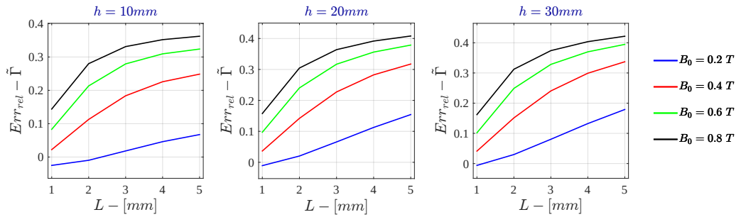
Figure H.40: Bidimensional LPM - Current Drive Relative Error - \tilde{\Gamma} for \sigma = 10^4 \text{ S/m} - r_{out} = 50\text{mm}
