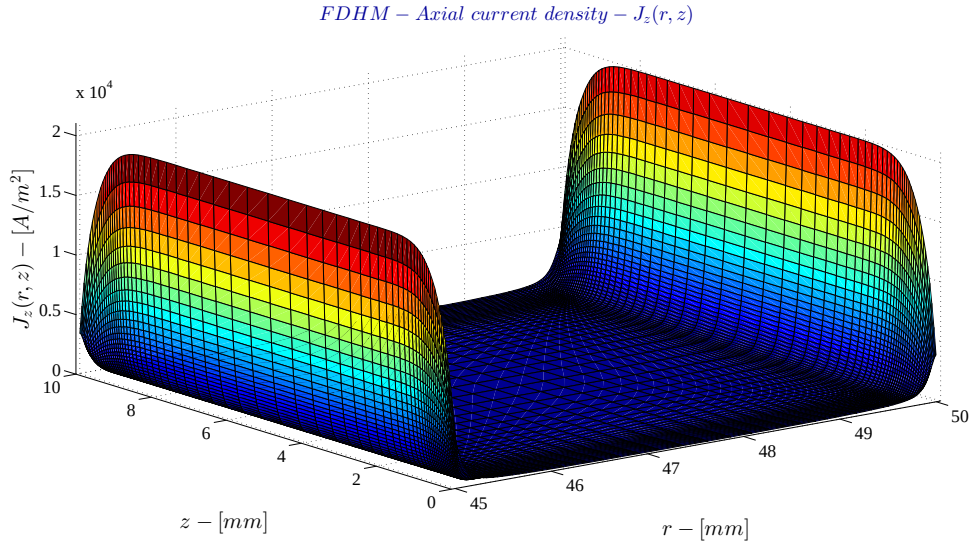
Figure 5.1: FDHM - Axial electric current density
