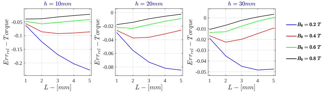
Figure H.21: Monodimensional LPM - Voltage Drive Relative Error - \dot{\Gamma} for \sigma = 10^4 \text{ S/m} - r_{out} = 50\text{mm}
