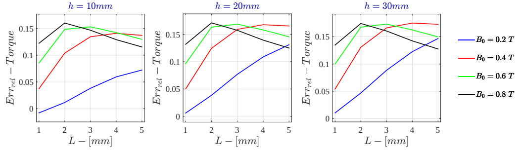
Figure H.45: Bidimensional LPM - Voltage Drive Relative Error - \dot{\Gamma} for \sigma = 10^4 \text{ S/m} - r_{out} = 50\text{mm}
