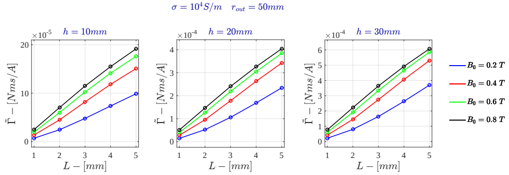
Figure D.10: Voltage Drive - Specific Angular Momentum for \sigma = 10^4 \text{ S/m} - FDHM
