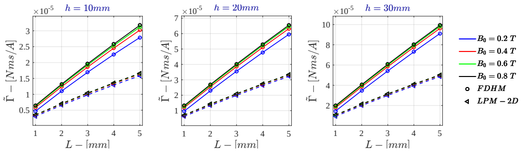
Figure 7.84: Bidimensional LPM - Current Drive \tilde{\Gamma} for \sigma = 10^6 S/m - r_{out} = 50 mm
