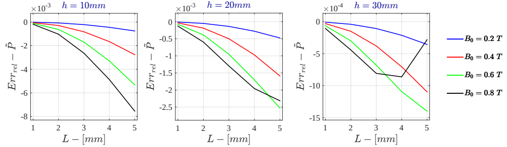
Figure F.47: Bidimensional LPM - Voltage Drive Relative Error - \tilde{P} for \sigma = 10^2 \text{ S/m} - r_{out} = 50\text{mm}
