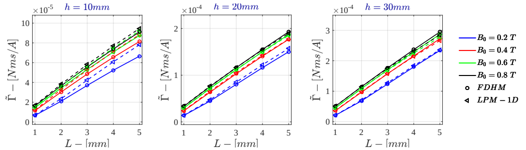
Figure I.12: Monodimensional LPM - Current Drive \tilde{\Gamma} for \sigma = 10^5 \text{ S/m} - r_{out} = 50\text{mm}
