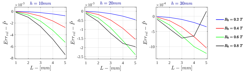
Figure F.39: Bidimensional LPM - Current Drive Relative Error - \tilde{P} for \sigma = 10^2 \text{ S/m} - r_{out} = 50\text{mm}
