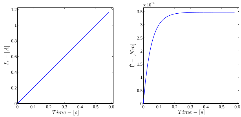
Figure 5.5: FDHM - Torque
