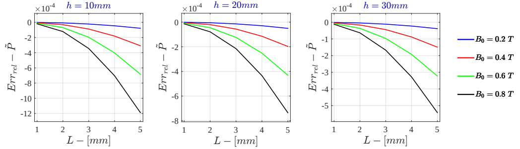
Figure 7.47: Bidimensional LPM - Voltage Drive Relative Error - \tilde{P} for \sigma = 10 \text{ S/m} - r_{out} = 50\text{mm}
