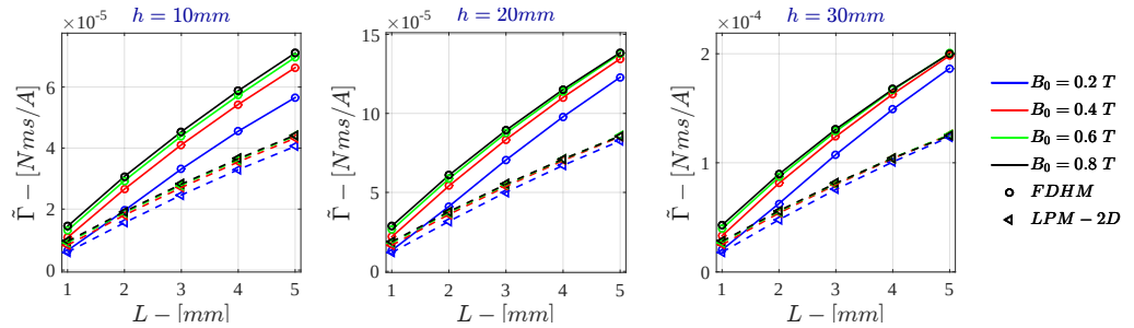
Figure I.44: Bidimensional LPM - Voltage Drive \tilde{\Gamma} for \sigma = 10^5 \text{ S/m} - r_{out} = 50 \text{ mm}
