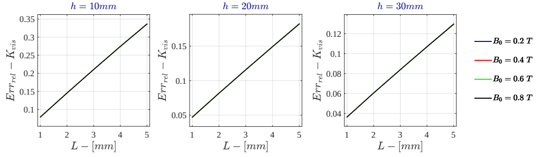
Figure 7.5: Monodimensional LPM Relative Error - K_{vis} for \sigma = 10 S/m - r_{out} = 50 mm
