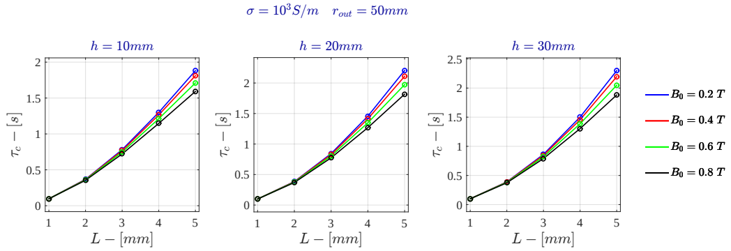
Figure C.2: Current Drive - Characteristic time for \sigma = 10^3 \text{ S/m} - FDHM
