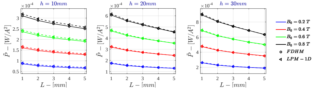
Figure 7.67: Monodimensional LPM - Voltage Drive \dot{P} for \sigma = 10^6 S/m - r_{out} = 50 mm
