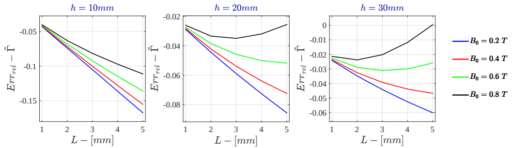
Figure F.40: Bidimensional LPM - Current Drive Relative Error - \tilde{I} for \sigma = 10^2 \text{ S/m} - r_{out} = 50\text{mm}
