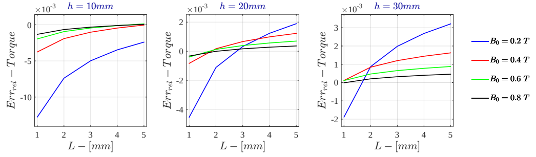
Figure 7.69: Monodimensional LPM - Voltage Drive Relative Error - \dot{\Gamma} for \sigma = 10^6 S/m - r_{out} = 50 mm
