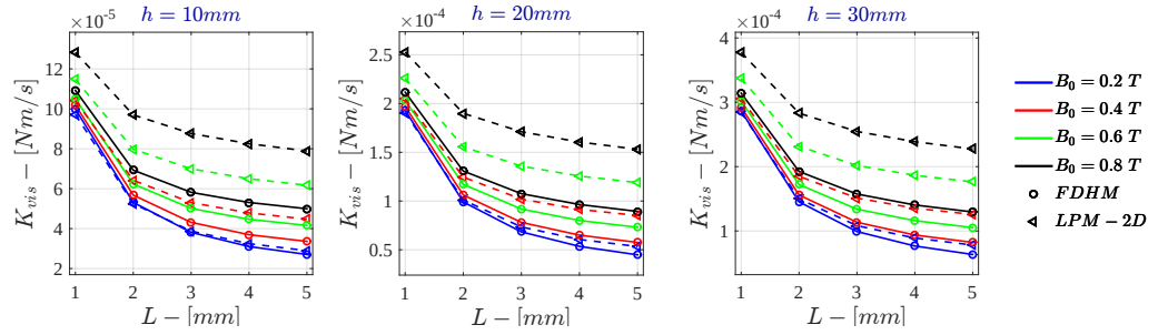
Figure H.25: Bidimensional LPM K_{vis} for \sigma = 10^4 \text{ S/m} - r_{out} = 50\text{mm}
