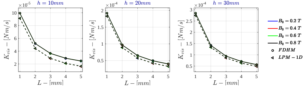
Figure F.1: K_{vis} for \sigma = 10^2 \text{ S/m} - r_{out} = 50 \text{ mm} - Monodimensional LPM
