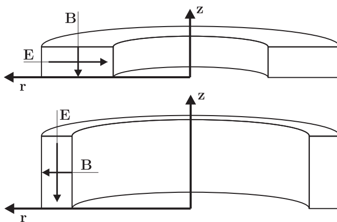
Figure 2.2: First (top) and second configuration (bottom) for electric field E and magnetic field B
