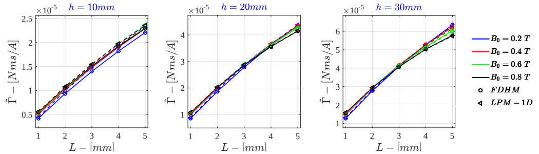
Figure 7.68: Monodimensional LPM - Voltage Drive \tilde{\Gamma} for \sigma = 10^6 S/m - r_{out} = 50 mm
