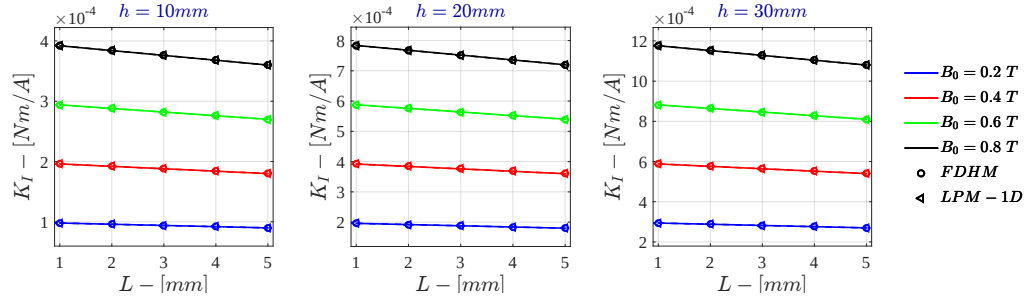
Figure G.2: Monodimensional LPM K_I for \sigma = 10^3 \text{ S/m} - r_{out} = 50\text{mm}
