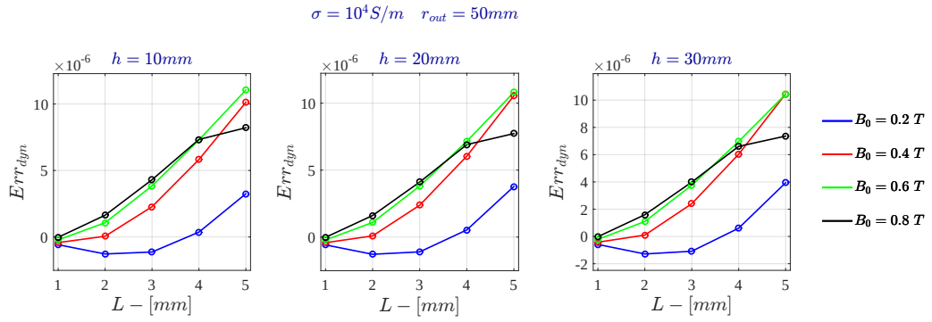
Figure D.11: Voltage Drive - Relative Dynamic Error for \sigma = 10^4 \text{ S/m} - FDHM
