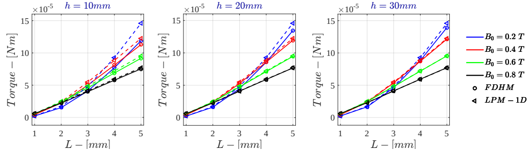
Figure H.17: Monodimensional LPM - Voltage Drive \dot{\Gamma} for \sigma = 10^4 \text{ S/m} - r_{\text{out}} = 50\text{mm}
