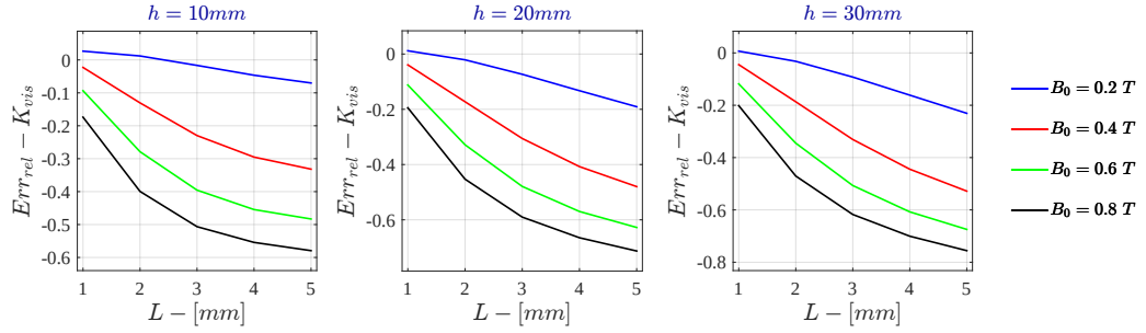
Figure H.29: Bidimensional LPM Relative Error - K_{vis} for \sigma = 10^4 \text{ S/m} - r_{out} = 50\text{mm}
