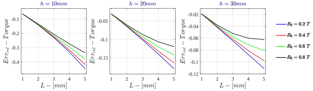
Figure G.13: Monodimensional LPM - Current Drive Relative Error - \dot{\Gamma} for \sigma = 10^3 \text{ S/m} - r_{out} = 50\text{mm}
