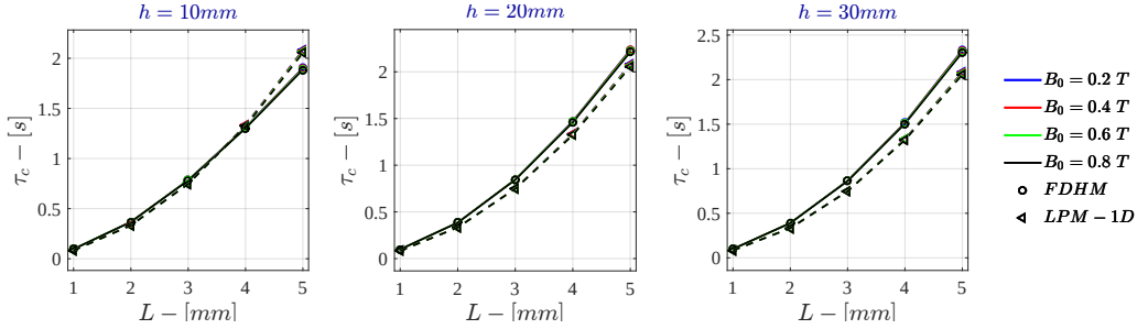
Figure 7.18: Monodimensional LPM - Voltage Drive \tau_c for \sigma = 10 \text{ S/m} - r_{out} = 50 \text{ mm}
