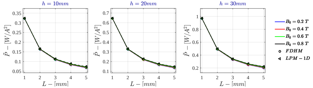
Figure F.35: Bidimensional LPM - Current Drive \dot{P} for \sigma = 10^2 \text{ S/m} - r_{\text{out}} = 50\text{mm}
