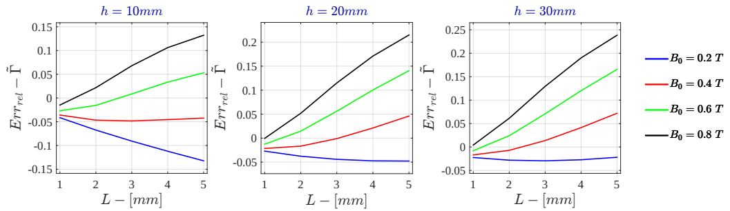
Figure G.40: Bidimensional LPM - Current Drive Relative Error - \tilde{I} for \sigma = 10^3 \text{ S/m} - r_{out} = 50\text{mm}
