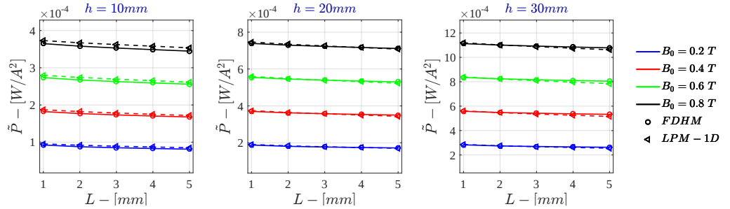
Figure 7.59: Monodimensional LPM - Current Drive \dot{P} for \sigma = 10^6 \text{ S/m} - r_{out} = 50\text{mm}
