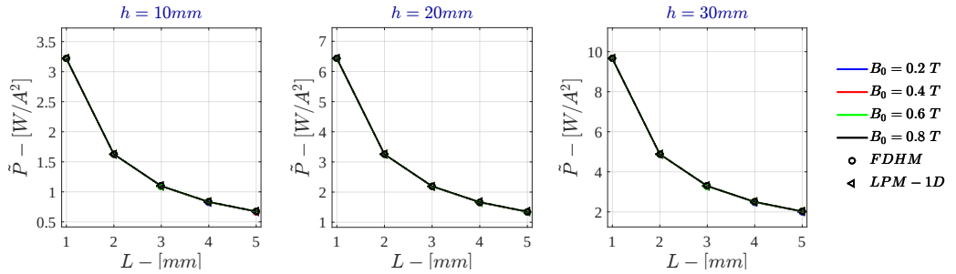
Figure 7.11: Monodimensional LPM - Current Drive \dot{P} for \sigma = 10 \text{ S/m} - r_{out} = 50 \text{ mm}
