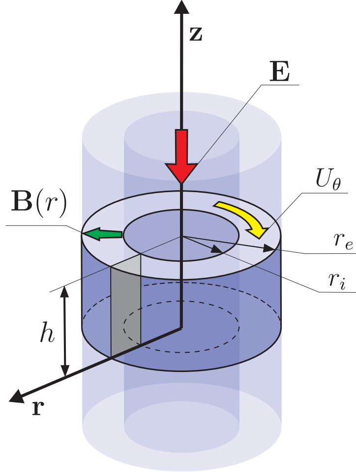
Figure 6.1: Section of an infinite annulus with applied electric field \mathbf{E} and radial magnetic field \mathbf{B}(r) .
