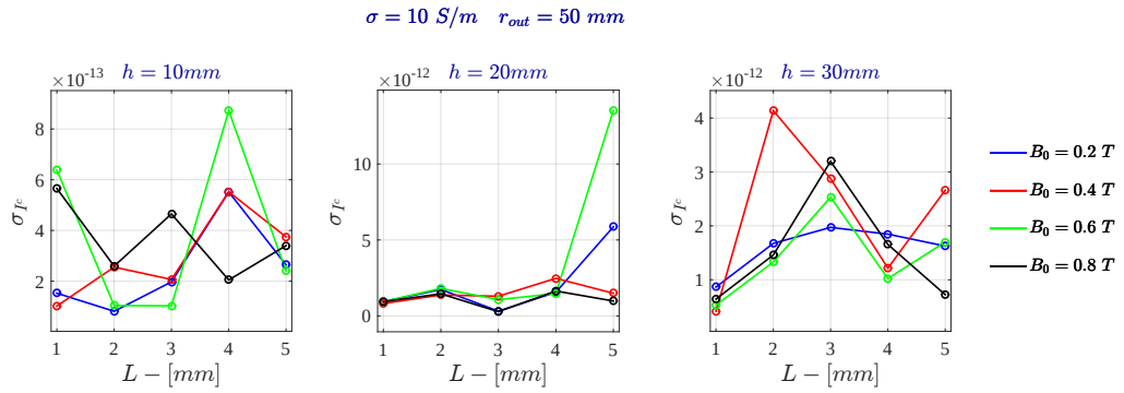
Figure 5.15: Current Drive - Standard deviation of the electric current for \sigma = 10 \text{ S/m} - FDHM
