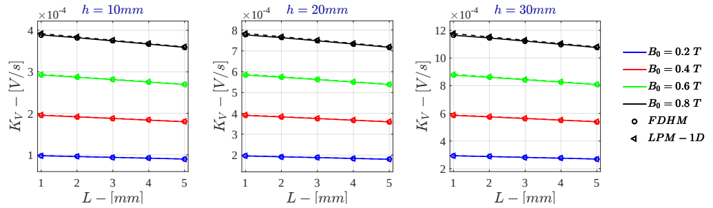
Figure 7.52: Monodimensional LPM K_V for \sigma = 10^6 S/m - r_{out} = 50mm
