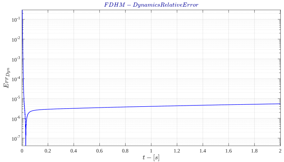
Figure 4.13: FDHM - Error of the dynamic side of the MHD problem
