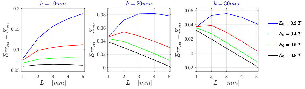
Figure I.5: Monodimensional LPM Relative Error - K_{vis} for \sigma = 10^5 \text{ S/m} - r_{out} = 50 \text{ mm}
