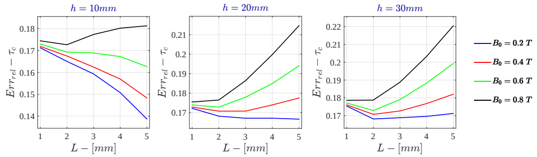
Figure I.38: Bidimensional LPM - Current Drive Relative Error - \tau_c for \sigma = 10^5 \text{ S/m} - r_{out} = 50\text{mm}
