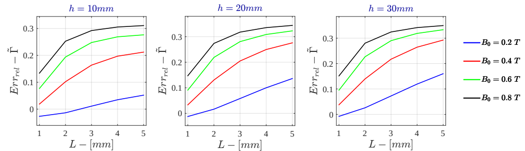
Figure H.48: Bidimensional LPM - Voltage Drive Relative Error - \tilde{I} for \sigma = 10^4 \text{ S/m} - r_{out} = 50\text{mm}
