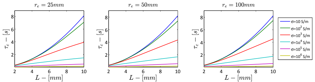
Figure 8.9: Characteristic time function of L for \sigma = 10 \div 10^6 S/m and 3 different outer radii r_e = 25, 50, 100mm . B_0 = 1.0 T . \rho = 1000 Kg/m^3 .
