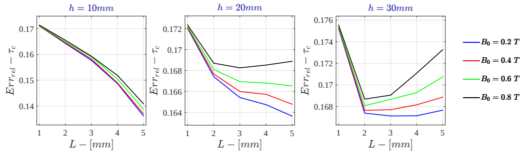
Figure 7.38: Bidimensional LPM - Current Drive Relative Error - \tau_c for \sigma = 10 \text{ S/m} - r_{out} = 50\text{mm}
