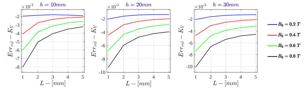
Figure 7.56: Monodimensional LPM Relative Error - K_V for \sigma = 10^6 S/m - r_{out} = 50 mm
