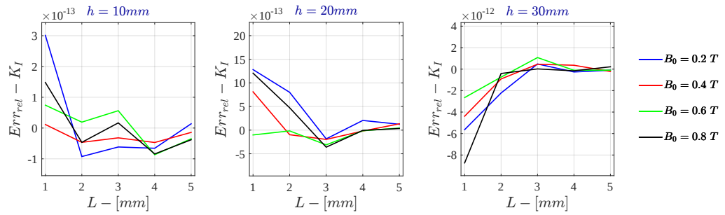
Figure F.30: Bidimensional LPM Relative Error - K_I for \sigma = 10^2 \text{ S/m} - r_{out} = 50\text{mm}
