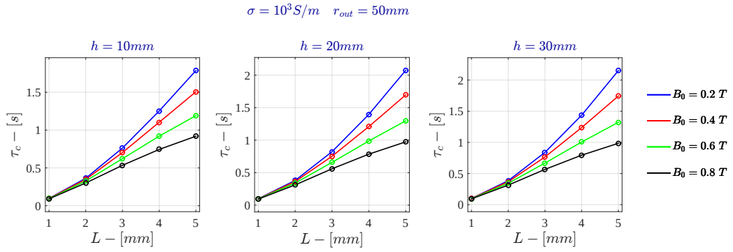
Figure C.8: Voltage Drive - Characteristic time for \sigma = 10^3 \text{ S/m} - FDHM
