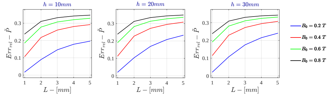
Figure I.47: Bidimensional LPM - Voltage Drive Relative Error - \tilde{P} for \sigma = 10^5 \text{ S/m} - r_{out} = 50\text{mm}
