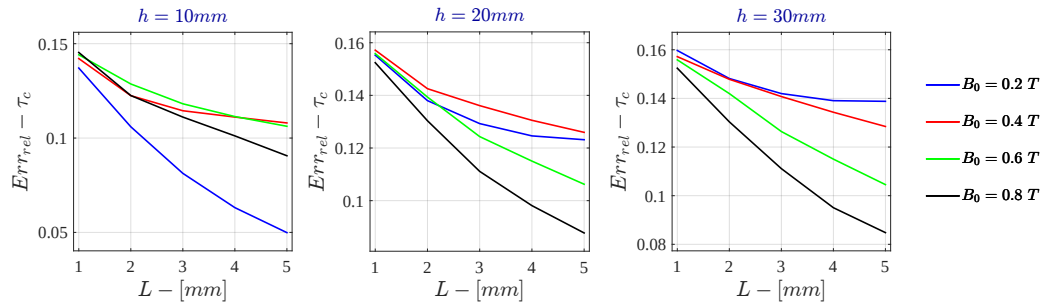
Figure H.22: Monodimensional LPM - Voltage Drive Relative Error - \tau_c for \sigma = 10^4 \text{ S/m} - r_{out} = 50\text{mm}
