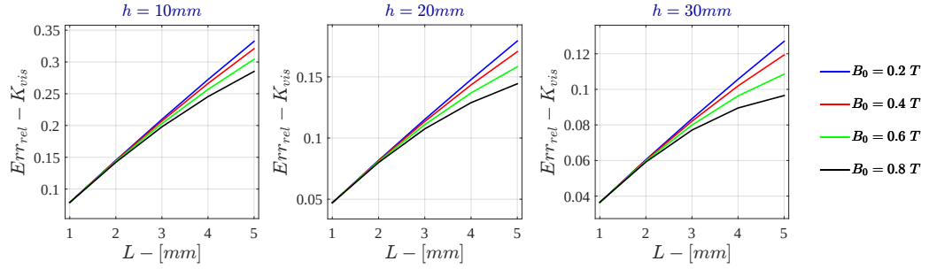
Figure G.5: Monodimensional LPM Relative Error - K_{vis} for \sigma = 10^3 \text{ S/m} - r_{out} = 50\text{mm}
