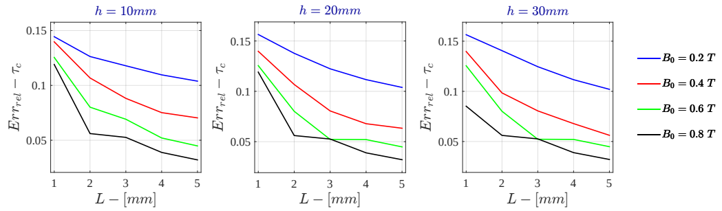
Figure I.22: Monodimensional LPM - Voltage Drive Relative Error - \tau_c for \sigma = 10^5 \text{ S/m} - r_{out} = 50\text{mm}
