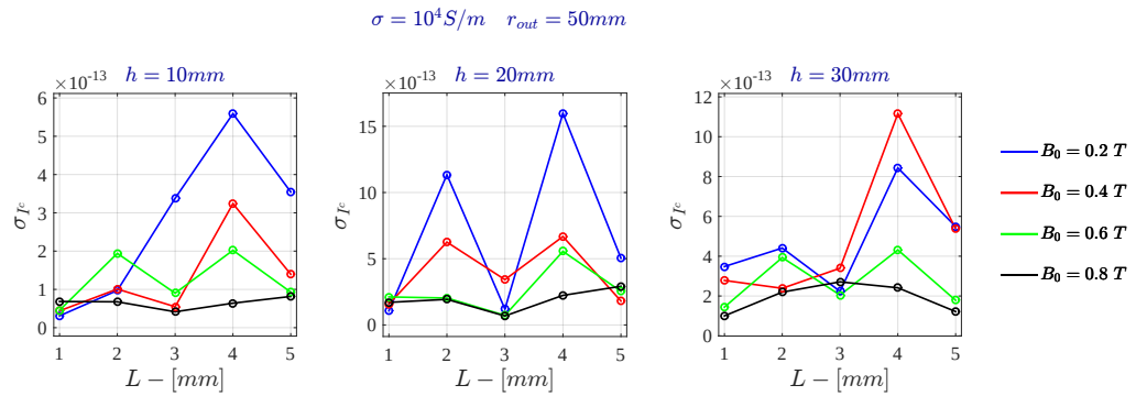
Figure D.12: Voltage Drive - Standard deviation of the electric current for \sigma = 10^4 \text{ S/m} - FDHM
