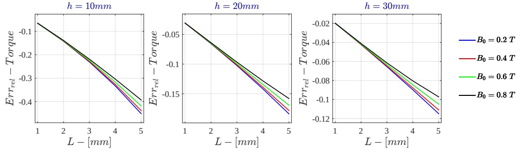
Figure F.21: Monodimensional LPM - Voltage Drive Relative Error - \dot{\Gamma} for \sigma = 10^2 \text{ S/m} - r_{out} = 50\text{mm}
