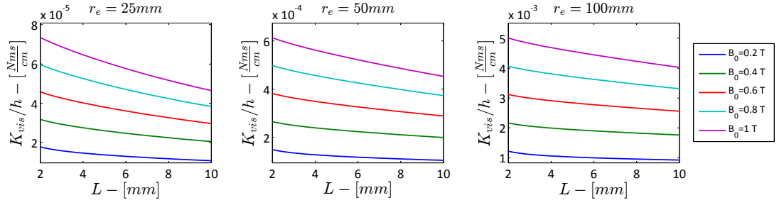
Figure 8.2: K_{vis} function of L for B_0 = 0.2 \div 1.0 and 3 different outer radii r_e = 25, 50, 100\text{mm} . Liquid: Mercury (Hg).
