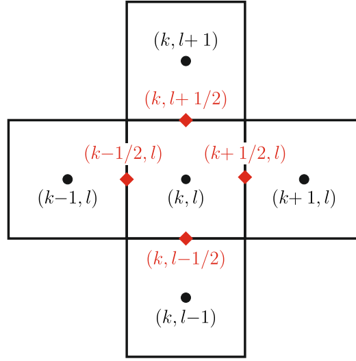
Figure 4.2: Finite Differences Model stencil.
