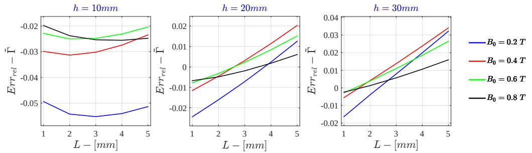
Figure 7.64: Monodimensional LPM - Current Drive Relative Error - \tilde{I} for \sigma = 10^6 S/m - r_{out} = 50mm
