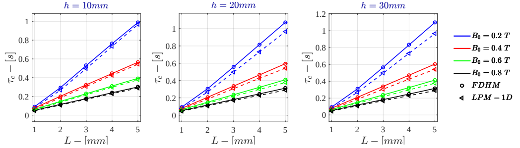
Figure I.10: Monodimensional LPM - Current Drive \tau_c for \sigma = 10^5 \text{ S/m} - r_{out} = 50\text{mm}
