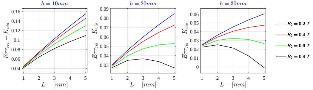
Figure F.29: Bidimensional LPM Relative Error - K_{vis} for \sigma = 10^2 \text{ S/m} - r_{out} = 50\text{mm}
