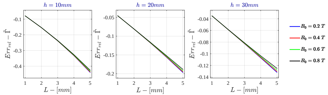
Figure F.16: Monodimensional LPM - Current Drive Relative Error - \tilde{I} for \sigma = 10^2 \text{ S/m} - r_{out} = 50\text{mm}
