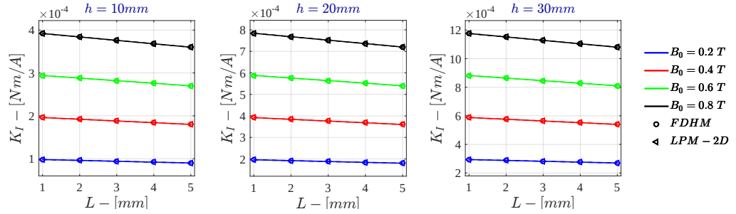
Figure F.26: Bidimensional LPM K_I for \sigma = 10^2 \text{ S/m} - r_{out} = 50 \text{ mm}
