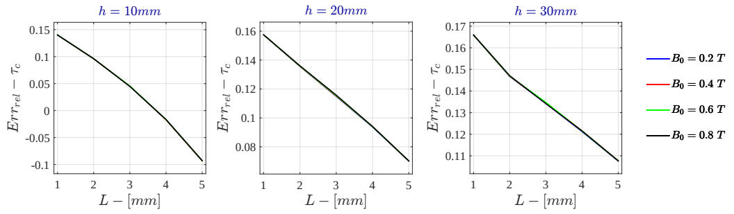
Figure 7.14: Monodimensional LPM - Current Drive Relative Error - \tau_c for \sigma = 10 \text{ S/m} - r_{out} = 50\text{mm}
