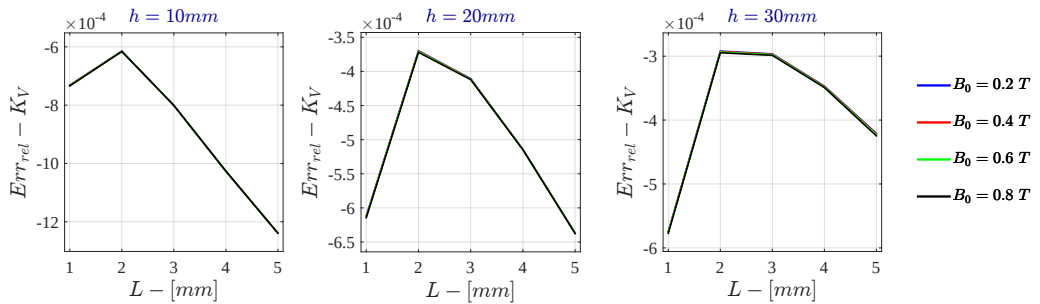
Figure F.8: Monodimensional LPM Relative Error - K_V for \sigma = 10^2 \text{ S/m} - r_{out} = 50\text{mm}
