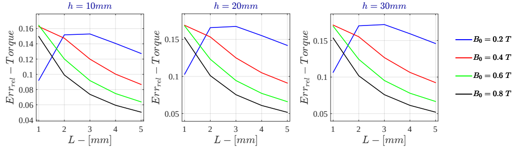
Figure I.45: Bidimensional LPM - Voltage Drive Relative Error - \dot{\Gamma} for \sigma = 10^5 \text{ S/m} - r_{out} = 50\text{mm}
