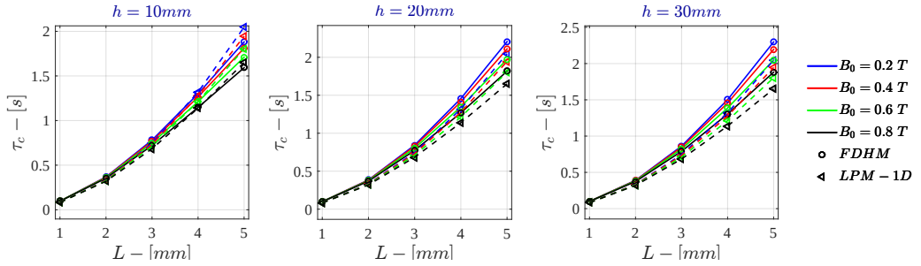
Figure G.10: Monodimensional LPM - Current Drive \tau_c for \sigma = 10^3 \text{ S/m} - r_{out} = 50\text{mm}
