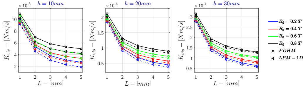
Figure H.1: K_{vis} for \sigma = 10^4 \text{ S/m} - r_{out} = 50 \text{ mm} - Monodimensional LPM
