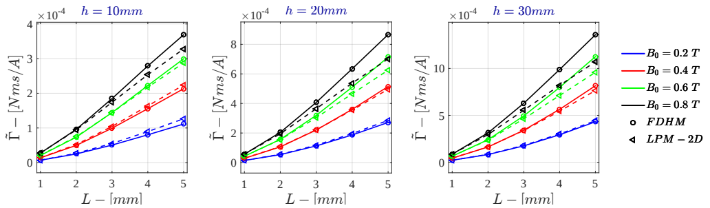
Figure G.44: Bidimensional LPM - Voltage Drive \tilde{\Gamma} for \sigma = 10^3 \text{ S/m} - r_{out} = 50\text{mm}
