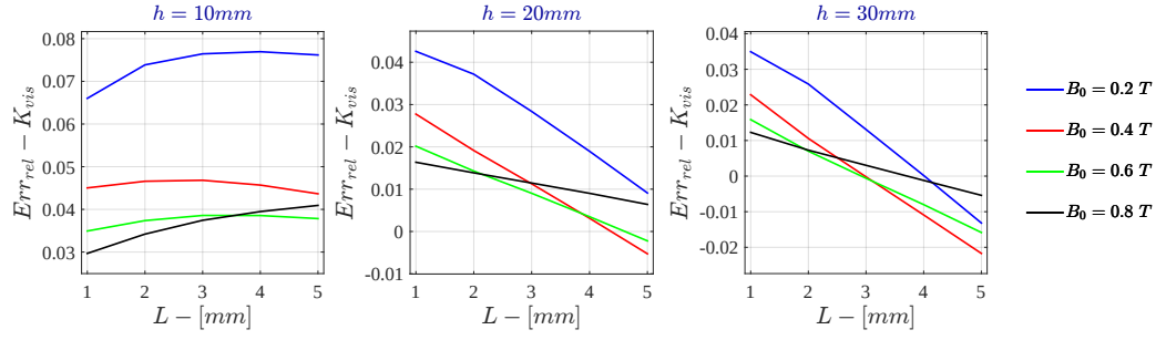
Figure 7.53: Monodimensional LPM Relative Error - K_{vis} for \sigma = 10^6 S/m - r_{out} = 50 mm
