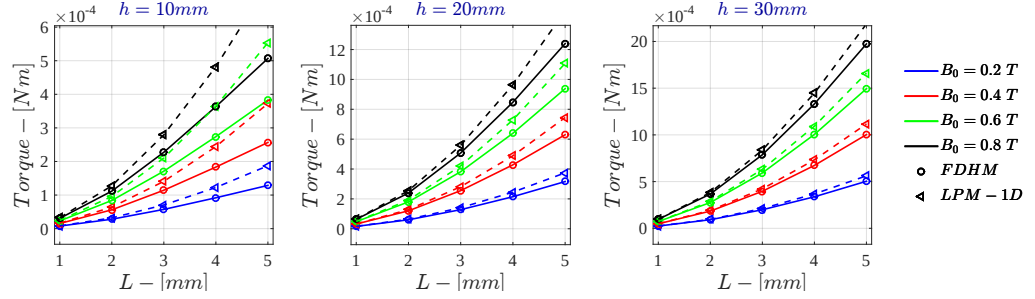
Figure F.9: Monodimensional LPM - Current Drive \dot{\Gamma} for \sigma = 10^2 \text{ S/m} - r_{out} = 50\text{mm}
