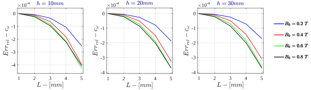
Figure H.7: Monodimensional LPM Relative Error - c_{\omega} for \sigma = 10^4 \text{ S/m} - r_{out} = 50\text{mm}
