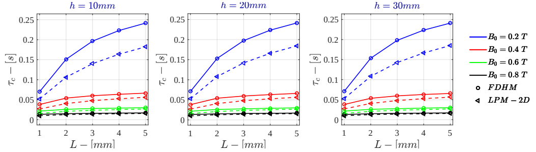
Figure I.42: Bidimensional LPM - Voltage Drive \tau_c for \sigma = 10^5 \text{ S/m} - r_{out} = 50 \text{ mm}
