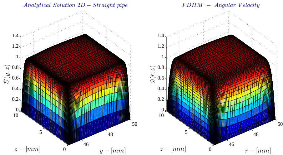
Figure 6.4: Comparison between MHD velocity field in a straight pipe under trasverse magnetic field and MHD angular velocity for an axially-symmetric torus under a radial magnetic field.
