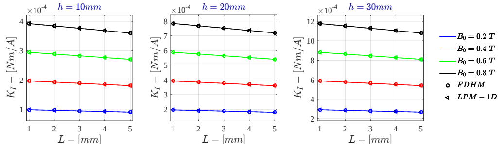
Figure H.2: Monodimensional LPM K_I for \sigma = 10^4 \text{ S/m} - r_{out} = 50 \text{ mm}
