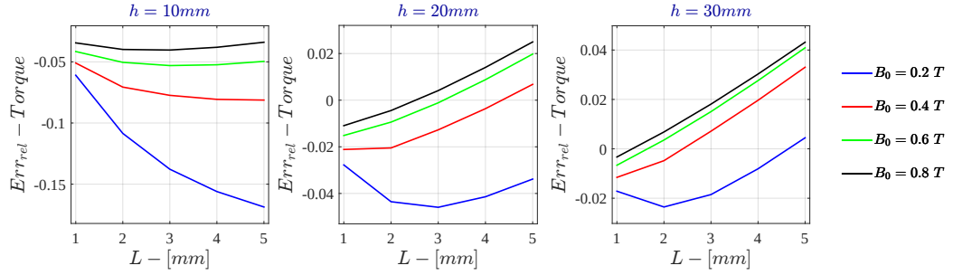
Figure I.13: Monodimensional LPM - Current Drive Relative Error - \dot{\Gamma} for \sigma = 10^5 \text{ S/m} - r_{out} = 50\text{mm}
