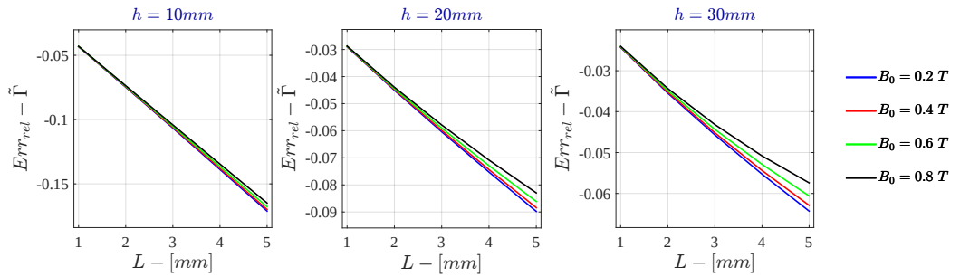
Figure 7.40: Bidimensional LPM - Current Drive Relative Error - \tilde{I} for \sigma = 10 \text{ S/m} - r_{out} = 50\text{mm}
