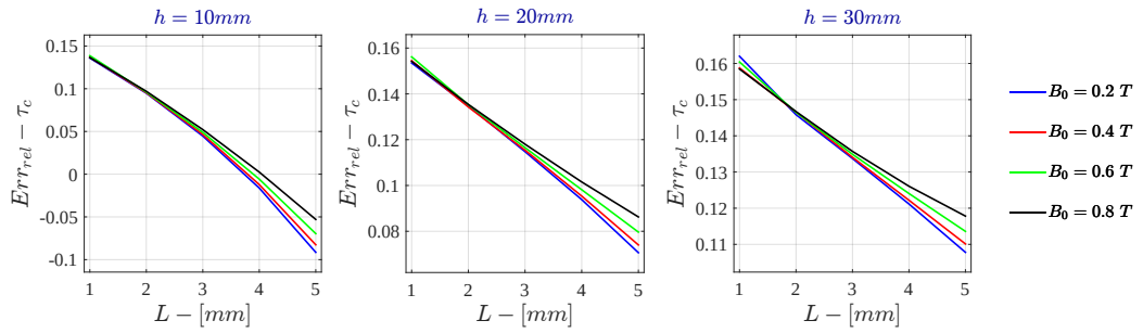
Figure F.22: Monodimensional LPM - Voltage Drive Relative Error - \tau_c for \sigma = 10^2 \text{ S/m} - r_{out} = 50\text{mm}
