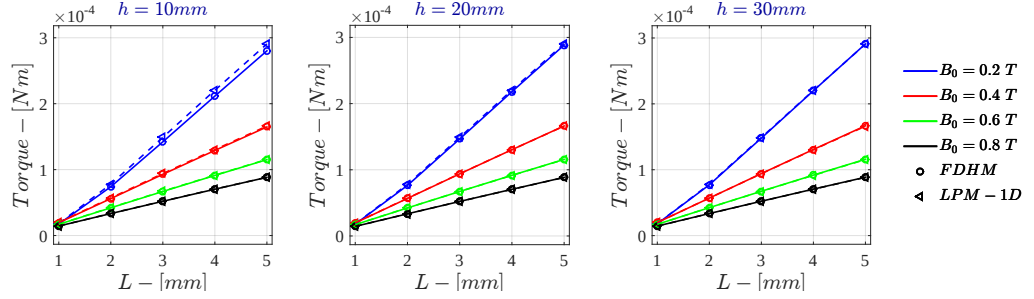
Figure I.17: Monodimensional LPM - Voltage Drive \dot{\Gamma} for \sigma = 10^5 \text{ S/m} - r_{out} = 50 \text{ mm}
