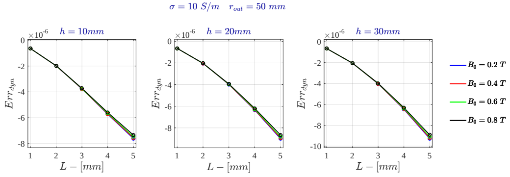
Figure 5.20: Voltage Drive - Relative Dynamic Error for \sigma = 10 \text{ S/m} - FDHM
