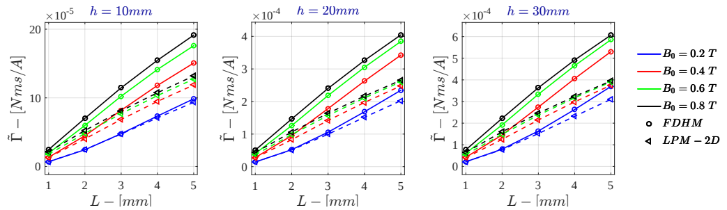
Figure H.44: Bidimensional LPM - Voltage Drive \tilde{\Gamma} for \sigma = 10^4 \text{ S/m} - r_{out} = 50\text{mm}
