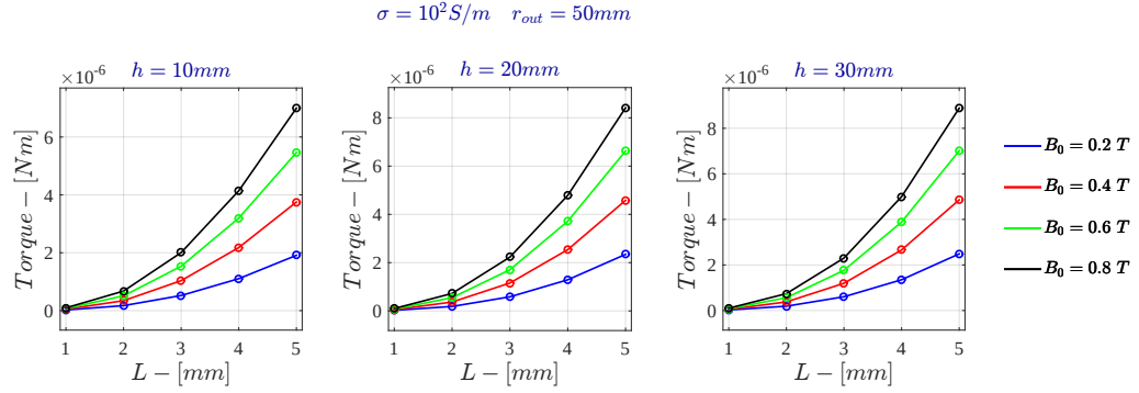
Figure B.7: Voltage Drive - Torque for \sigma = 10^2 \text{ S/m} - FDHM
