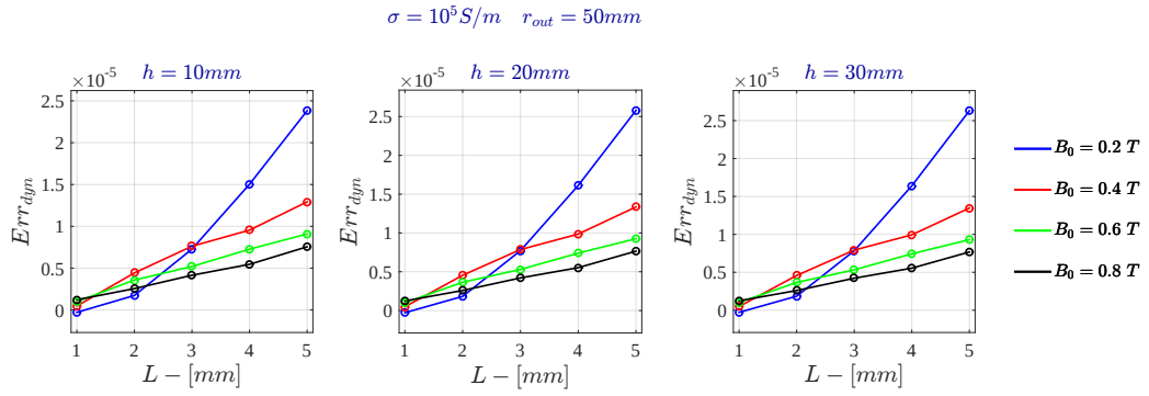
Figure E.5: Current Drive - Relative Dynamic Error for \sigma = 10^5 \text{ S/m} - FDHM
