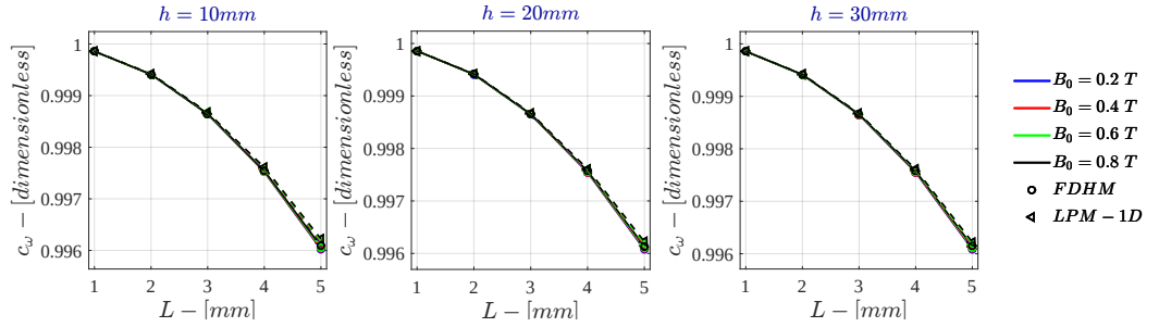
Figure F.3: Monodimensional LPM c_\omega for \sigma = 10^2 \text{ S/m} - r_{out} = 50 \text{ mm}
