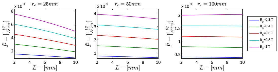
Figure 8.4: Power consumption function of L for B_0 = 0.2 \div 1.0 and 3 different outer radii r_e = 25, 50, 100\text{mm} . Liquid: Mercury (Hg).
