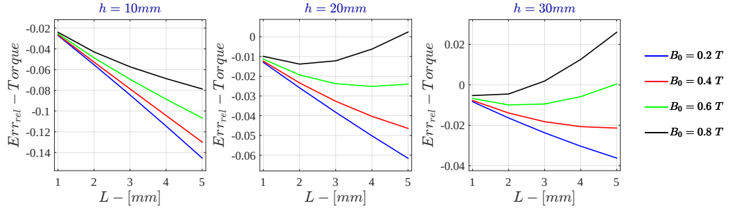
Figure F.45: Bidimensional LPM - Voltage Drive Relative Error - \dot{\Gamma} for \sigma = 10^2 \text{ S/m} - r_{out} = 50\text{mm}
