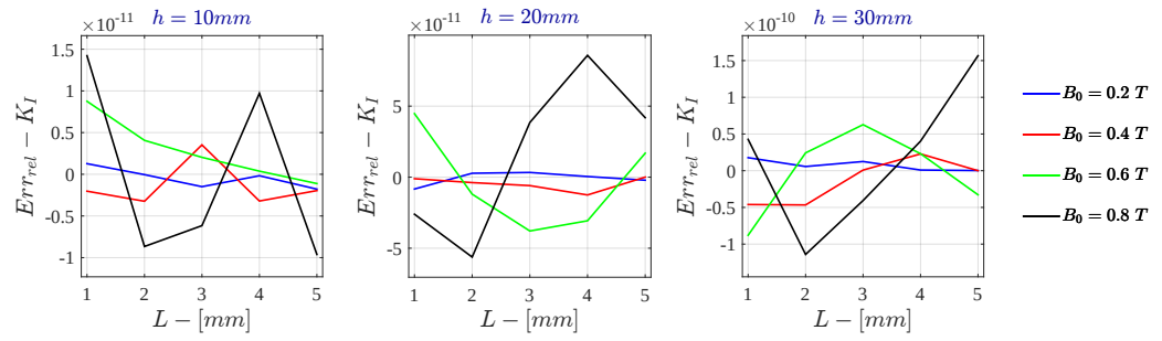
Figure 7.54: Monodimensional LPM Relative Error - K_I for \sigma = 10^6 S/m - r_{out} = 50 mm
