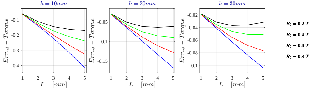
Figure G.21: Monodimensional LPM - Voltage Drive Relative Error - \dot{\Gamma} for \sigma = 10^3 \text{ S/m} - r_{out} = 50\text{mm}
