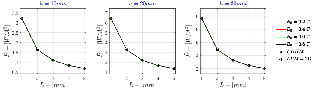
Figure 7.35: Bidimensional LPM - Current Drive \dot{P} for \sigma = 10 \text{ S/m} - r_{out} = 50\text{mm}
