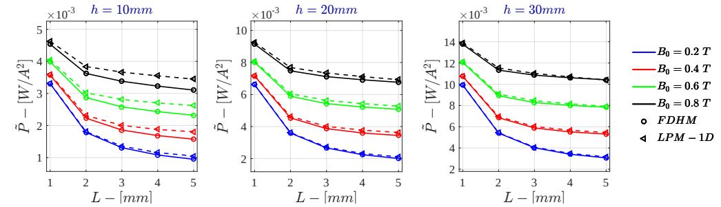
Figure H.11: Monodimensional LPM - Current Drive \dot{P} for \sigma = 10^4 \text{ S/m} - r_{out} = 50 \text{ mm}
