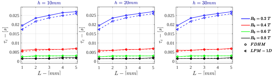
Figure 7.66: Monodimensional LPM - Voltage Drive \tau_c for \sigma = 10^6 S/m - r_{out} = 50 mm
