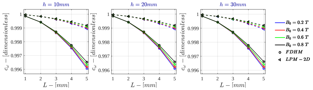
Figure G.27: Bidimensional LPM c_\omega for \sigma = 10^3 \text{ S/m} - r_{out} = 50\text{mm}
