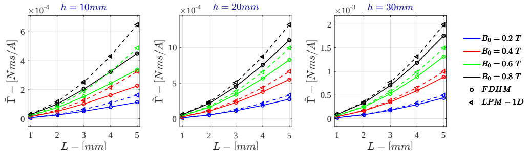
Figure 7.20: Monodimensional LPM - Voltage Drive \tilde{\Gamma} for \sigma = 10 \text{ S/m} - r_{out} = 50 \text{ mm}
