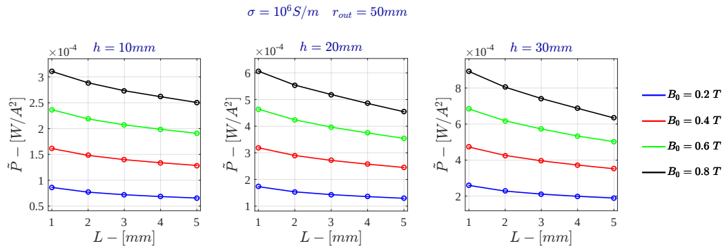
Figure 5.30: Voltage Drive - Specific Power for \sigma = 10^6 \text{ S/m} - FDHM
