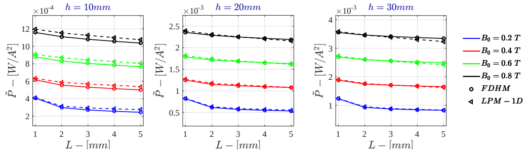
Figure I.35: Bidimensional LPM - Current Drive \dot{P} for \sigma = 10^5 \text{ S/m} - r_{out} = 50 \text{ mm}
