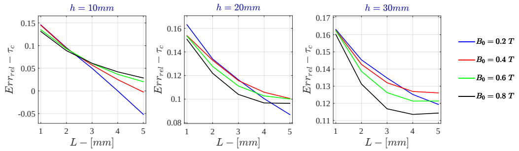
Figure H.14: Monodimensional LPM - Current Drive Relative Error - \tau_c for \sigma = 10^4 \text{ S/m} - r_{out} = 50\text{mm}
