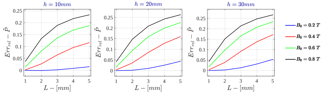
Figure H.47: Bidimensional LPM - Voltage Drive Relative Error - \tilde{P} for \sigma = 10^4 \text{ S/m} - r_{out} = 50\text{mm}
