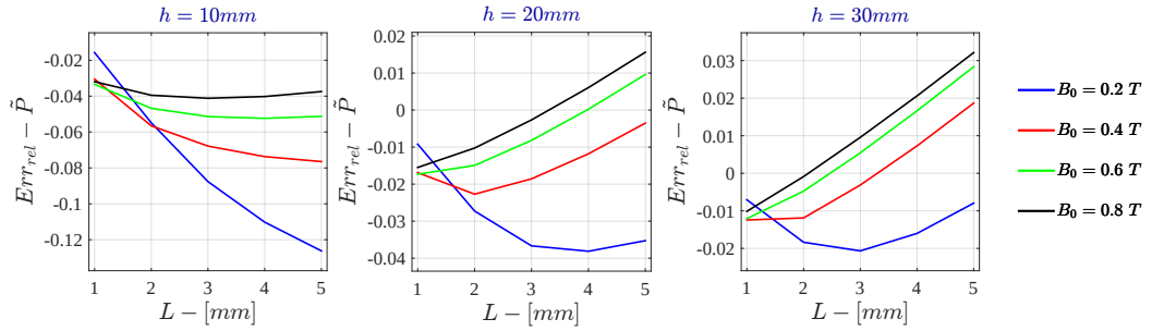
Figure I.15: Monodimensional LPM - Current Drive Relative Error - \tilde{P} for \sigma = 10^5 \text{ S/m} - r_{out} = 50\text{mm}
