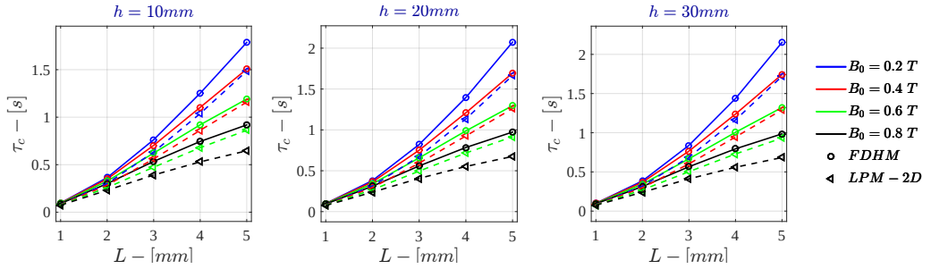
Figure G.42: Bidimensional LPM - Voltage Drive \tau_c for \sigma = 10^3 \text{ S/m} - r_{out} = 50\text{mm}
