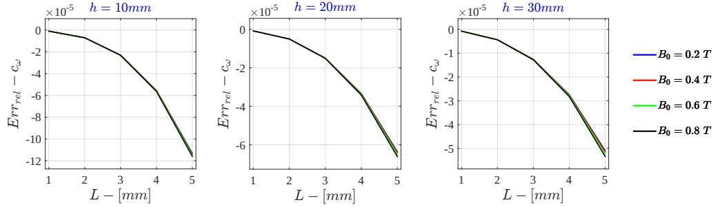
Figure 7.7: Monodimensional LPM Relative Error - c_{\omega} for \sigma = 10 S/m - r_{out} = 50 mm
