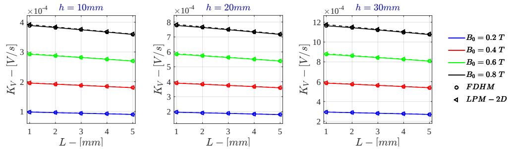
Figure 7.76: Bidimensional LPM K_V for \sigma = 10^6 S/m - r_{out} = 50\text{mm}
