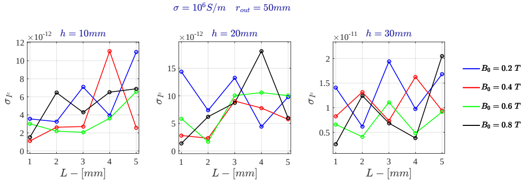
Figure 5.33: Voltage Drive - Standard deviation of the electric current for \sigma = 10^6 \text{ S/m} - FDHM
