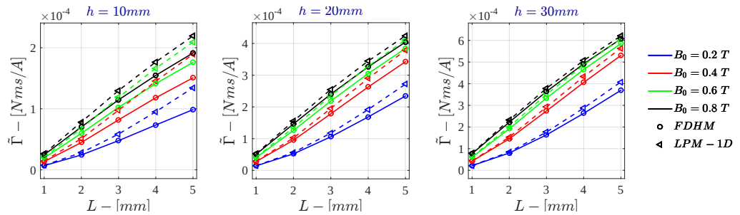
Figure H.20: Monodimensional LPM - Voltage Drive \dot{\Gamma} for \sigma = 10^4 \text{ S/m} - r_{\text{out}} = 50\text{mm}
