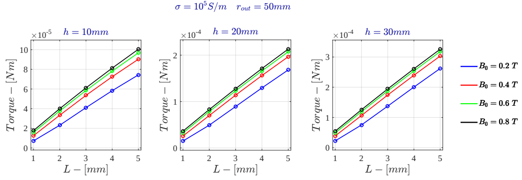
Figure E.1: Current Drive - Torque for \sigma = 10^5 \text{ S/m} - FDHM
