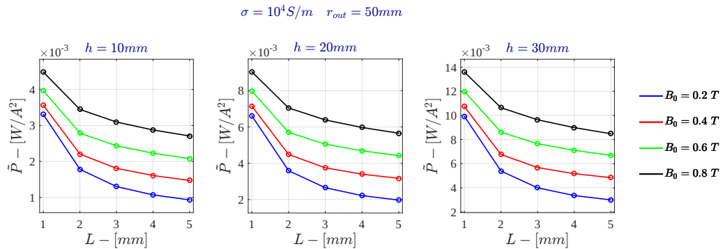
Figure D.9: Voltage Drive - Specific Power for \sigma = 10^4 \text{ S/m} - FDHM
