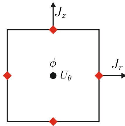
Figure 4.1: Arrangement of the physical quantities in a collocated grid.
