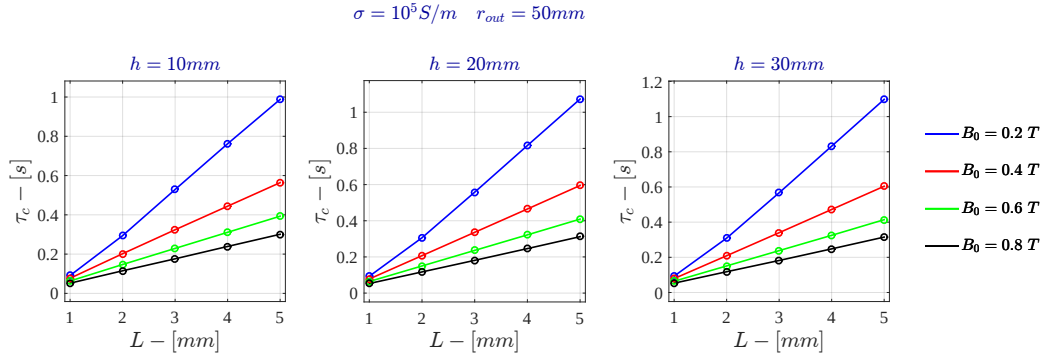
Figure E.2: Current Drive - Characteristic time for \sigma = 10^5 \text{ S/m} - FDHM
