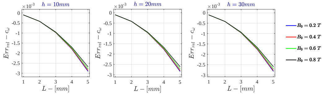
Figure G.31: Bidimensional LPM Relative Error - c_\omega for \sigma = 10^3 \text{ S/m} - r_{out} = 50\text{mm}
