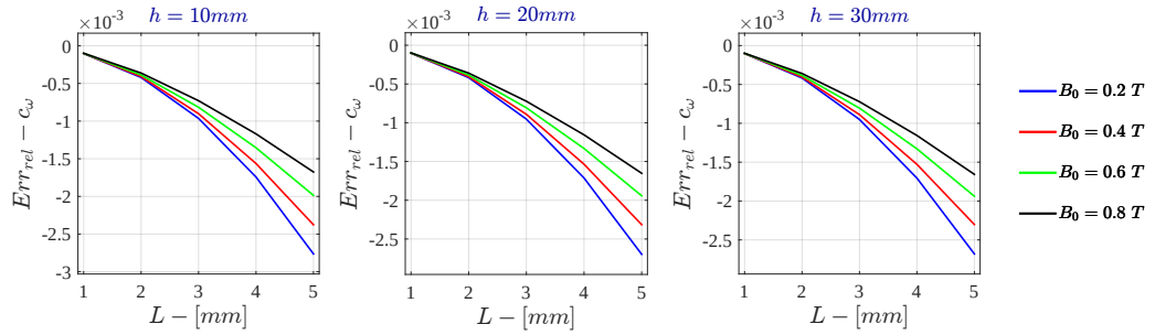
Figure H.31: Bidimensional LPM Relative Error - c_\omega for \sigma = 10^4 \text{ S/m} - r_{out} = 50\text{mm}
