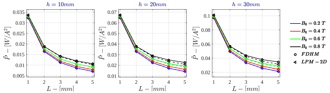
Figure G.43: Bidimensional LPM - Voltage Drive \tilde{P} for \sigma = 10^3 \text{ S/m} - r_{out} = 50\text{mm}
