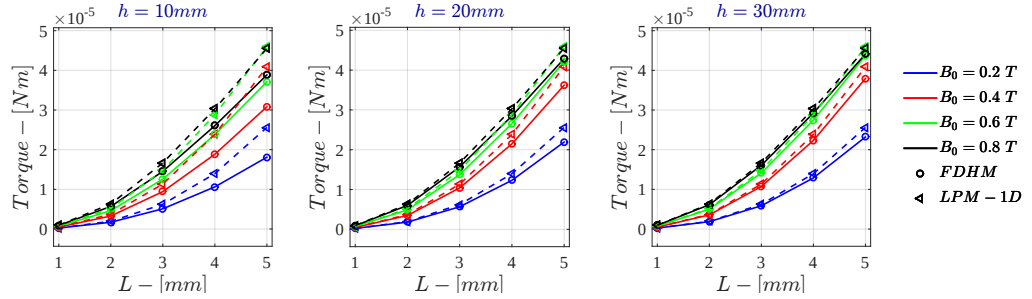
Figure G.17: Monodimensional LPM - Voltage Drive \dot{\Gamma} for \sigma = 10^3 \text{ S/m} - r_{out} = 50 \text{ mm}
