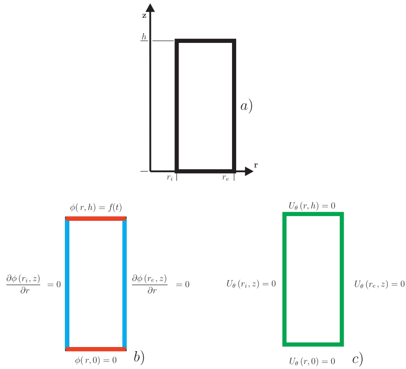
Figure 3.1: Boundary Condition applied to the Finite Difference model. a) Reference system and dimension of the cross section b) Electric boundary conditions c) Fluid-dynamics boundary conditions
