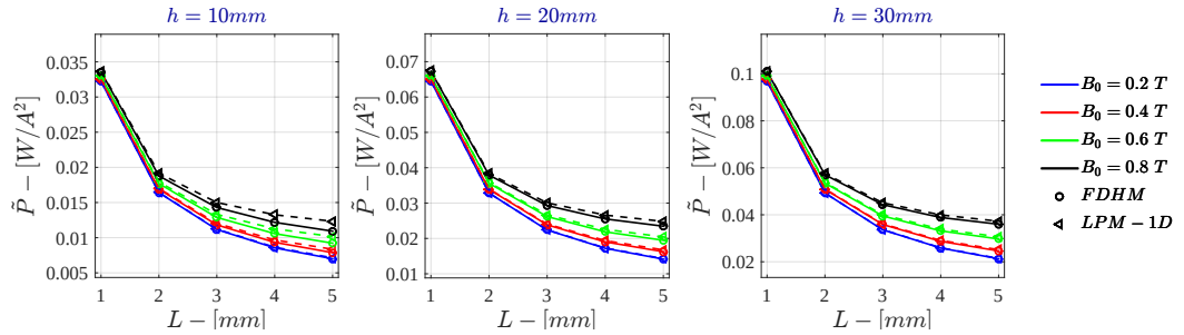
Figure G.11: Monodimensional LPM - Current Drive \dot{P} for \sigma = 10^3 \text{ S/m} - r_{out} = 50\text{mm}
