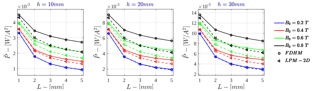
Figure H.43: Bidimensional LPM - Voltage Drive \tilde{P} for \sigma = 10^4 \text{ S/m} - r_{out} = 50\text{mm}
