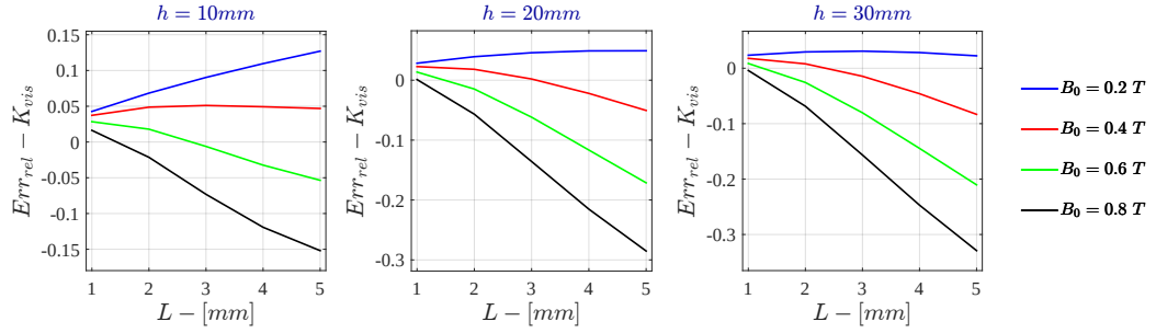
Figure G.29: Bidimensional LPM Relative Error - K_{vis} for \sigma = 10^3 \text{ S/m} - r_{out} = 50\text{mm}
