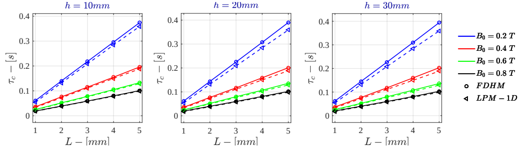
Figure 7.58: Monodimensional LPM - Current Drive \tau_c for \sigma = 10^6 \text{ S/m} - r_{out} = 50\text{mm}
