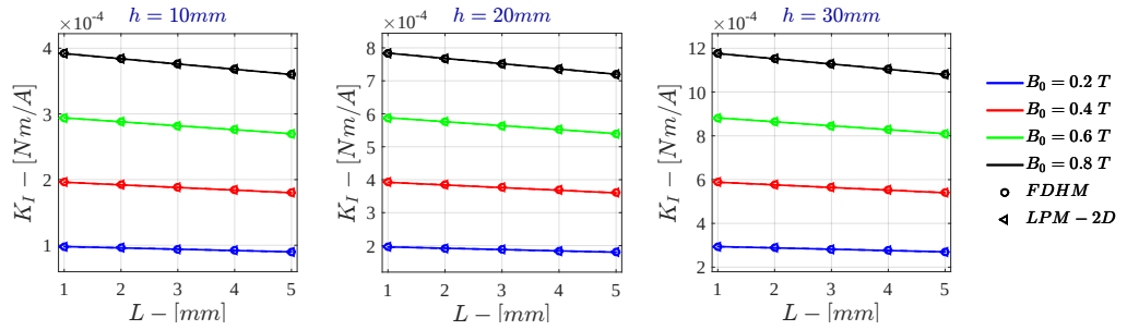
Figure G.26: Bidimensional LPM K_I for \sigma = 10^3 \text{ S/m} - r_{out} = 50\text{mm}
