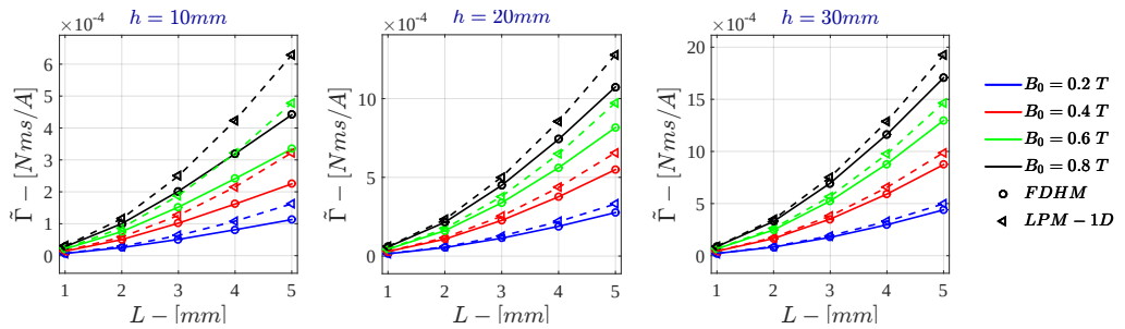
Figure F.20: Monodimensional LPM - Voltage Drive \tilde{\Gamma} for \sigma = 10^2 \text{ S/m} - r_{out} = 50\text{mm}
