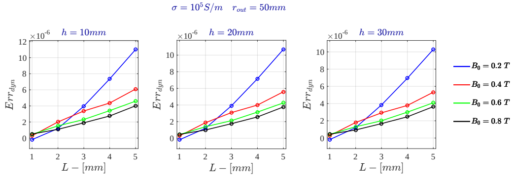
Figure E.11: Voltage Drive - Relative Dynamic Error for \sigma = 10^5 \text{ S/m} - FDHM
