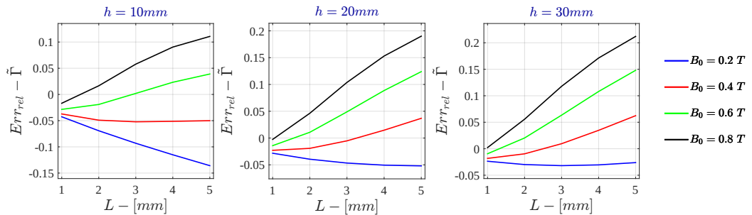
Figure G.48: Bidimensional LPM - Voltage Drive Relative Error - \tilde{I} for \sigma = 10^3 \text{ S/m} - r_{out} = 50\text{mm}
