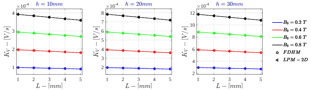
Figure 7.28: Bidimensional LPM K_V for \sigma = 10 S/m - r_{out} = 50mm
