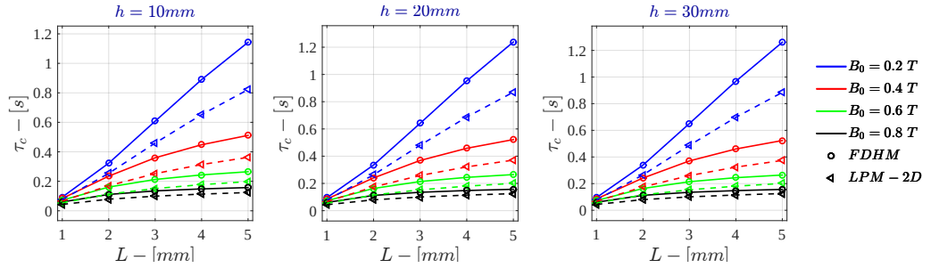
Figure H.42: Bidimensional LPM - Voltage Drive \tau_c for \sigma = 10^4 \text{ S/m} - r_{out} = 50\text{mm}
