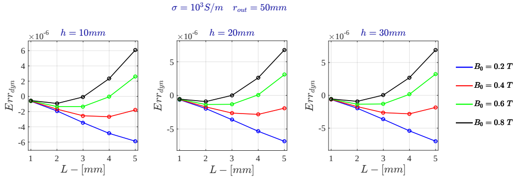
Figure C.11: Voltage Drive - Relative Dynamic Error for \sigma = 10^3 \text{ S/m} - FDHM
