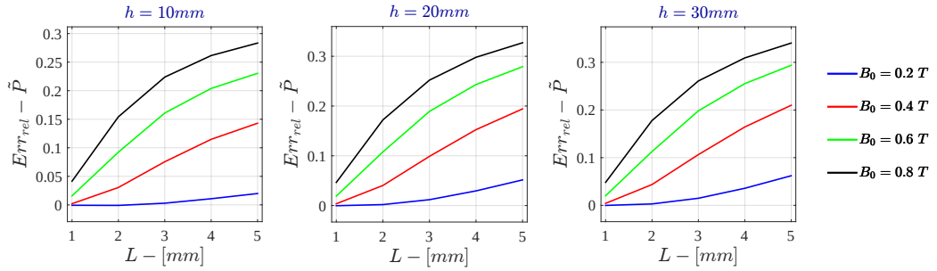
Figure H.39: Bidimensional LPM - Current Drive Relative Error - \tilde{P} for \sigma = 10^4 \text{ S/m} - r_{out} = 50\text{mm}
