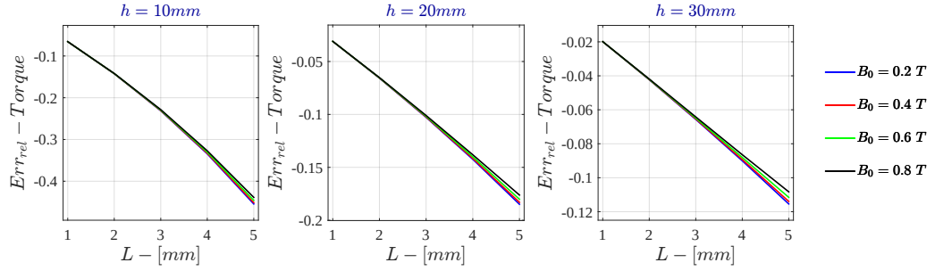
Figure F.13: Monodimensional LPM - Current Drive Relative Error - \dot{\Gamma} for \sigma = 10^2 \text{ S/m} - r_{out} = 50\text{mm}
