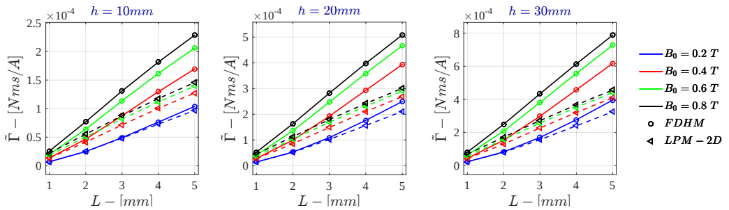
Figure H.36: Bidimensional LPM - Current Drive \tilde{\Gamma} for \sigma = 10^4 \text{ S/m} - r_{out} = 50\text{mm}
