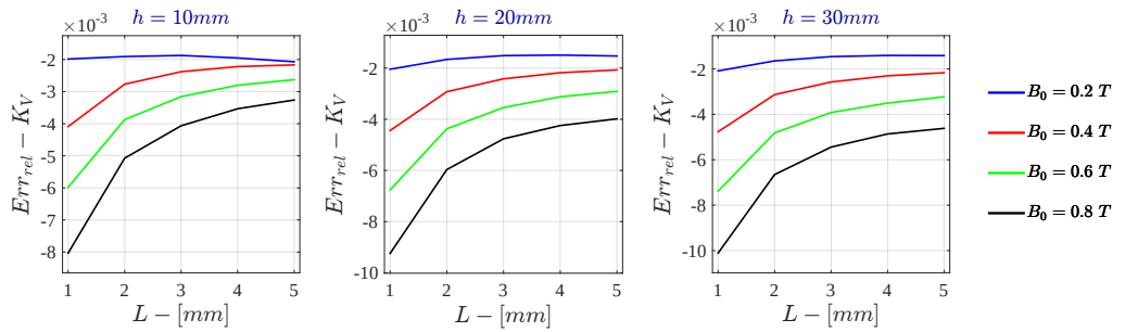
Figure 7.80: Bidimensional LPM Relative Error - K_V for \sigma = 10^6 S/m - r_{out} = 50 mm
