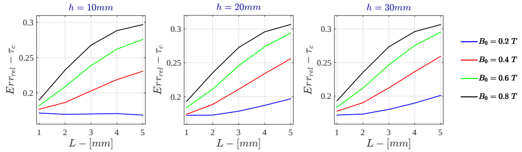
Figure G.46: Bidimensional LPM - Voltage Drive Relative Error - \tau_c for \sigma = 10^3 \text{ S/m} - r_{out} = 50\text{mm}
