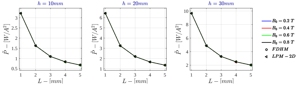
Figure 7.43: Bidimensional LPM - Voltage Drive \tilde{P} for \sigma = 10 S/m - r_{out} = 50 mm
