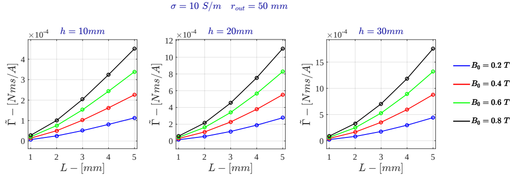
Figure 5.19: Voltage Drive - Specific Angular Momentum for \sigma = 10 \text{ S/m} - FDHM
