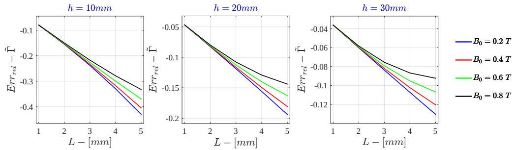
Figure G.24: Monodimensional LPM - Voltage Drive Relative Error - \tilde{I} for \sigma = 10^3 \text{ S/m} - r_{out} = 50\text{mm}
