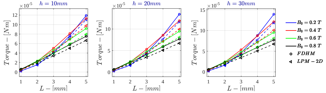
Figure H.41: Bidimensional LPM - Voltage Drive \dot{\Gamma} for \sigma = 10^4 \text{ S/m} - r_{out} = 50\text{mm}
