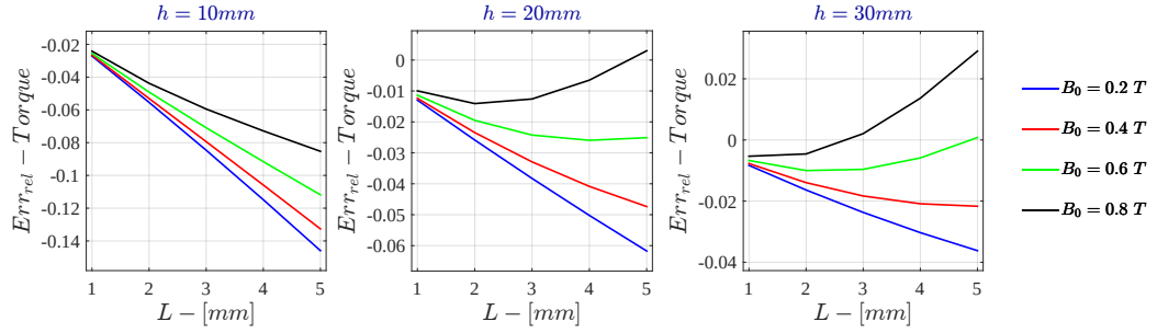
Figure H.37: Bidimensional LPM - Current Drive Relative Error - \dot{\Gamma} for \sigma = 10^4 \text{ S/m} - r_{out} = 50\text{mm}
