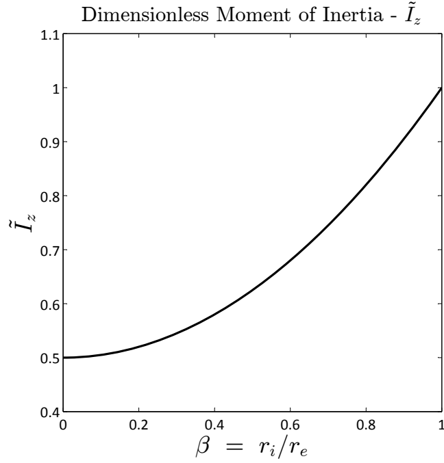
Figure 2.4: Dimensionless Moment of Inertia
