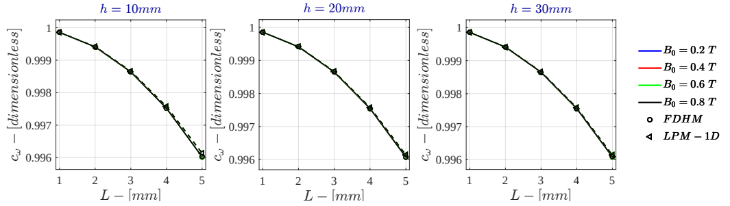
Figure 7.3: Monodimensional LPM c_w for \sigma = 10 S/m - r_{out} = 50mm
