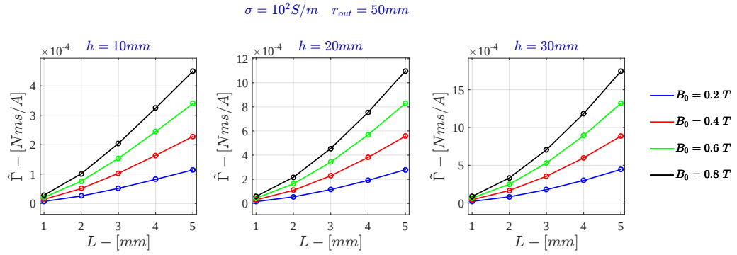
Figure B.4: Current Drive - Specific Angular Momentum for \sigma = 10^2 \text{ S/m} - FDHM
