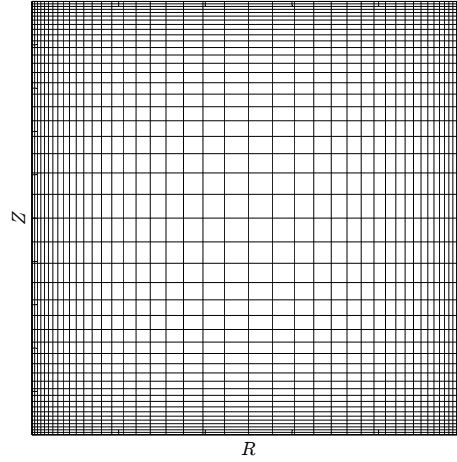
Figure 4.4: Grid for \delta_{Sh} > h/6 and \delta_{Hrtm} > (r_e - r_i)/6 .
