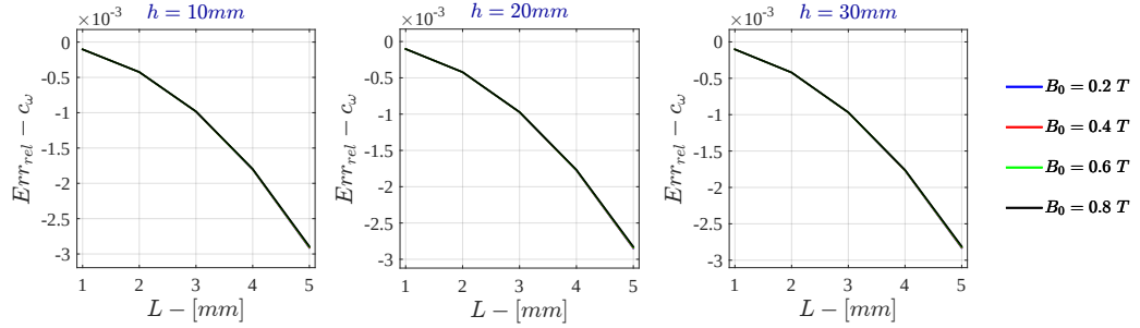
Figure F.31: Bidimensional LPM Relative Error - c_{\omega} for \sigma = 10^2 \text{ S/m} - r_{out} = 50\text{mm}
