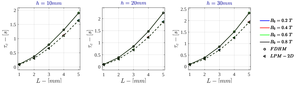
Figure 7.34: Bidimensional LPM - Current Drive \tau_c for \sigma = 10 \text{ S/m} - r_{out} = 50\text{mm}
