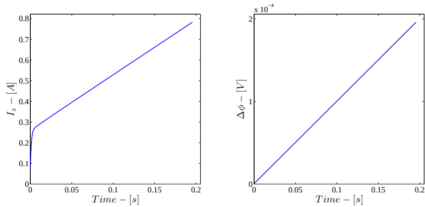
Figure 5.7: FDHM - Voltage Drive
