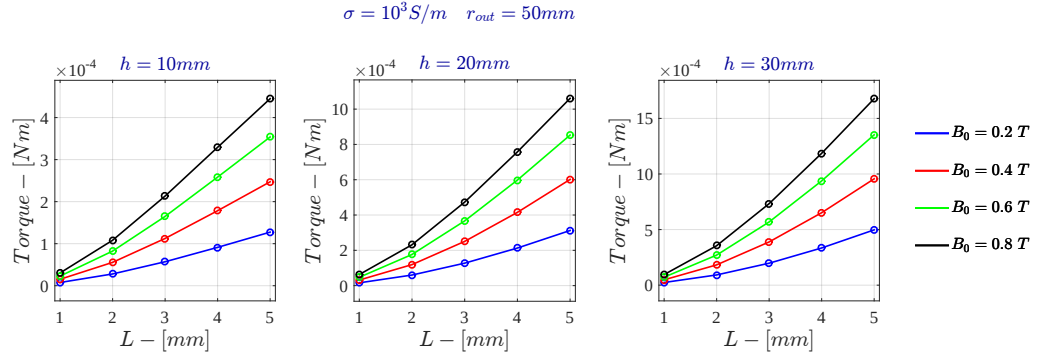
Figure C.1: Current Drive - Torque for \sigma = 10^3 \text{ S/m} - FDHM
