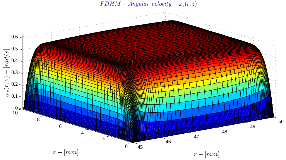
Figure 5.4: FDHM - Angular velocity
