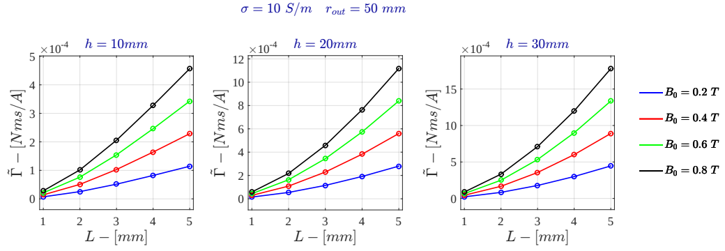
Figure 5.13: Current Drive - Specific Angular Momentum for \sigma = 10 \text{ S/m} - FDHM
