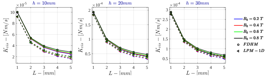
Figure G.1: K_{vis} for \sigma = 10^3 \text{ S/m} - r_{out} = 50\text{mm} - Monodimensional LPM
