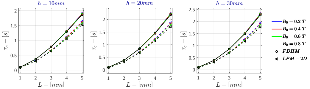
Figure F.34: Bidimensional LPM - Current Drive \tau_c for \sigma = 10^2 \text{ S/m} - r_{\text{out}} = 50\text{mm}
