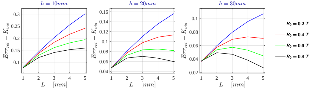
Figure H.5: Monodimensional LPM Relative Error - K_{vis} for \sigma = 10^4 \text{ S/m} - r_{out} = 50\text{mm}
