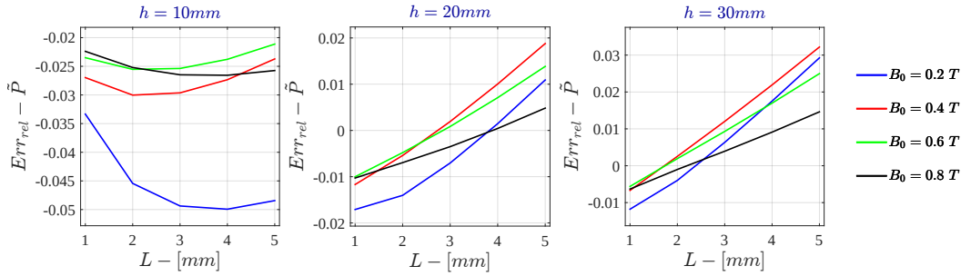
Figure 7.63: Monodimensional LPM - Current Drive Relative Error - \tilde{P} for \sigma = 10^6 S/m - r_{out} = 50mm
