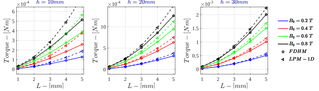
Figure 7.33: Bidimensional LPM - Current Drive \dot{\Gamma} for \sigma = 10 \text{ S/m} - r_{out} = 50\text{mm}
