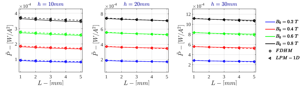
Figure 7.83: Bidimensional LPM - Current Drive \tilde{P} for \sigma = 10^6 S/m - r_{out} = 50 mm
