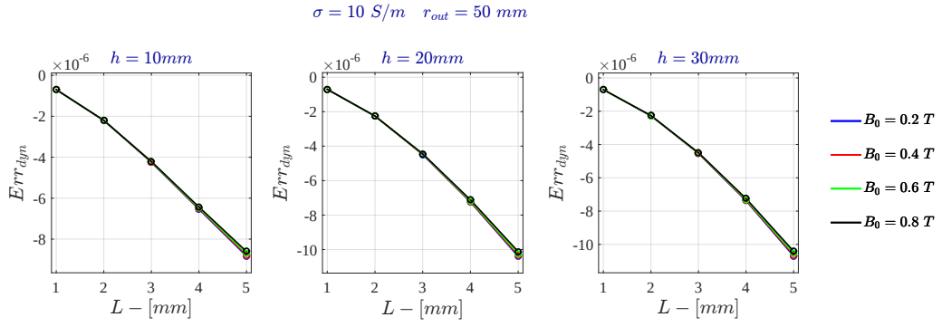
Figure 5.14: Current Drive - Relative Dynamic Error for \sigma = 10 \text{ S/m} - FDHM
