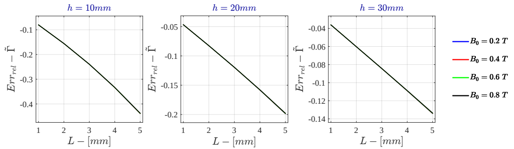
Figure 7.24: Monodimensional LPM - Voltage Drive Relative Error - \tilde{I} for \sigma = 10 \text{ S/m} - r_{out} = 50\text{mm}
