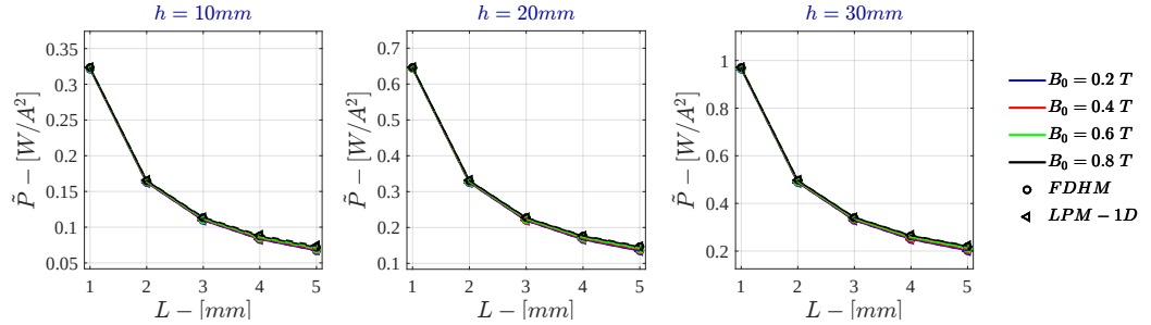
Figure F.11: Monodimensional LPM - Current Drive \dot{P} for \sigma = 10^2 \text{ S/m} - r_{out} = 50\text{mm}
