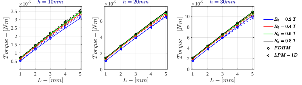
Figure 7.57: Monodimensional LPM - Current Drive \dot{\Gamma} for \sigma = 10^6 \text{ S/m} - r_{out} = 50\text{mm}
