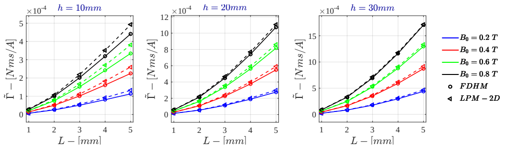
Figure F.44: Bidimensional LPM - Voltage Drive \tilde{\Gamma} for \sigma = 10^2 \text{ S/m} - r_{out} = 50\text{mm}
