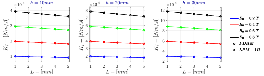
Figure 7.2: Monodimensional LPM K_I for \sigma = 10 S/m - r_{out} = 50mm
