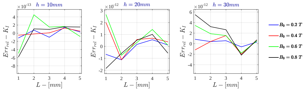
Figure H.6: Monodimensional LPM Relative Error - K_I for \sigma = 10^4 \text{ S/m} - r_{out} = 50\text{mm}
