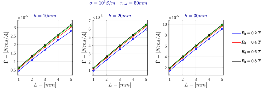
Figure 5.25: Current Drive - Specific Angular Momentum for \sigma = 10^6 \text{ S/m} - FDHM
