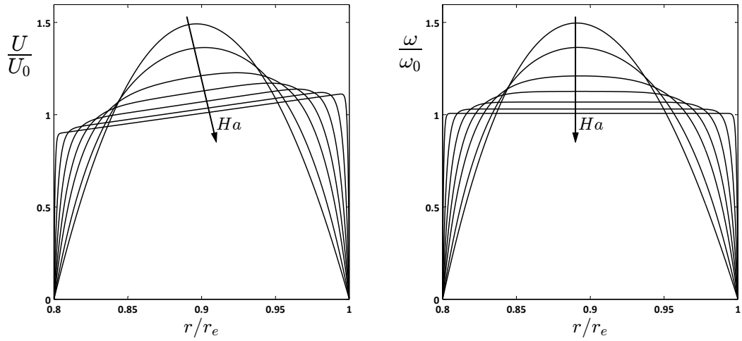
Figure 6.2: Analytical solutions for dimensionless linear and angular velocities at different Hartmann Number Ha .
