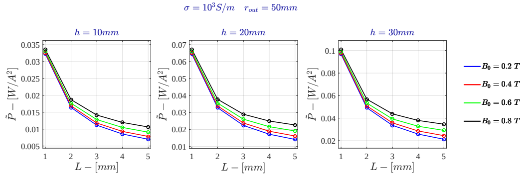
Figure C.9: Voltage Drive - Specific Power for \sigma = 10^3 \text{ S/m} - FDHM
