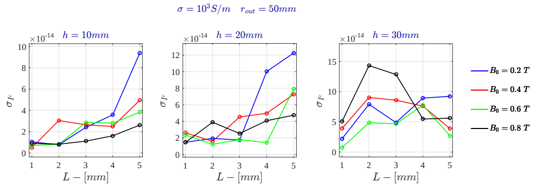
Figure C.12: Voltage Drive - Standard deviation of the electric current for \sigma = 10^3 \text{ S/m} - FDHM
