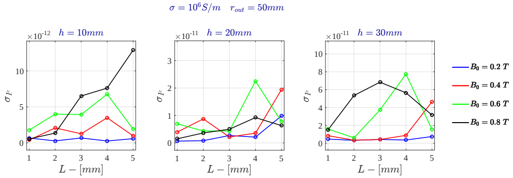
Figure 5.27: Current Drive - Standard deviation of the electric current for \sigma = 10^6 \text{ S/m} - FDHM
