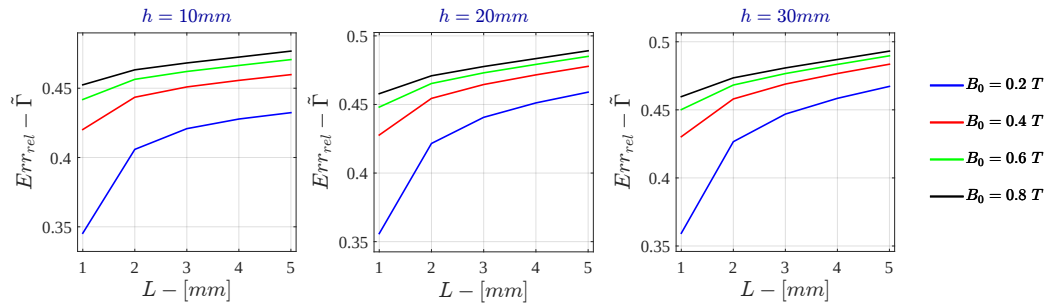
Figure 7.88: Bidimensional LPM - Current Drive Relative Error - \tilde{I} for \sigma = 10^6 S/m - r_{out} = 50 mm
