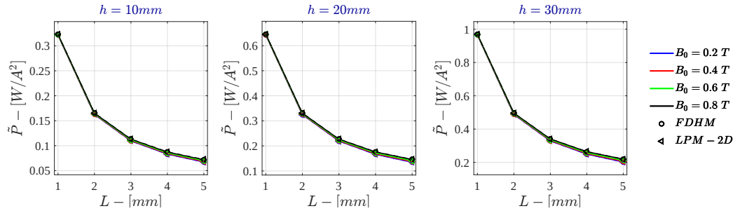
Figure F.43: Bidimensional LPM - Voltage Drive \dot{P} for \sigma = 10^2 \text{ S/m} - r_{out} = 50\text{mm}
