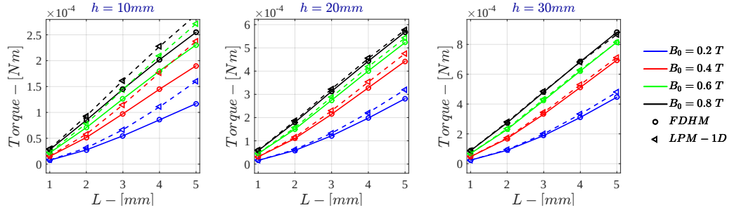
Figure H.33: Bidimensional LPM - Current Drive \dot{\Gamma} for \sigma = 10^4 \text{ S/m} - r_{out} = 50\text{mm}
