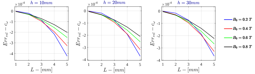
Figure I.7: Monodimensional LPM Relative Error - c_{\omega} for \sigma = 10^5 \text{ S/m} - r_{out} = 50 \text{ mm}
