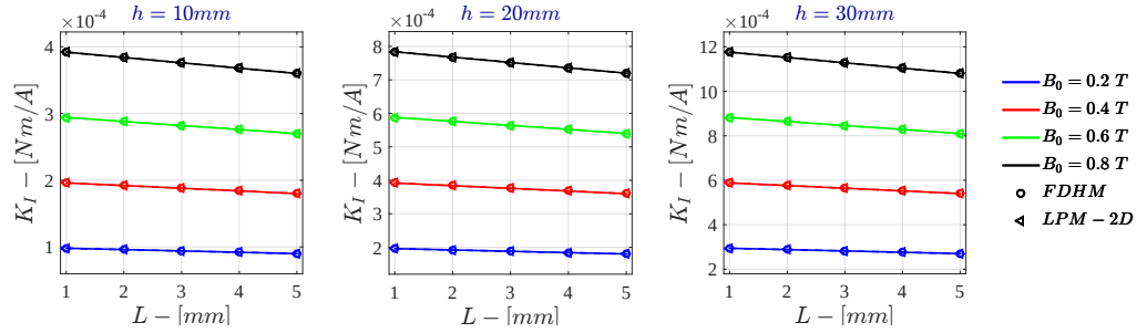
Figure 7.74: Bidimensional LPM K_I for \sigma = 10^6 S/m - r_{out} = 50\text{mm}
