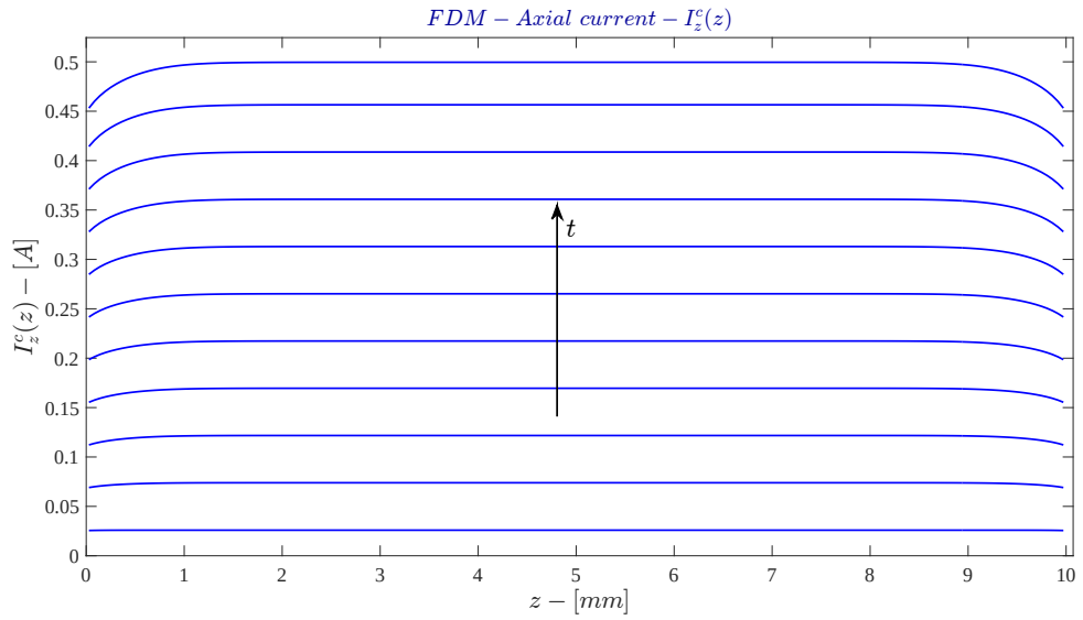
Figure 4.6: FDM - Total axial electric current
