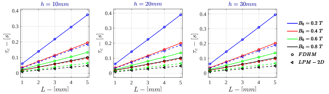
Figure 7.82: Bidimensional LPM - Current Drive \tau_c for \sigma = 10^6 S/m - r_{out} = 50 mm
