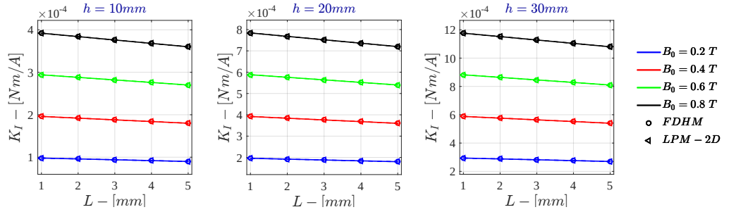
Figure I.26: Bidimensional LPM K_I for \sigma = 10^5 \text{ S/m} - r_{out} = 50\text{mm}
