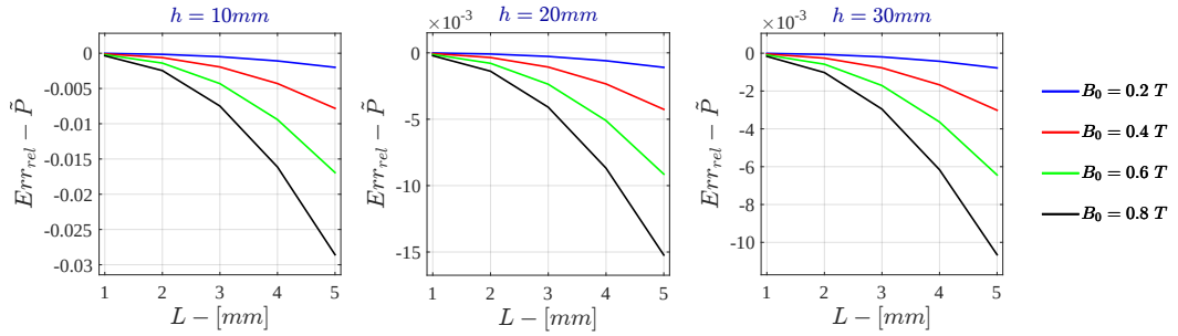
Figure F.15: Monodimensional LPM - Current Drive Relative Error - \tilde{P} for \sigma = 10^2 \text{ S/m} - r_{out} = 50\text{mm}
