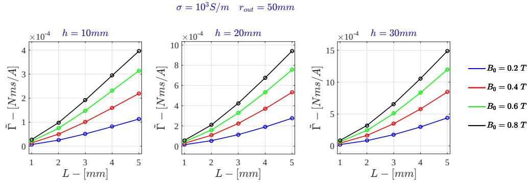
Figure C.4: Current Drive - Specific Angular Momentum for \sigma = 10^3 \text{ S/m} - FDHM
