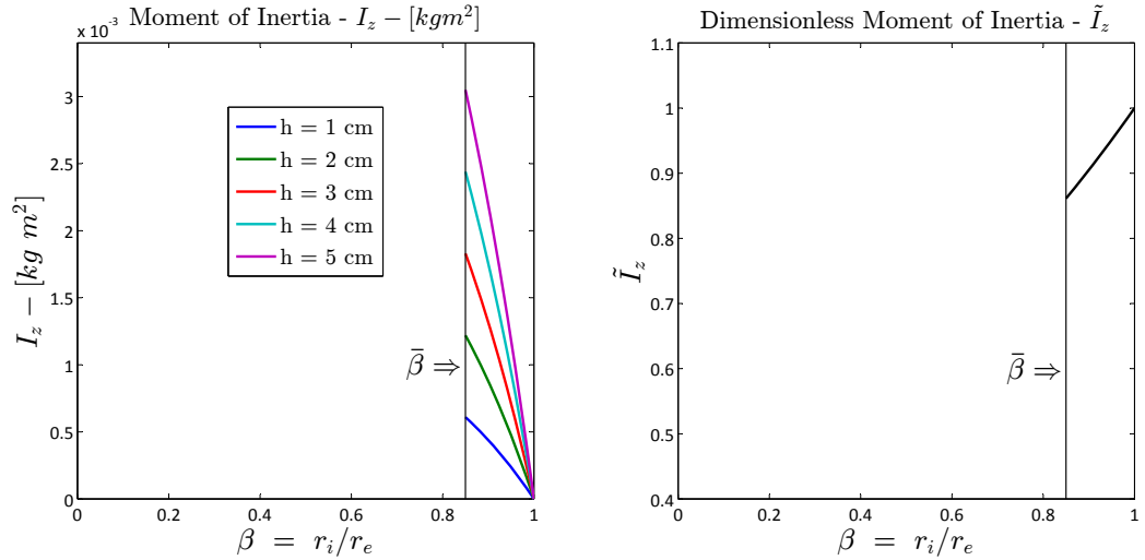
Figure 2.6: Dimensional and Dimensionless Moment of Inertia - 2 st Configuration
