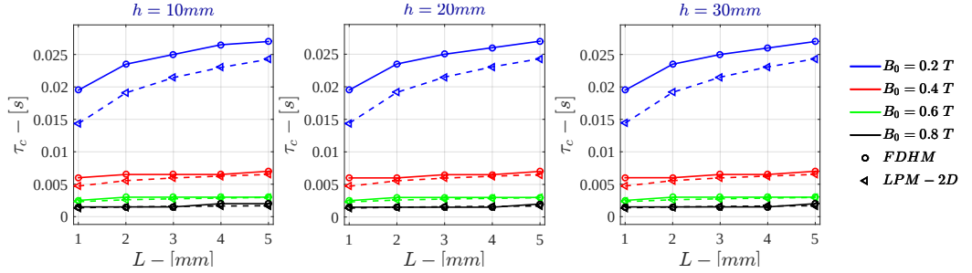
Figure 7.90: Bidimensional LPM - Voltage Drive \tau_c for \sigma = 10^6 S/m - r_{out} = 50 mm
