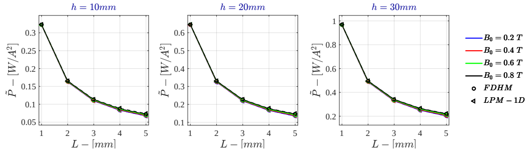
Figure G.19: Monodimensional LPM - Voltage Drive \dot{P} for \sigma = 10^3 \text{ S/m} - r_{out} = 50 \text{ mm}
