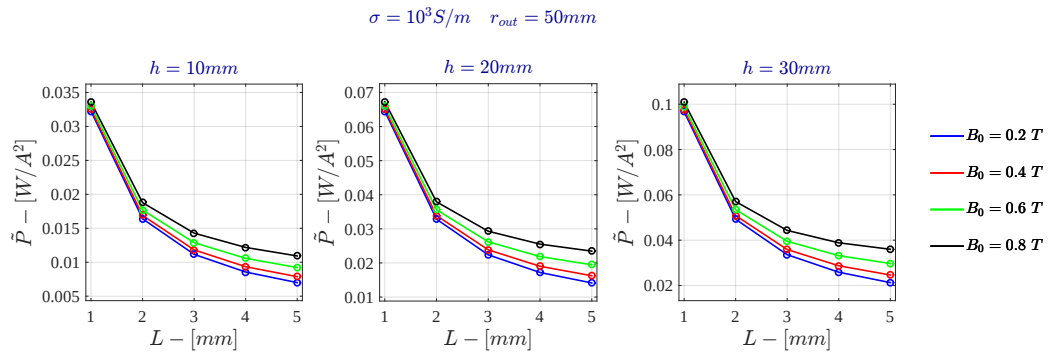
Figure C.3: Current Drive - Specific Power for \sigma = 10^3 \text{ S/m} - FDHM
