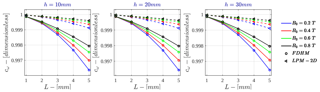
Figure H.27: Bidimensional LPM c_\omega for \sigma = 10^4 \text{ S/m} - r_{out} = 50\text{mm}
