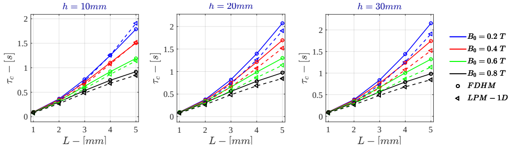
Figure G.18: Monodimensional LPM - Voltage Drive \tau_c for \sigma = 10^3 \text{ S/m} - r_{out} = 50 \text{ mm}
