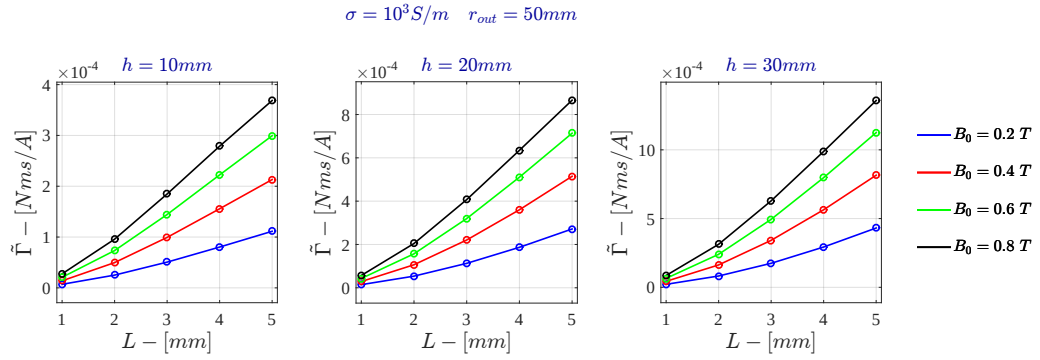
Figure C.10: Voltage Drive - Specific Angular Momentum for \sigma = 10^3 \text{ S/m} - FDHM
