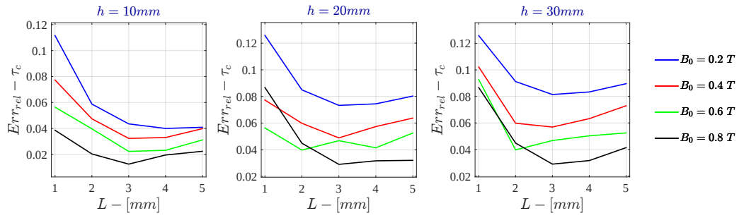
Figure 7.62: Monodimensional LPM - Current Drive Relative Error - \tau_c for \sigma = 10^6 S/m - r_{out} = 50mm
