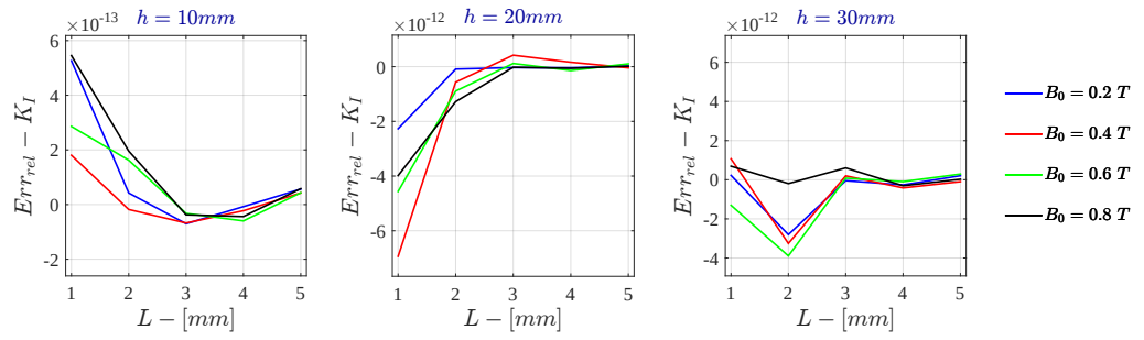
Figure 7.6: Monodimensional LPM Relative Error - K_I for \sigma = 10 S/m - r_{out} = 50 mm
