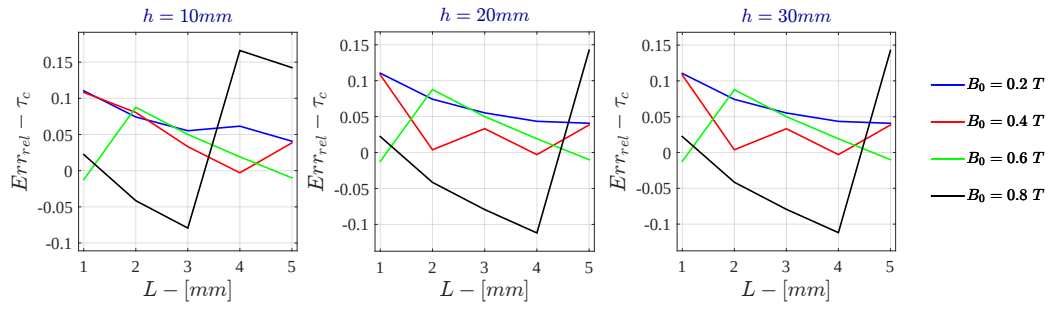
Figure 7.70: Monodimensional LPM - Voltage Drive Relative Error - \tau_c for \sigma = 10^6 S/m - r_{out} = 50 mm
