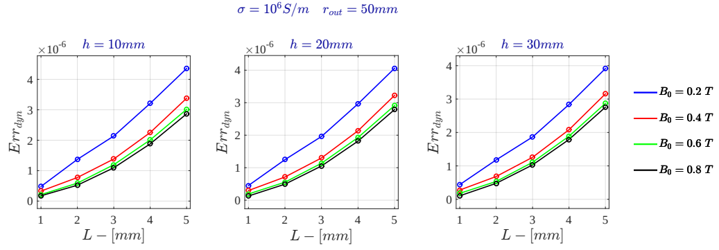
Figure 5.32: Voltage Drive - Relative Dynamic Error for \sigma = 10^6 \text{ S/m} - FDHM
