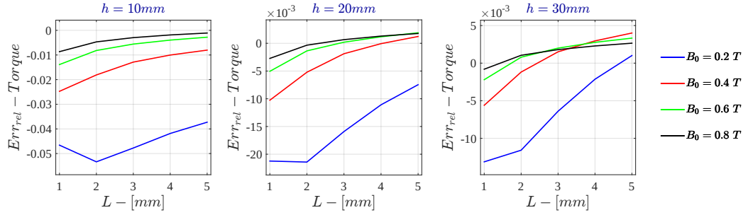
Figure I.21: Monodimensional LPM - Voltage Drive Relative Error - \dot{\Gamma} for \sigma = 10^5 \text{ S/m} - r_{out} = 50\text{mm}
