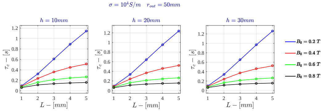
Figure D.8: Voltage Drive - Characteristic time for \sigma = 10^4 \text{ S/m} - FDHM
