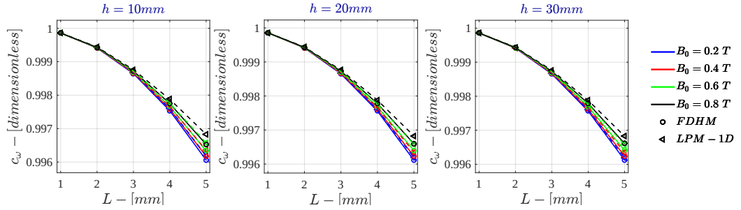
Figure G.3: Monodimensional LPM c_\omega for \sigma = 10^3 \text{ S/m} - r_{out} = 50\text{mm}
