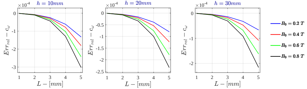
Figure G.7: Monodimensional LPM Relative Error - c_\omega for \sigma = 10^3 \text{ S/m} - r_{out} = 50\text{mm}
