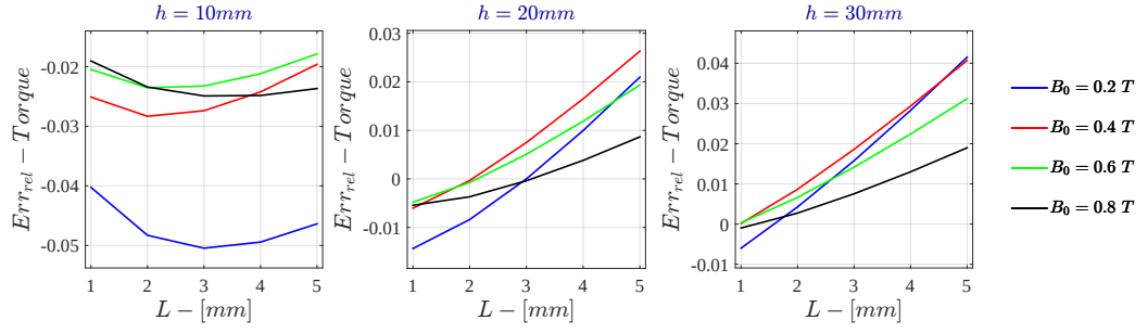
Figure 7.61: Monodimensional LPM - Current Drive Relative Error - \dot{\Gamma} for \sigma = 10^6 S/m - r_{out} = 50mm
