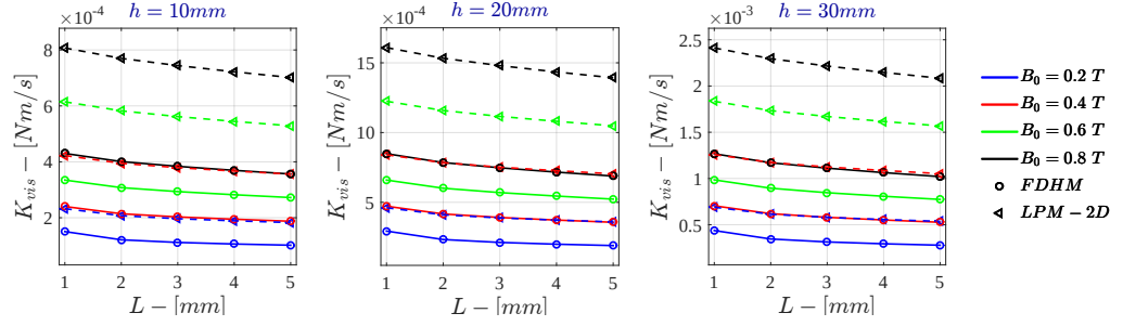
Figure 7.73: Bidimensional LPM K_{vis} for \sigma = 10^6 S/m - r_{out} = 50\text{mm}
