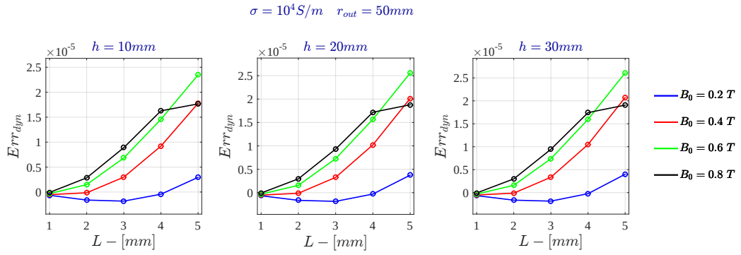
Figure D.5: Current Drive - Relative Dynamic Error for \sigma = 10^4 \text{ S/m} - FDHM
