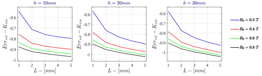
Figure 7.77: Bidimensional LPM Relative Error - K_{vis} for \sigma = 10^6 S/m - r_{out} = 50 mm
