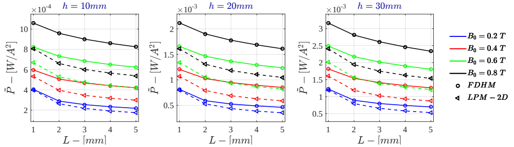
Figure I.43: Bidimensional LPM - Voltage Drive \dot{P} for \sigma = 10^5 \text{ S/m} - r_{out} = 50 \text{ mm}
