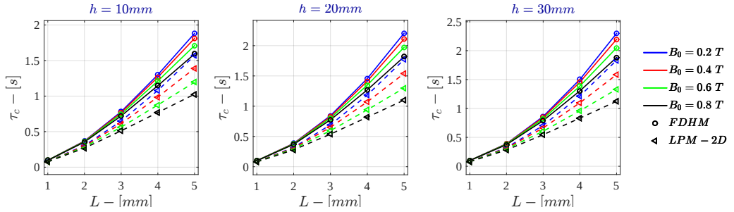
Figure G.34: Bidimensional LPM - Current Drive \tau_c for \sigma = 10^3 \text{ S/m} - r_{out} = 50\text{mm}
