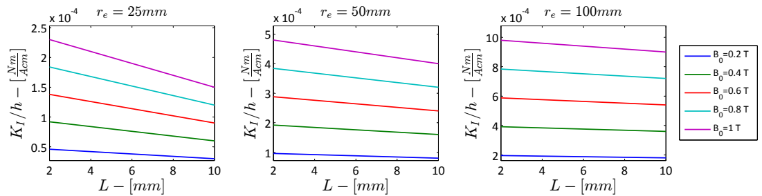
Figure 8.1: K_I function of L for B_0 = 0.2 \div 1.0 and 3 different outer radii r_e = 25, 50, 100\text{mm} . Liquid: Mercury (Hg).
