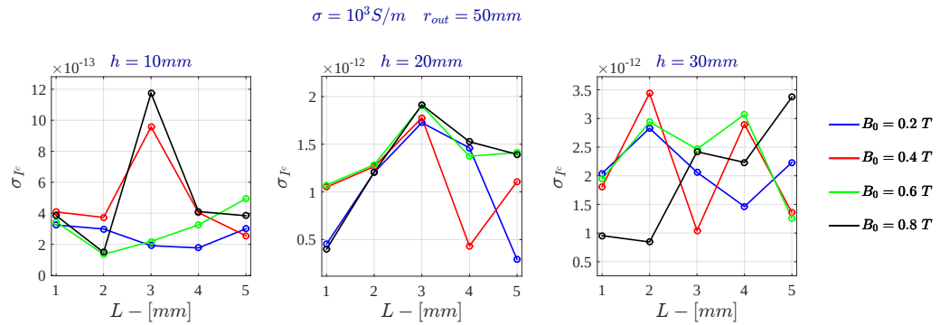
Figure C.6: Current Drive - Standard deviation of the electric current for \sigma = 10^3 \text{ S/m} - FDHM
