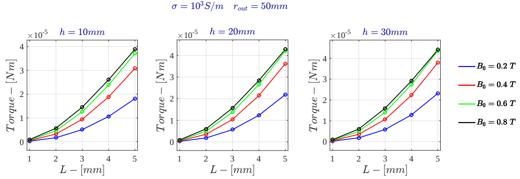
Figure C.7: Voltage Drive - Torque for \sigma = 10^3 \text{ S/m} - FDHM
