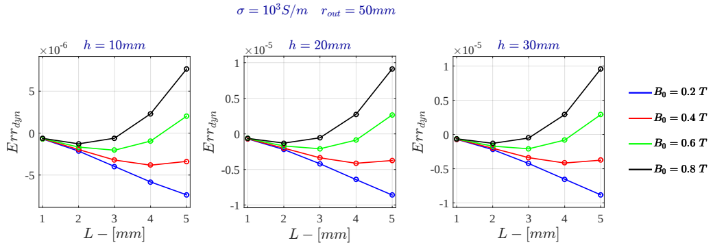
Figure C.5: Current Drive - Relative Dynamic Error for \sigma = 10^3 \text{ S/m} - FDHM
