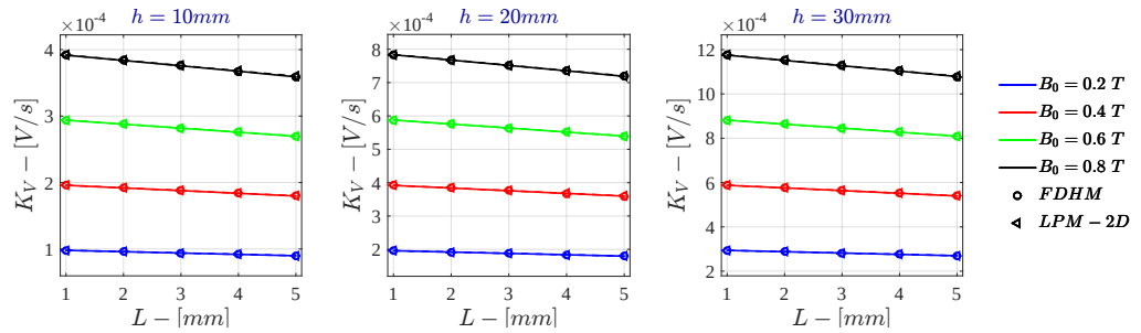
Figure H.28: Bidimensional LPM K_V for \sigma = 10^4 \text{ S/m} - r_{out} = 50\text{mm}
