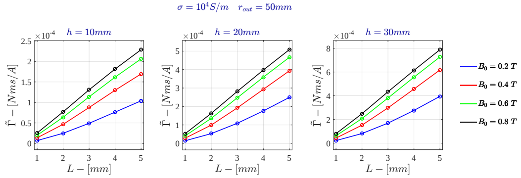
Figure D.4: Current Drive - Specific Angular Momentum for \sigma = 10^4 \text{ S/m} - FDHM
