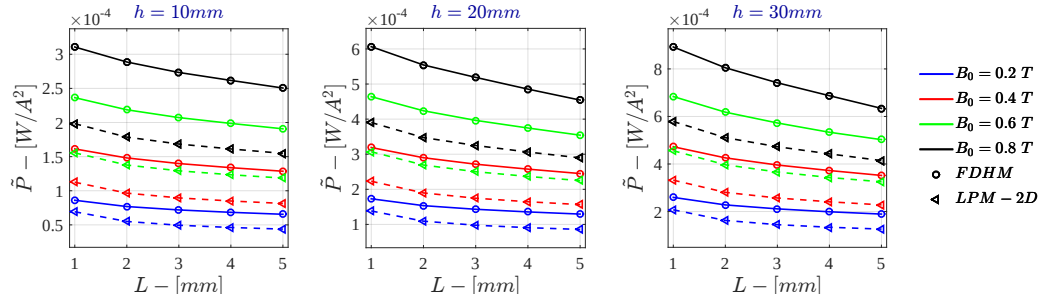
Figure 7.91: Bidimensional LPM - Voltage Drive \tilde{P} for \sigma = 10^6 S/m - r_{out} = 50 mm
