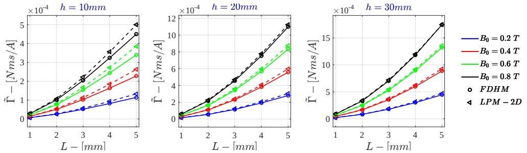
Figure F.36: Bidimensional LPM - Current Drive \tilde{\Gamma} for \sigma = 10^2 \text{ S/m} - r_{\text{out}} = 50\text{mm}
