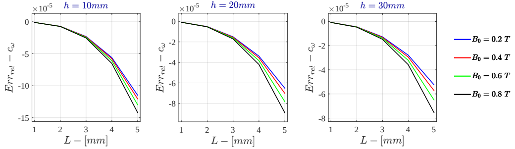
Figure F.7: Monodimensional LPM Relative Error - c_\omega for \sigma = 10^2 \text{ S/m} - r_{out} = 50\text{mm}
