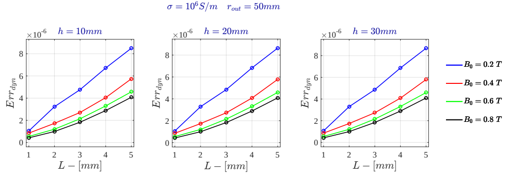
Figure 5.26: Current Drive - Relative Dynamic Error for \sigma = 10^6 \text{ S/m} - FDHM
