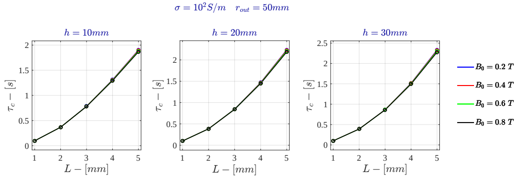
Figure B.2: Current Drive - Characteristic time for \sigma = 10^2 \text{ S/m} - FDHM
