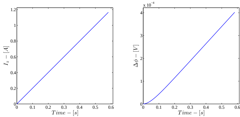
Figure 5.6: FDHM - Current Drive
