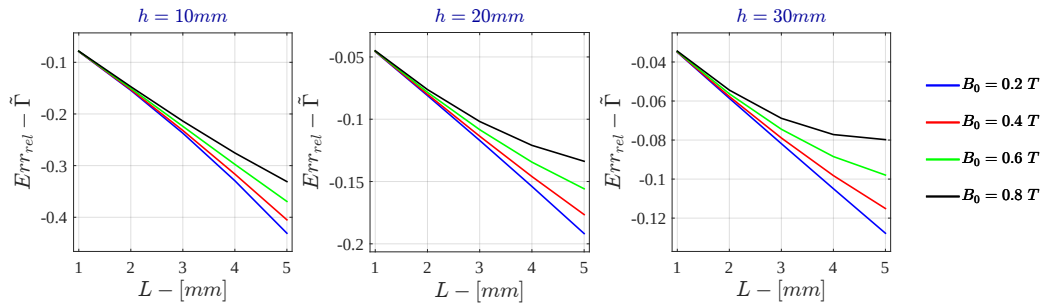
Figure G.16: Monodimensional LPM - Current Drive Relative Error - \tilde{I} for \sigma = 10^3 \text{ S/m} - r_{out} = 50\text{mm}
