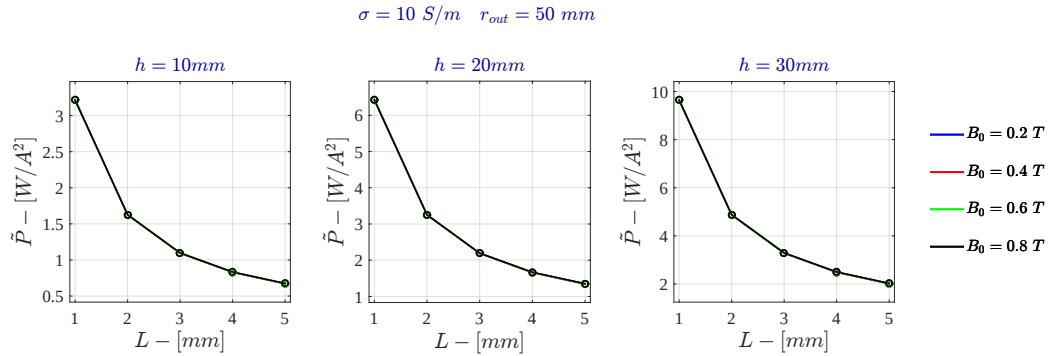
Figure 5.12: Current Drive - Specific Power for \sigma = 10 \text{ S/m} - FDHM
