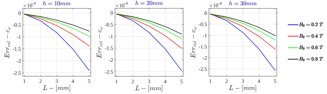
Figure 7.55: Monodimensional LPM Relative Error - c_\omega for \sigma = 10^6 S/m - r_{out} = 50 mm
