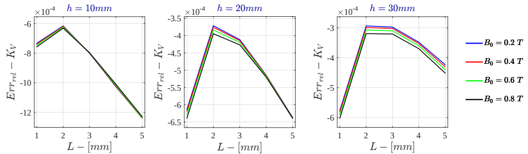
Figure G.8: Monodimensional LPM Relative Error - K_V for \sigma = 10^3 \text{ S/m} - r_{out} = 50\text{mm}
