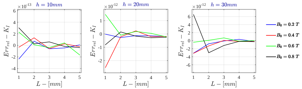
Figure G.30: Bidimensional LPM Relative Error - K_I for \sigma = 10^3 \text{ S/m} - r_{out} = 50\text{mm}
