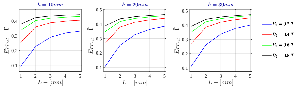
Figure I.40: Bidimensional LPM - Current Drive Relative Error - \tilde{\Gamma} for \sigma = 10^5 \text{ S/m} - r_{out} = 50\text{mm}
