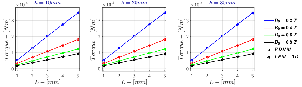
Figure 7.65: Monodimensional LPM - Voltage Drive \dot{\Gamma} for \sigma = 10^6 S/m - r_{out} = 50 mm
