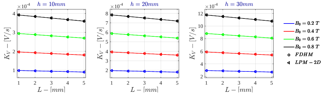
Figure F.28: Bidimensional LPM K_V for \sigma = 10^2 \text{ S/m} - r_{out} = 50 \text{ mm}
