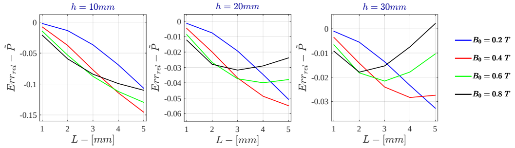
Figure H.15: Monodimensional LPM - Current Drive Relative Error - \tilde{P} for \sigma = 10^4 \text{ S/m} - r_{out} = 50\text{mm}
