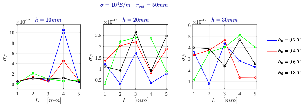
Figure D.6: Current Drive - Standard deviation of the electric current for \sigma = 10^4 \text{ S/m} - FDHM
