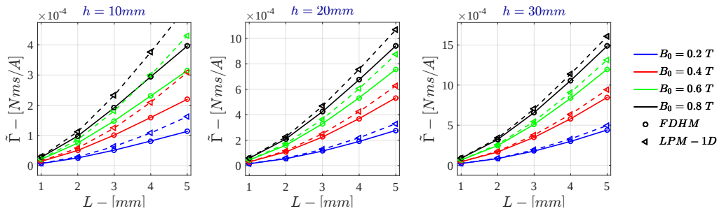
Figure G.12: Monodimensional LPM - Current Drive \tilde{\Gamma} for \sigma = 10^3 \text{ S/m} - r_{out} = 50\text{mm}
