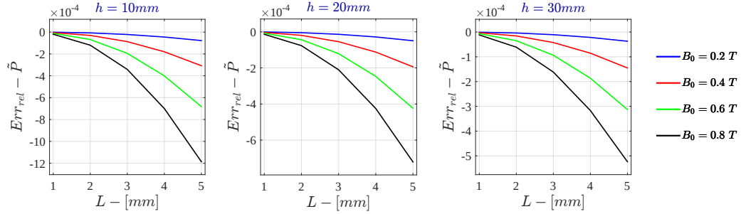
Figure 7.39: Bidimensional LPM - Current Drive Relative Error - \tilde{P} for \sigma = 10 \text{ S/m} - r_{out} = 50\text{mm}
