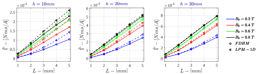
Figure H.12: Monodimensional LPM - Current Drive \dot{\Gamma} for \sigma = 10^4 \text{ S/m} - r_{out} = 50 \text{ mm}
