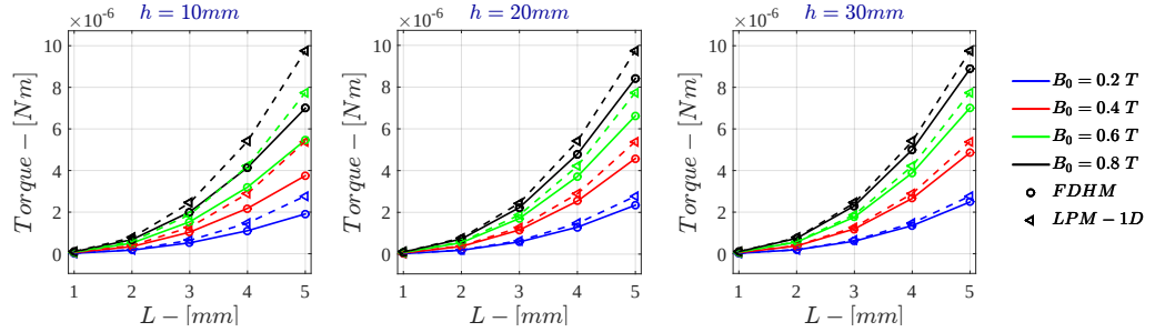
Figure F.17: Monodimensional LPM - Voltage Drive \dot{\Gamma} for \sigma = 10^2 \text{ S/m} - r_{out} = 50\text{mm}
