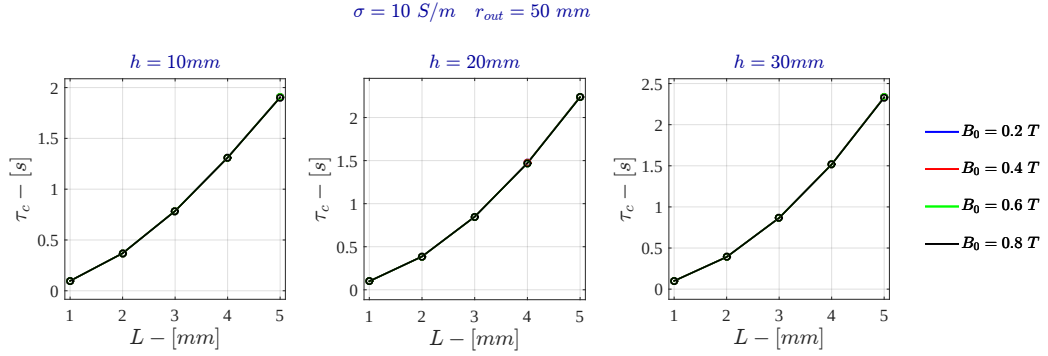
Figure 5.11: Current Drive - Characteristic time for \sigma = 10 \text{ S/m} - FDHM
