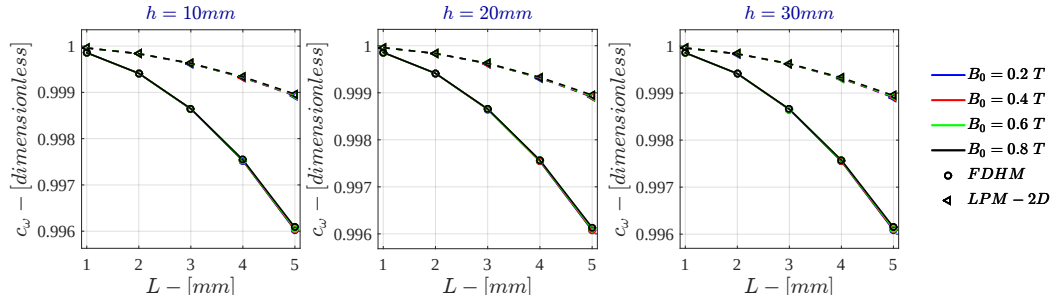
Figure F.27: Bidimensional LPM c_\omega for \sigma = 10^2 \text{ S/m} - r_{out} = 50 \text{ mm}
