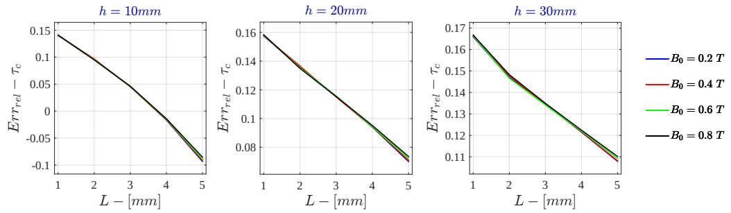
Figure F.14: Monodimensional LPM - Current Drive Relative Error - \tau_c for \sigma = 10^2 \text{ S/m} - r_{out} = 50\text{mm}
