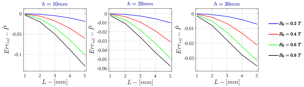
Figure G.15: Monodimensional LPM - Current Drive Relative Error - \tilde{P} for \sigma = 10^3 \text{ S/m} - r_{out} = 50\text{mm}
