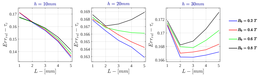
Figure 7.46: Bidimensional LPM - Voltage Drive Relative Error - \tau_c for \sigma = 10 \text{ S/m} - r_{out} = 50\text{mm}
