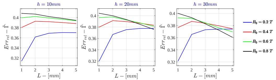
Figure 7.96: Bidimensional LPM - Voltage Drive Relative Error - \tilde{I} for \sigma = 10^6 S/m - r_{out} = 50 mm
