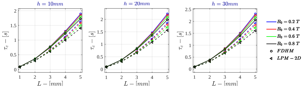
Figure F.42: Bidimensional LPM - Voltage Drive \tau_c for \sigma = 10^2 \text{ S/m} - r_{out} = 50\text{mm}
