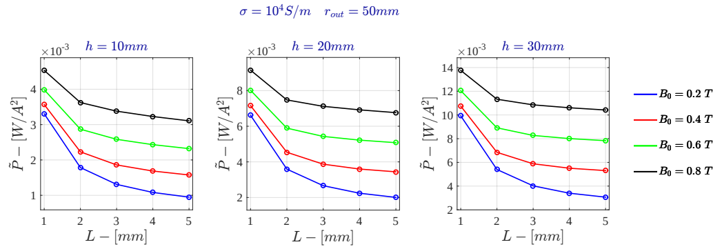
Figure D.3: Current Drive - Specific Power for \sigma = 10^4 \text{ S/m} - FDHM
