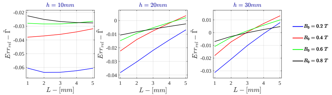
Figure 7.72: Monodimensional LPM - Voltage Drive Relative Error - \tilde{I} for \sigma = 10^6 S/m - r_{out} = 50 mm
