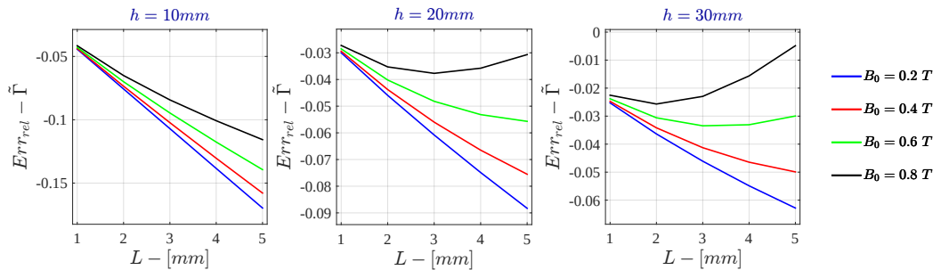
Figure F.48: Bidimensional LPM - Voltage Drive Relative Error - \tilde{I} for \sigma = 10^2 \text{ S/m} - r_{out} = 50\text{mm}
