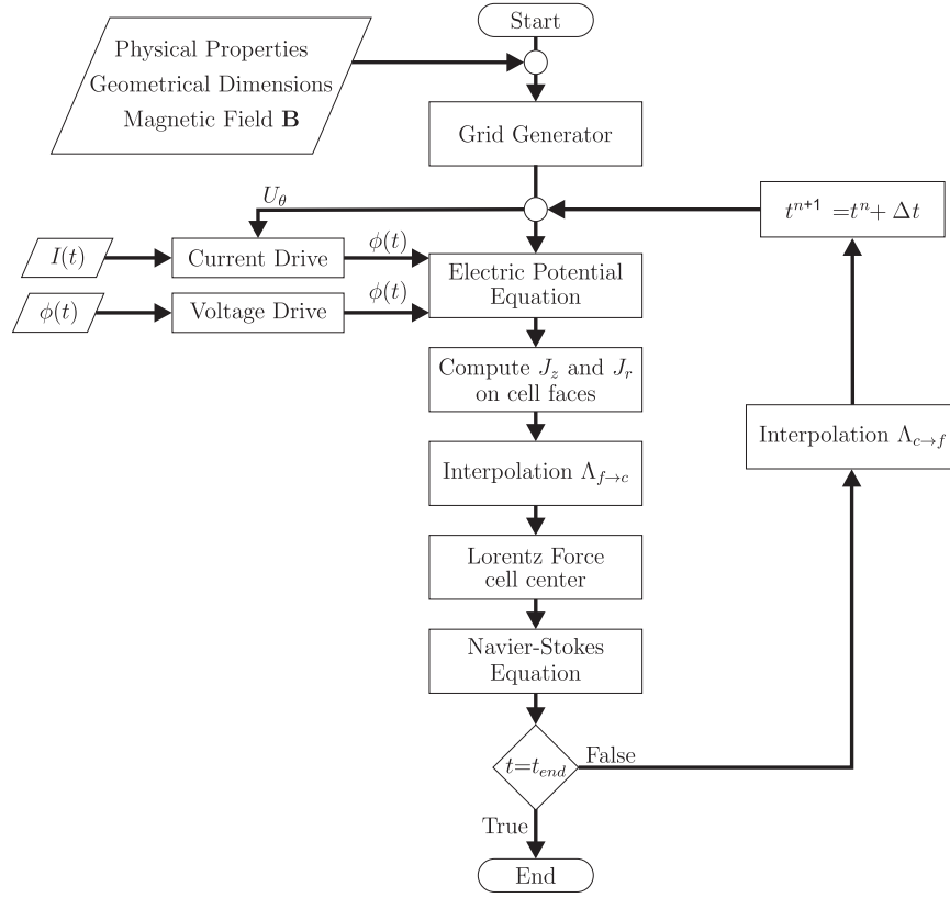
Figure 4.5: Flux Diagram of the FDM model
