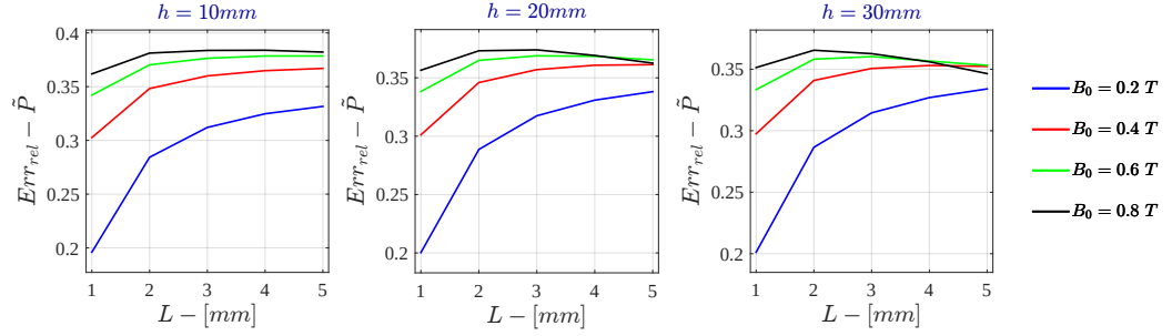
Figure 7.95: Bidimensional LPM - Voltage Drive Relative Error - \tilde{P} for \sigma = 10^6 S/m - r_{out} = 50 mm
