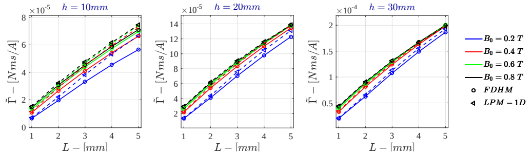
Figure I.20: Monodimensional LPM - Voltage Drive \tilde{\Gamma} for \sigma = 10^5 \text{ S/m} - r_{out} = 50 \text{ mm}
