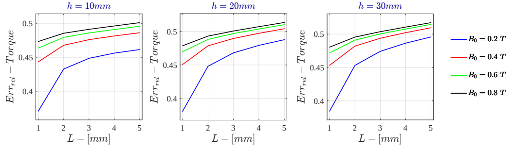
Figure 7.85: Bidimensional LPM - Current Drive Relative Error - \dot{\Gamma} for \sigma = 10^6 S/m - r_{out} = 50 mm
