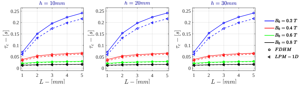
Figure I.18: Monodimensional LPM - Voltage Drive \tau_c for \sigma = 10^5 \text{ S/m} - r_{out} = 50 \text{ mm}
