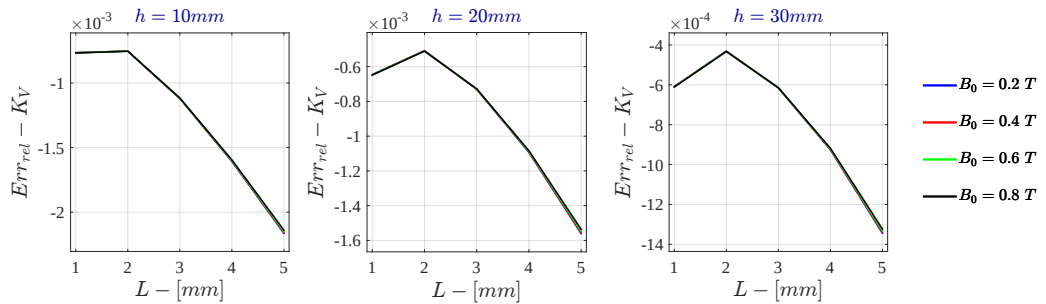
Figure I.32: Bidimensional LPM Relative Error - K_V for \sigma = 10^5 \text{ S/m} - r_{out} = 50\text{mm}
