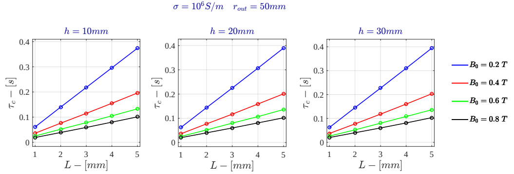
Figure 5.23: Current Drive - Characteristic time for \sigma = 10^6 \text{ S/m} - FDHM
