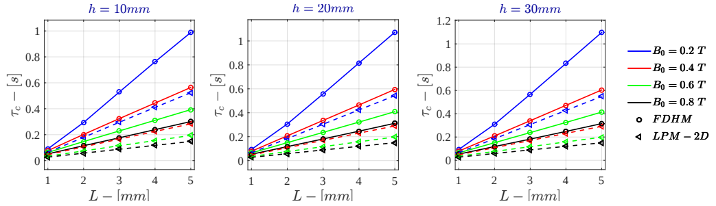
Figure I.34: Bidimensional LPM - Current Drive \tau_c for \sigma = 10^5 \text{ S/m} - r_{out} = 50 \text{ mm}
