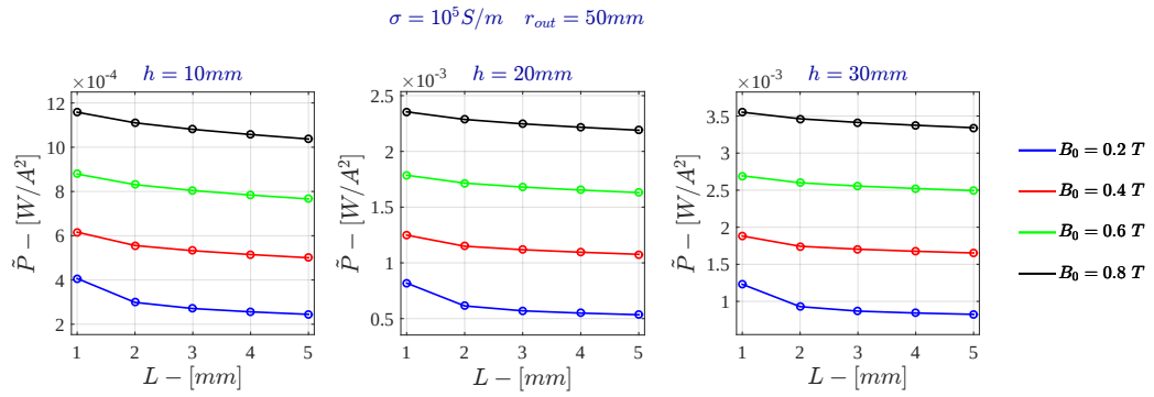
Figure E.3: Current Drive - Specific Power for \sigma = 10^5 \text{ S/m} - FDHM
