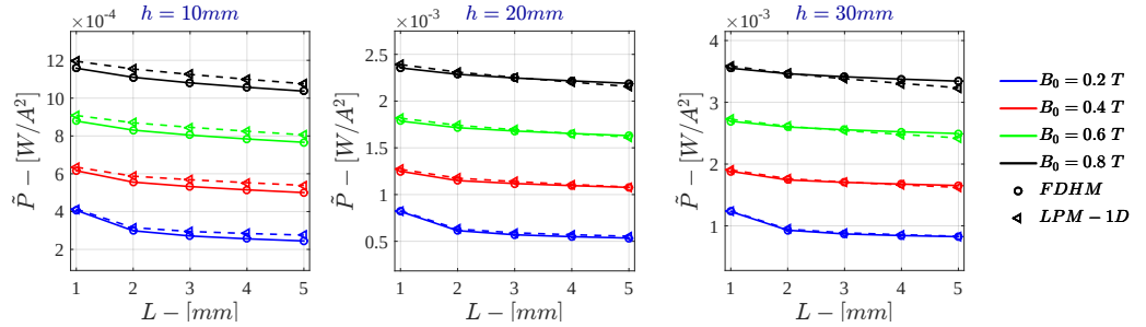
Figure I.11: Monodimensional LPM - Current Drive \dot{P} for \sigma = 10^5 \text{ S/m} - r_{out} = 50\text{mm}
