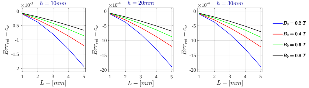
Figure I.31: Bidimensional LPM Relative Error - c_\omega for \sigma = 10^5 \text{ S/m} - r_{out} = 50\text{mm}
