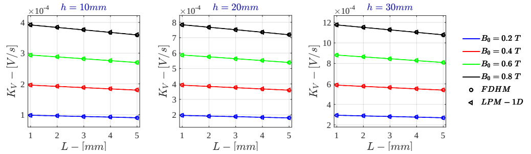
Figure 7.4: Monodimensional LPM K_V for \sigma = 10 S/m - r_{out} = 50mm
