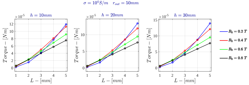
Figure D.7: Voltage Drive - Torque for \sigma = 10^4 \text{ S/m} - FDHM
