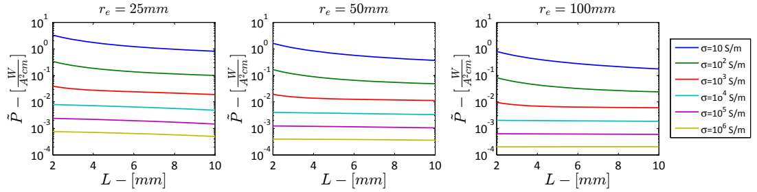
Figure 8.8: Power consumption function of L for \sigma = 10 \div 10^6 S/m and 3 different outer radii r_e = 25, 50, 100mm . B_0 = 1.0 T . \rho = 1000 Kg/m^3 .
