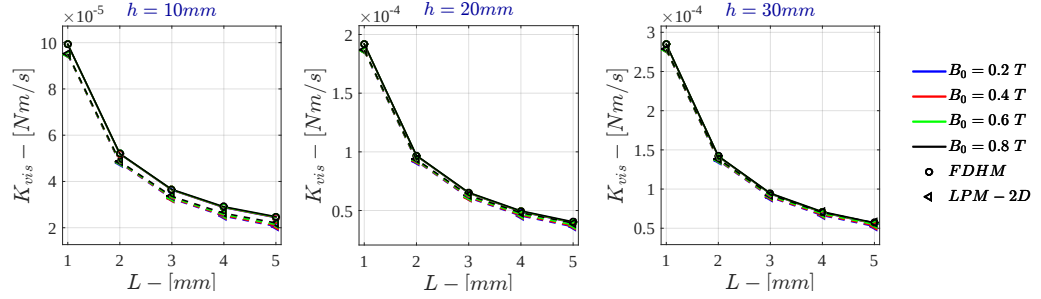
Figure F.25: Bidimensional LPM K_{vis} for \sigma = 10^2 \text{ S/m} - r_{out} = 50 \text{ mm}
