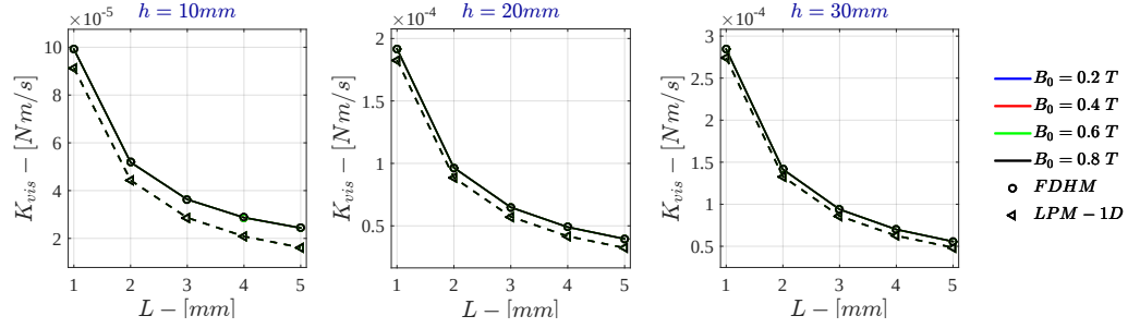
Figure 7.1: K_{vis} for \sigma = 10 S/m - r_{out} = 50mm - Monodimensional LPM
