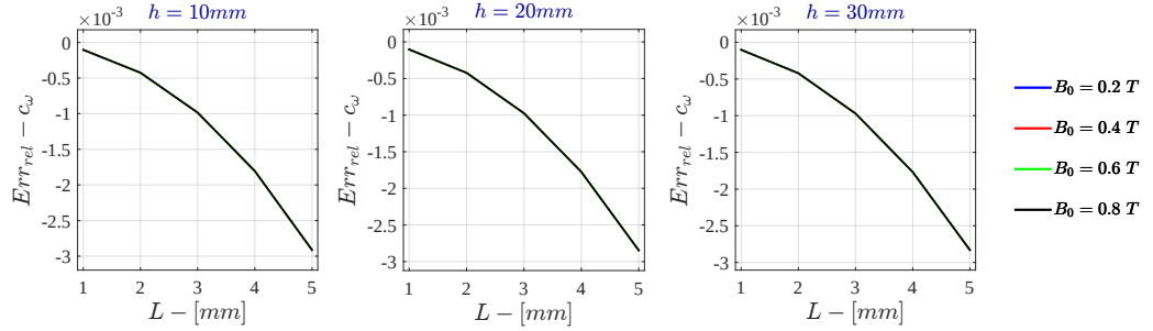
Figure 7.31: Bidimensional LPM Relative Error - c_{\omega} for \sigma = 10 S/m - r_{out} = 50 mm
