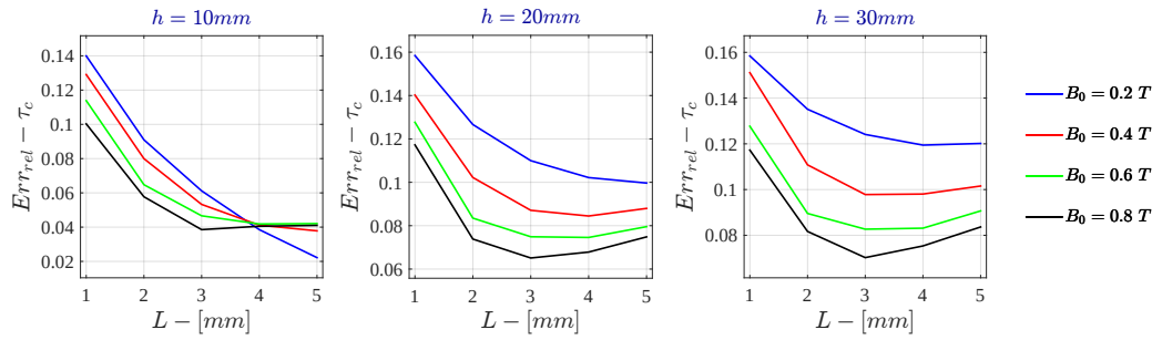
Figure I.14: Monodimensional LPM - Current Drive Relative Error - \tau_c for \sigma = 10^5 \text{ S/m} - r_{out} = 50\text{mm}
