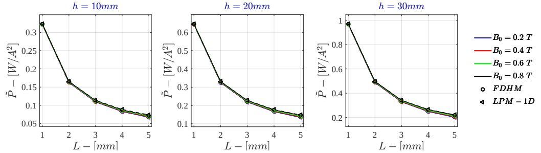
Figure I.19: Monodimensional LPM - Voltage Drive \dot{P} for \sigma = 10^5 \text{ S/m} - r_{out} = 50 \text{ mm}
