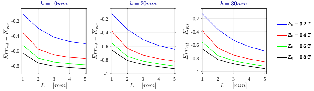
Figure I.29: Bidimensional LPM Relative Error - K_{vis} for \sigma = 10^5 \text{ S/m} - r_{out} = 50\text{mm}
