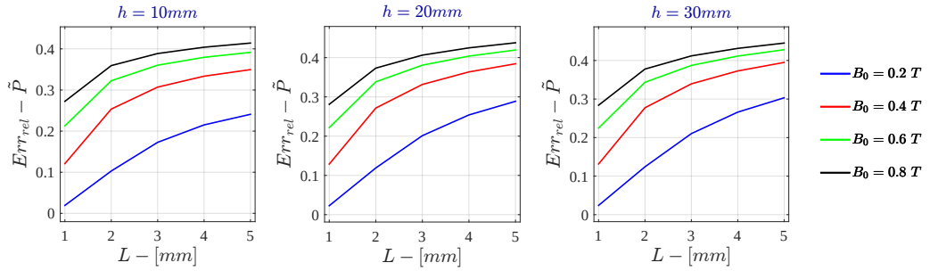
Figure I.39: Bidimensional LPM - Current Drive Relative Error - \tilde{P} for \sigma = 10^5 \text{ S/m} - r_{out} = 50\text{mm}
