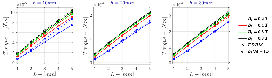
Figure I.33: Bidimensional LPM - Current Drive \dot{\Gamma} for \sigma = 10^5 \text{ S/m} - r_{out} = 50 \text{ mm}
