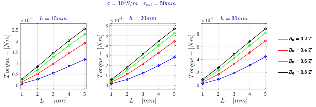
Figure D.1: Current Drive - Torque for \sigma = 10^4 \text{ S/m} - FDHM
