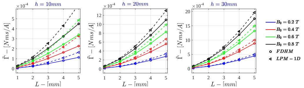
Figure F.12: Monodimensional LPM - Current Drive \tilde{\Gamma} for \sigma = 10^2 \text{ S/m} - r_{out} = 50\text{mm}
