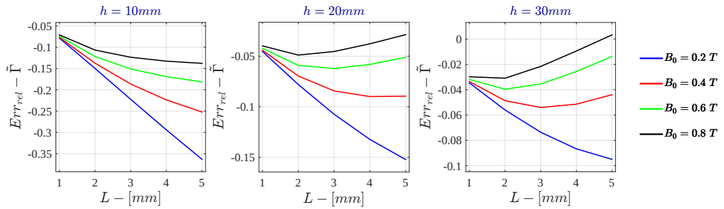
Figure H.16: Monodimensional LPM - Current Drive Relative Error - \tilde{\Gamma} for \sigma = 10^4 \text{ S/m} - r_{out} = 50\text{mm}
