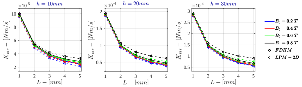
Figure G.25: Bidimensional LPM K_{vis} for \sigma = 10^3 \text{ S/m} - r_{out} = 50\text{mm}
