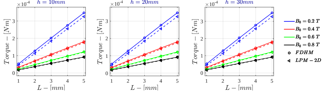
Figure 7.89: Bidimensional LPM - Voltage Drive \dot{\Gamma} for \sigma = 10^6 S/m - r_{out} = 50 mm
