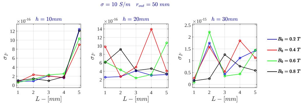
Figure 5.21: Voltage Drive - Standard deviation of the electric current for \sigma = 10 \text{ S/m} - FDHM
