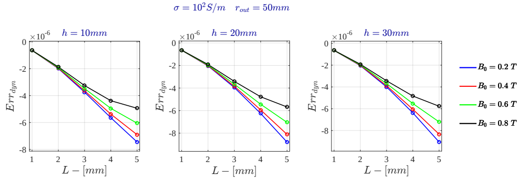
Figure B.11: Voltage Drive - Relative Dynamic Error for \sigma = 10^2 \text{ S/m} - FDHM
