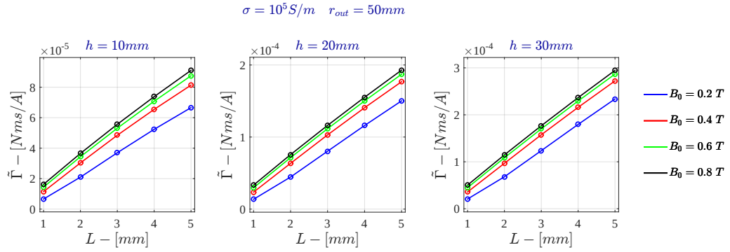
Figure E.4: Current Drive - Specific Angular Momentum for \sigma = 10^5 \text{ S/m} - FDHM
