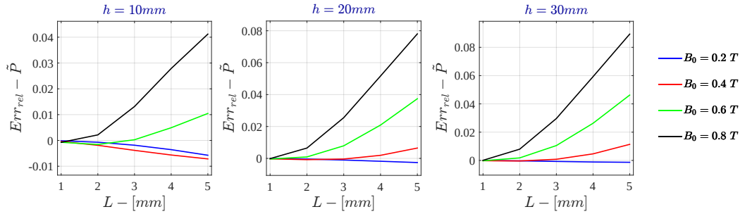
Figure G.47: Bidimensional LPM - Voltage Drive Relative Error - \tilde{P} for \sigma = 10^3 \text{ S/m} - r_{out} = 50\text{mm}
