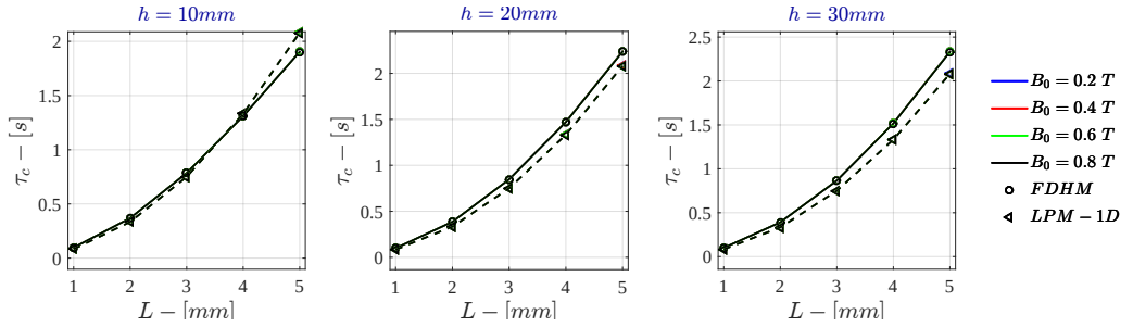
Figure 7.10: Monodimensional LPM - Current Drive \tau_c for \sigma = 10 \text{ S/m} - r_{out} = 50 \text{ mm}
