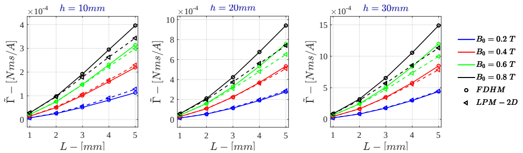
Figure G.36: Bidimensional LPM - Current Drive \tilde{\Gamma} for \sigma = 10^3 \text{ S/m} - r_{out} = 50\text{mm}
