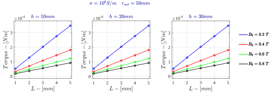
Figure 5.28: Voltage Drive - Torque for \sigma = 10^6 \text{ S/m} - FDHM
