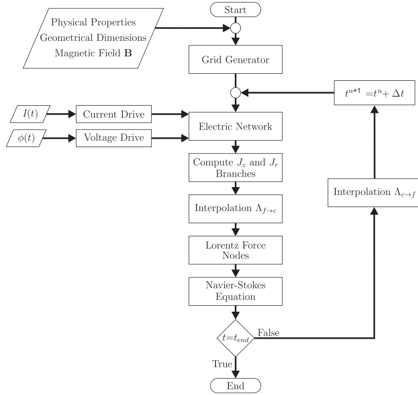
Figure 4.9: Flux Diagram of the FDHM model
