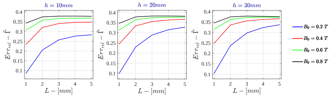
Figure I.48: Bidimensional LPM - Voltage Drive Relative Error - \dot{\Gamma} for \sigma = 10^5 \text{ S/m} - r_{out} = 50\text{mm}
