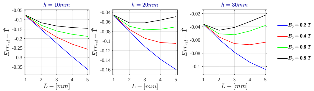
Figure H.24: Monodimensional LPM - Voltage Drive Relative Error - \tilde{I} for \sigma = 10^4 \text{ S/m} - r_{out} = 50\text{mm}
