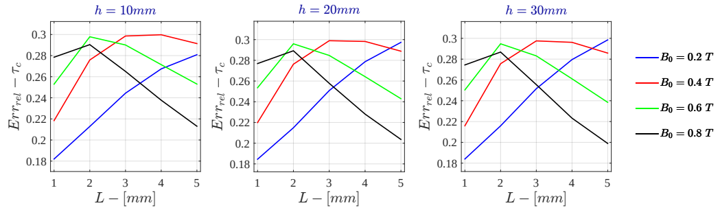
Figure H.46: Bidimensional LPM - Voltage Drive Relative Error - \tau_c for \sigma = 10^4 \text{ S/m} - r_{out} = 50\text{mm}
