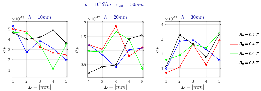
Figure B.6: Current Drive - Standard deviation of the electric current for \sigma = 10^2 \text{ S/m} - FDHM
