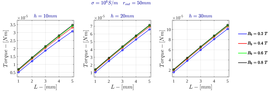
Figure 5.22: Current Drive - Torque for \sigma = 10^6 \text{ S/m} - FDHM
