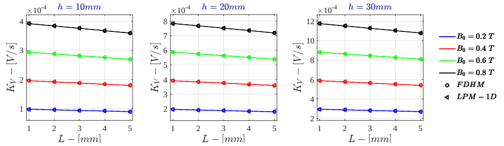
Figure F.4: Monodimensional LPM K_V for \sigma = 10^2 \text{ S/m} - r_{out} = 50 \text{ mm}
