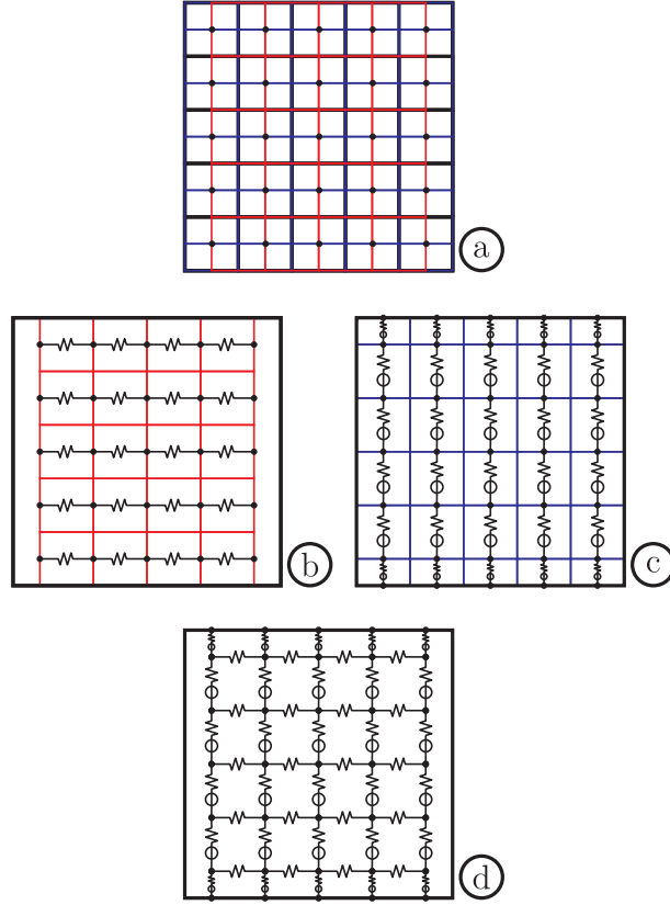
Figure 4.8: Equivalent electric network.
