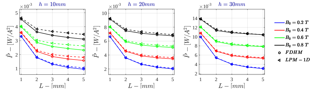
Figure H.35: Bidimensional LPM - Current Drive \tilde{P} for \sigma = 10^4 \text{ S/m} - r_{out} = 50\text{mm}
