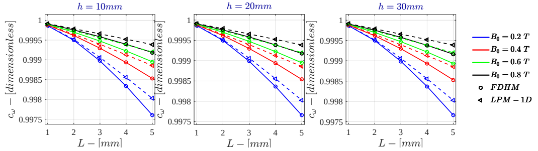
Figure I.3: Monodimensional LPM c_\omega for \sigma = 10^5 \text{ S/m} - r_{out} = 50 \text{ mm}
