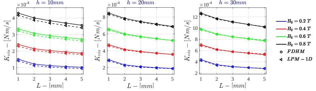
Figure 7.49: K_{vis} for \sigma = 10^6 S/m - r_{out} = 50mm - Monodimensional LPM
