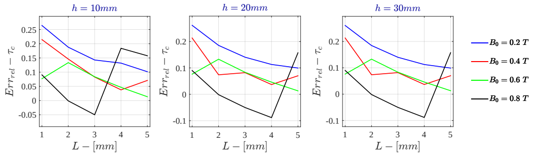
Figure 7.94: Bidimensional LPM - Voltage Drive Relative Error - \tau_c for \sigma = 10^6 S/m - r_{out} = 50 mm
