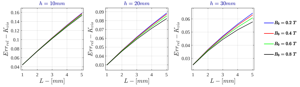
Figure 7.29: Bidimensional LPM Relative Error - K_{vis} for \sigma = 10 S/m - r_{out} = 50 mm
