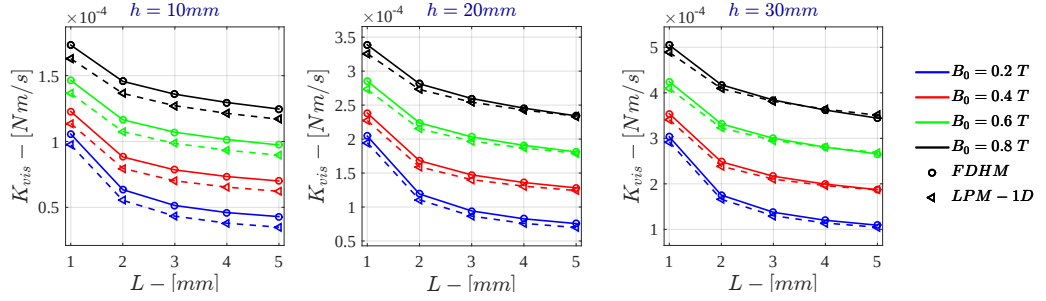
Figure I.1: K_{vis} for \sigma = 10^5 \text{ S/m} - r_{out} = 50 \text{ mm} - Monodimensional LPM
