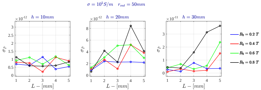
Figure E.6: Current Drive - Standard deviation of the electric current for \sigma = 10^5 \text{ S/m} - FDHM
