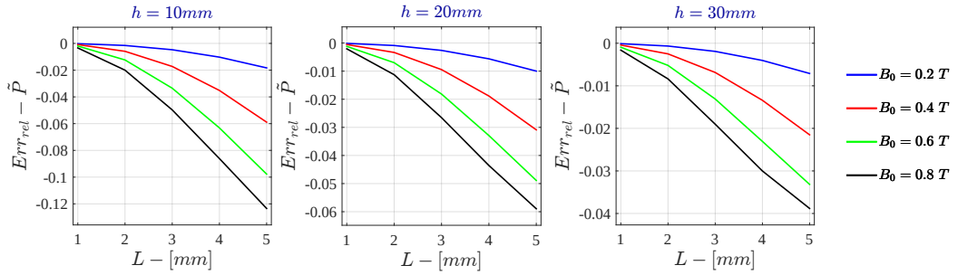
Figure G.23: Monodimensional LPM - Voltage Drive Relative Error - \tilde{P} for \sigma = 10^3 \text{ S/m} - r_{out} = 50\text{mm}
