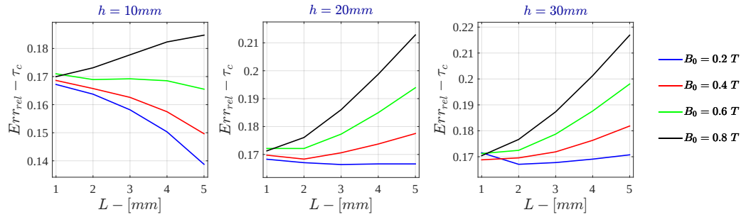
Figure F.46: Bidimensional LPM - Voltage Drive Relative Error - \tau_c for \sigma = 10^2 \text{ S/m} - r_{out} = 50\text{mm}
