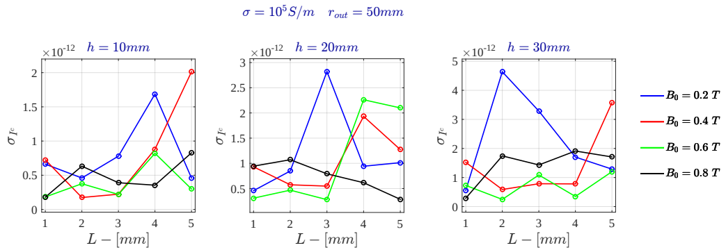
Figure E.12: Voltage Drive - Standard deviation of the electric current for \sigma = 10^5 \text{ S/m} - FDHM
