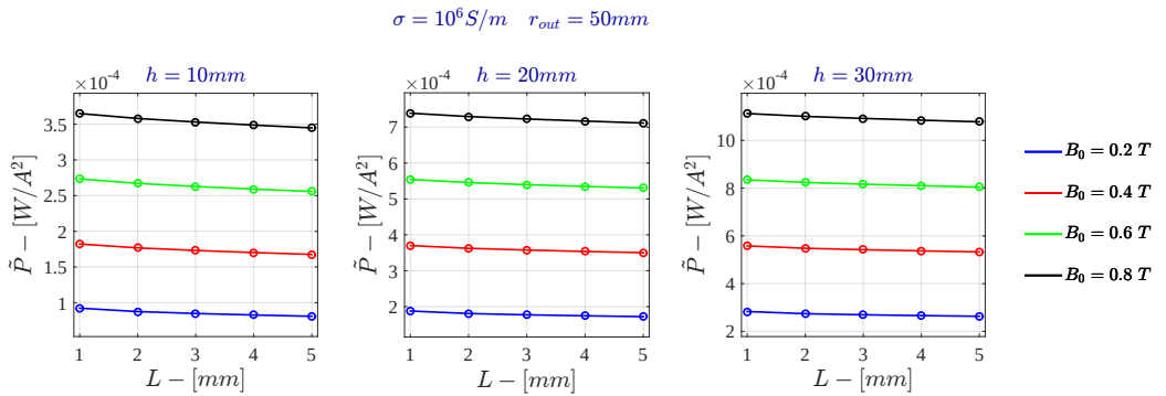
Figure 5.24: Current Drive - Specific Power for \sigma = 10^6 \text{ S/m} - FDHM
