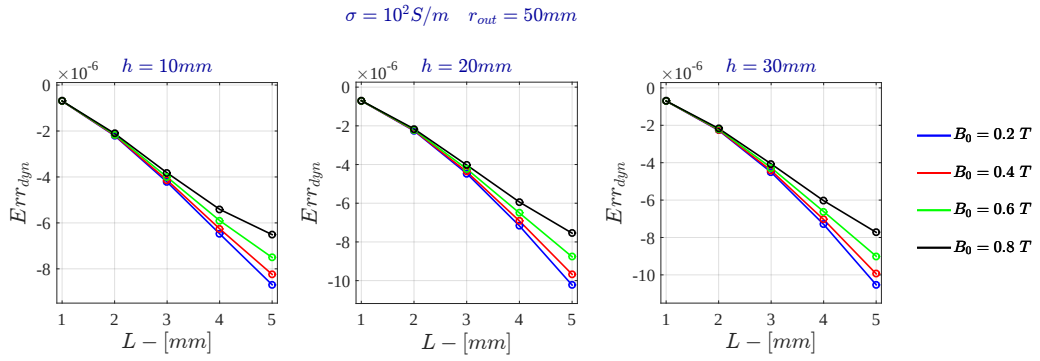
Figure B.5: Current Drive - Relative Dynamic Error for \sigma = 10^2 \text{ S/m} - FDHM
