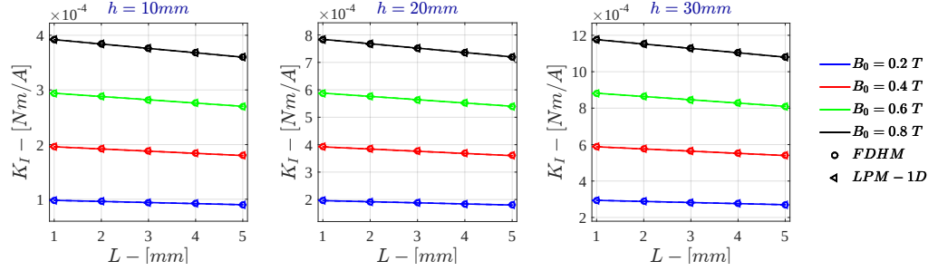
Figure I.2: Monodimensional LPM K_I for \sigma = 10^5 \text{ S/m} - r_{out} = 50 \text{ mm}
