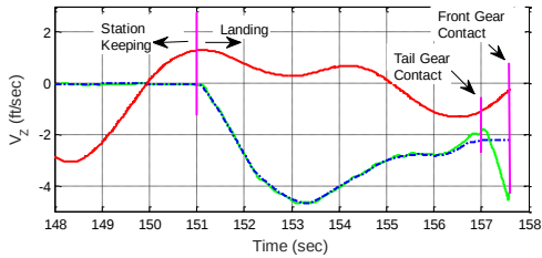
Figure 3. Lateral and Vertical Velocities of C.G.
