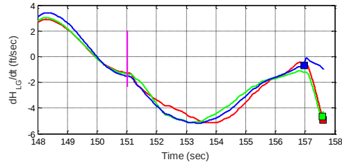
Figure 4. Height and Vertical Velocity of Landing Gear Relative to Deck
